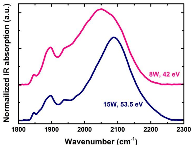
Figure 4.16 FTIR spectra in range from 1800 to 2300 \text{ cm}^{-1} for two reference \mu\text{-Si:H} films deposited using standard single-frequency (13.56 MHz) excitation source.
