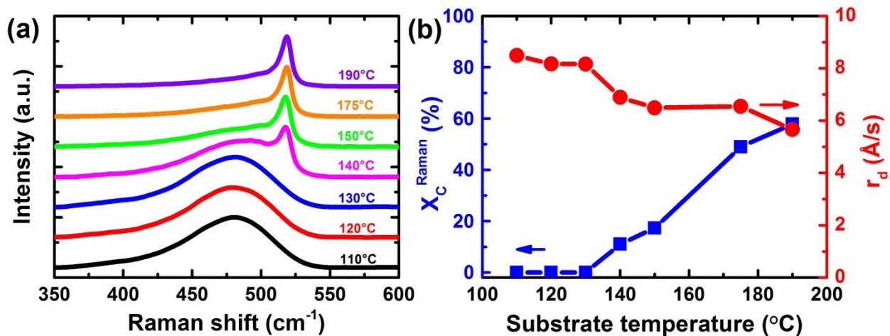
Figure 3.3 (a) Raman spectra for films deposited at different temperatures. (b) Variation of X_C^{\text{Raman}} (left axis, blue square) and r_d (right axis, red circle) for these films deposited with varying temperature.
