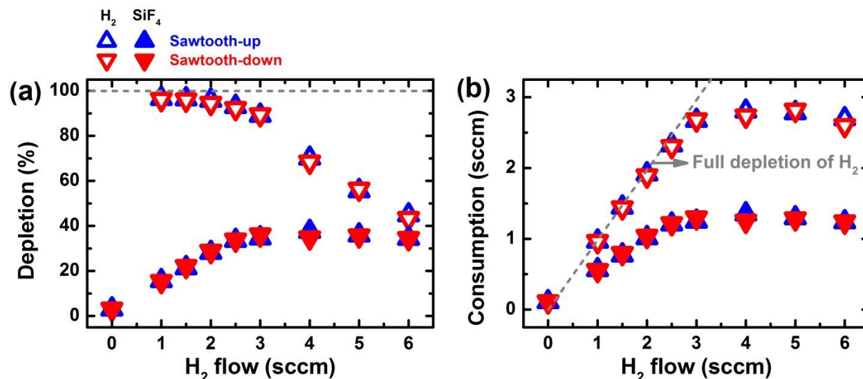
Figure 5.10 (a) Depletion and (b) consumption of H 2 (open symbols) and SiF 4 (solid symbols) as a function of H 2 flow rate, as measured using RGA. The dashed line in (b) indicates the full depletion of H 2 .
