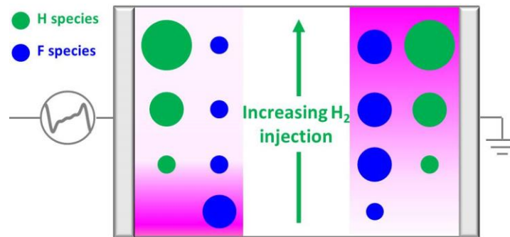
Figure 5.17 Qualitative comparison of hydrogen and active fluorinated concentration (v): varying H_2 flow.
