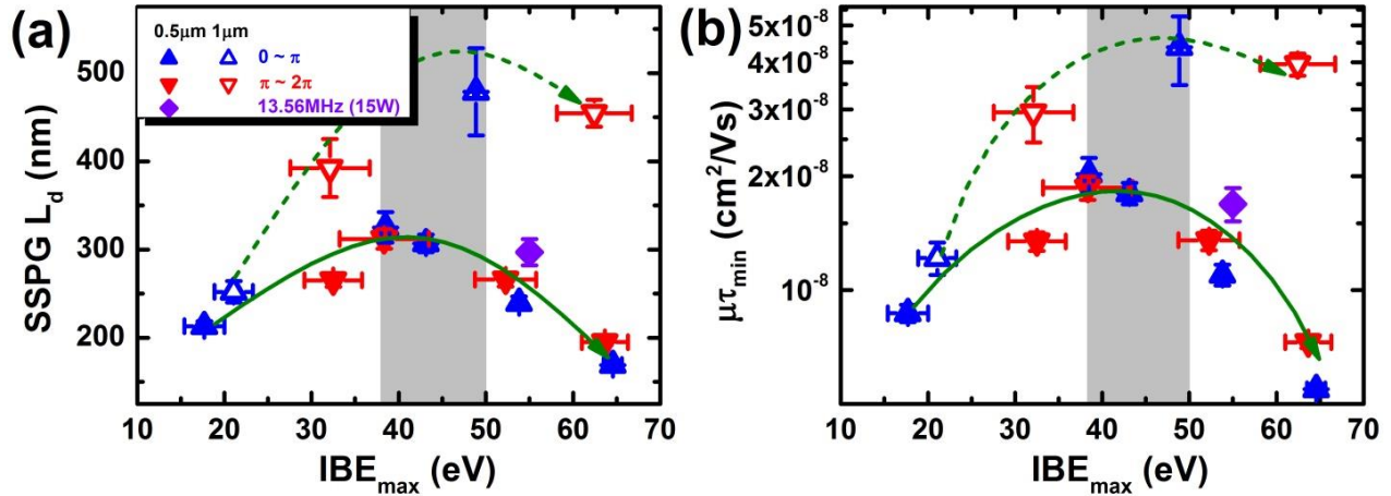
Figure 4.17 Variation of (a) L_d and (b) \mu\tau_{min} at room temperature for two sets of \mu\text{c-Si:H} films with varying IBE_{max} . The solid and open triangles correspond to films with 0.5 \mu\text{m} and 1 \mu\text{m} thickness, respectively. The purple diamond corresponds to the 0.5 \mu\text{m} thick reference film.
