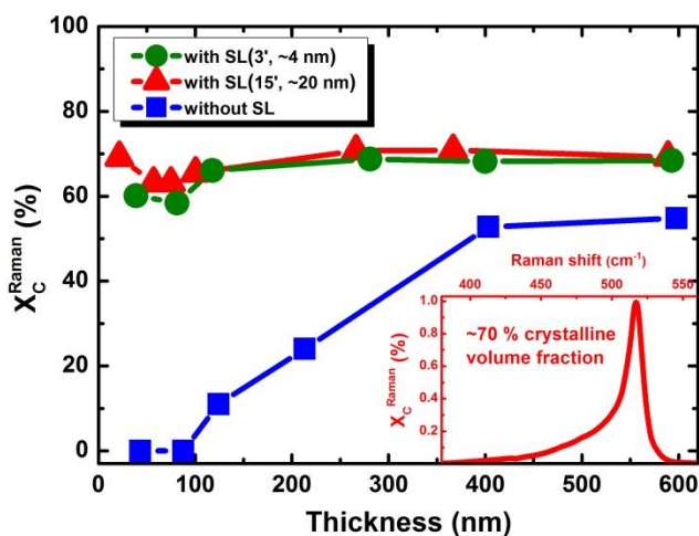
Figure 3.16 Evolution of X_c^{Raman} during growth process for \mu c-Si:H films with \sim 4 nm (green circles) and \sim 20 nm seed layer (red triangles) deposition compared to one-step process deposited films (blue squares). The inset shows the Raman spectra of the \sim 20 nm seed layer.
