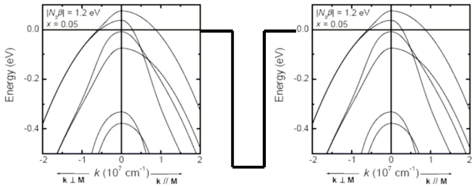
Figure 55: Transmission of electrons through tunnel barrier in the VB with the magnetization direction perpendicular to the wavevector in the contacts.
