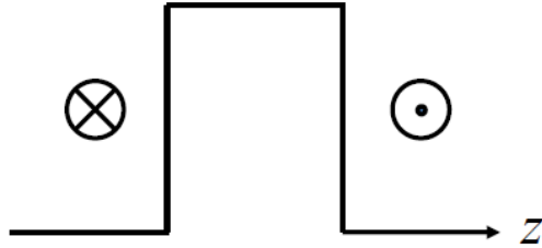
Figure 47: Tunnel junction grown along the z direction with Rashba SOI in the barrier under AP configuration, \vec{M} \parallel x , \vec{k}_{\parallel} = (0, \xi) .
