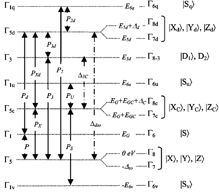
Figure 32: Wave functions in the 30-band \mathbf{k.p} model at \mathbf{k}=0 for O_h group [57].
