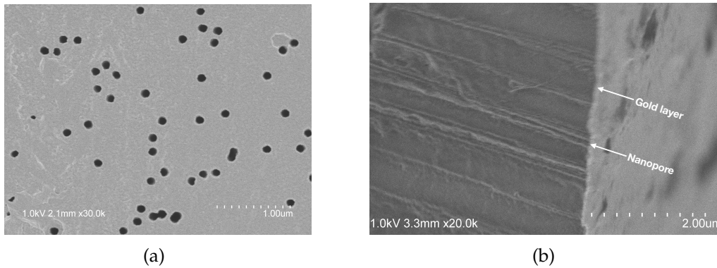
FIGURE 8.4: (a). FESEM image of the PVDF surface after chemical etching (fluence 5.10^8.\text{cm}^{-2} ); (b). Cross-section of the PVDF .
