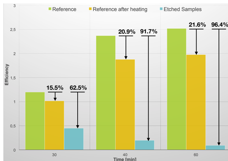
FIGURE 9.12: chemical etching impact on the electric efficiency. Etching times: 30, 40 and 60 minutes. PVDF Reference (■), temperature (■) and chemical etching (■) impact on the electrical efficiency.
