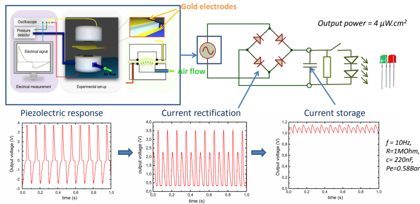
FIGURE 9.2: electrical circuit used to harvest energy from a piezoelectric PVDF film.
