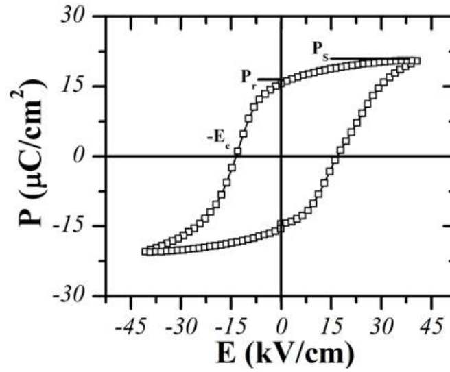
FIGURE 2.3: Hysteresis loop for a general ferroelectric material.
