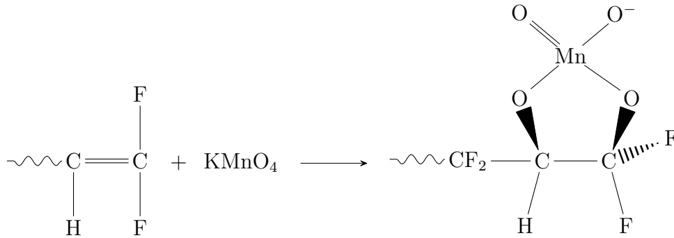
FIGURE 5.3: Typical reaction mechanism between double bond in PVDF chain termination and Potassium permanganate
