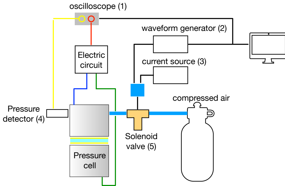
FIGURE 7.3: experimental set-up. (1) - PicoScope 4000 series; (2) - KEITHLEY 3390 waveform generator; (3) - ISO-TECH DC power supply IPS 303DD; (4) - GEMS pressure sensor; (5) - Solenoid valve SMC VDW250.
