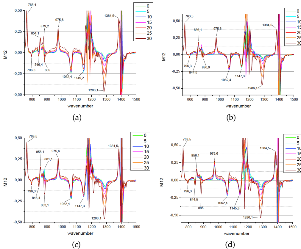
FIGURE 9.8: spectra dichroism matrix M_{12} function of \theta angle (range 0 - 30deg) for irradiated PVDF. Irradiation doses: (a). 5kGy; (b). 10kGy; (c). 50 kGy; (d). 100kGy.
