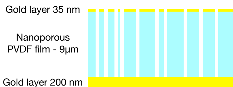
FIGURE 5.4: Nanoporous PVDF with double gold layer
