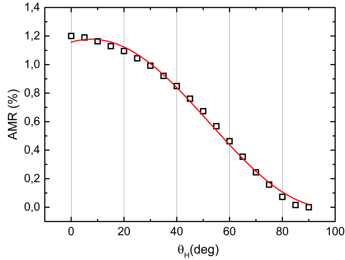
FIGURE 5.10: AMR vs \theta_H ( H=10\text{kOe} ). Fit function: 1.178\cos^2(\theta - 7.57) .
