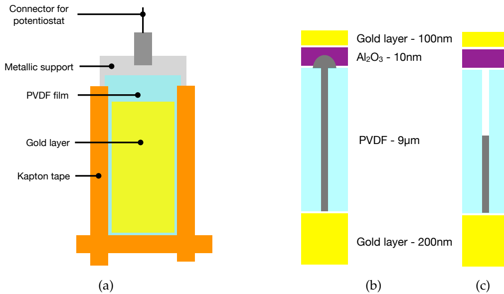
FIGURE 7.1: (a). Preparation sample for electrodeposition; (b). Cross-section of the PVDF film with electrodeposited Ni NW and multi-layer Al 2 O 3 /Au on the top; (c) intermediate electrodeposition time.
