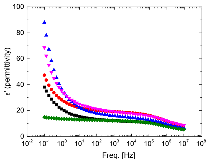
FIGURE 9.15: dielectric permittivity ( \epsilon' ) for nanostructured samples. PVDF reference ( \blacklozenge ), nanoporous PVDF/ Al_2O_3 layer ( \blacksquare ), Electrodeposition times of the Ni NWs: 50 ( \bullet ), 100 ( \blacktriangle ), 150 seconds ( \blacktriangledown ).
