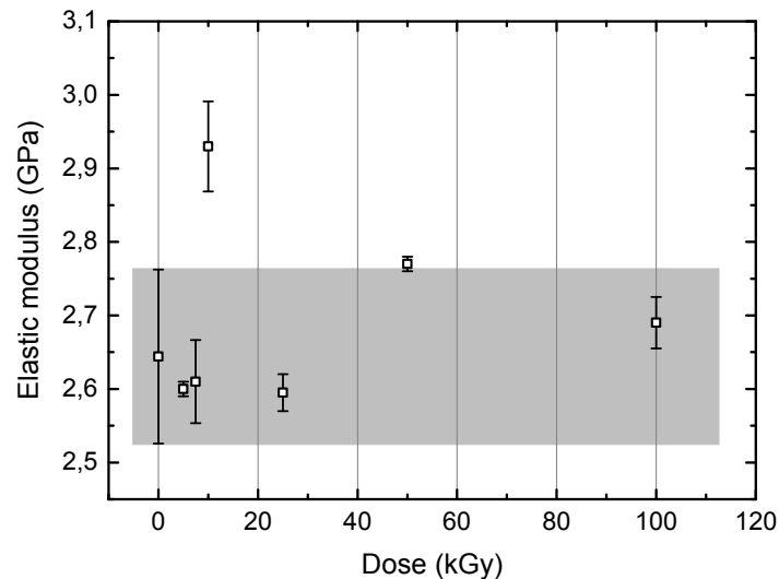
FIGURE 9.10: elastic modulus versus e-beam radiation doses (kGy).
