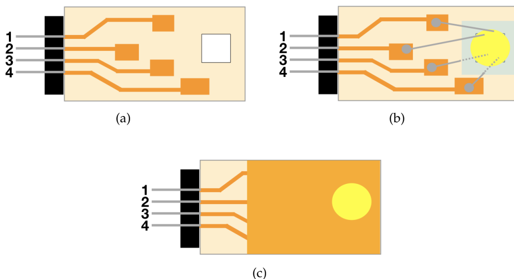
FIGURE 5.5: Preparation sample for electrodeposition: (a) printed silicate plate with peltier plate (white square in the figure); (b) PVDF film is fixed on the peltier plate and four Contacts are provided for each pin; (c) The contacts are protected by kapton tape. Only a small area is exposed to the electrolyte.
