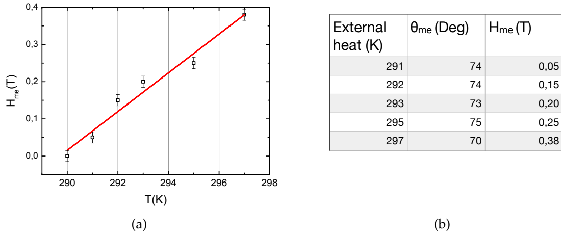
FIGURE 6.7: (a). Magnetoelastic field induced by the external stress on the Ni NW as a function of the temperature. The linear fit yields a slope of about 0.05T.K^{-1} ; (b). Parameters at various temperatures for the AMR fit. H_{me} is deduced from the equation 4.19
