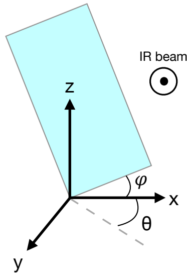
FIGURE 8.8: orientation of the PVDF film respect to IR beam: rotation around y ( \varphi angle) and z ( \theta angle) axis.
