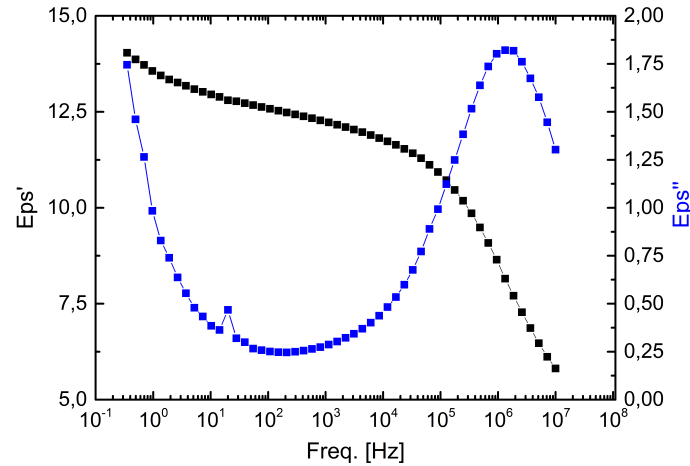
FIGURE 8.9: \epsilon' and \epsilon'' function of frequency.
