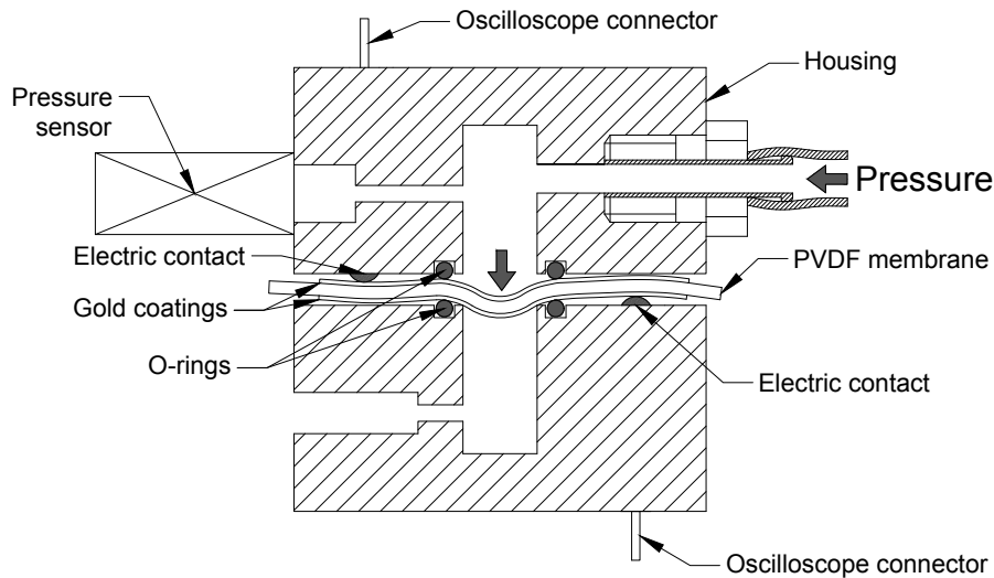
FIGURE 7.2: section of the pressure cell. Pressure chamber in contact with the PVDF film.
