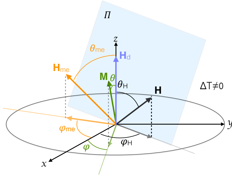
FIGURE 6.6: out-of-plane vectors due to \vec{H}_{me}
