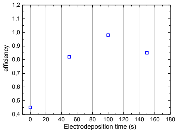
FIGURE 9.14: electrical efficiency versus electrodeposition time (s).
