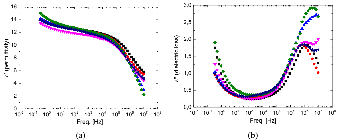
FIGURE 9.9: (a). Dielectric permittivity ( \epsilon' ); and (b) dielectric loss ( \epsilon'' ) at e-beam radiation doses (kGy): 0 (■), 5 (●), 10 (▲), 25 (▼), 50 (◆), 100 (◄)
