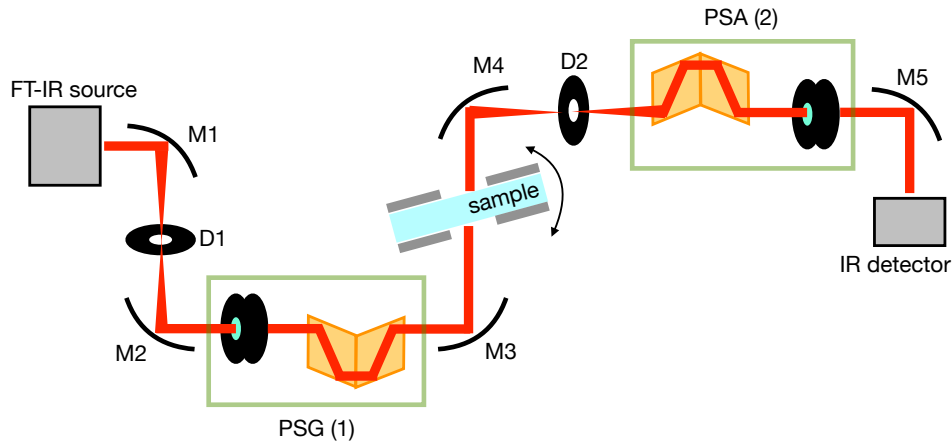
FIGURE 8.7: schema of the IR Mueller ellipsometer. (1) polarization state generator in the entry arm; (2) polarization state analyzer in the exit arm; D1-D2: diaphragms; M1-M5 mirrors.
