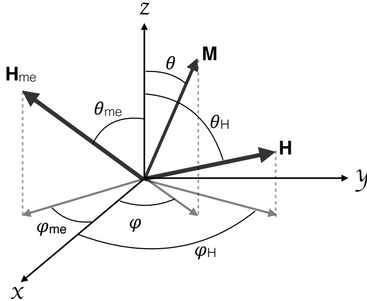
FIGURE 4.4: 3D orientation of the magnetization, magnetic and magnetoelastic field respect to NW-axis (z-axis).
