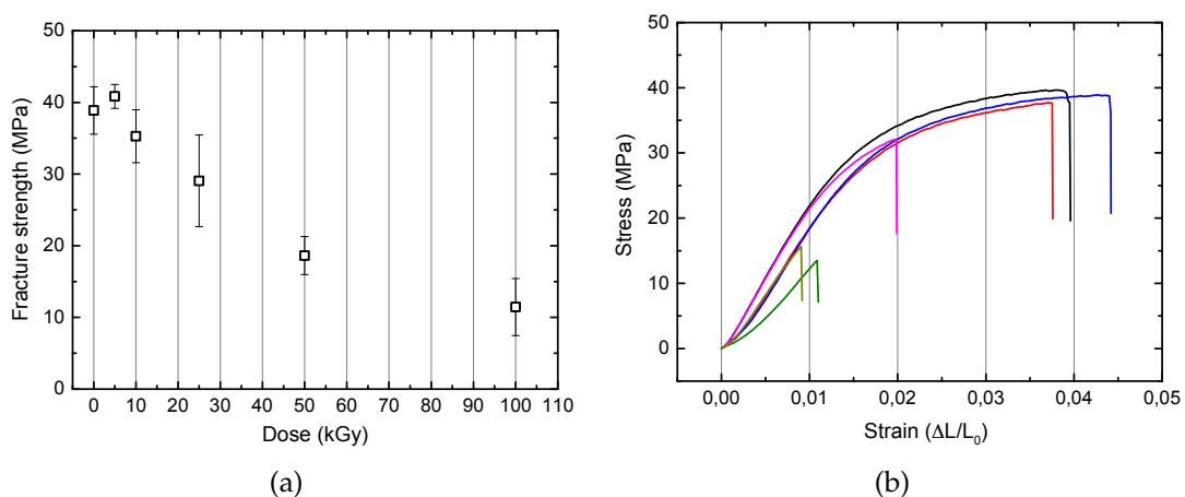
FIGURE 9.11: (a). Fracture strength (MPa) versus e-beam radiation doses (kGy) of a copolymer P(VDF-TrFe)(70/30); (b). Stress-Strain curves of an irradiated copolymer P(VDF-TrFe)(70/30) at different doses (kGy): 0 (black line), 5 (red line), 10 (blue line), 25 (magenta line), 50 (olive line), 100 (green line).
