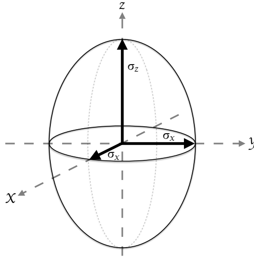
FIGURE 4.5: Prolate-spheroid shape of \beta -PVDF stress \sigma occurring in the polymer film during thermal expansion.
