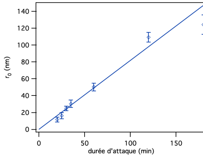
FIGURE 8.6: average radius versus etching time. Irradiation fluence 5.10^8 .cm^{-2} . Equation fit: r_0 = (0.82 \pm 0.05)t . [72]
