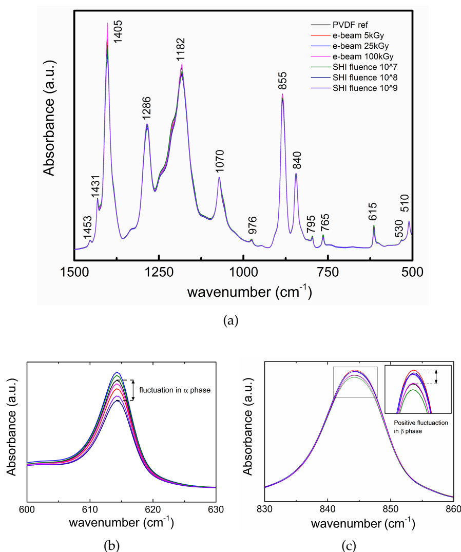
FIGURE 9.6: (a). FT-IR spectra in transmission mode of polarized bi-oriented polarized PVDF treated at various doses using electrons (normalized band was 1070\text{ cm}^{-1} ): 0 kGy (black line), 5 kGy (red line), 25 kGy (blue line) and 100 kGy (magenta line) and using SHI at doses of 0.076 kGy (green line), 0.76 kGy (cyan line) and 7.6 kGy (violet line). (b). 615\text{ cm}^{-1} \alpha peak. (c) 840\text{ cm}^{-1} \beta peak.
