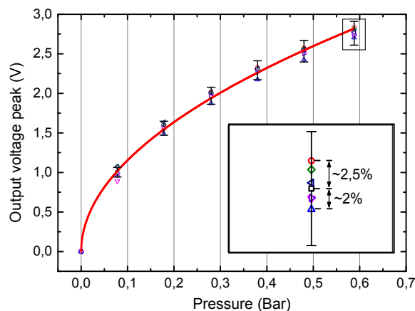
FIGURE 9.3: irradiated polarized PVDF films output voltages at various pressures – PVDF reference: (□); electron irradiated doses: 5kGy (○), 25kGy (△), 100kGy (▽); SHI irradiated doses: 0.076 kGy (◇), 0.76 kGy (◁), 7.6 kGy (▷).
