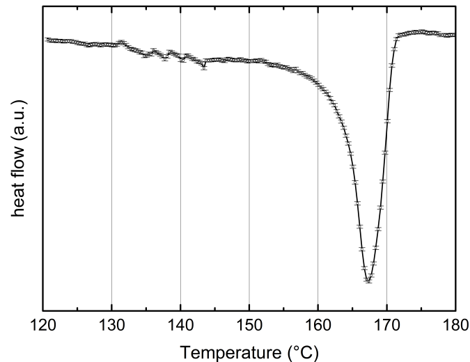
FIGURE 8.3: DSC melting peak of neat PVDF.
