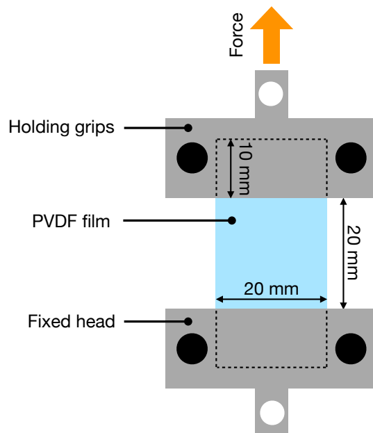
FIGURE 8.10: collets for tensile test measurement.
