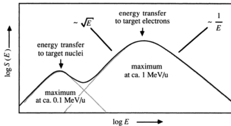
FIGURE 3.1: Qualitative shape of stopping function S(E) versus kinetic energy E of the projectile-ion. [29]
