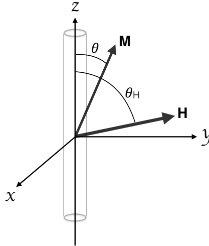
FIGURE 4.1: Orientation of the magnetization and external magnetic field respect to NW-axis.
