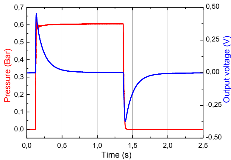
FIGURE 7.5: output voltage under cycling bending stress condition. Frequency=0.4Hz; width=1.25s; \Delta P=0.6\text{bar} ; R_1=20\text{M}\Omega
