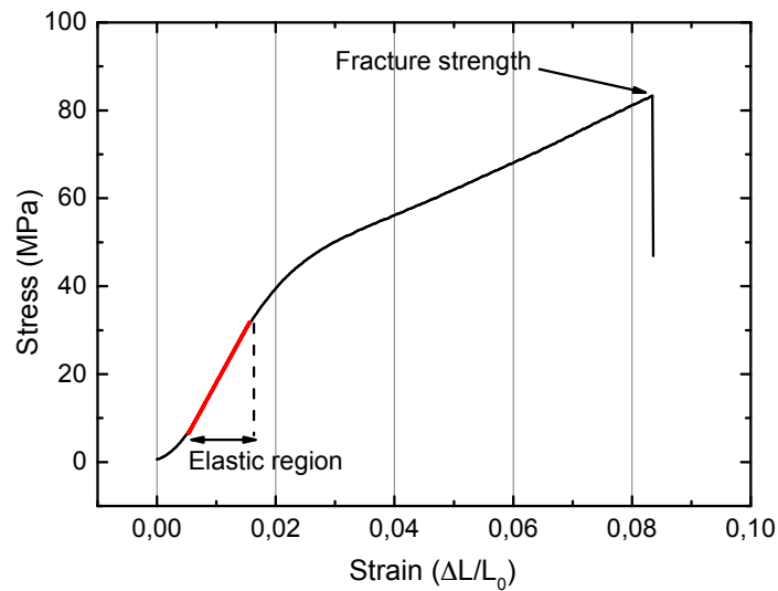
FIGURE 8.11: Stress vs strain of neat PVDF film. fit function: \sigma = -6,475 + 2454,45\epsilon
