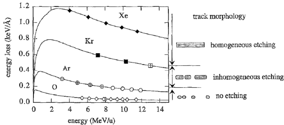
FIGURE 3.2: Calculated curves of the energy loss of Xe-, Kr-, Ar-, and O-ions in kapton as function of their specific energy. Full symbols (◆,■): etched tracks with small pore size distribution, crossed symbols (⊕,⊞): etched tracks with wide pore size distribution, open symbols (◇,○): no pores. [53]
