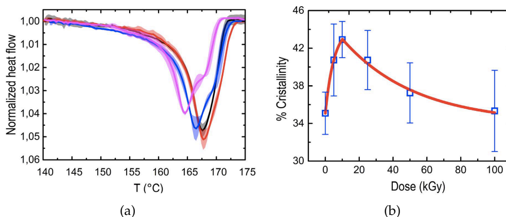
FIGURE 9.5: (a). Differential Scanning Calorimetry spectra registered at 20^{\circ}\text{C}\cdot\text{min}^{-1} - focus in the PVDF melting peaks region between 140^{\circ}\text{C} and 175^{\circ}\text{C} at e-beam irradiation doses of 0 (black line), 5 (red line), 10 (blue line) and 100 kGy (magenta line). Curve shadows represent error bar variations. (b). Degree of crystallinity versus irradiated doses.
