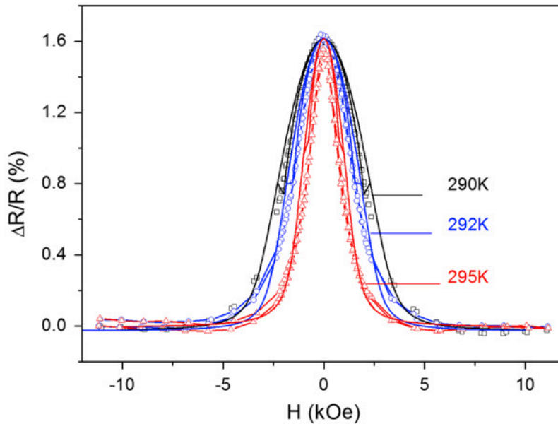
FIGURE 6.1: coercivity variation of the AMR signal in Ni NW embedded in PC matrix under thermo-elastic deformation
