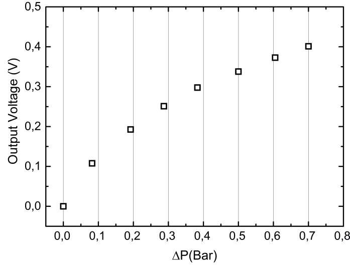
FIGURE 7.6: Output voltage vs applied \Delta P
