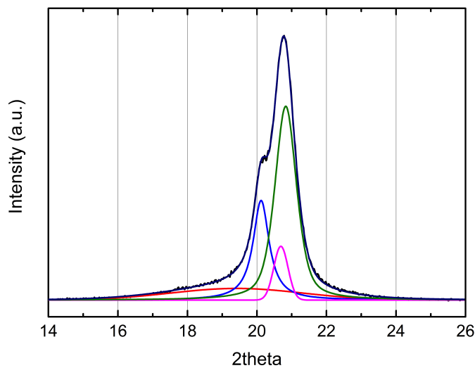
FIGURE 8.2: typical XRD spectrum for bi-oriented neat PVDF. Blue, magenta, green and red lines represent respectively: \alpha ( 2\theta=20.119 ), \beta ( 2\theta=20.688 ), \beta ( 2\theta=20.828 ) and the broad peak.
