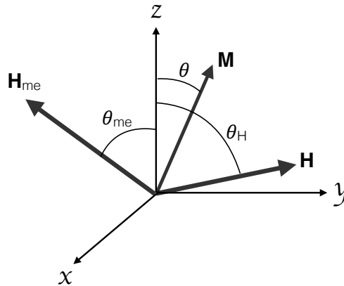
FIGURE 4.3: Orientation of the magnetization, magnetic and magnetoelastic field respect to NW-axis.
