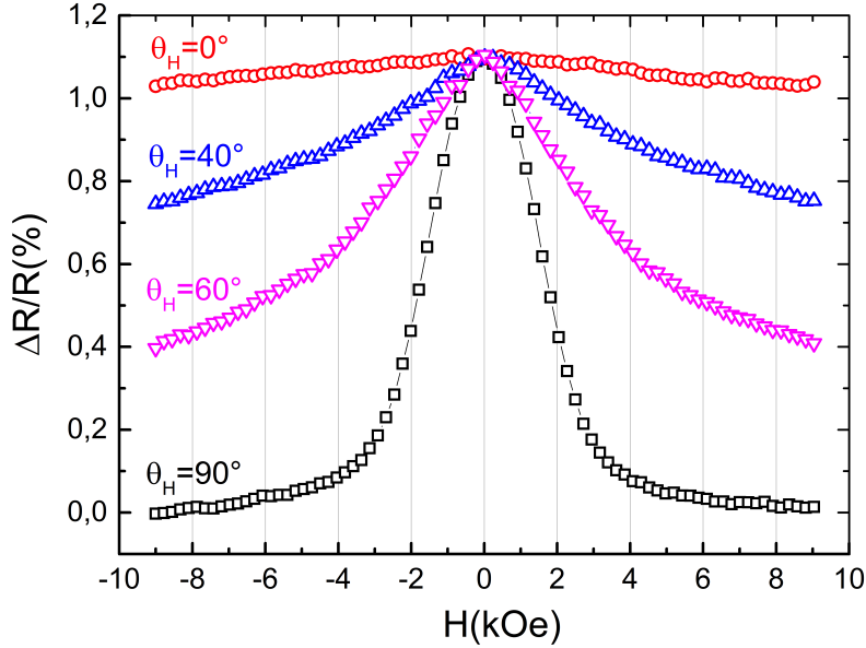
FIGURE 4.2: AMR at different \theta_H .
