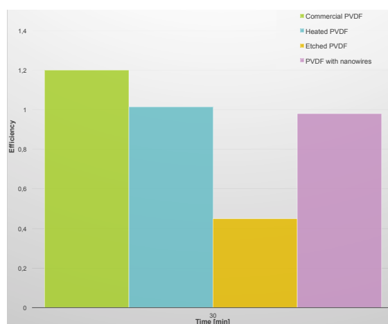
FIGURE 9.13: chemical etching impact on the electric efficiency. Etching time: 30 minutes. PVDF Reference (■), temperature (■), chemical etching (■) and Ni NWs (■) impact on the electrical efficiency.
