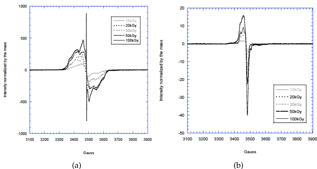
FIGURE 3.3: (a).Alkyl radicals in PVDF NPs irradiated under vacuum (2.5 MeV electron Van de Graaf accelerator); (b). Peroxy and alkyl radicals in PVDF NPs in presence of air.
