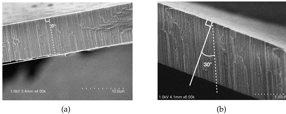
FIGURE 8.5: Cross section of track-etched PVDF. Nanopores perpendicular to the surface (a), and at 30^{\circ} respect to perpendicular axis at the surface (b).
