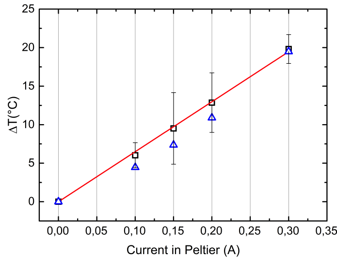
FIGURE 5.11: \Delta T vs injected current in the Peltier plate. Calculated data ( \square ); measured data ( \triangle )
