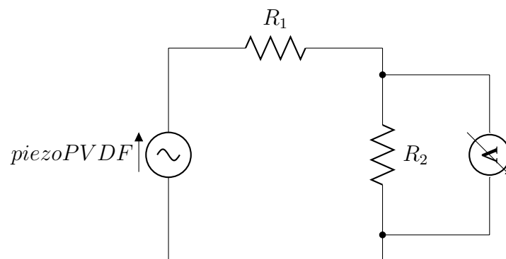
FIGURE 7.4: electric circuit used to measure the output voltage from the Piezo-PVDF film under bending stress condition
