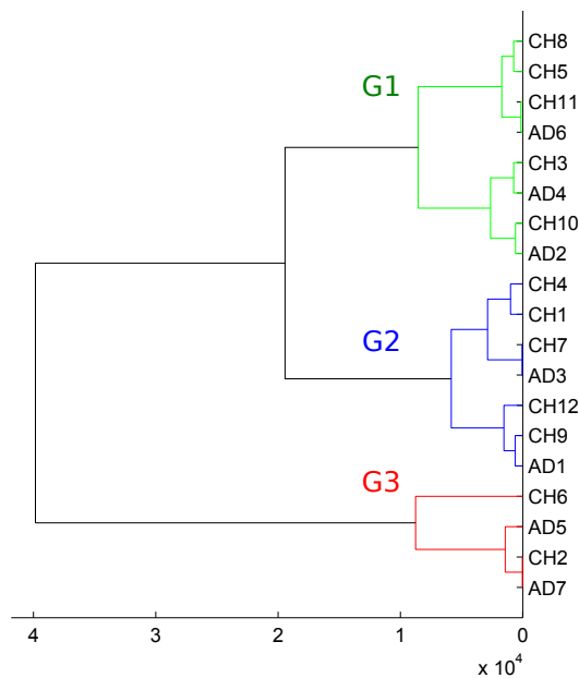
Figure 2.5: Dendrogram Analysis
