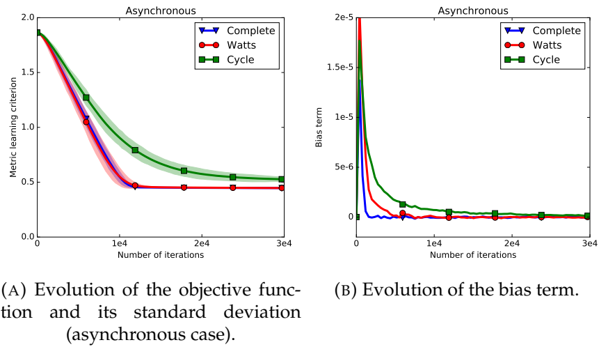
FIGURE 5.5: Metric learning experiments on a real dataset.
