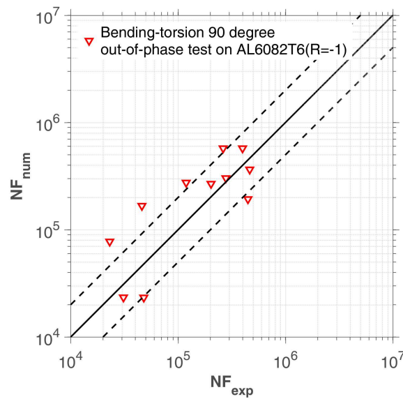
(c) Bending-torsion 90° out of phase tests on 6082 T6 aluminum(R=-1)
