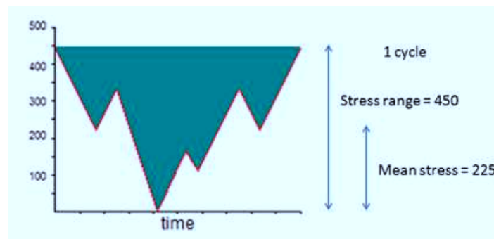
Figure 4.15 – Imagine Filling with Water and Extract Stress Range and Mean Stress (retrieved from “How to Calculate Fatigue Life When The Load History Is Complex”, February 13, 2015, author: Michael Bak, https://caei.com/blog/how-calculate-fatigue-life-when-load-history-complex )
