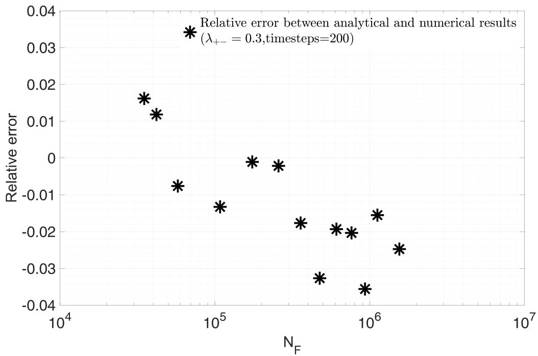
Figure 5.14 – Relative error \left(\frac{NF_{opt} - NF_{analytical}}{NF_{analytical}}\right) between analytical and numerical results with optimal time steps methods ( \beta = 1.1, a = 0.01, \Delta\alpha = 2 \times 10^{-5} in unit cycle)
