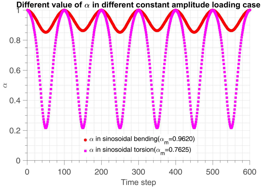
Figure 5.9 – The evolution of \alpha in bending and torsion with \Sigma_y = 1080 MPa, \Sigma_{bending} = \Sigma_{torsion} = 500 MPa, a = 0.3 and 200 time steps in one cycle
