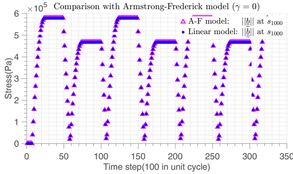
(a) Linear back stress evolution at sinusoidal cyclic load
