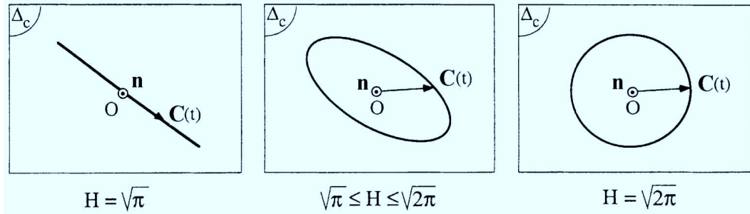
Figure 2.8 – Different paths of loading in the plane and corresponding values of the phase-difference coefficient H (Morel [2000]). For a proportional loading, H is equal to \sqrt{\pi} . In the case of a particular circular path, H reaches the maximum value \sqrt{2\pi} (Figure 2.8). The linear path and the circular one lead to two bounds of the coefficient H .
