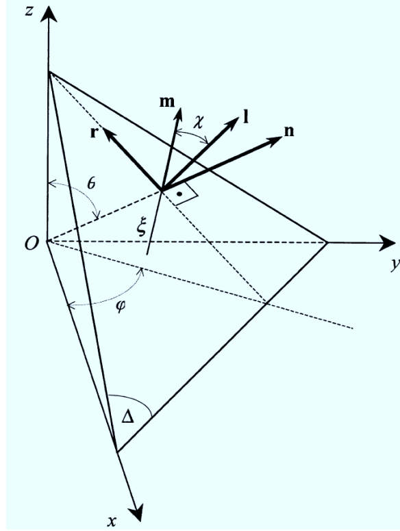
Figure 3.3 – Material plane \Delta passing through point O of a body and its associated (n, l, r) frame.
