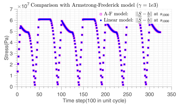
(b) \|\underline{S} - \underline{b}\| evolution at sinusoidal cyclic load
