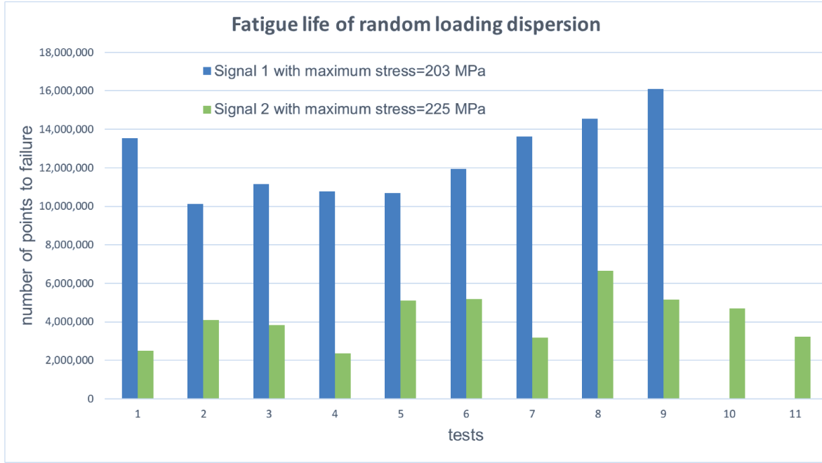
Figure 5.31 – Fatigue life of random loading dispersion on AW-6106 T6 aluminum, test data provided by CETIM
