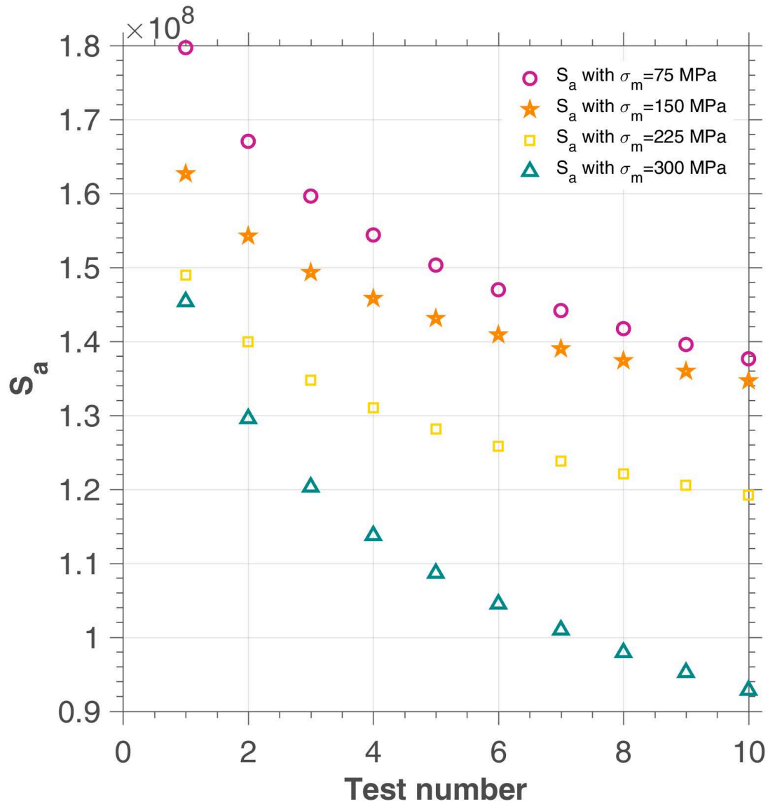
Figure 6.18 – S_a of bending tests with mean stress on 10HNAP
