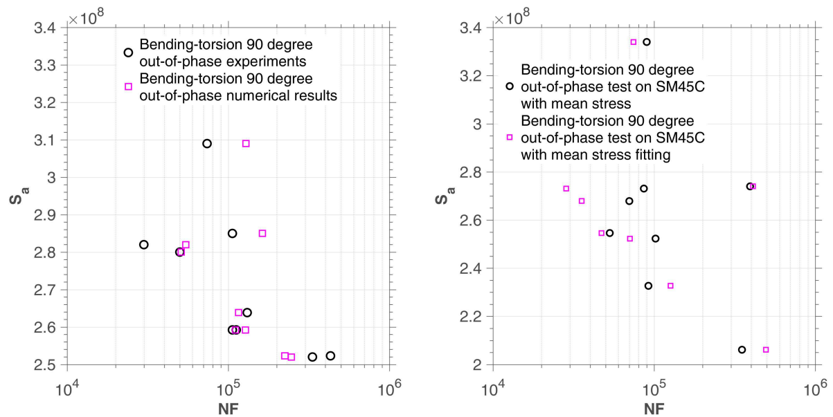
(c) Bending-torsion 90 degree out-of-phase tests on SM45C steel
