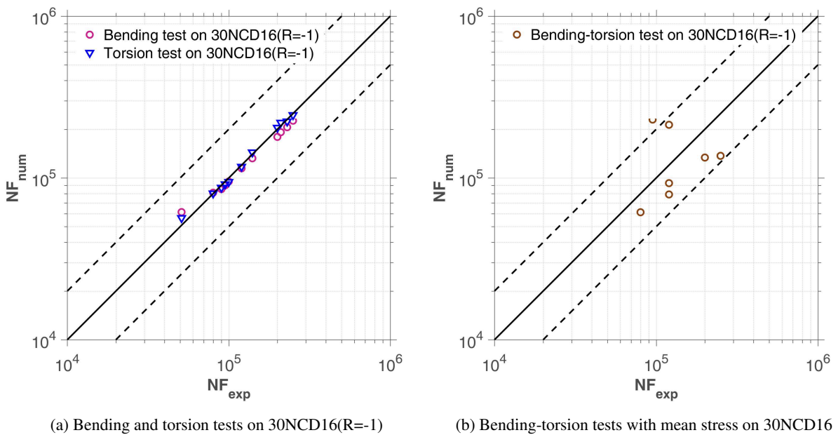
Figure 6.11 – Calibration on 30NCD16 (Dubar [1992]). In figure (c) test 29 (same N_F with test 30 but with smaller \sigma_{x,m} ) and test 32 (2-D with large mean stress) from Tab.6.15 are more dispersed. The numerical tests are carried out using the coefficients of Tab.6.16
