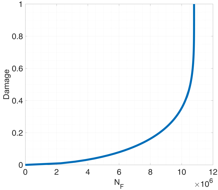
Figure 4.4 – Damage accumulation in terms of N in constant loading condition, with D and N are related by the evolution equation (4.1.12)
