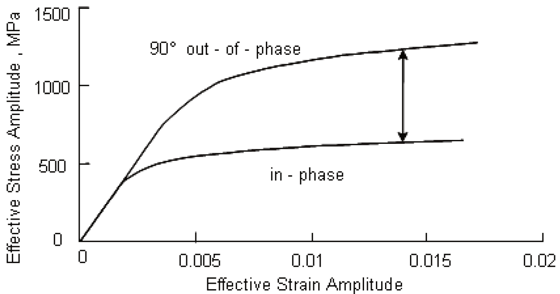
Figure 6.8 – The 90° out-of-phase loading path has been found to produce the largest degree of non-proportional hardening (EFA).
