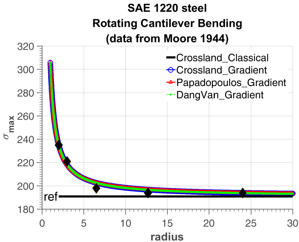
Figure 3.7 – Fatigue limits with gradient effect for different radii (Moore and Morkovin [1944]).
