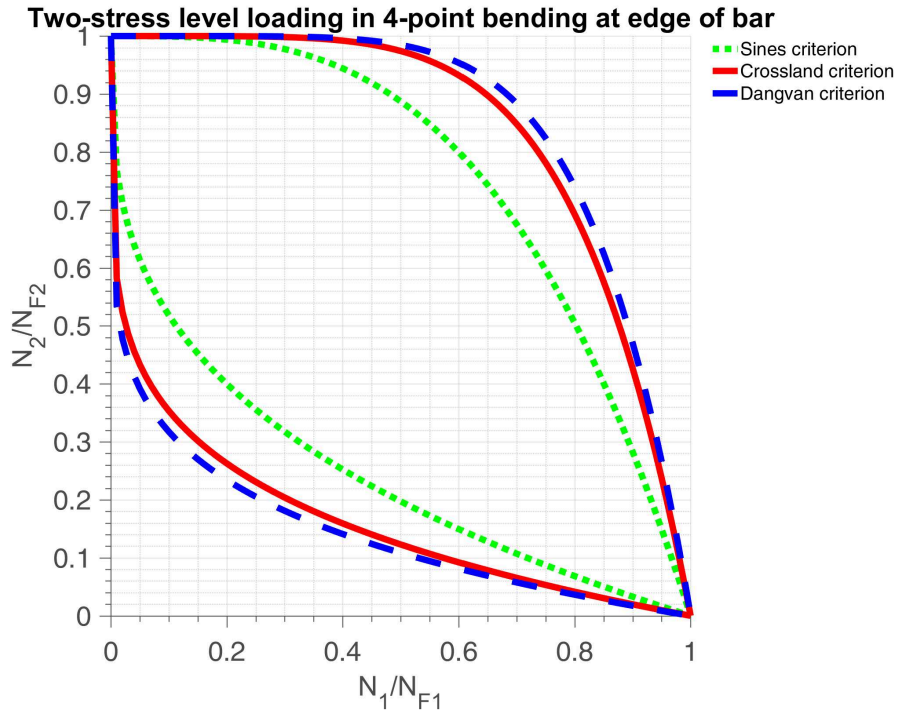
Figure 4.10 – Two-stress level loading in 4-point bending at y=3 . The lower curve displays the relative proportion of cycles in high-low sequence, the upper curve displays the same information in a low-high sequence
