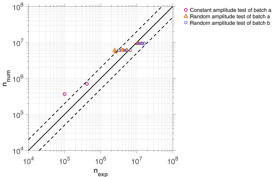
Figure 6.4 – Comparison between experimental and numerical results of 1D cyclic and random loading on aluminum fatigue tests by CETIM with constant \alpha from the first row of Tab.6.7
