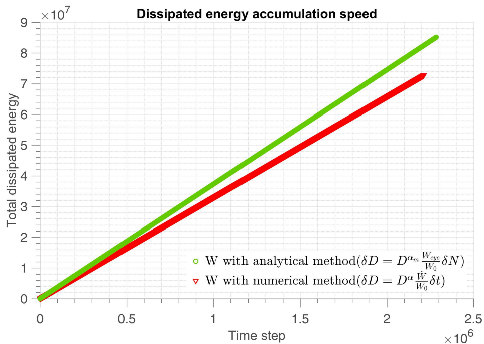
Figure 5.26 – Validation of dissipated energy in all scales with analytical and numerical method with \beta = 5, \Sigma = 0.4\sigma_y
