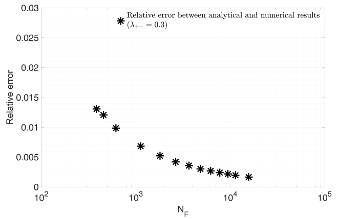
(d) Relative error \left( \frac{NF_{num} - NF_{analytical}}{NF_{analytical}} \right) with 100 time steps in unit cycle ( \beta = 1.1, a = 0.001 )
