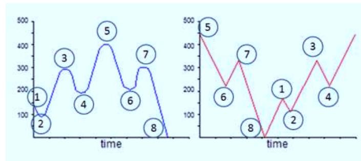
Figure 4.14 – Reorder to Start from Absolute Maximum (retrieved from “How to Calculate Fatigue Life When The Load History Is Complex”, February 13, 2015, author: Michael Bak, https://caesai.com/blog/how-calculate-fatigue-life-when-load-history-complex )
