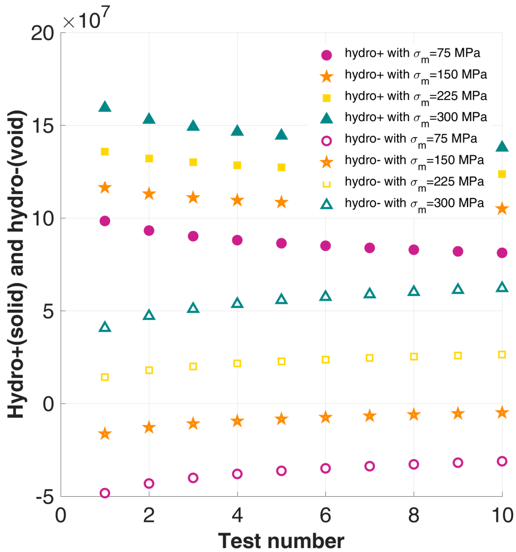
Figure 6.19 – \text{Hydro}_{+-} of bending tests with mean stress on 10HNAP
