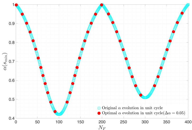
Figure 5.10 – Comparing numerical strategy with optimal time steps in one cycle with the old one, in this way the number of steps in unit cycle is reduced from 400 to 35, meaning a cost reduction factor of 0.0875 (with \Delta\alpha = 0.05 , a = 0.4 , \lambda = 0.1 , \Sigma_y = 230 MPa, \Sigma_{bending} = 225 MPa)
