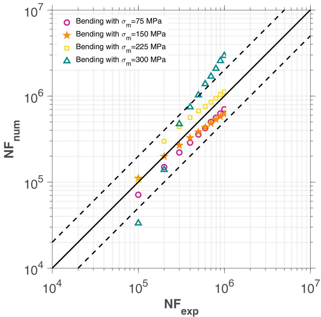
Figure 6.23 – Calibration on 10HNAP steel, bending tests with various mean stress on 10HNAP, data from Tab.6.25 and results obtained with the coefficients of Tab.6.28. For the case of \sigma_m = 300 MPa, the macroscopic maximum stress is greater than yield limit, which does not match our assumption that the material stays in elastic regime macroscopically (section 5.4.1).
