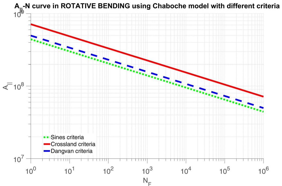
Figure 4.11 – A_{II} - N_F curve in rotative bending at r=3
