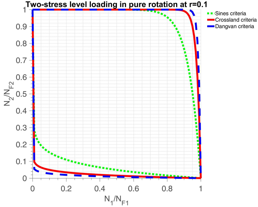
Figure 4.8 – Two-stress level loading in pure rotation at r=0.1 . The lower curve displays the relative proportion of cycles in high-low sequence, the upper curve displays the same information in a low-high sequence
