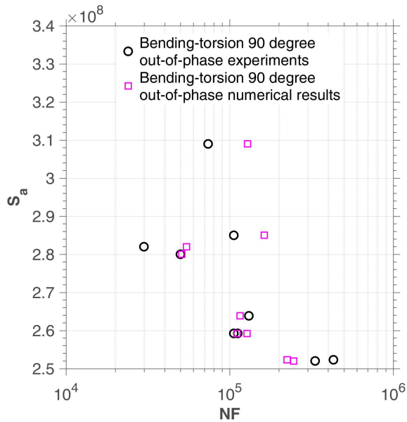
(c) Bending-torsion 90 degree out-of-phase tests on SM45C steel
