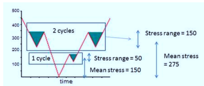
Figure 4.16 – Drain Water Starting at Lowest Valley and Repeat Cycle Extraction (retrieved from “How to Calculate Fatigue Life When The Load History Is Complex”, February 13, 2015, author: Michael Bak, https://caesai.com/blog/how-calculate-fatigue-life-when-load-history-complex )
