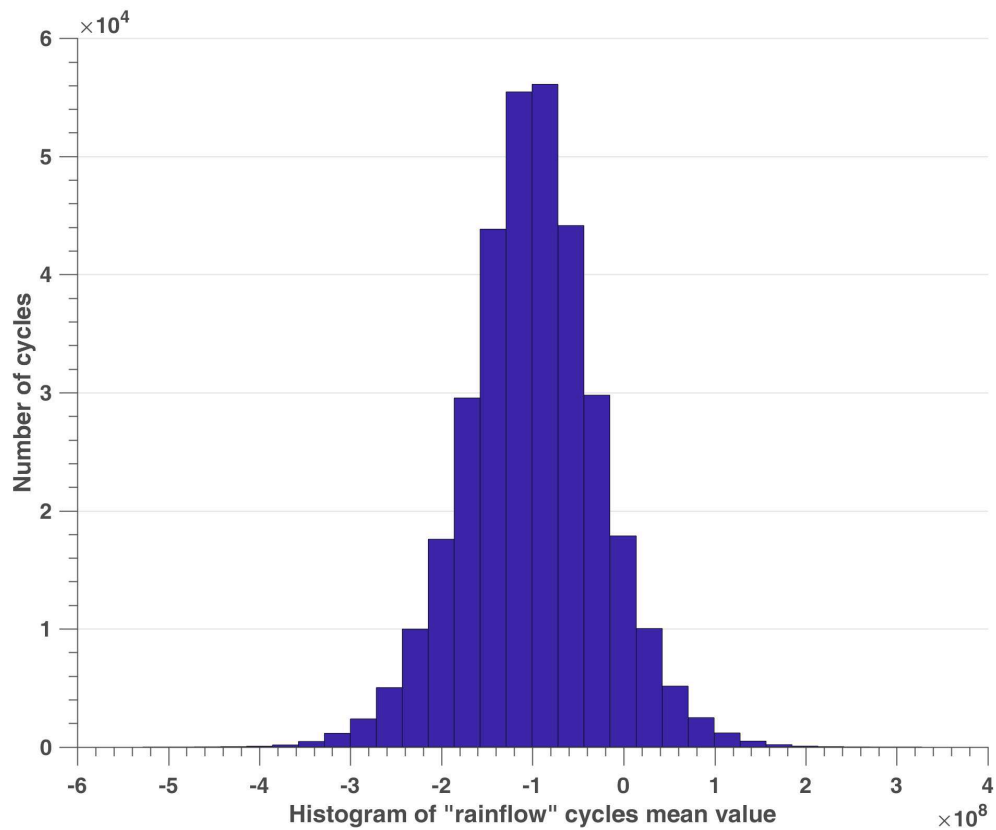
Figure 4.20 – Mean stresses distribution extracted from Figure 4.18
