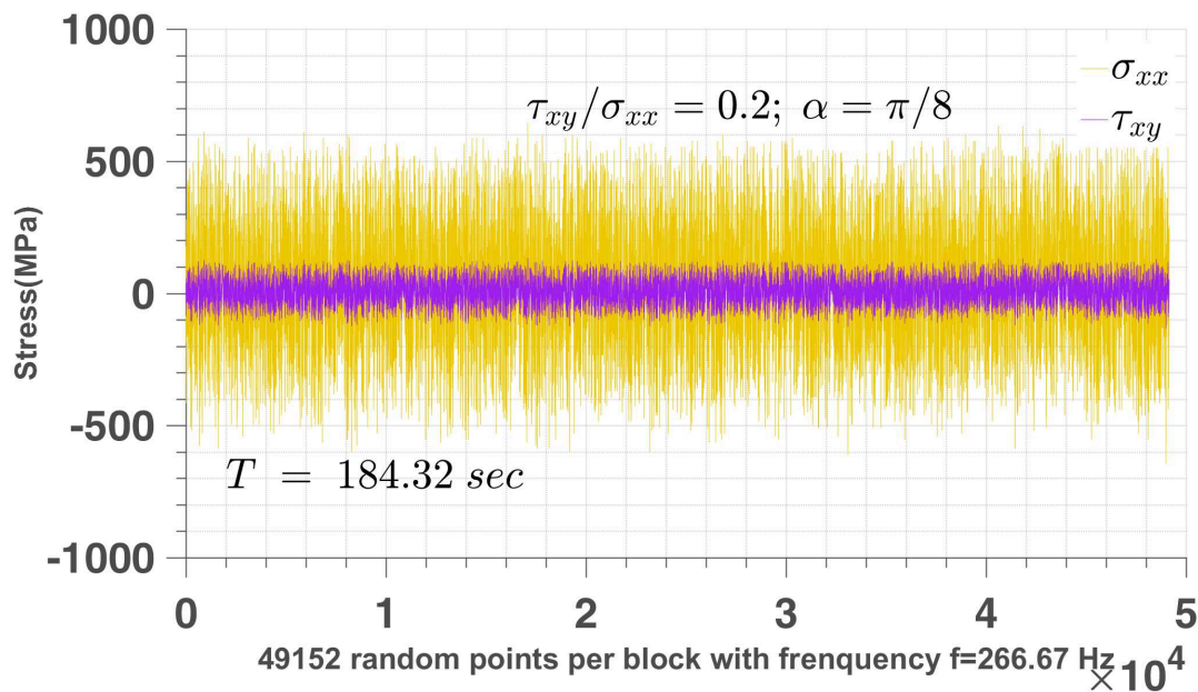
Figure 6.17 – Multiaxial random loading sequence
