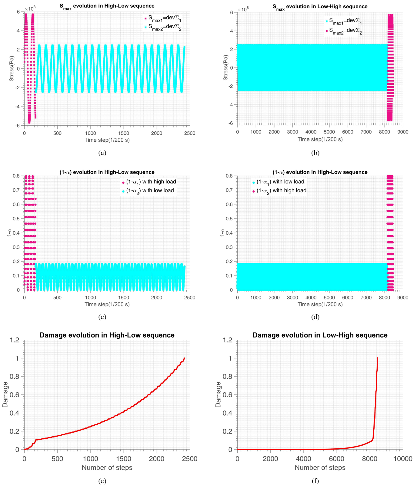
Figure 5.30 – Two level sequence effect. By comparing the vertical figures we can see high stress gives high (1 - \alpha) value which causes fast damage accumulation speed. The evolution of (1 - \alpha) is highly nonlinear and follows the value of stress at each time step.
