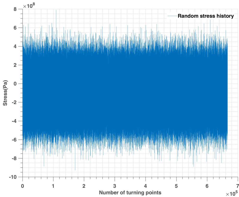
Figure 4.18 – One million normally distributed random stresses around -100MPa
