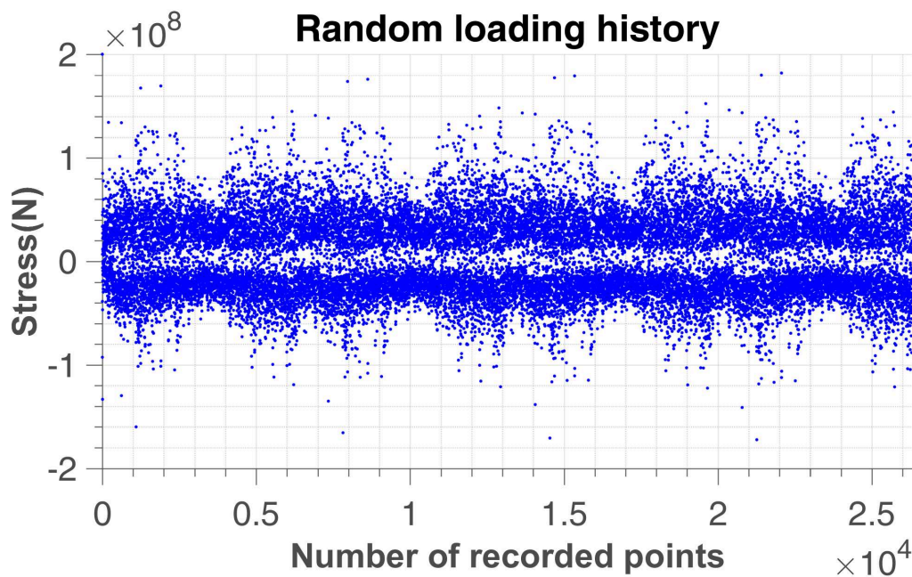
Figure 6.3 – Random loading history on BATCH_A_06 of AW-6106 T6 aluminum (see Tab.6.2)
