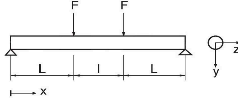
Figure 3.4 – 4-point bending test (Papadopoulos and Panoskaltsis [1996])
