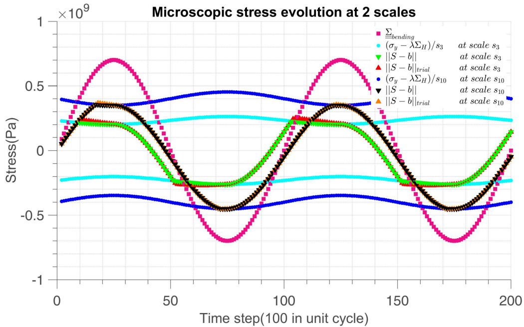
Figure 5.16 – Microscopic \left( \underline{S} - \underline{b} \right)_{trial} and \left( \underline{S} - \underline{b} \right) evolution with time under different weakening scales ( s_3 = 1.21 and s_{10} = 1.13 ) in sinusoidal load with zero mean stress
