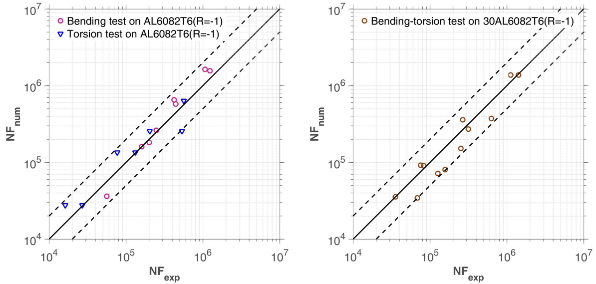
(a) Bending and torsion tests on 6082 T6 aluminum(R=-1)
