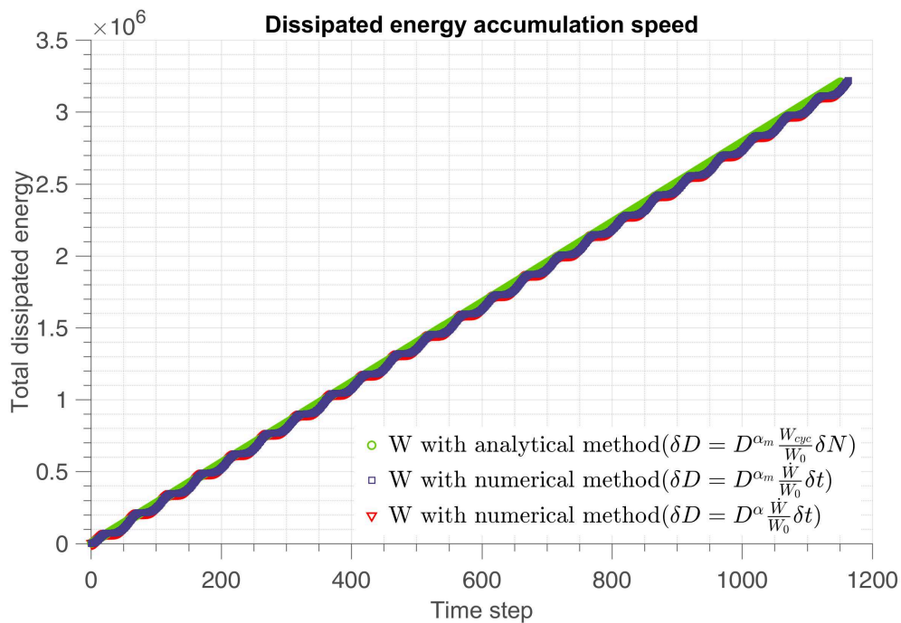
Figure 5.20 – Dissipated energy accumulation through time with different methods, there are 100 time steps in unit cycle
