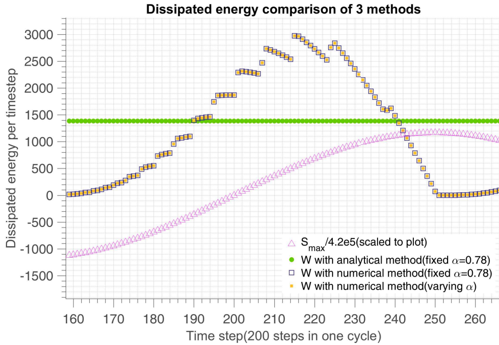
Figure 5.19 – Validation of dissipated energy in all scales with analytical and numerical method(enlargement of Figure 5.18)
