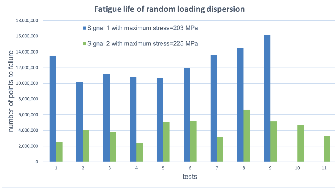
Figure 5.31 – Fatigue life of random loading dispersion on AW-6106 T6 aluminum, test data provided by CETIM
