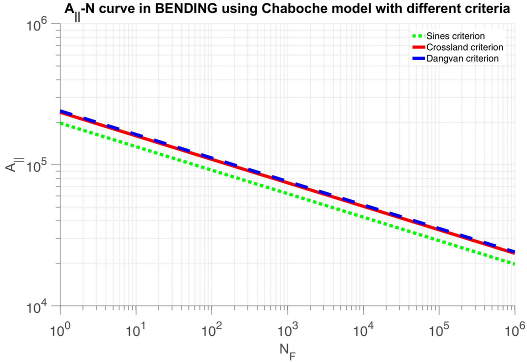
Figure 4.9 – A_{II} - N_F curve in 4-point bending at y=3
