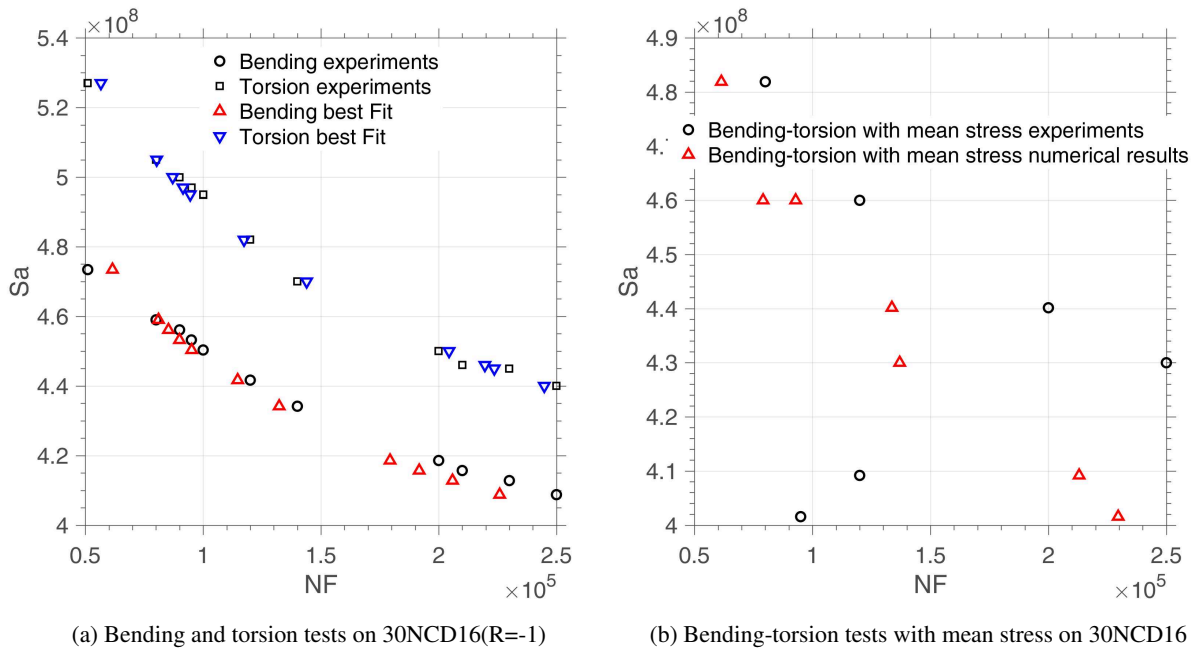
Figure 6.10 – Calibration on 30NCD16 (Dubar [1992]). We can observe that the bending-torsion experimental values are largely dispersed
