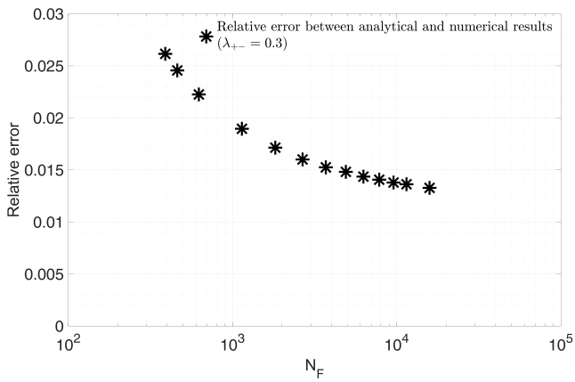
(c) Relative error \left( \frac{NF_{num} - NF_{analytical}}{NF_{analytical}} \right) with 30 time steps in unit cycle ( \beta = 1.1, a = 0.001 )
