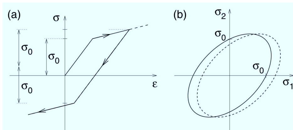
Figure 5.1 – Kinematic hardening: a) uniaxial stress-strain diagram, b) evolution of the yield surface in the biaxial stress plane
