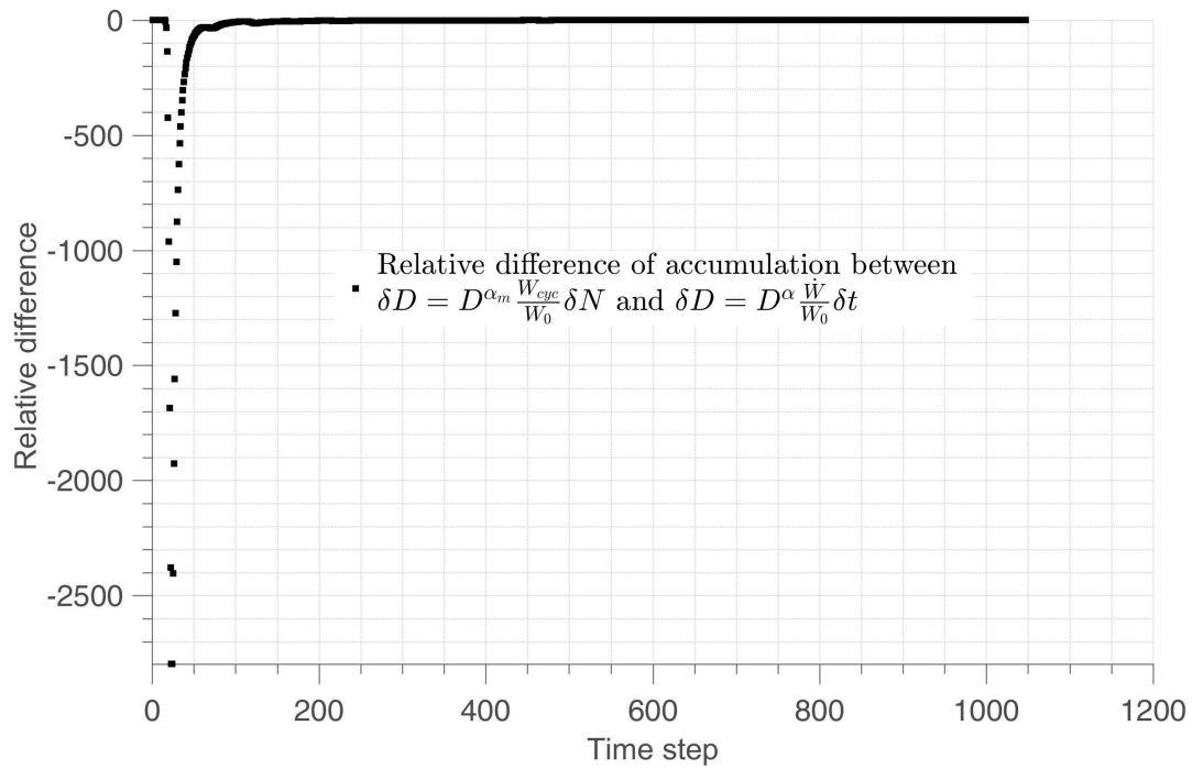
Figure 5.25 – Relative difference \frac{D_{analytical} - D_{numerical}}{D_{analytical}} evolution with time of Figure 5.23
