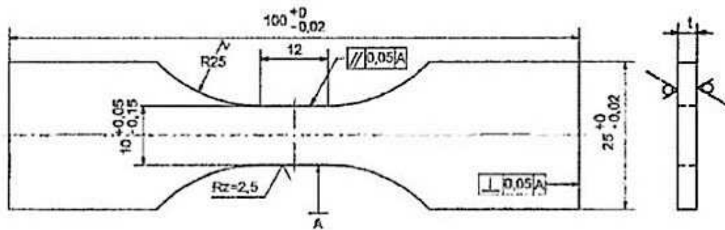
Figure 6.2 – Specimen geometry for fatigue tests of AW-6106 T6 aluminum (sample given by PSA)
