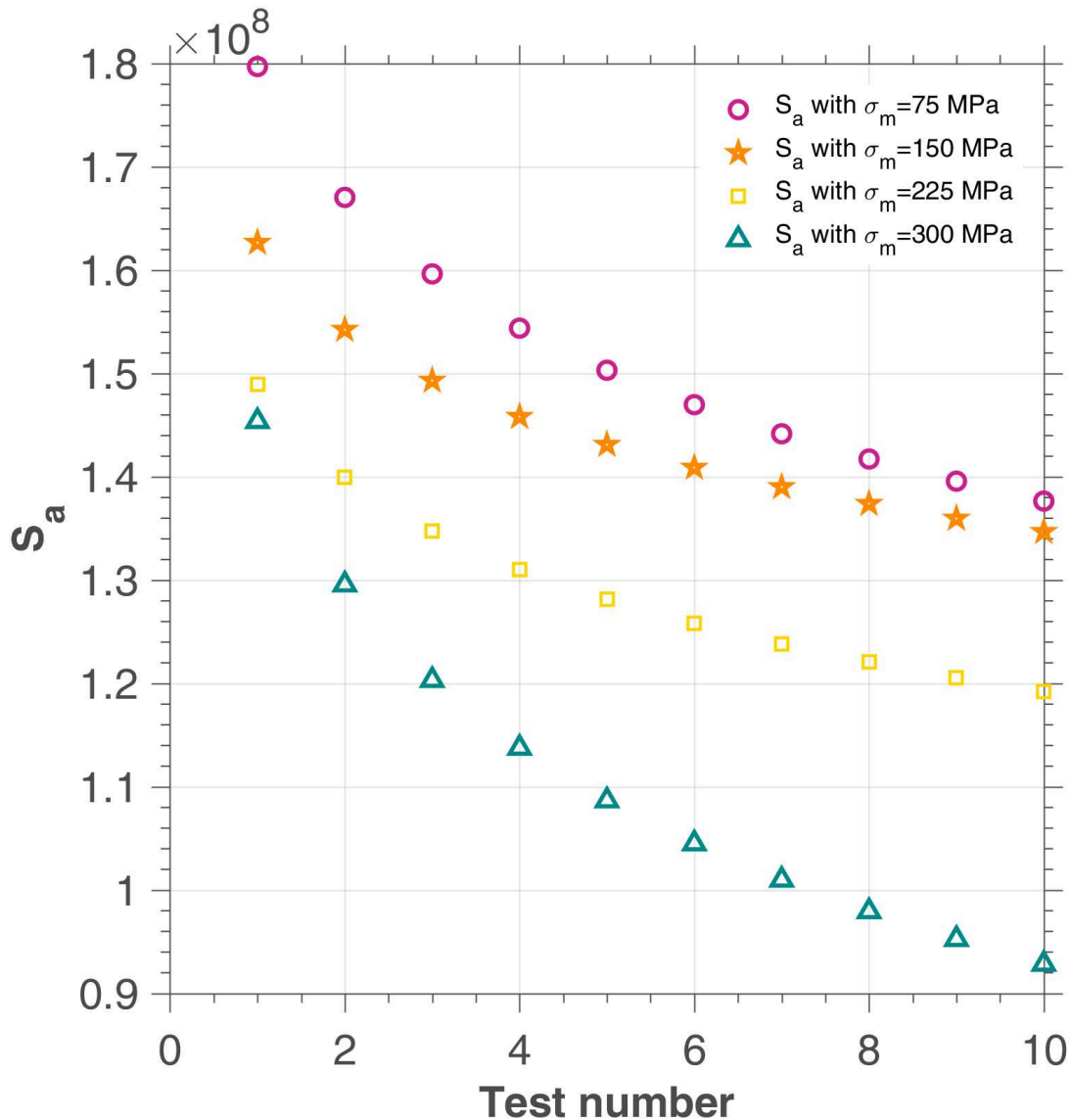
Figure 6.18 – S_a of bending tests with mean stress on 10HNP
