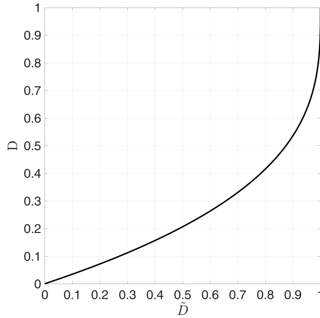
Figure 5.7 – The relation between \tilde{D} and D when \gamma = 2
