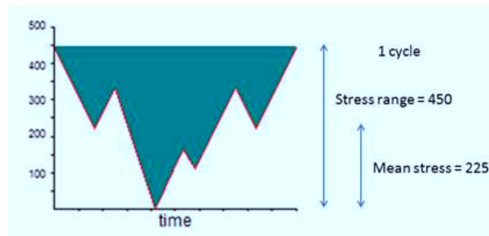
Figure 4.15 – Imagine Filling with Water and Extract Stress Range and Mean Stress (retrieved from “How to Calculate Fatigue Life When The Load History Is Complex”, February 13, 2015, author: Michael Bak, https://caesai.com/blog/how-calculate-fatigue-life-when-load-history-complex )
