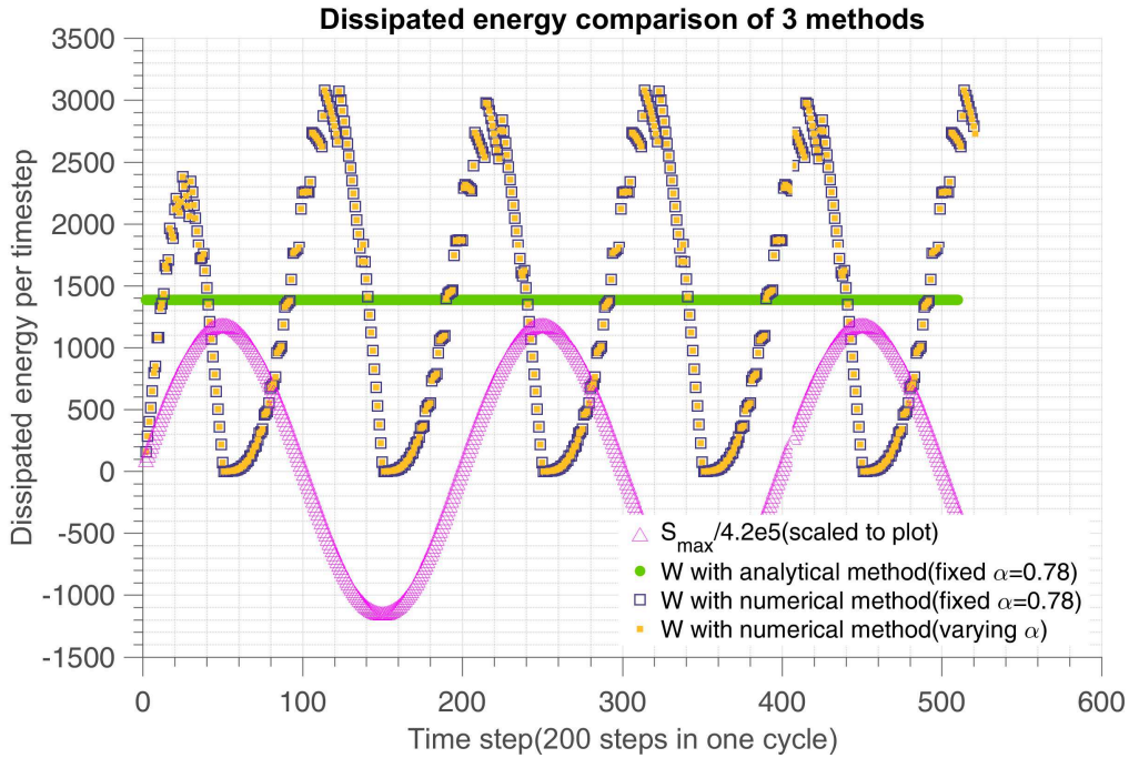
Figure 5.18 – Validation of dissipated energy in all scales with analytical (method 3) and numerical method (method 1) with \beta = 1.1, \Sigma = 0.85\sigma_y . The time evolution of \alpha does not play a role in the dissipation calculation which is normal since \alpha does not enter in the dissipation calculation
