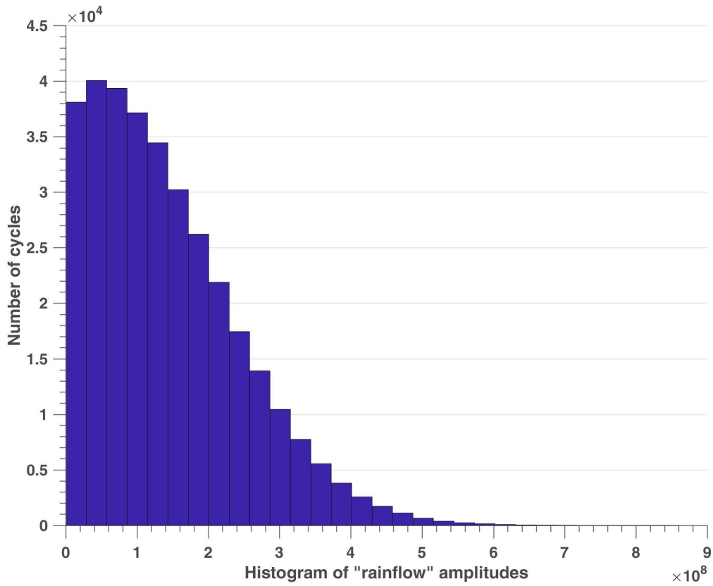
Figure 4.19 – Amplitudes distribution extracted from Figure 4.18
