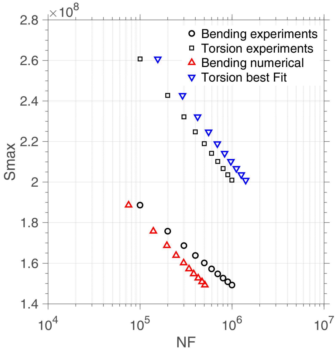
Figure 6.20 – Bending and torsion test on 10HNAP steel( R=-1 ). Data are presented in Tab.6.30 and 6.31. The torsion best fit and the bending numerical results(optimal time step of method 2 deduced in Chapter 5) are obtained with the coefficients of Tab.6.28
