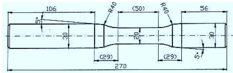
Figure 6.6 – Specimen geometry for fatigue tests of aluminum 6082 T6 (dimension in millimeters), from Susmel and Petrone [2003]
