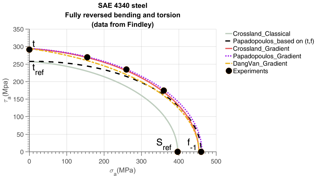
Figure 3.10 – Fully reversed combined bending-twisting fatigue limit data (Findley et al. [1956], Papadopoulos and Panoskaltis [1996]) compared with updated values computed with gradient effects using Eq.(3.6.34), Eq.(3.6.35), Eq.(3.6.36), Eq.(3.6.37) and Eq.(3.6.38) with l_g = 2.5 \text{ mm} . In absence of gradient effect, we would get the inner gray ellipse corresponding to classical Crossland criterion.
