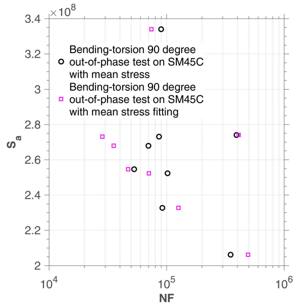
(d) Bending-torsion 90 degree out-of-phase tests with mean stress on SM45C steel
