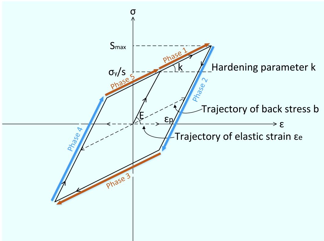
Figure 5.5 – Illustration of uniaxial cyclic load with microscopic plastic dissipation at scale s
