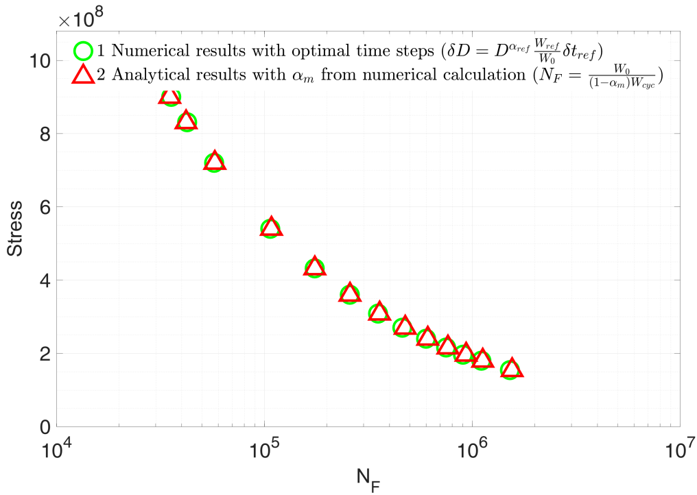
Figure 5.12 – S-N curve using analytical and numerical results with optimal time steps methods ( \beta = 1.1 , a = 0.01 , \Delta\alpha = 2E - 5 in unit cycle), yielding 200 full time steps reduced to 197 optimal time steps
