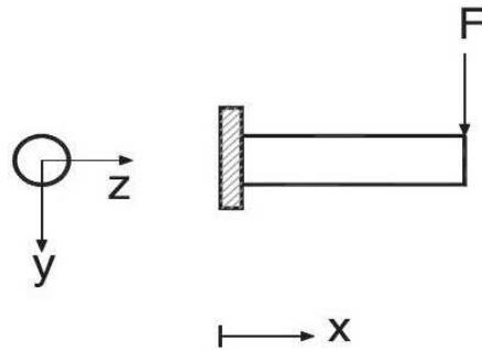
Figure 3.5 – Cantilever bending test (Papadopoulos and Panoskaltsis [1996])
