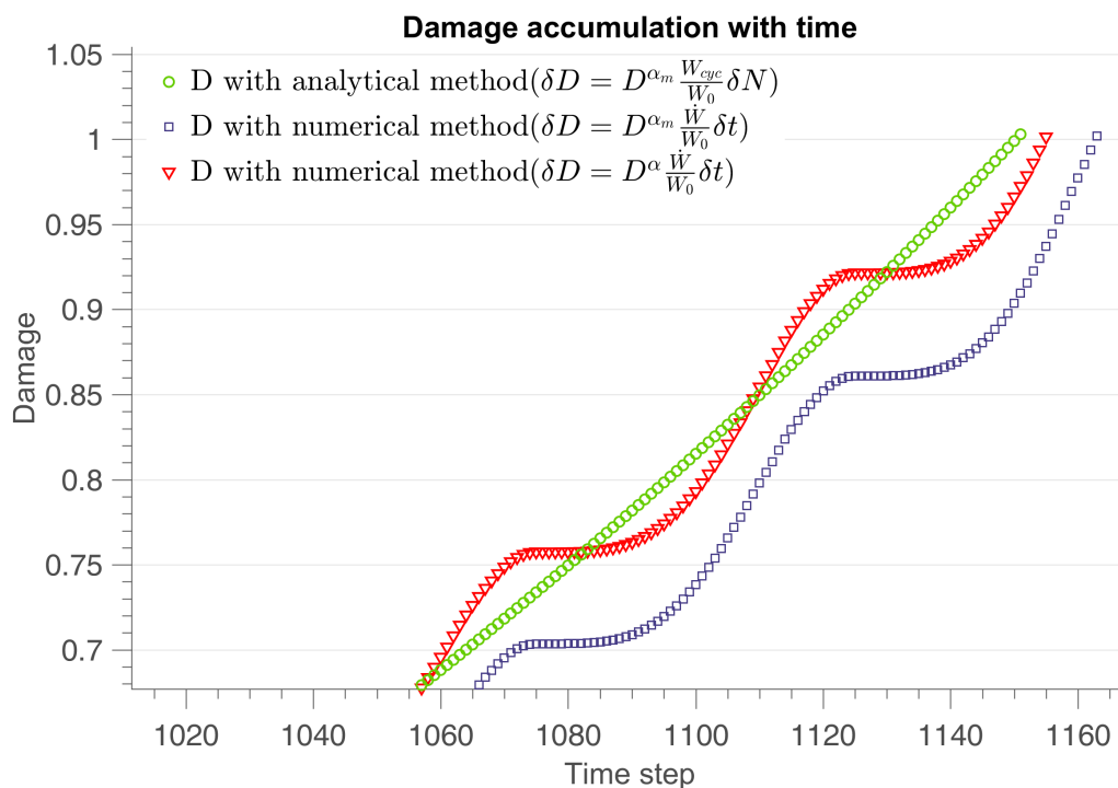
Figure 5.24 – Damage evolution with time under sinusoidal load with two different methods(enlargement of Figure 5.23)
