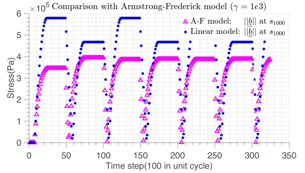
(b) Nonlinear back stress evolution at sinusoidal cyclic load
