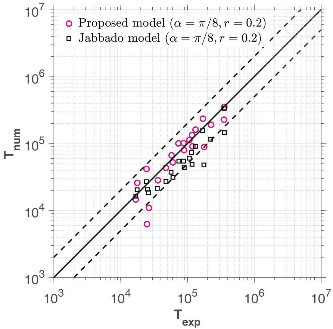
Figure 6.24 – Random bending-torsion 2D tests on 10HNAP, data from Tab.6.26 and Jabbado [2006]. Results are obtained with the coefficients of Tab.6.29 ( \alpha_M = \pi/8 and r = 0.2 )
