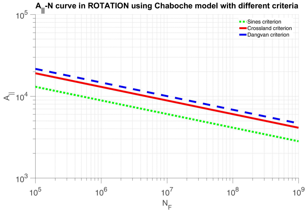
Figure 4.7 – A_{II} - N_F curve in rotation at r=0.1
