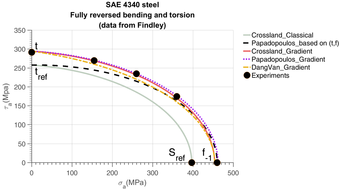
Figure 3.10 – Fully reversed combined bending-twisting fatigue limit data (Findley et al. [1956], Papadopoulos and Panoskaltsis [1996]) compared with updated values computed with gradient effects using Eq.(3.6.34), Eq.(3.6.35), Eq.(3.6.36), Eq.(3.6.37) and Eq.(3.6.38) with l_g = 2.5 \text{ mm} . In absence of gradient effect, we would get the inner gray ellipse corresponding to classical Crossland criterion.
