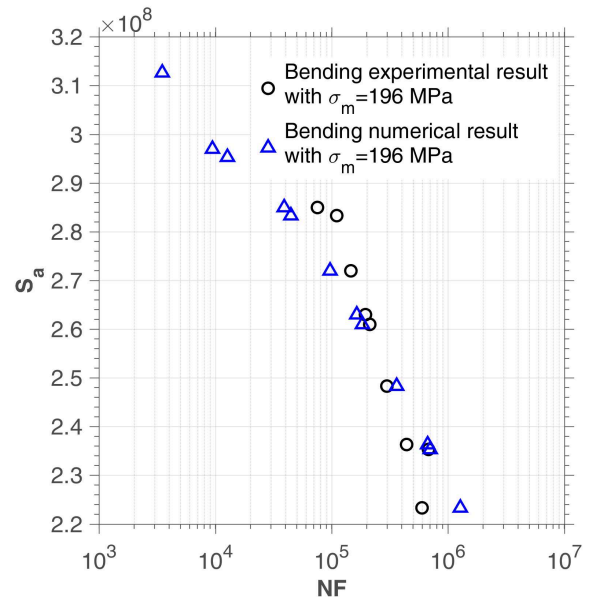
(b) Bending test with mean stress on SM45C steel ( \sigma_m = 196MPa )
