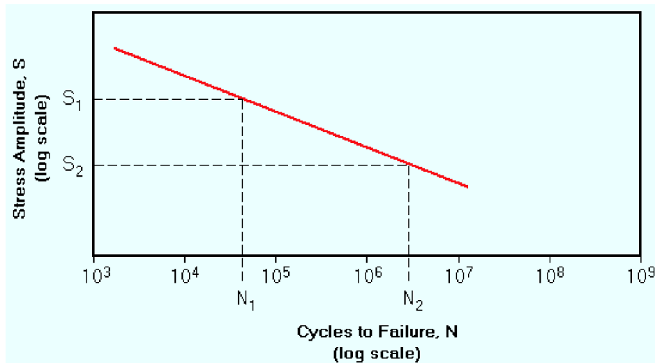
Figure 2.1 – Idealized S-N curve for high cycle fatigue.
