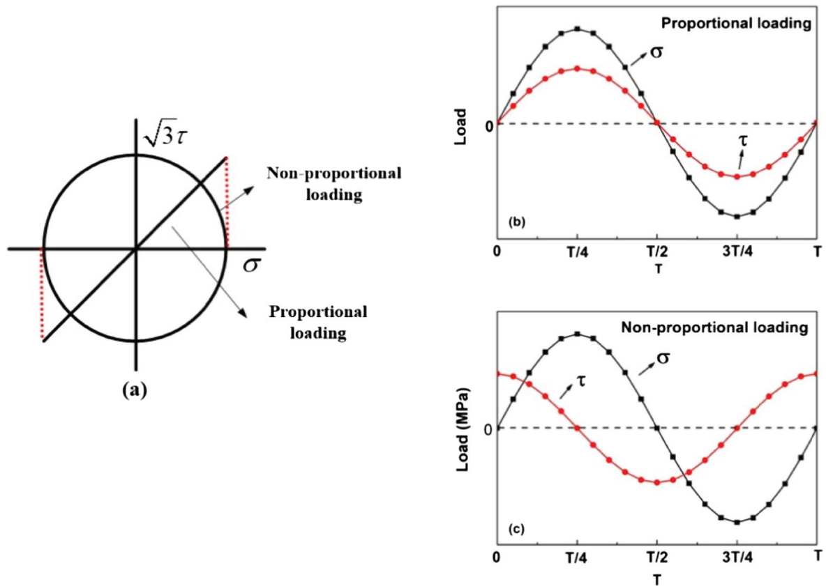
Figure 6.7 – The loading path and loading waveform of multiaxial corrosion fatigue (stress control) (a) loading path of proportional and non-proportional, (b) loading waveform of proportional loading, (c) loading waveform of non-proportion (Huang et al. [2017])
