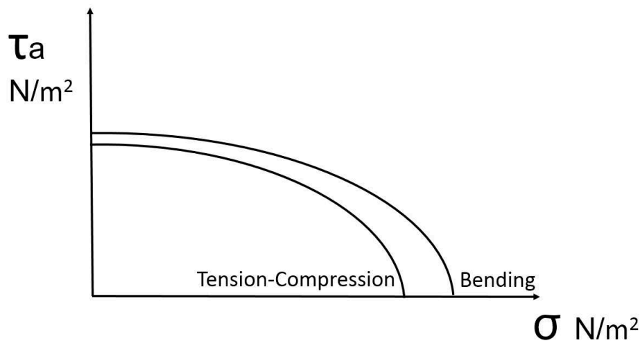
Figure 3.2 – Schematic representation of the nominal fatigue limit (ellipse arc) for two different tests: the arc is larger in the case of bending-torsion (presence of stress gradient) than in tension-compression.
