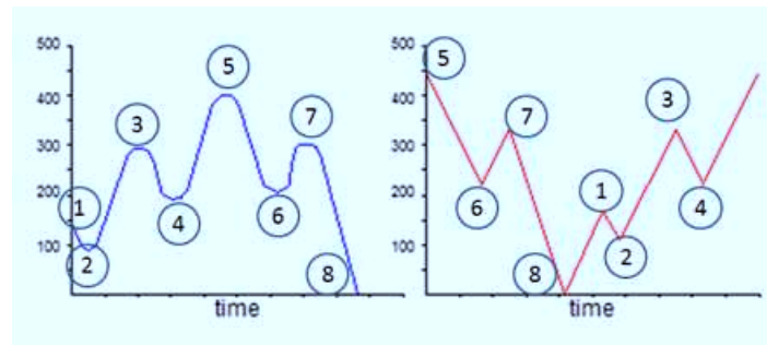
Figure 4.14 – Reorder to Start from Absolute Maximum (retrieved from “How to Calculate Fatigue Life When The Load History Is Complex”, February 13, 2015, author: Michael Bak, https://caei.com/blog/how-calculate-fatigue-life-when-load-history-complex )
