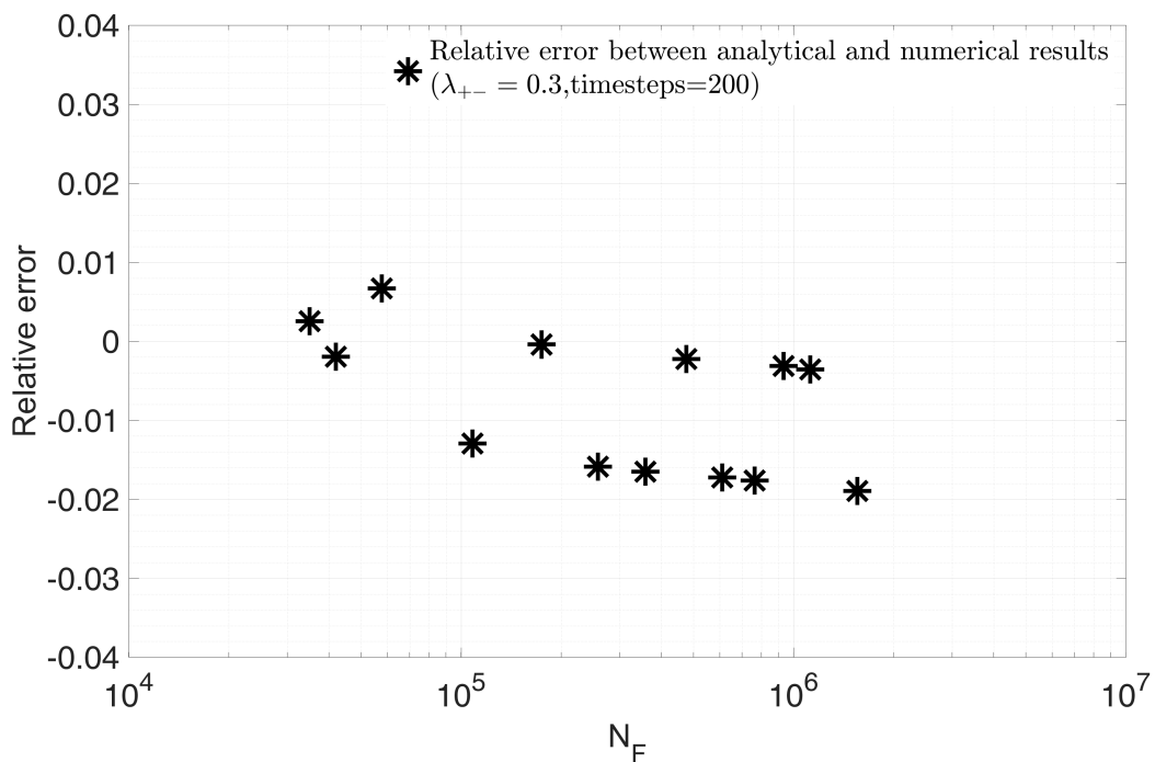
Figure 5.15 – Relative error \left(\frac{NF_{opt} - NF_{analytical}}{NF_{analytical}}\right) between analytical and numerical results with optimal time steps methods ( \beta = 1.1, a = 0.01, \Delta\alpha = 1 \times 10^{-5} in unit cycle)
