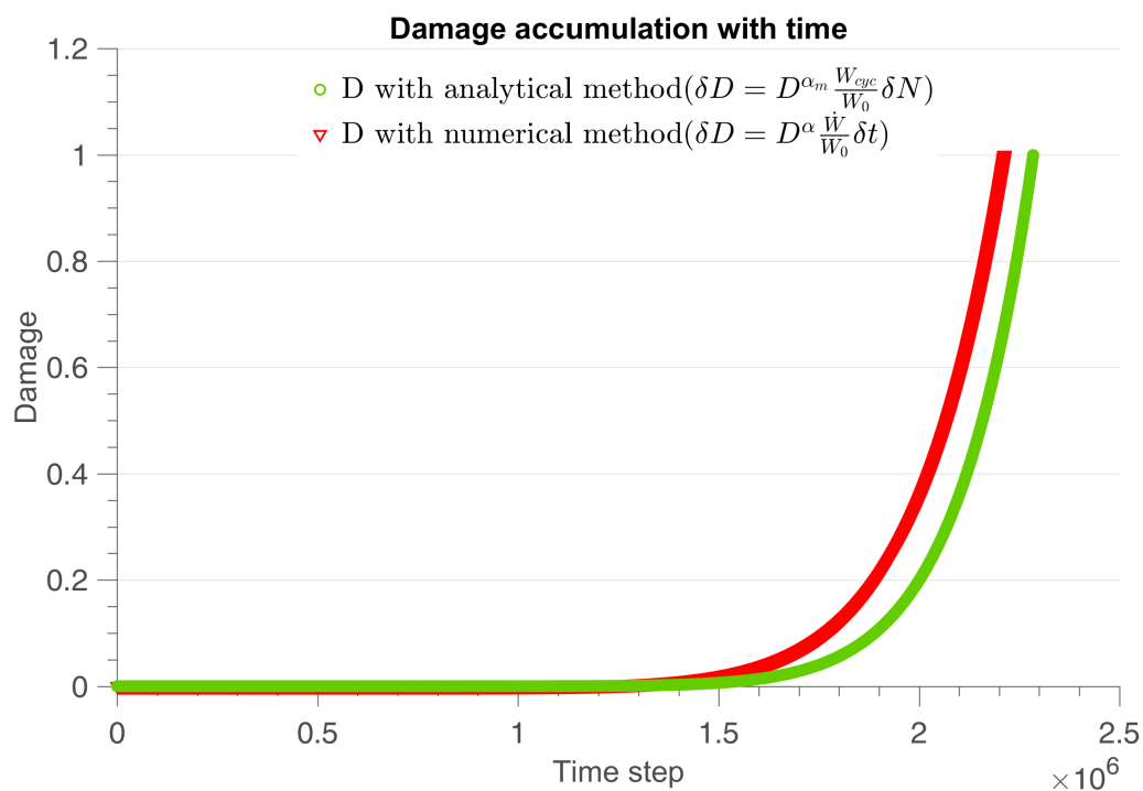
Figure 5.28 – Damage evolution with time under sinusoidal load with \beta = 5 , \Sigma = 0.4\sigma_y . In such a severe loading and with extreme non-linearity, the simple Chaboche like formula with frozen \alpha departs from the outcome of the full numerical model
