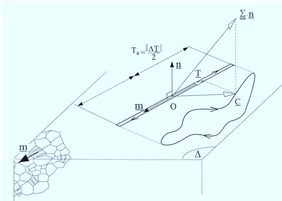
Figure 2.6 – Path of the macroscopic shear stress \underline{C} acting on a material plane \Delta and the corresponding path of the macroscopic resolved shear stress \underline{T} acting on an easy glide direction (Morel [2000]).
