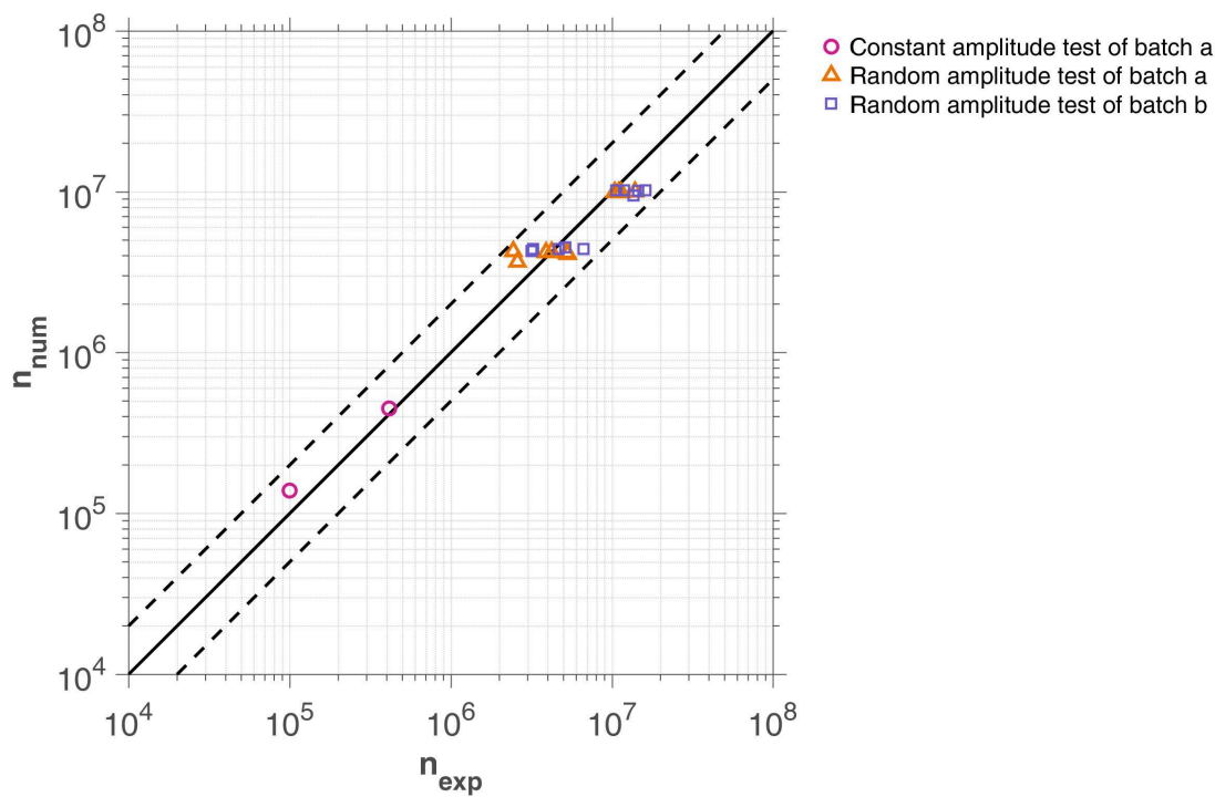
Figure 6.5 – Comparison between experimental and numerical results of 1D cyclic and random loading on aluminum fatigue tests by Cetim with load dependent \alpha . Coefficients data are given in the second row of Tab.6.7
