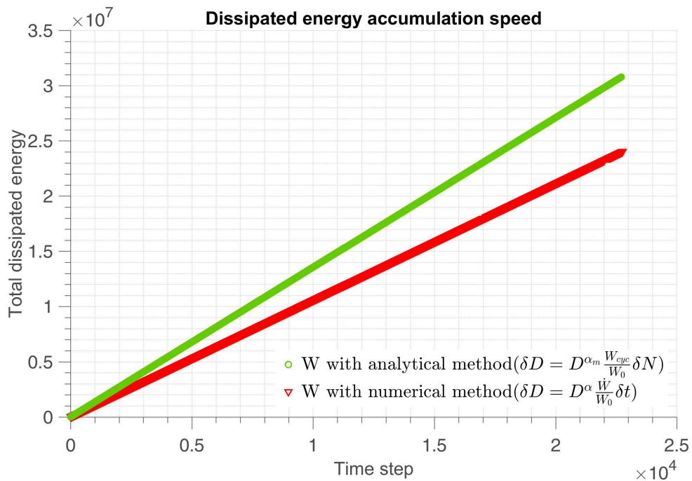
Figure 5.27 – Validation of dissipated energy in all scales with analytical and numerical method with \beta = 5 , \Sigma = 0.8\sigma_y
