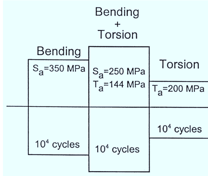
Figure 2.9 – block sequence tests (bending/bending+torsion/torsion) performed on a mild steel XC18.
