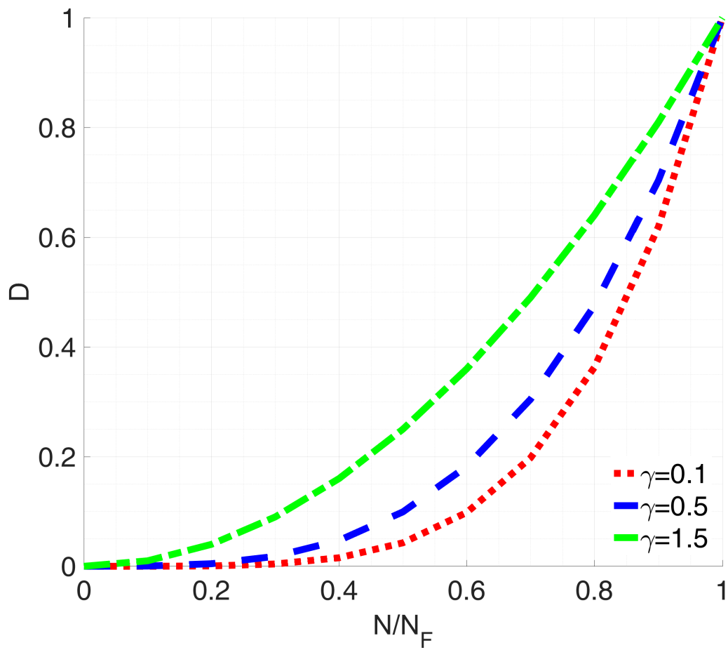
Figure 4.6 – Influence of function \hat{\gamma} in a plot of damage versus fatigue life ratio with \alpha = 0.8
