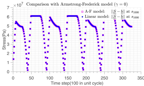
(a) \|\underline{S} - \underline{b}\| evolution at sinusoidal cyclic load
