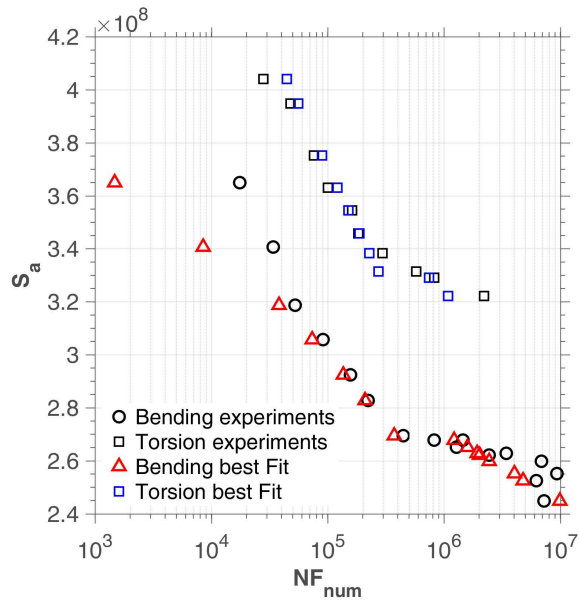
(a) Bending and torsion test on SM45C steel(R=-1)
