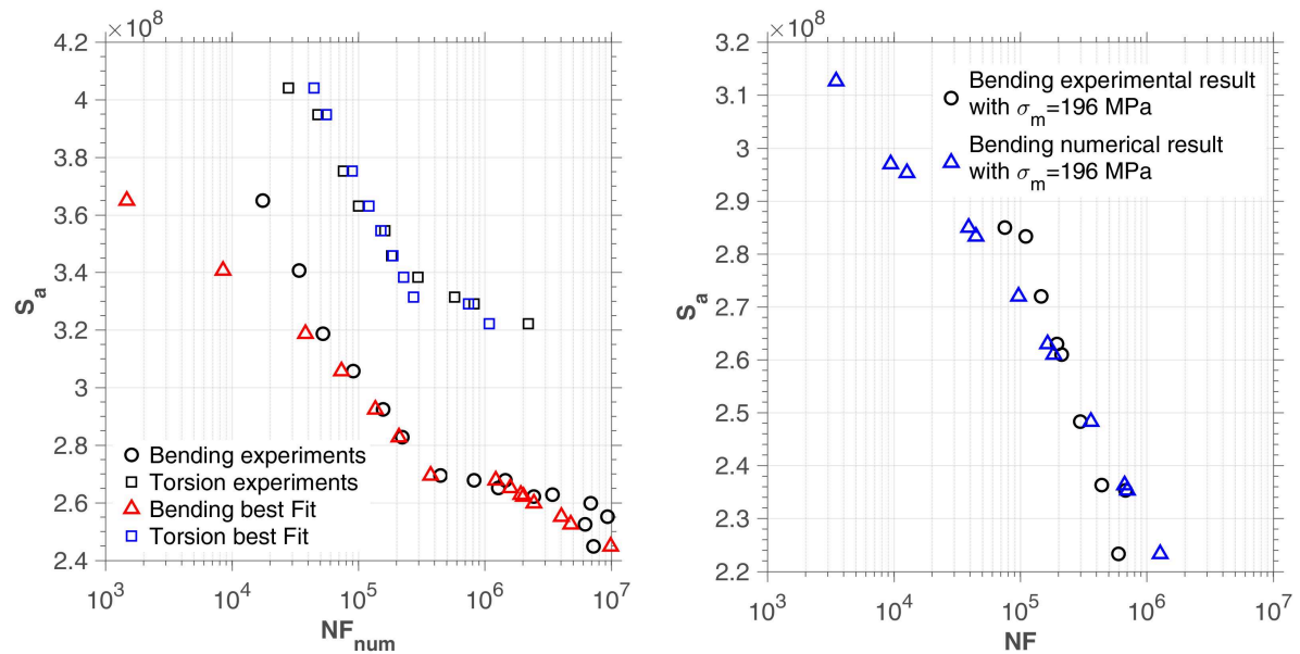
(a) Bending and torsion test on SM45C steel( R=-1 )
