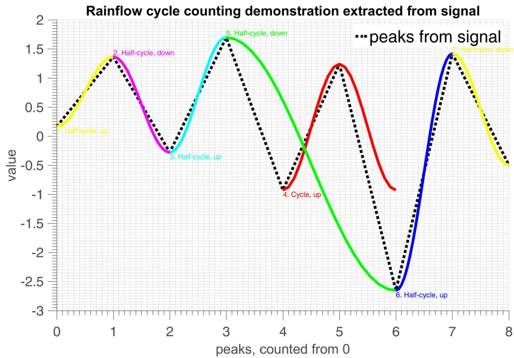
Figure 4.17 – Rainflow counting method demonstration
