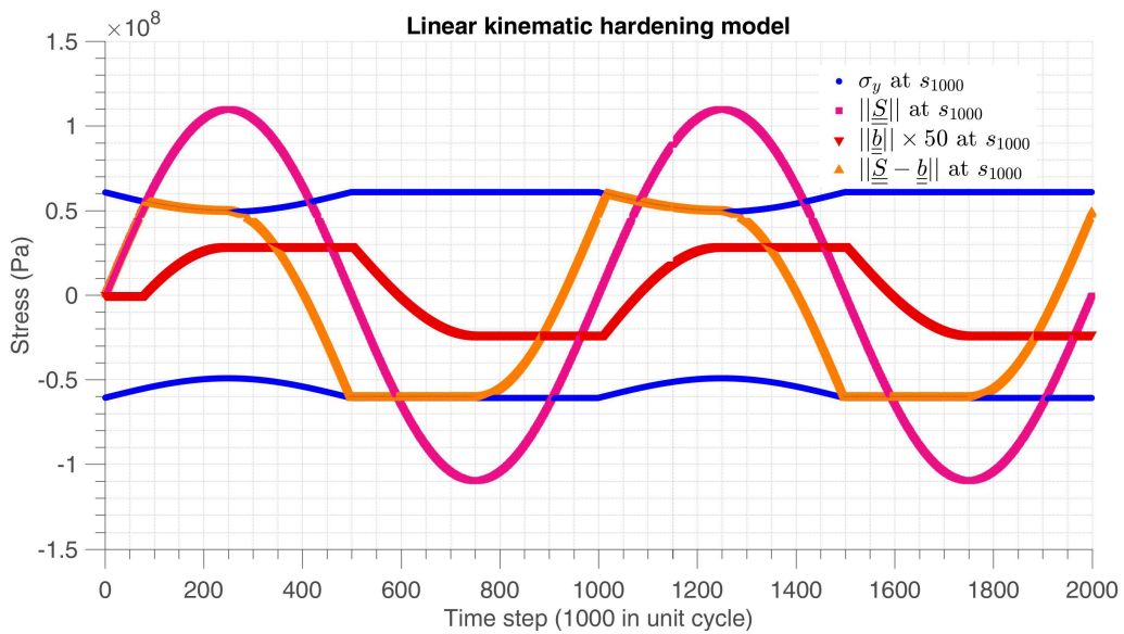
Figure 5.6 – Illustration of uniaxial cyclic load with microscopic plastic dissipation at scale s . With \Sigma_y = 298\text{MPa} , \Sigma_a = 190\text{MPa} , \lambda_+ = 0.9 , \lambda_- = 0 . There is energy dissipation when \|\underline{\Sigma} - \underline{b}\|(t) projects on the local yield limit (\sigma_y - \lambda \Sigma_H) / s(t) .
