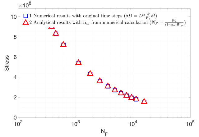
(b) 100 time steps in unit cycle ( \beta = 1.1, a = 0.001 ).
