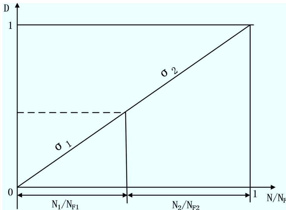
Figure 4.1 – Linear accumulation of damage with linear evolution
