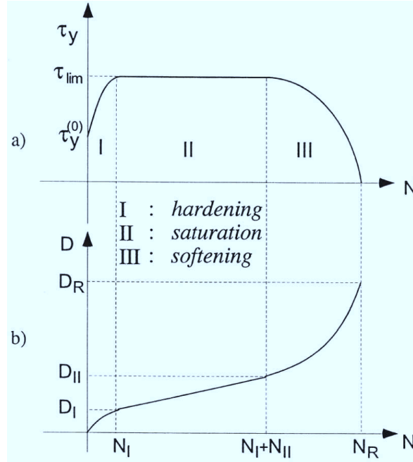
Figure 2.7 – (a) Yield limit evolutions and (b) damage evolution in the three behavior phases (hardening, saturation and softening) when a cyclic loading is applied (Morel [2000]).
