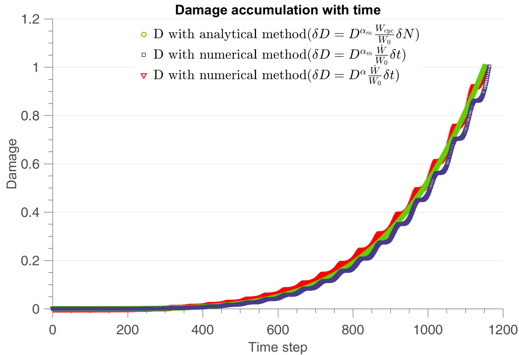
Figure 5.23 – Damage evolution with time under sinusoidal load with different methods, there are 100 time steps in unit cycle( \beta = 1.1, \Sigma = 0.85\sigma_y )
