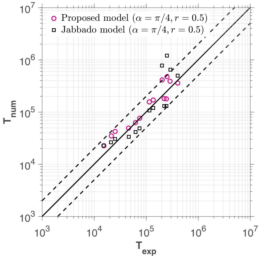
Figure 6.25 – Random bending-torsion 2D tests on 10HNAP, data from Tab.6.27 and Jabbado [2006]. Results are obtained with the coefficients of Tab.6.29 ( \alpha_M = \pi/4 and r = 0.5 )
