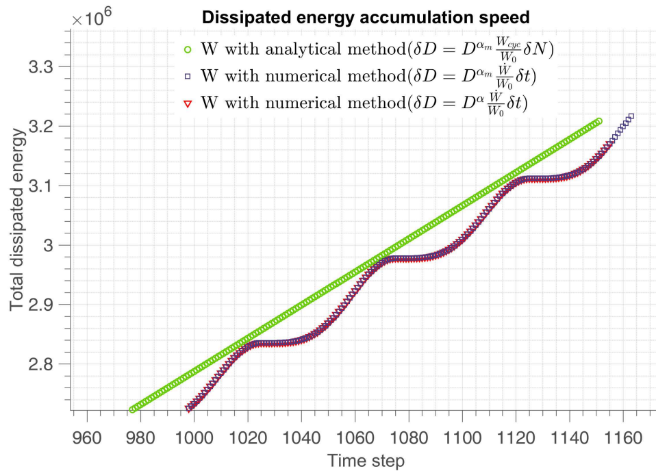
Figure 5.21 – Dissipated energy accumulation through time with of 3 methods(enlargement of Figure 5.20)
