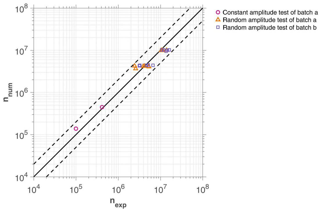
Figure 6.5 – Comparison between experimental and numerical results of 1D cyclic and random loading on aluminum fatigue tests by Cetim with load dependent \alpha . Coefficients data are given in the second row of Tab.6.7
