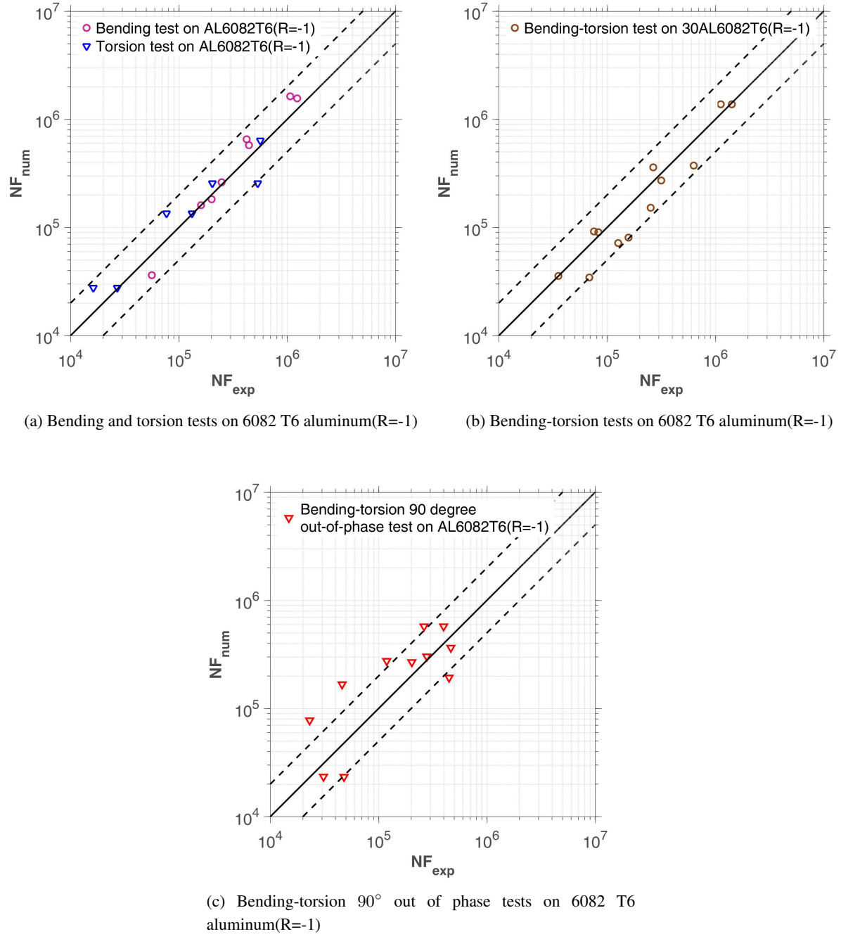
Figure 6.9 – Calibration on on 6082 T6 aluminum ( Susmel and Petrone [2003] ). Comparison between experimental results and our model used with coefficients given in Tab.6.11. We obtain a good correlation in bending and torsion tests. The out of phase test are not satisfactory in these batches: P32BT8, P41BT15, P36BT11.
