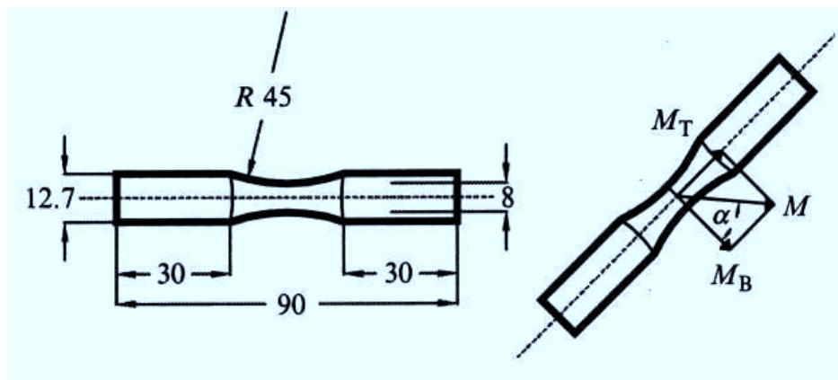
Figure 6.15 – Bending-torsion fatigue tests on cylindrical specimens (Carpinteri et al. [2003])
