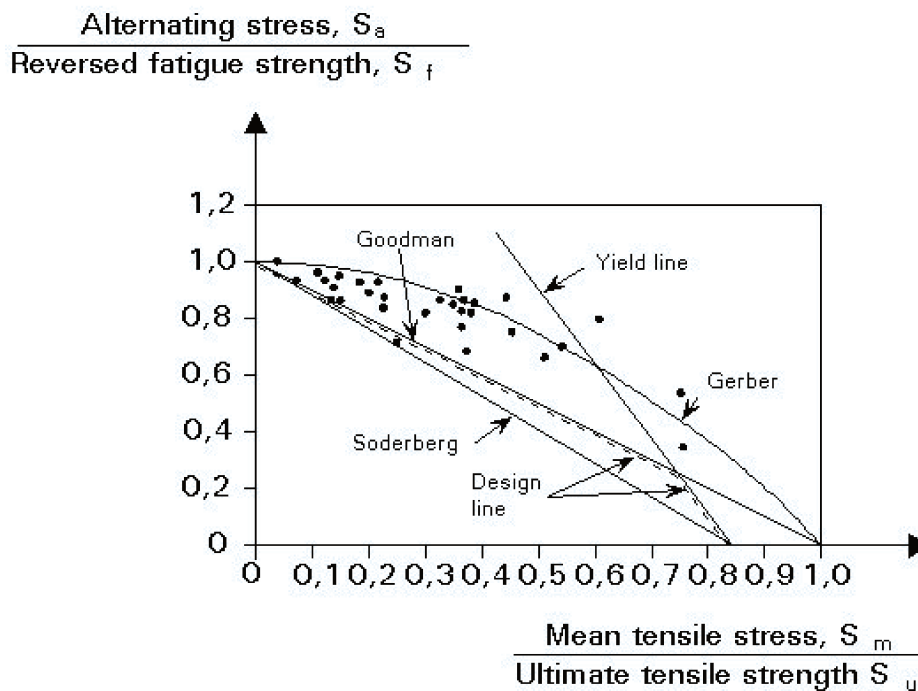
Figure 5.2 – Haigh diagram showing test data points for the effect of mean stress, and the Gerber, modified Goodman and Soderberg relations.
