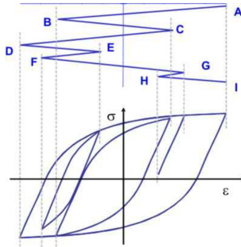
Figure 4.13 – Complex Cyclic Loading
