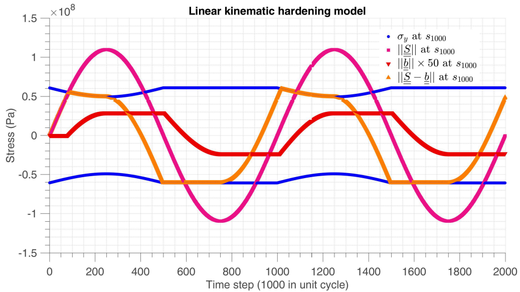
Figure 5.6 – Illustration of uniaxial cyclic load with microscopic plastic dissipation at scale s . With \Sigma_y = 298\text{MPa} , \Sigma_a = 190\text{MPa} , \lambda_+ = 0.9 , \lambda_- = 0 . There is energy dissipation when \|\underline{S} - \underline{b}\|(t) projects on the local yield limit (\sigma_y - \lambda \Sigma_H) / s(t) .
