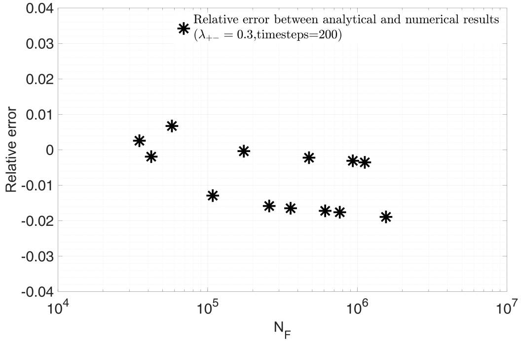
Figure 5.15 – Relative error \left( \frac{NF_{opt} - NF_{analytical}}{NF_{analytical}} \right) between analytical and numerical results with optimal time steps methods ( \beta = 1.1, a = 0.01, \Delta\alpha = 1 \times 10^{-5} in unit cycle)
