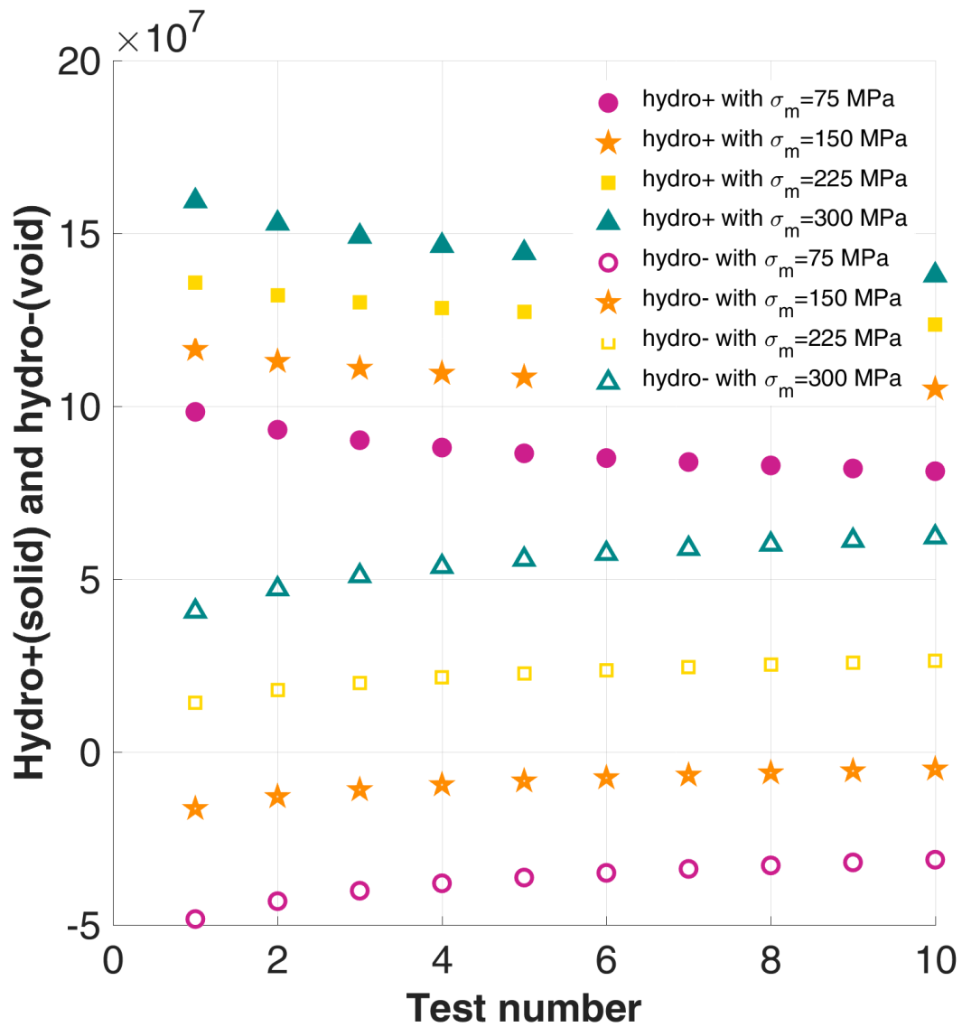
Figure 6.19 – Hydro_{+-} of bending tests with mean stress on 10HNAP
