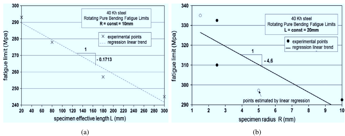
Figure 3.1 – Constant moment bending fatigue limit data: (a) constant radius R ; (b) constant length L (Results of Pogoretskii [1966], represented by Weber [1999]).
