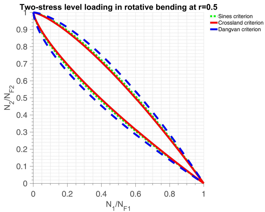
Figure 4.12 – Two-stress level loading in rotative bending at r=0.5 . The lower curve displays the relative proportion of cycles in high-low sequence, the upper curve displays the same information in a low-high sequence
