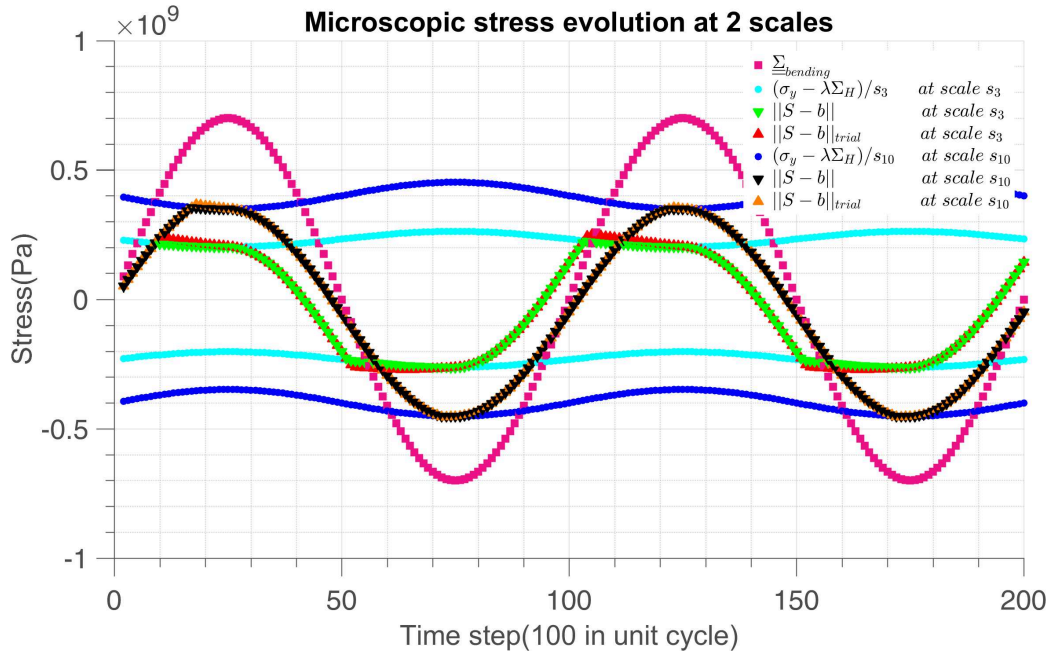
Figure 5.16 – Microscopic (\underline{S} - \underline{b})_{trial} and (\underline{S} - \underline{b}) evolution with time under different weakening scales ( s_3 = 1.21 and s_{10} = 1.13 ) in sinusoidal load with zero mean stress
