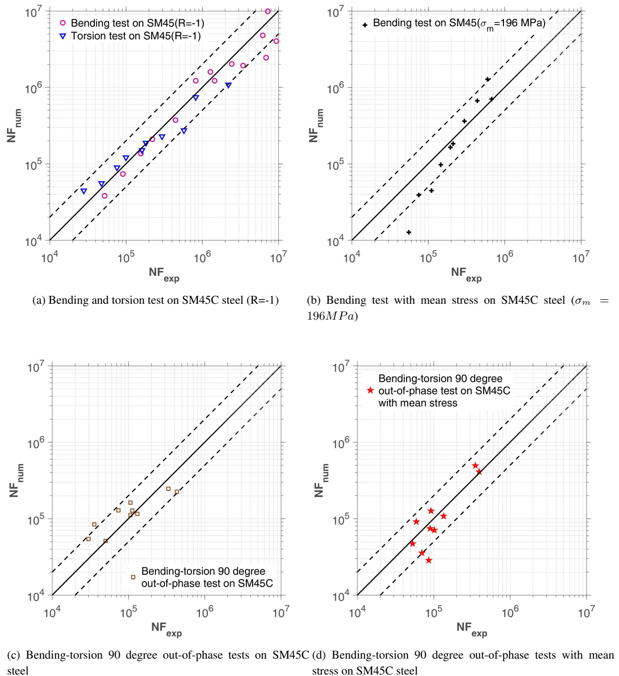
Figure 6.14 – Calibration on SM45C. The numerical tests are carried out using the coefficients of Tab.6.22
