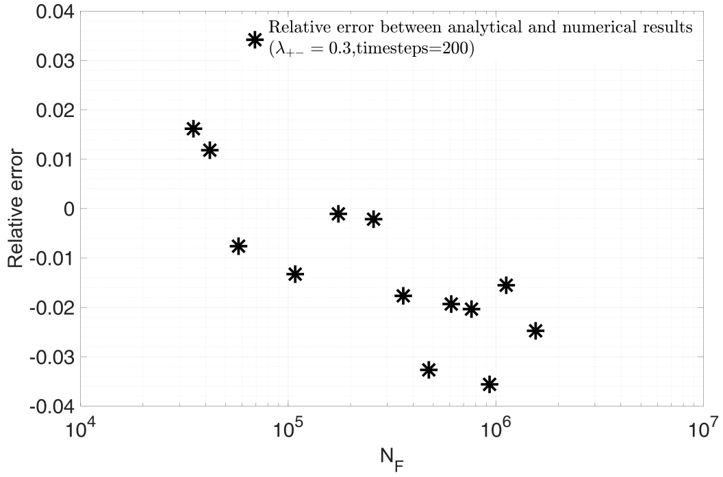
Figure 5.14 – Relative error \left( \frac{NF_{opt} - NF_{analytical}}{NF_{analytical}} \right) between analytical and numerical results with optimal time steps methods ( \beta = 1.1, a = 0.01, \Delta\alpha = 2 \times 10^{-5} in unit cycle)
