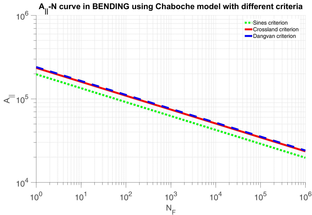
Figure 4.9 – A_{II} - N_F curve in 4-point bending at y=3
