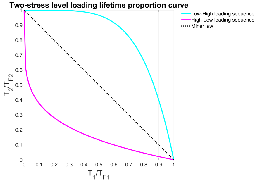
Figure 5.8 – High to low and low to high loading sequence comparison in 4-point bending ( F_{low} = 5000N , F_{high} = 30000N , Radius = 0.2m , \Sigma_u = 167MPa ), with the proposed damage accumulation law (Eq.(5.6.5)) induced equation Eq.(5.6.10) and Chaboche type \alpha (Eq.(5.6.7)) containing Crossland criterion
