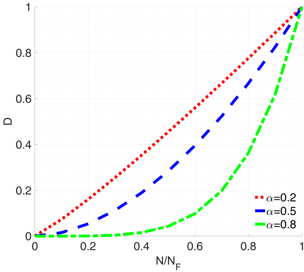
Figure 4.5 – Influence of function \alpha in fatigue damage versus fatigue life ratio ( \hat{\gamma} = 0.1 )
