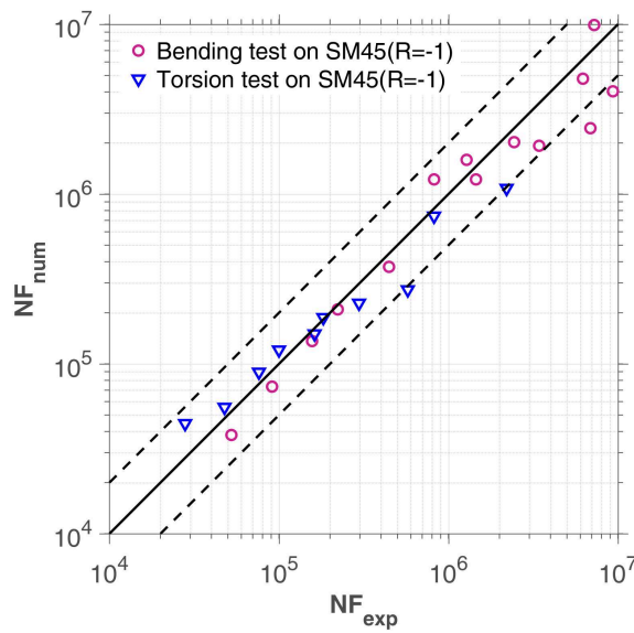
(a) Bending and torsion test on SM45C steel ( R=-1 )
