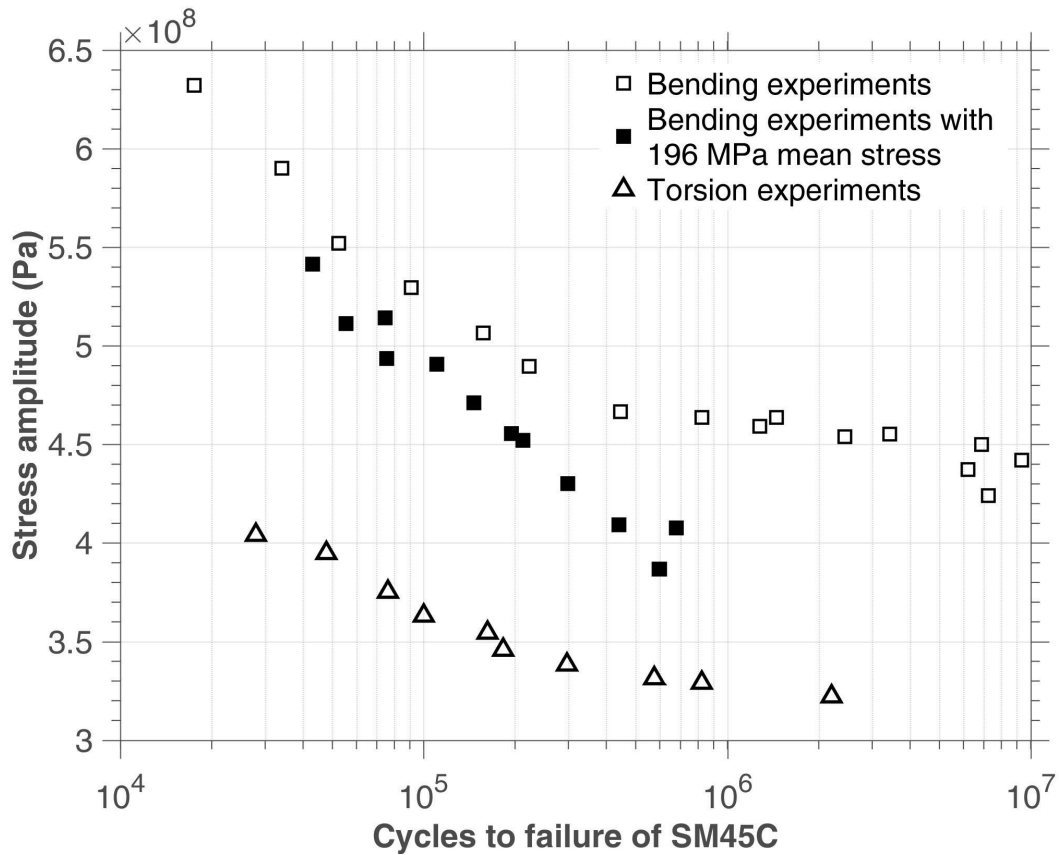
Figure 6.12 – Fatigue curves on SM45C steel by Lee [2013]
