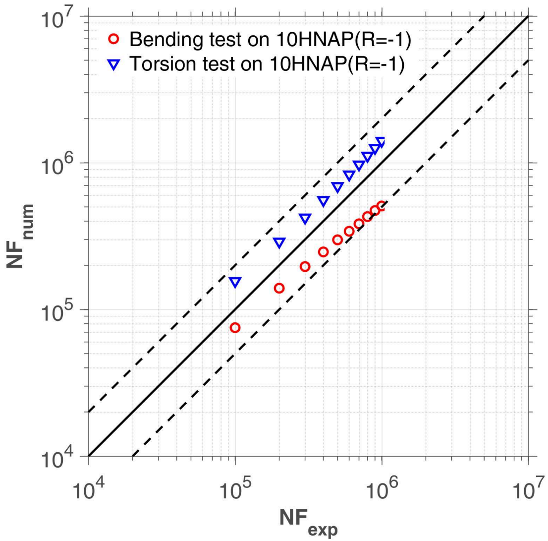
Figure 6.22 – Calibration on 10HNAP steel, bending and torsion tests on 10HNAP(R=-1). Data are presented in Tab.6.30 and 6.31 and results obtained with the coefficients of Tab.6.28
