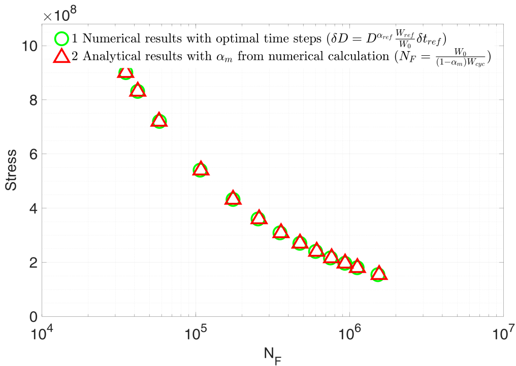
Figure 5.13 – S-N curve using analytical and numerical results with optimal time steps methods ( \beta = 1.1 , a = 0.01 , \Delta\alpha = 1E - 5 in unit cycle), yielding 200 full time steps reduced to 199 optimal time steps
