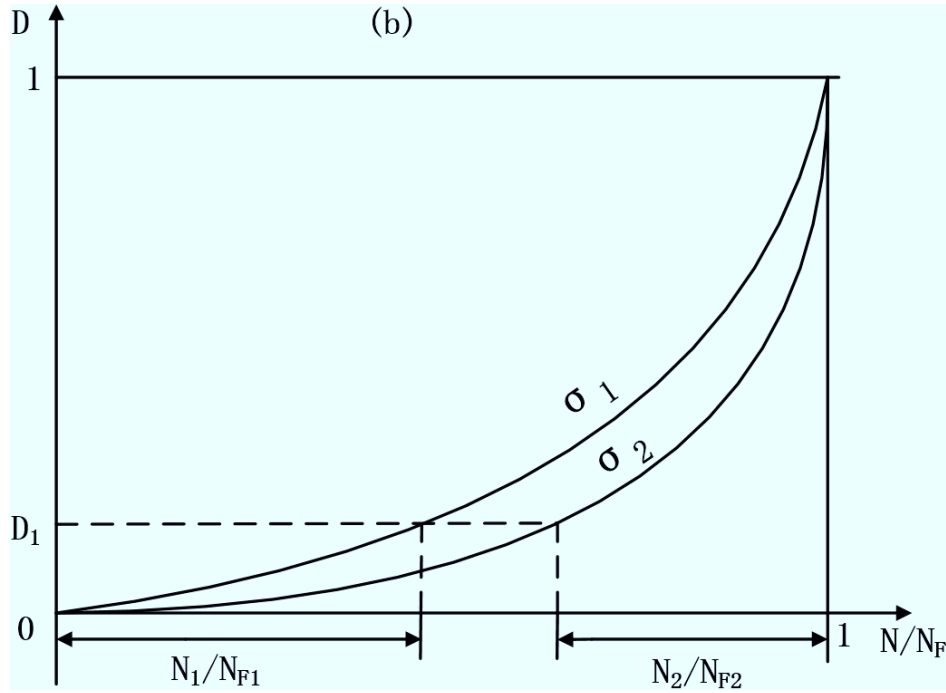
Figure 4.3 – Damage with nonlinear evolution and nonlinear accumulation, where high stress and low stress follow different damage evolution curve. This leads to differences into the summation of fatigue life proportion between different loading sequences.
