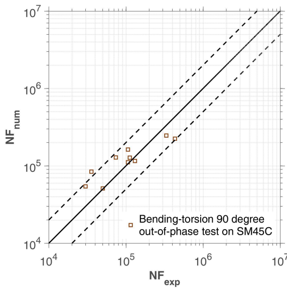
(c) Bending-torsion 90 degree out-of-phase tests on SM45C steel
