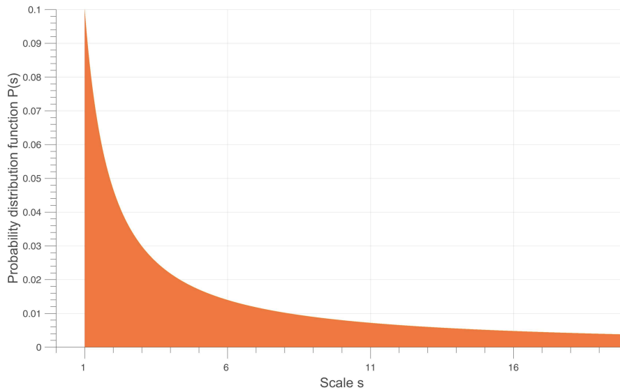
Figure 5.3 – Weakening scales s probability distribution curve when \beta = 1.5
