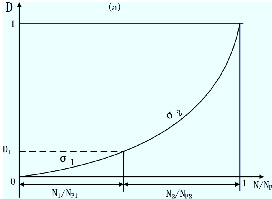
Figure 4.2 – Damage with nonlinear evolution and linear accumulation, where high then low stress loading sequence leads to the same fatigue life.
