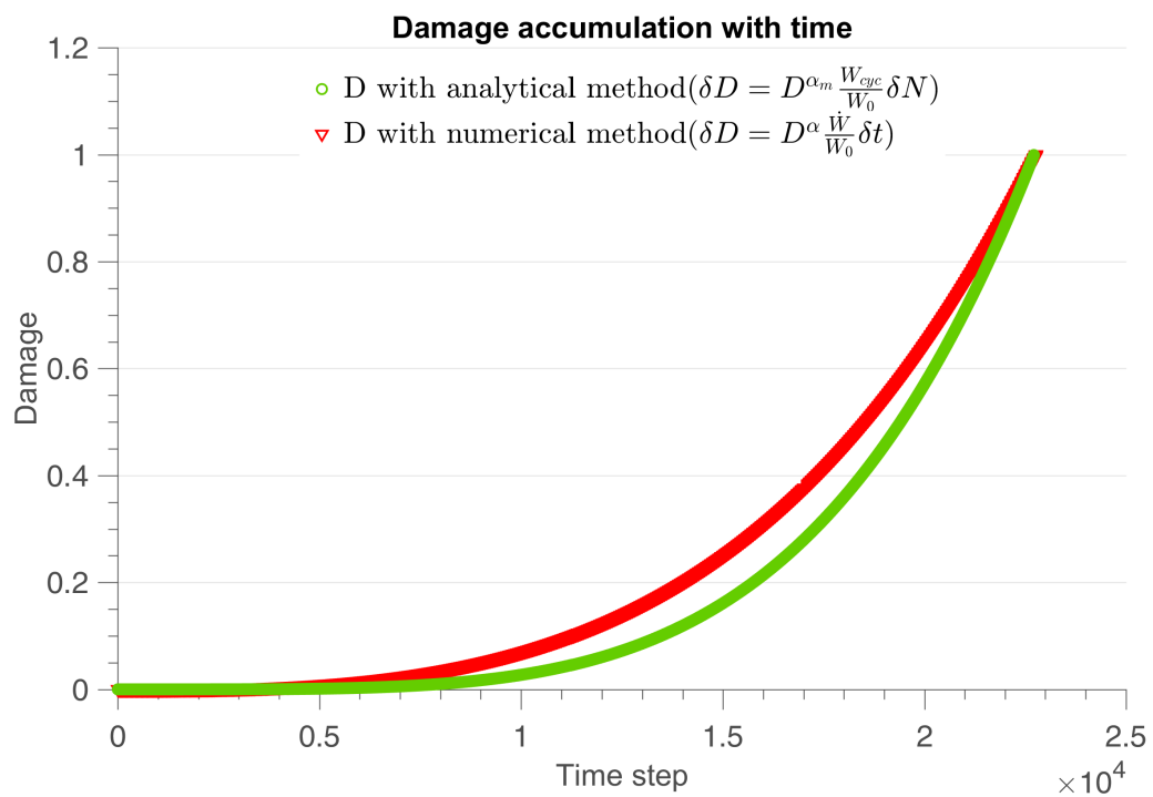
Figure 5.29 – Damage evolution with time under sinusoidal load with \beta = 5 , \Sigma = 0.8\sigma_y
