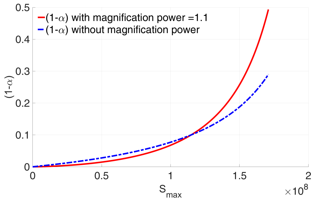
Figure 5.33 – (1-\alpha) term which stands for the load intensity evolution, both with and without the magnification power f
