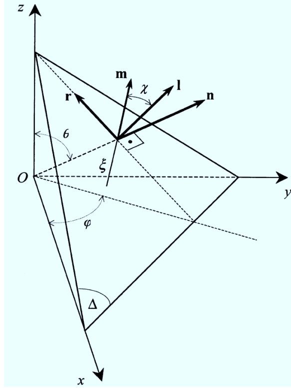
Figure 2.3 – Material plane \Delta passing through point O of a body and its associated (n, l, r) frame (Papadopoulos [1993]).
