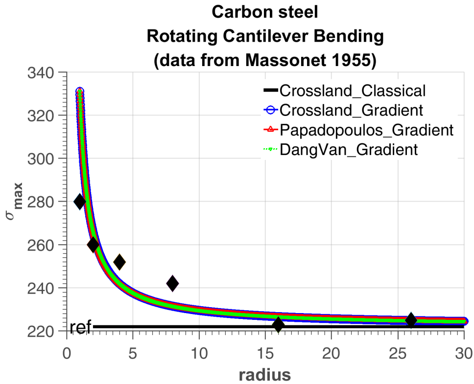
Figure 3.6 – Fatigue limits with gradient effect for different radii (Massonet [1955]).
