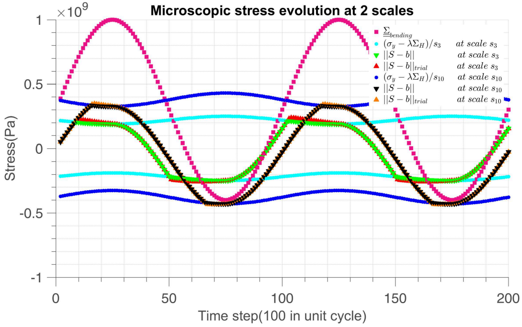
Figure 5.17 – Microscopic (\underline{S} - \underline{b})_{trial} and (\underline{S} - \underline{b}) evolution with time under different weakening scales ( s_3 = 1.21 and s_{10} = 1.13 ) in sinusoidal load with mean stress=300 MPa
