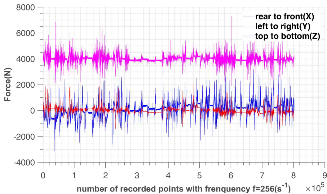
Figure 6.1 – Complex loading of a car suspension arm (data from PSA tests)
