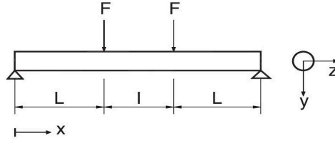
Figure 3.4 – 4-point bending test (Papadopoulos and Panoskaltis [1996])
