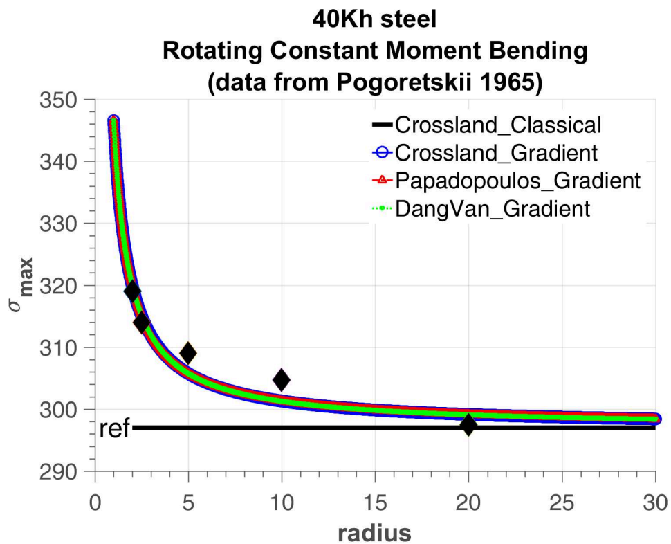
Figure 3.9 – Fatigue limits with gradient effect for different radii (Papadopoulos and Panoskaltis [1996]).
