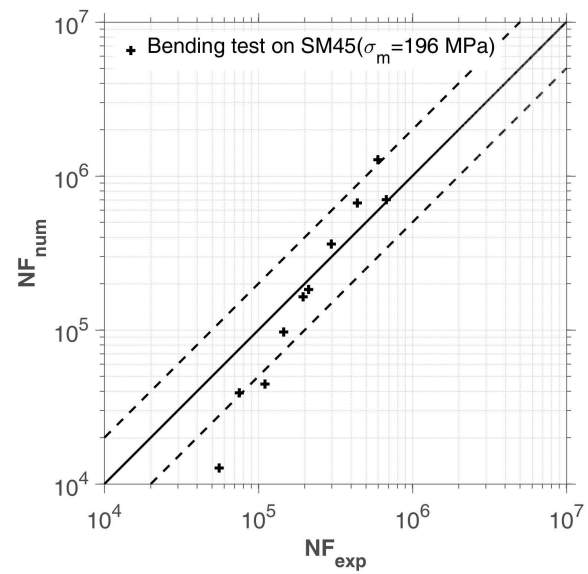
(b) Bending test with mean stress on SM45C steel ( \sigma_m = 196 \text{ MPa} )
