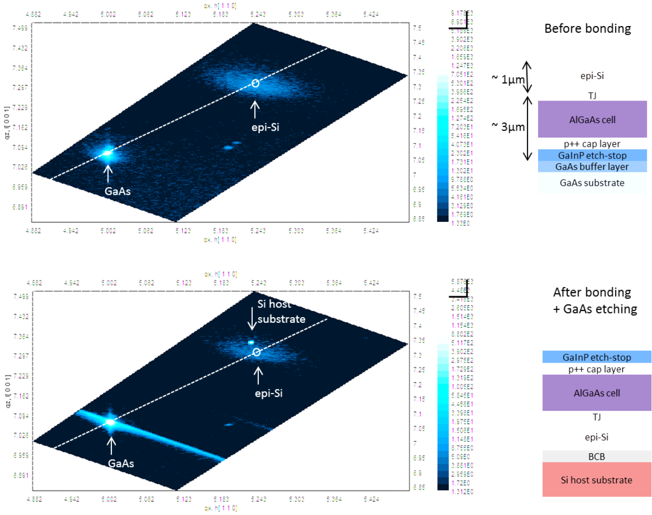
Figure 5.21 - {224} reciprocal space mapping of a tandem stack before and after bonding and substrate removal.
