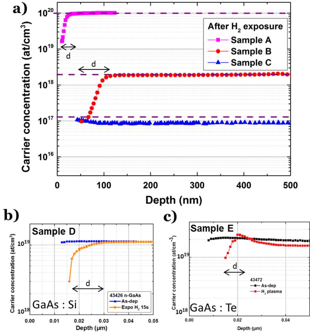
Figure 3.10 - a) Carrier concentration profiles measured by ECV of three p-GaAs:C samples with different initial doping levels, after hydrogen plasma exposure. Dashed lines show the nominal carrier concentrations of each sample. b) c) Carrier concentration profiles before and after plasma exposure for b) GaAs:Si, c) GaAs:Te
