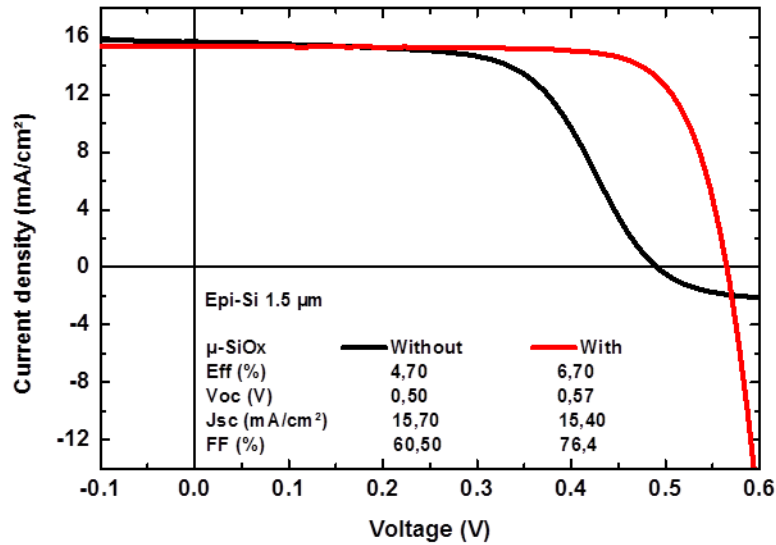
Figure 2.23 - J-V characteristics of as-deposited 1.5 μm thick epi-Si without the addition of μ-SiO x (black curve), and with (red curve)
