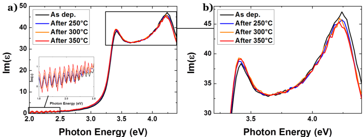
Figure 2.10 - a) Ellipsometric spectra of the samples as-deposited, and annealed at 250°C, 300 °C and 350 °C, along with a zoom on the low energy oscillations b) zoom on the characteristic peaks at E_1 and E_2
