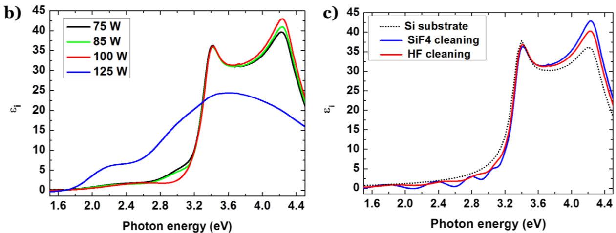
Figure 2.9 - a) Optimized cleaning and deposition conditions in Octopus reactor, b) ellipsometric spectra of 5 minutes growth Si after cleaning at various values of the RF power c) comparison of the best \text{SiF}_4 cleaning with HF cleaning, along with the substrate reference
