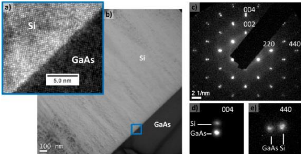
Figure 3.2 - a) Cross-section HRTEM image of epi-Si/GaAs interface. b) Low magnification cross section picture of a 650 nm thick epi-Si layer on GaAs. c) Diffraction pattern of PECVD epi-Si/GaAs interface: the double points visible for each reflection (see zooms (d,e)) are the signature of both Si and GaAs lattices. From Cariou et al. 6
