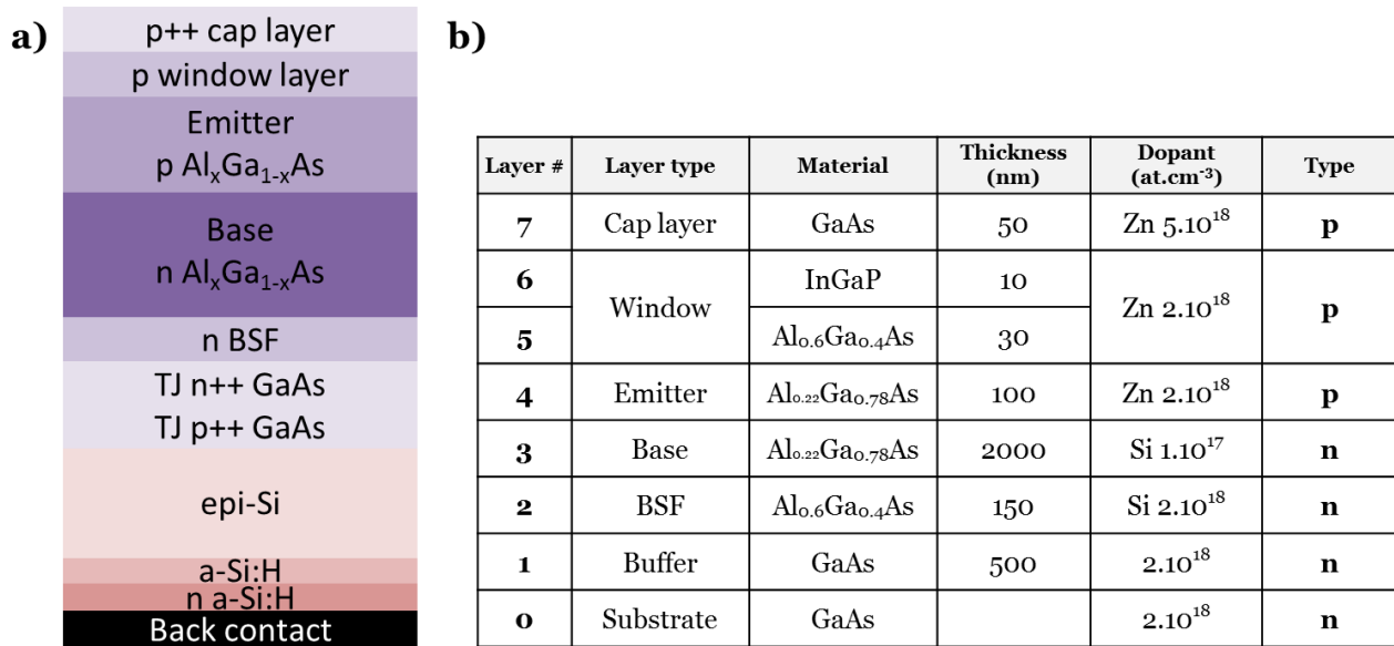
Figure 5.2 - a) Complete structure of the tandem solar cell b) Al 0.22 Ga 0.78 As solar cell structure grown by MOVPE on GaAs substrate
