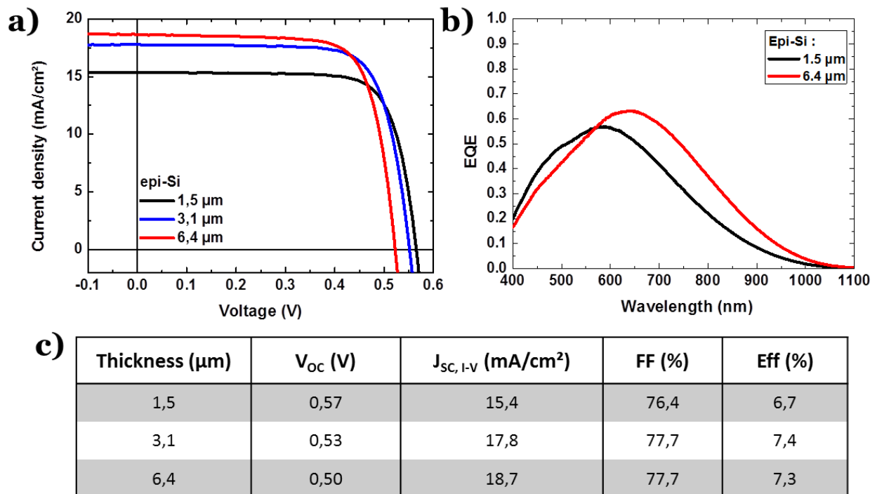
Figure 2.25 - J-V characteristics at low-temperature and b) external quantum efficiency of all the solar cells with various epitaxial thicknesses, c) solar cells characteristics calculated from J-V measurements
