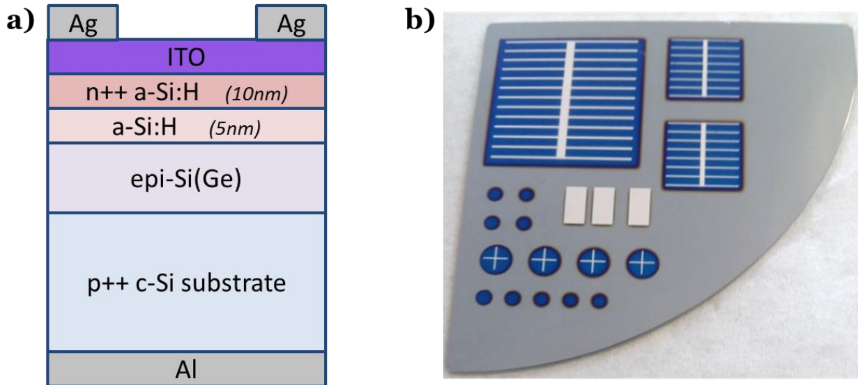
Figure 2.20 - a) Structure of the heterojunction solar cell grown and processed, b) top-view picture of the device after ITO deposition and metallization : one 2 \times 2 \text{ cm}^2 and two 1 \times 1 \text{ cm}^2 cells can be distinguished.
