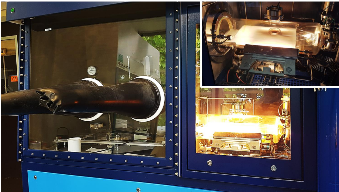
Figure 4.5 - MOVPE reactor with its glovebox while heating. Inset up right: reactor during a process
