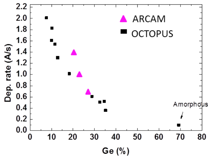
Figure 2.16 - Deposition rate as a function of Ge content for various calibration samples in Octopus reactor (squares) and Arcam reactor (triangle): Deposition rate strongly decreases with %Ge. Too high %Ge leads to amorphous growth.
