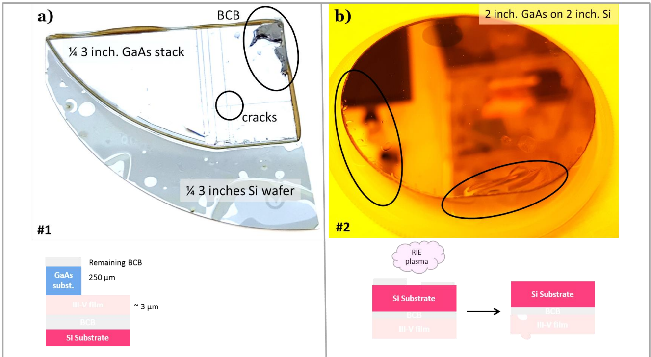
Figure 5.14 - a) Picture a wafer #1 after substrate removal with some remaining BCB, b) picture of wafer #2 after substrate removal followed by a RIE
