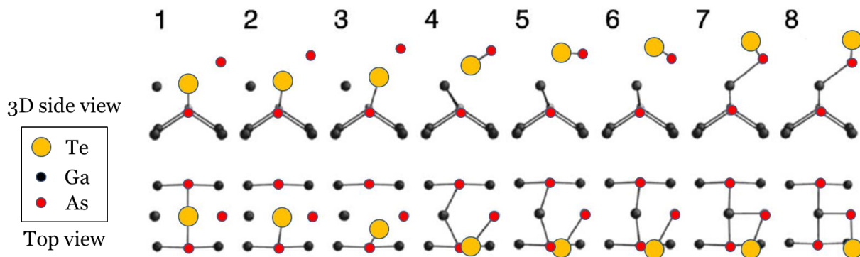
Figure 4.17 - Exchange process between Te surfactant and GaAs (From Consorte et al. 187 )
