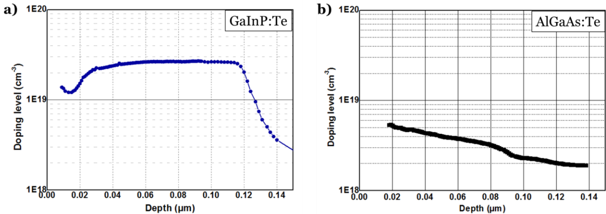
Figure 4.18 - ECV measurements : best doping profiles obtained for a. GaInP doped with Te, b. AlGaAs doped with Te.
