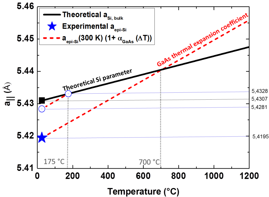
Figure 3.8 - Evolution of a_{\parallel} of a bulk Si as a function of temperature (black) and expected evolution of a_{\parallel} of epi-Si layer that follows the GaAs substrate expansion.
