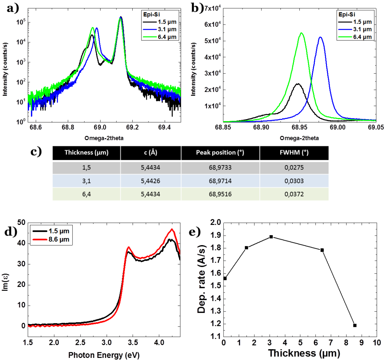
Figure 2.13 - a) \omega -2 \theta XRD scans of samples with various thicknesses: 1.5 \mu\text{m} , 3.1 \mu\text{m} and 6.4 \mu\text{m} , b) zoom on the epi layer peak in linear scale, c) lattice parameter, peak position and FWHM deduced from XRD data d) ellipsometric spectra of 1.5 \mu\text{m} and 8.6 \mu\text{m} samples, e) evolution of deposition rate as a function of the thickness of the film.
