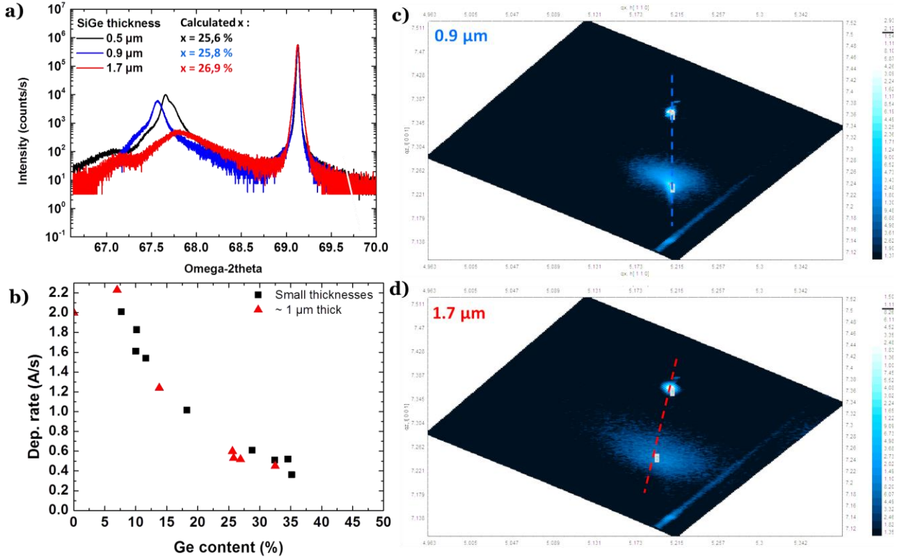
Figure 2.18 - \omega - 2\theta XRD scans of SiGe 25.8 with increasing thicknesses: 0.5 \mu\text{m} , 0.9 \mu\text{m} and 1.7 \mu\text{m} , b) Deposition rate as a function of Ge content for the thin calibration layers (<200 nm) and the thick layers. c)d) RSM of 0.9 and 1.7 \mu\text{m} samples: the latest is partly relaxed.
