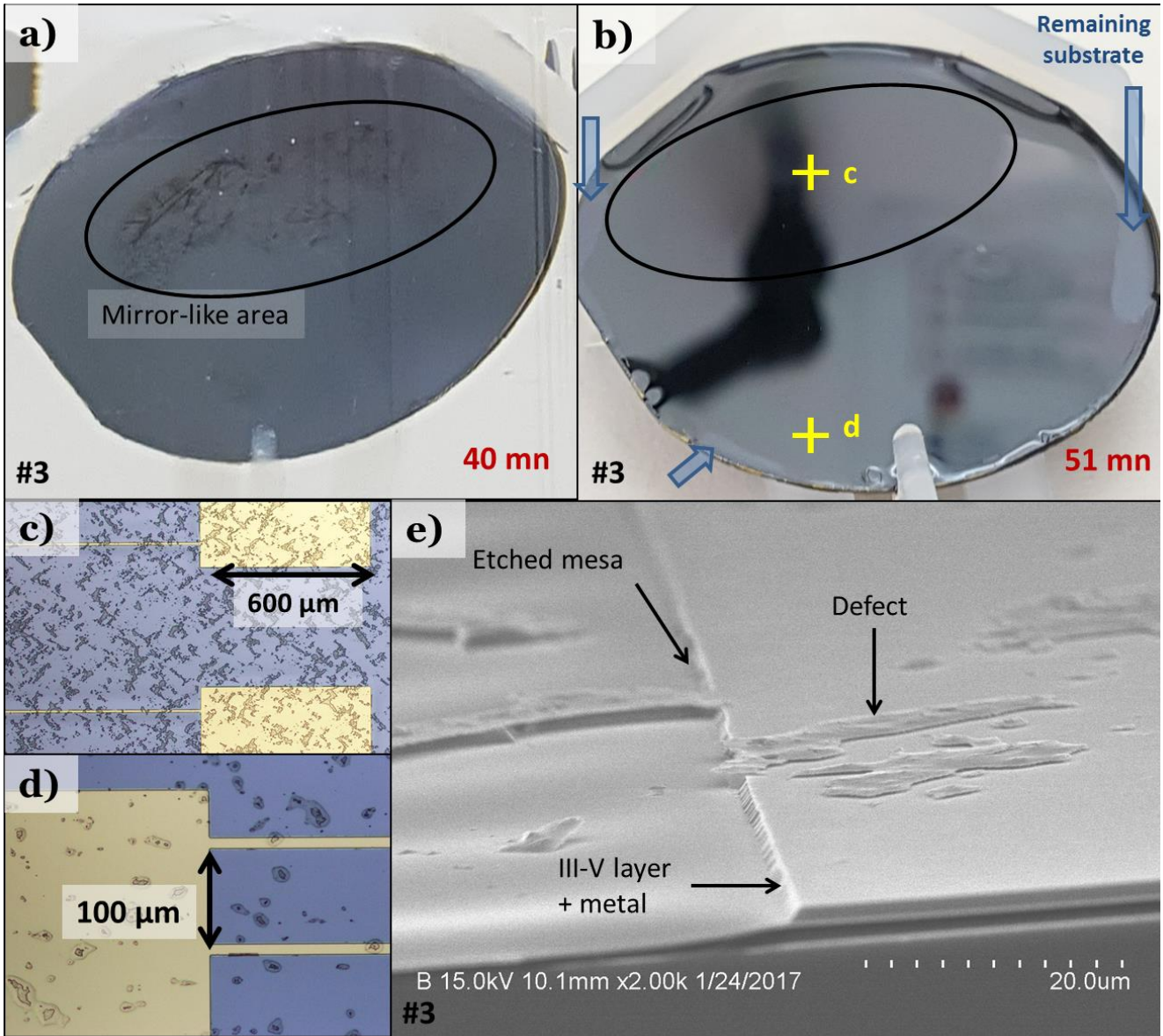
Figure 5.15 - a) Picture of wafer #3 after 40 mn of wafer etching, b) after 51 mn. c) and d) microscope images of the surface in area c and d, e) SEM image in area c.
