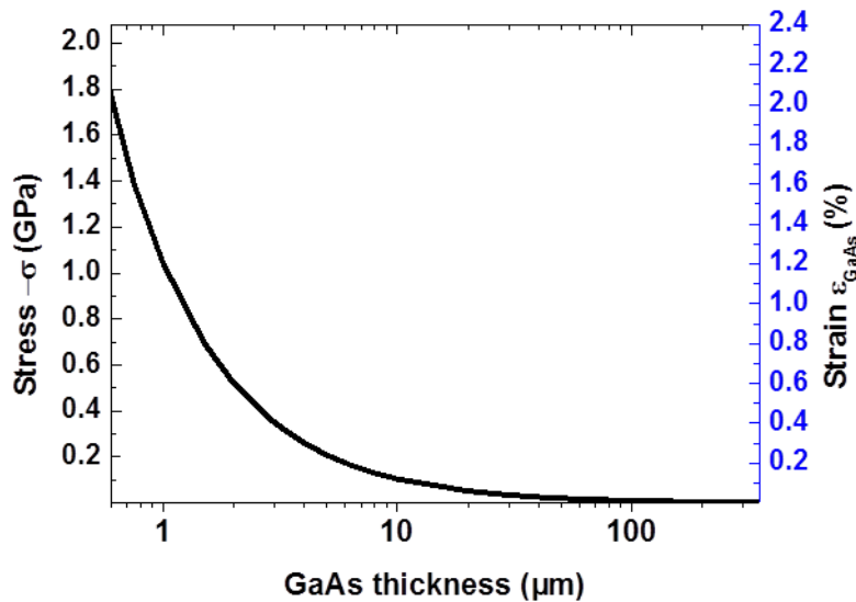
Figure 5.23 : Stress and strain in the III-V stack during GaAs substrate removal
