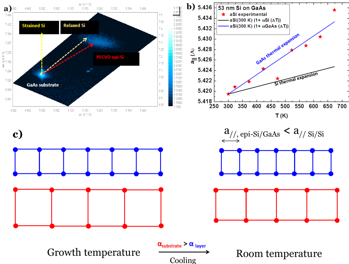
Figure 3.7 - a) {224} reciprocal space mapping of an epi-Si/GaAs sample, b) evolution of the lattice-parameter of an epi-Si while performing an annealing up to 400 °C, c) Schematics of the lattice of a relaxed Si layer on top of a GaAs during growth, and after cooling down to room temperature, considering that Si follows GaAs thermal expansion coefficient.
