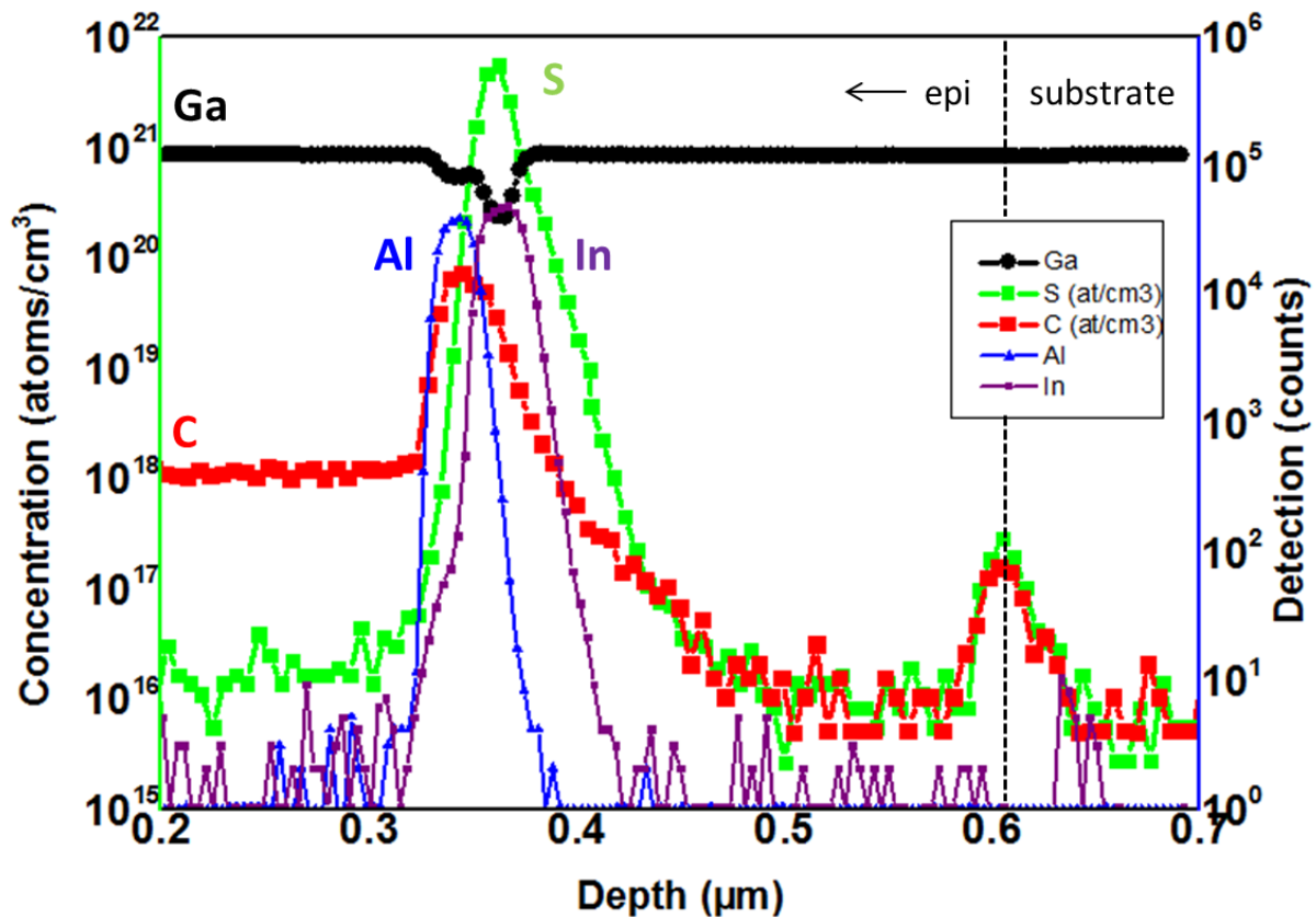
Figure 4.11 - SIMS analysis of AlGaAs/GaN tunnel junction.
