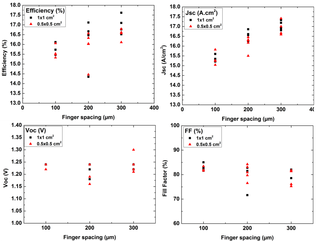
Figure 5.10 - Solar cell parameters as a function of the finger spacing. Black squares correspond to the large cells ( 1 \times 1\text{ cm}^2 ) and red triangles to the small ones ( 0.5 \times 0.5\text{ cm}^2 )
