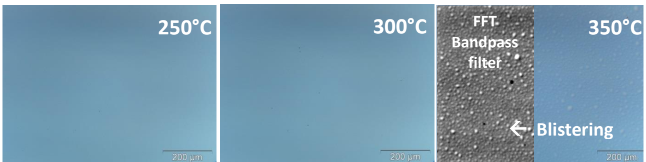
Figure 2.12 - Optical microscope images of the sample surface for different annealing temperatures
