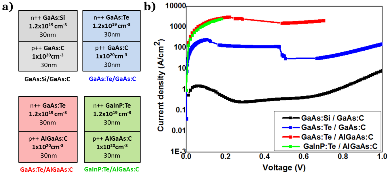
Figure 4.20 - a) Tunnel junction structures b) and J-V characteristics
