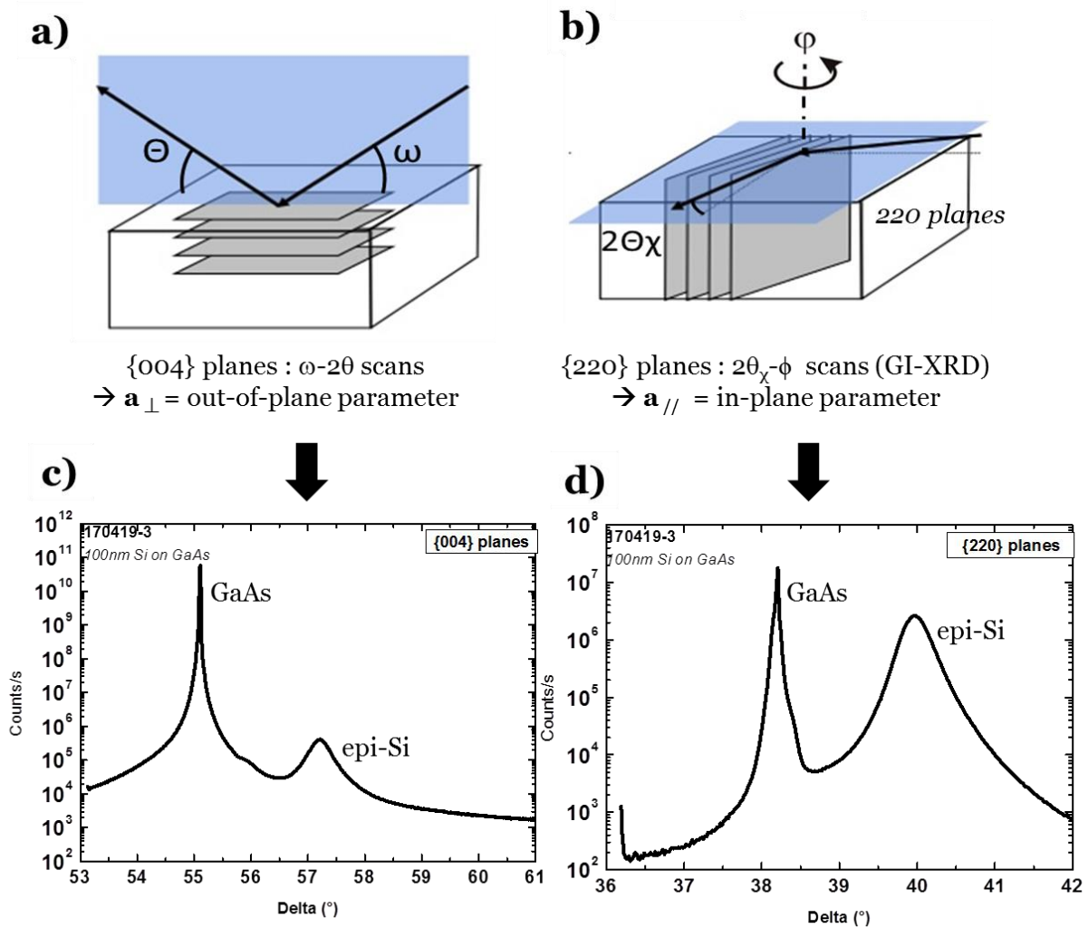
Figure 3.3 - Schematics of a sample and the planes probed in a) a \omega - 2\theta configuration b) GIXRD configuration. c) and d) corresponding scans on a 100 nm thick epi-Si sample on GaAs.
