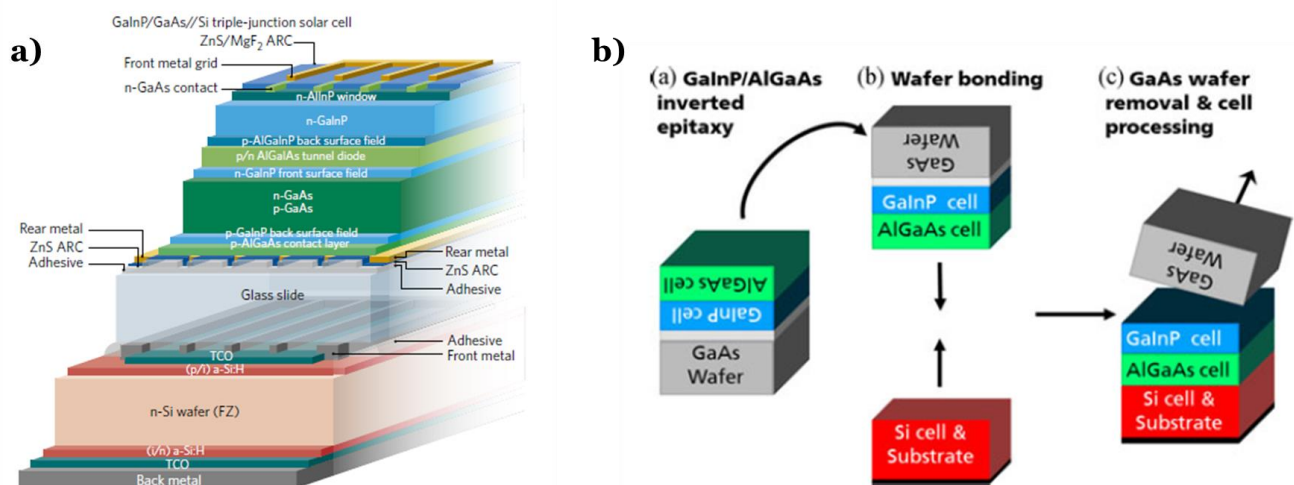
Figure 1.14 - a) Design of the four-terminal GaInP/GaAs//Si triple junction solar cell with 35.9 % efficiency (Essig et al. 50 ) b) Design and process flow of GaInP/AlGaAs//Si triple junction wafer-bonded solar cell with 30.1% efficiency (Cariou et al. 47 )
