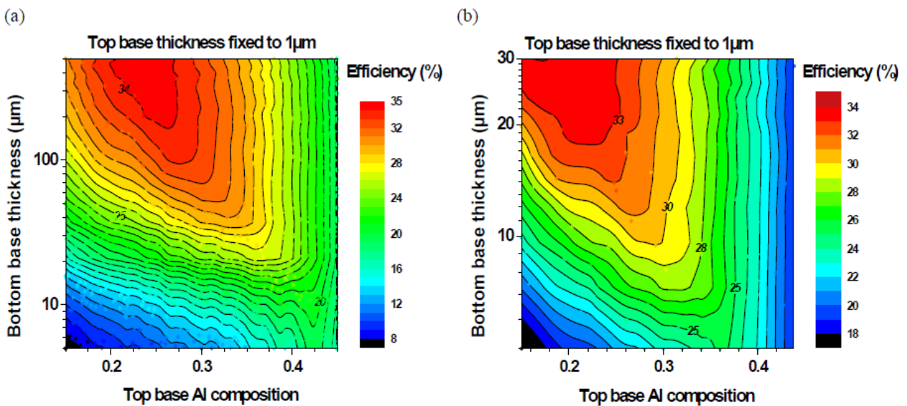
Figure 1.17 - Maps of tandem cell efficiencies simulated for different combinations of top base Aluminum compositions and bottom base thicknesses: (a) for a bottom cell in epi-Si and (b) for a bottom cell in epi-Si 0.63 Ge 0.27
