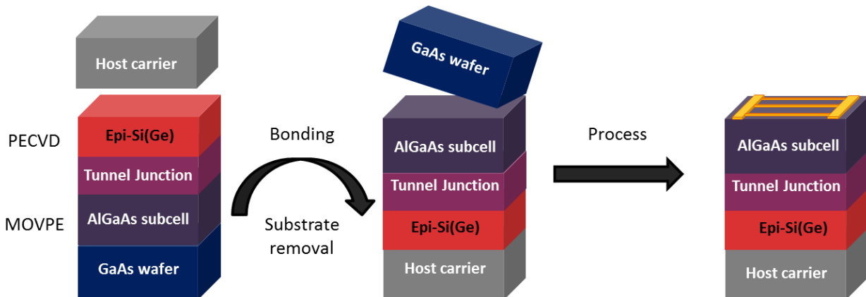
Figure 1.15 - Principle of the IMPETUS project. AlGaAs is grown on a GaAs substrate by MOVPE, followed by a tunnel junction and crystalline Si or SiGe grown by PECVD below 200 °C. The structure grown is then transferred to a low-cost carrier, the substrate removed, and the device is fabricated by standard clean room processes.
