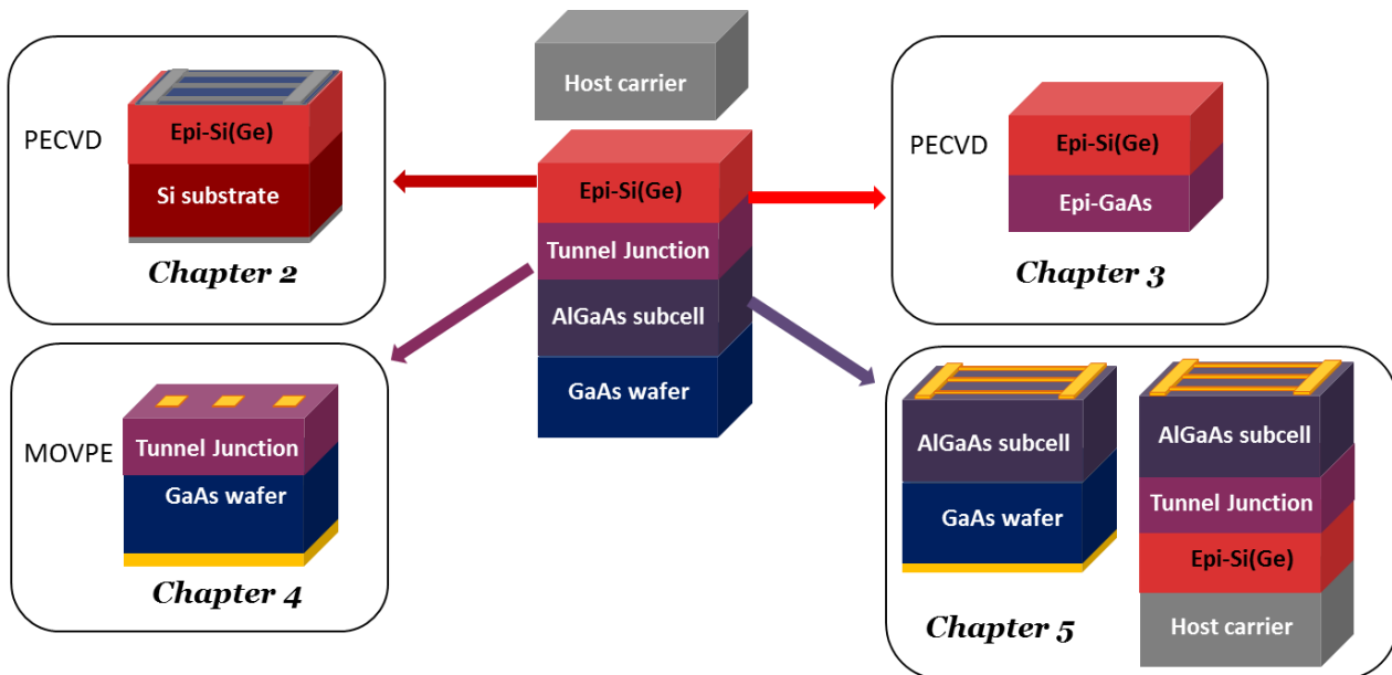
Figure 1.18 - Different building blocks of the tandem solar cell
