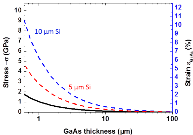
Figure 5.24 - Stress and strain in the III-V stack during GaAs substrate removal for various epi-Si thicknesses
