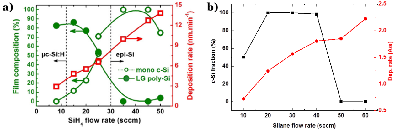
Figure 2.8 - Deposition rate and percentages of monocrystalline silicon, as deduced from spectroscopic ellipsometry measurements, plotted as a function of the silane flow rate. a) from Roca I Cabarrocas et al. 22 in Arcam reactor, b) in Octopus reactor
