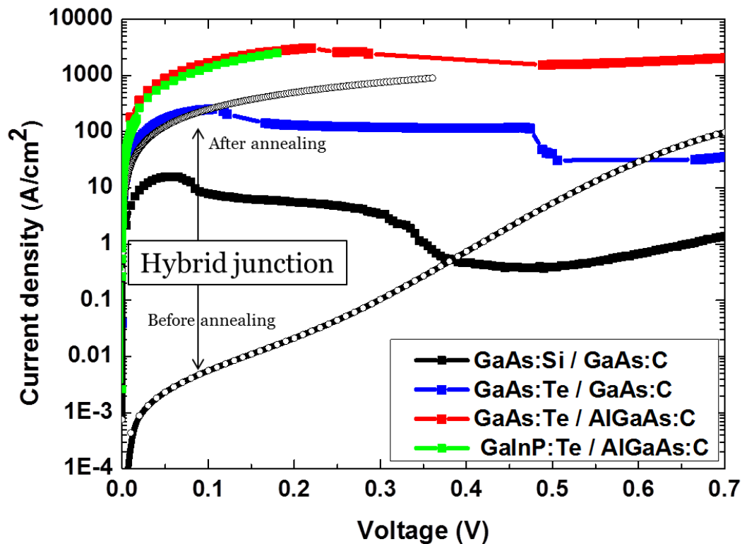
Figure 4.25 - Hybrid Si/GaAs junction as compared with III-V tunnel junctions before and after annealing
