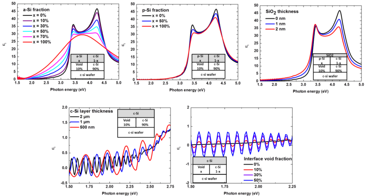
Figure 2.4 - Ellipsometric spectra (imaginary part of the dielectric function) simulated with DeltaPsi2 by varying a) c-Si/a-Si fraction, b) c-Si/p-Si fraction, c) native SiO 2 thickness d) c-Si thickness e) roughness or defectivity of interface between substrate and epi-layer
