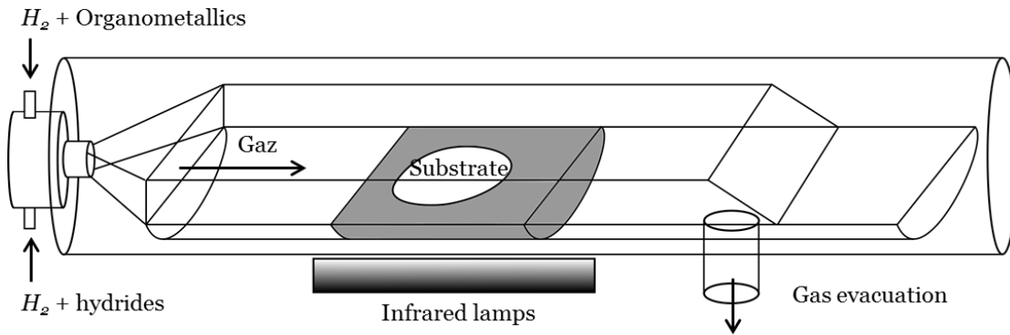
Figure 4.4 - Principle of the AIX200 reactor
