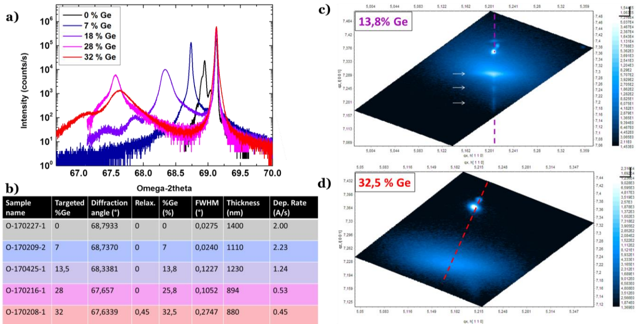
Figure 2.17 - \omega - 2\theta XRD scans of \text{Si}_{1-x}\text{Ge}_x for various x values, aiming at a thickness of 1\ \mu\text{m} b) fitted parameters deduced from XRD (diffraction angle, Ge content, FWHM) and SEM (thickness) d), RSM of the samples with x=13.8\% and x=32.5\% samples: the latest is partly relaxed.
