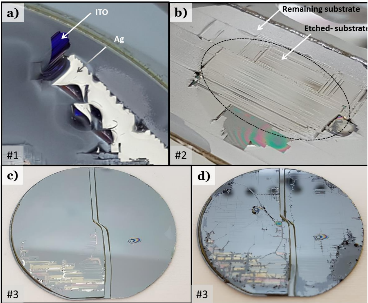
Figure 5.20 - a) Picture of layer detachment between Ag and ITO, b) picture of a tandem solar cell (#2) after 750 \mu\text{m} -thick GaAs substrate removal, c) picture of a tandem solar cell (#3) after 350 \mu\text{m} - thick substrate removal d) #3 after GaInP etch-stop etching
