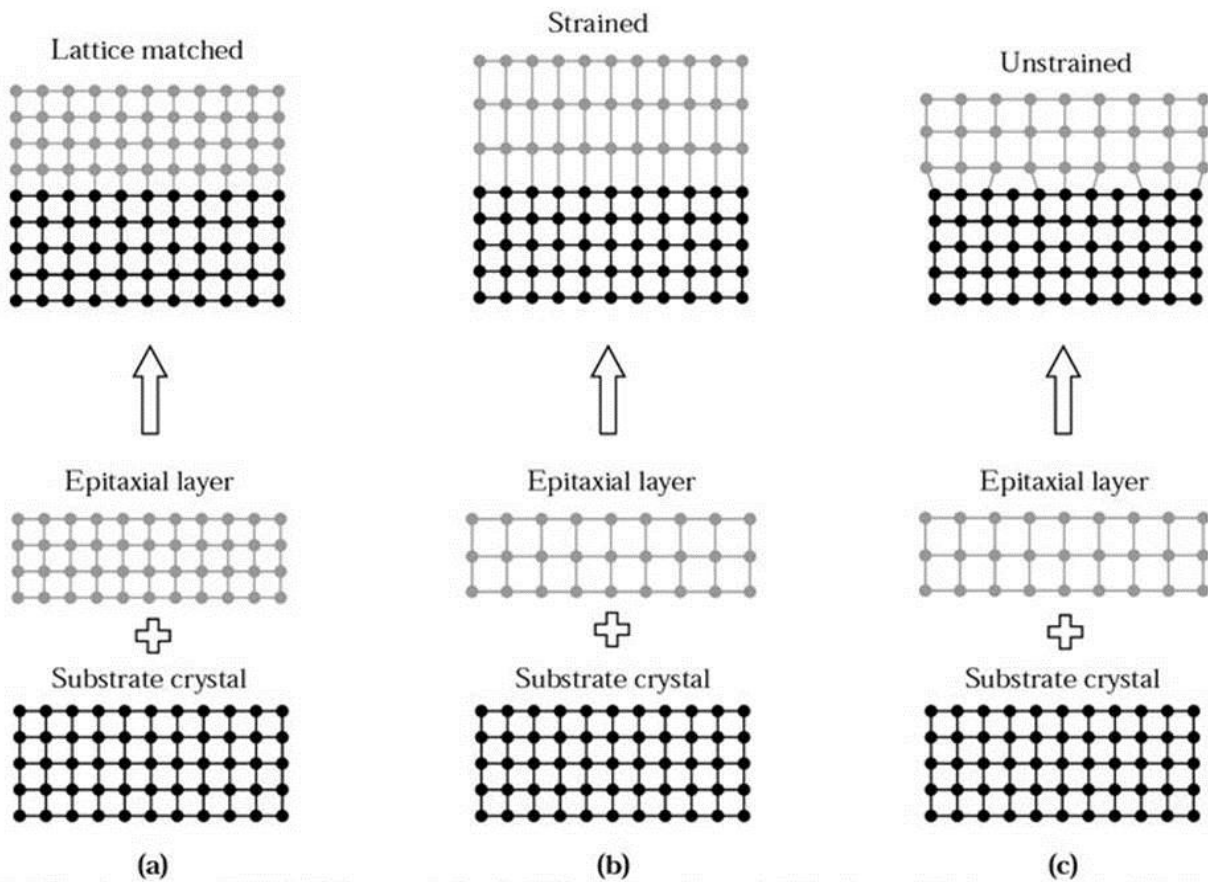
Figure 1.7 - Schematic illustration of (a) lattice-matched, (b) strained and (c) relaxed hetero-epitaxial structures. (b) and (c) are shown in case of a_{\text{substrate}} < a_{\text{layer}} (22)
