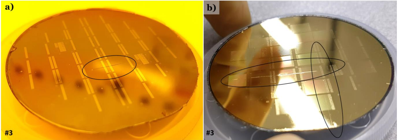
Figure 5.16 - Wafer #3 a) after resist deposition, b) after front metal deposition
