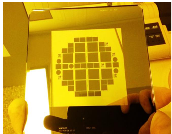
Figure 5.5 - Picture of the lithographic mask used to define the mesa etching pattern
