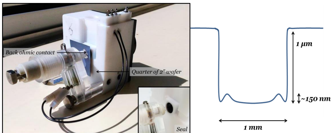
Figure 3.9 - a) Picture of the electrochemical cell used in ECV. Inset down right: picture of the seal that contacts the wafer surface b) Depth profile of a typical crater after etching.
