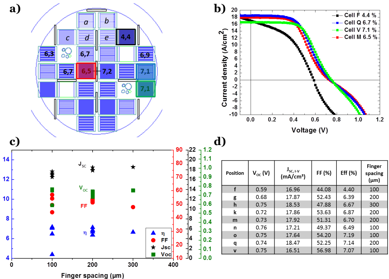
Figure 5.18 - a) Spatial repartition of the different cells that are not shunted with their efficiency. b) J-V curve of 4 of these functioning cells c) V oc , J sc , FF and efficiency as a function of the finger spacing, d) Results on each functioning cell
