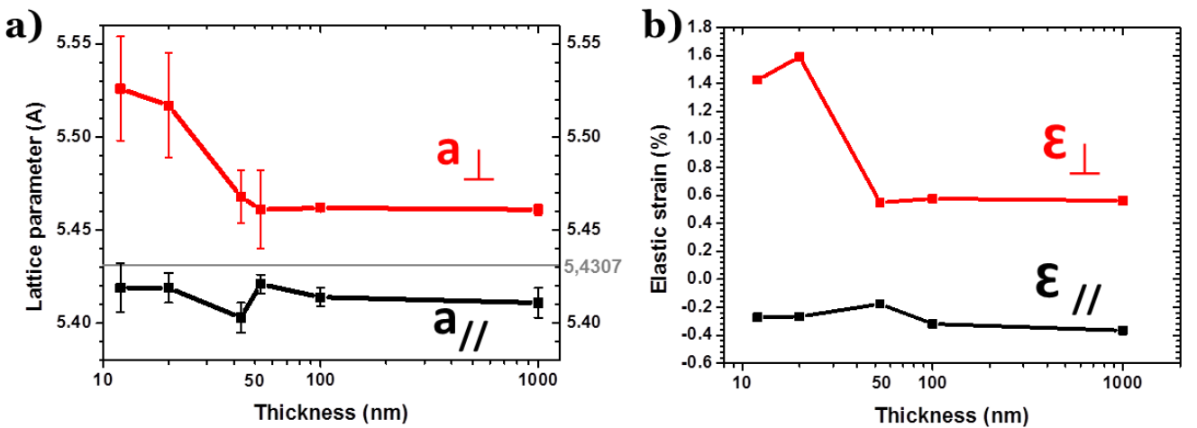
Figure 3.5 - a) evolution of the in-plane ( a_{\parallel} ) and out-of-plane ( a_{\perp} ) lattice parameters as a function of the layer thickness, b) elastic deformation as a function of the layer thickness.
