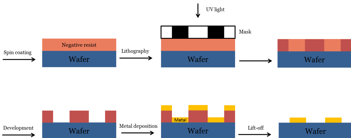
Figure 4.6 - Detailed process of a metal pattern by lift-off technique
