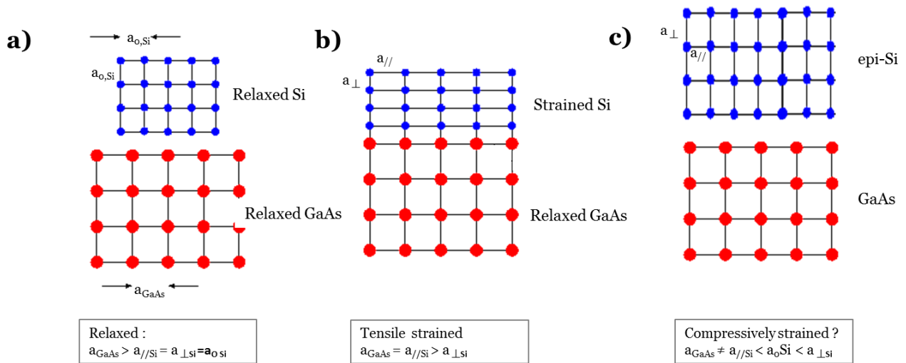
Figure 3.4 - Schematics of an heteroepitaxy in case of a larger substrate lattice constant than that of the epi-layer in the a) relaxed configuration, b) strained configuration (tensile strain) c) schematics of four epi-Si/GaAs according to the lattice parameters deduced from XRD measurements
