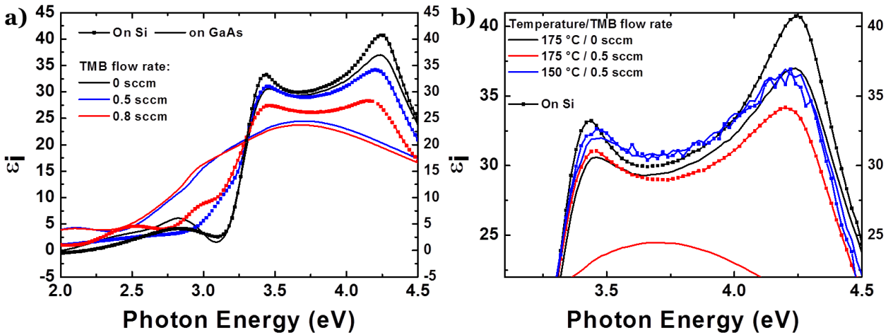
Figure 4.24 - a) Ellipsometric spectra of Si grown with TMB on Si substrate (squares) and on epi-GaAs (lines) with various TMB flow rates, b) Ellipsometric spectra on Si and epi-GaAs at various TMB flow rate and temperatures
