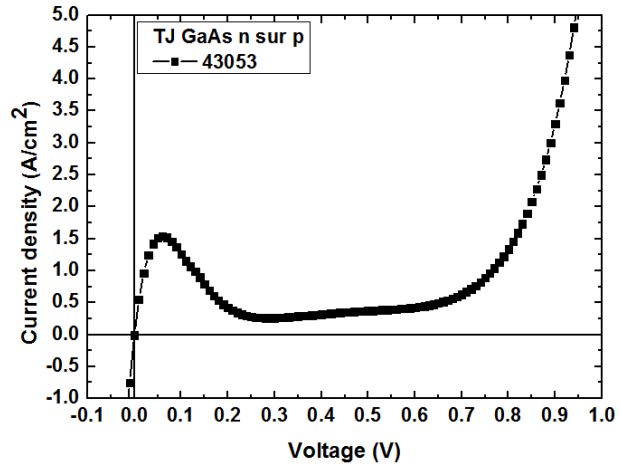
Figure 4.9 - J - V characteristics of n on p GaAs tunnel junction
