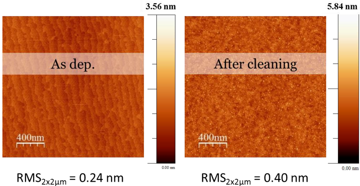
Figure 3.1 - AFM images of the surface of the epitaxial GaAs layer before and after plasma cleaning under optimized process conditions for Si heteroepitaxy
