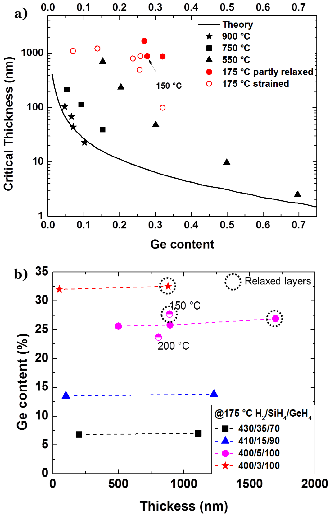
Figure 2.19 - a) Critical thickness of SiGe reported from Hull et al. 107 as a function of the growth temperature, compared to our samples. Low-temperature PECVD has a higher critical thickness than other techniques b) Ge content as a function of thickness for various growth conditions.
