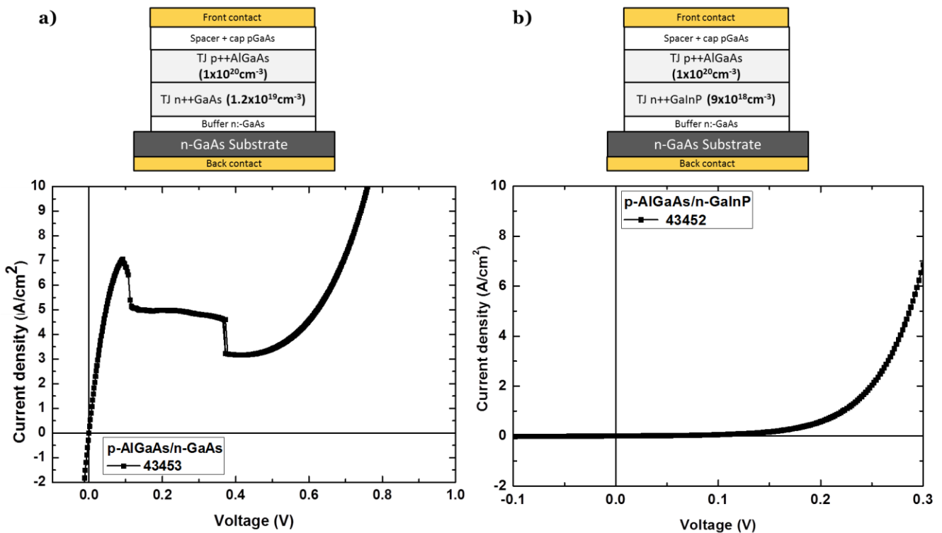
Figure 4.10 - Structure and J-V characteristics of a) AlGaAs/GaAs tunnel junction and b) AlGaAs/GaInP
