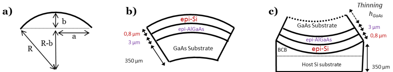
Figure 5.22 - a) schematics of the radius of curvature as a function of the bowing, b) schematics of the tandem solar cell before bonding, c) schematics of the tandem solar cell after bonding during substrate removal
