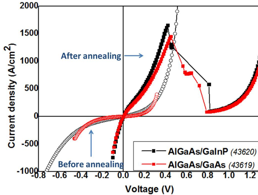
Figure 4.22 - J-V characteristics of AlGaAs/GaInP (black) and AlGaAs/GaAs (red) tunnel junctions before (open symbols) and after annealing (full symbols)
