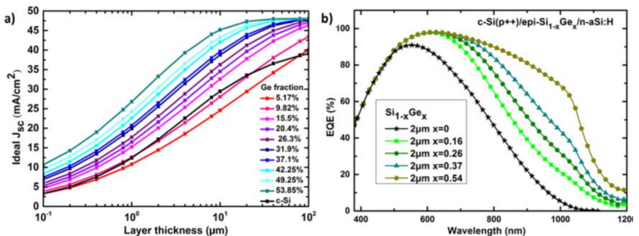
Figure 2.26 - Ideal J_{sc} as a function of SiGe thickness for various Ge content. b) PC1D model of EQE variation with Ge content for a (p++)c-Si/epi-SiGe/n-a-Si:H solar cell. From Cariou thesis p155.
