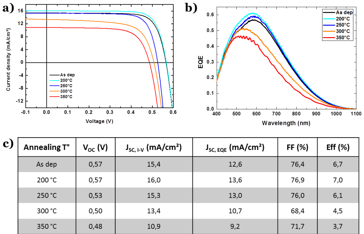
Figure 2.24 - a) J-V characteristics at low-temperature and b) external quantum efficiency of all the solar cells processed after various annealing temperatures, c) Solar cells characteristics calculated from I-V measurements and EQE
