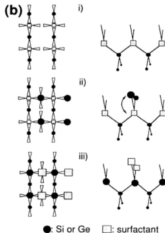
Figure 4.16 - Schematic representation of atomic mechanisms with reactive surfactant (from Grandjean et. al. 186 )
