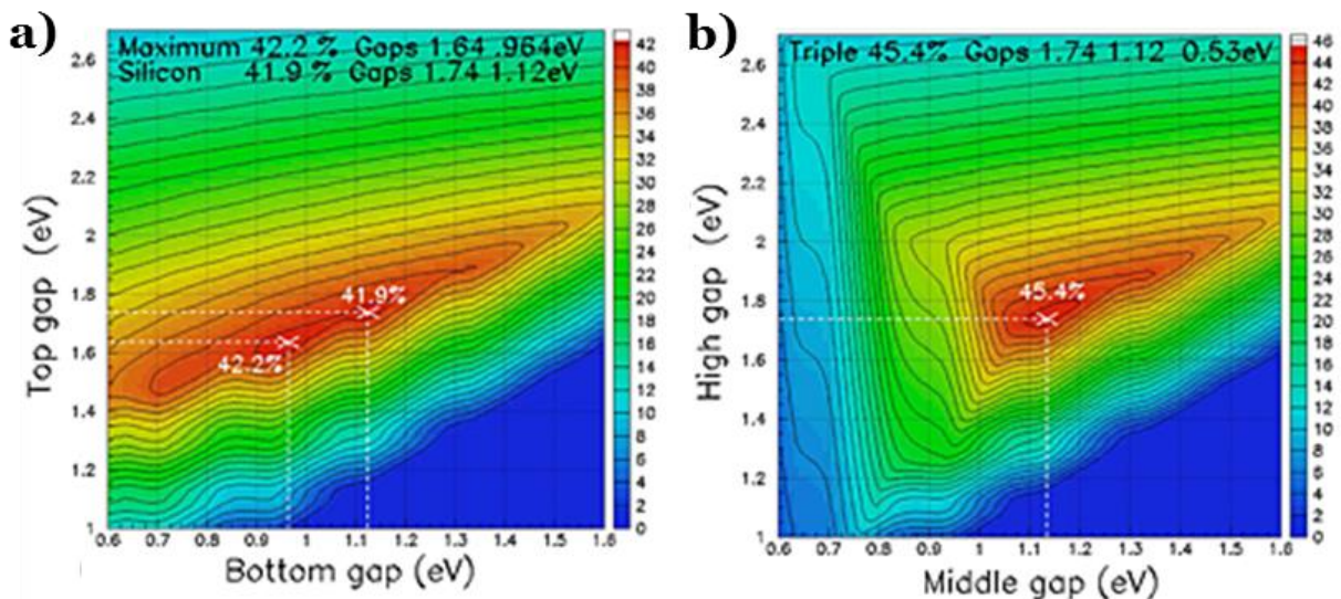
Figure 1.6 - a) Theoretical efficiencies for a tandem junction as a function of top cell and bottom cell bandgaps, when connected in series b) Theoretical efficiencies for a triple junction as a function of top and middle bandgap subcells. (Connolly et al. 18 )
