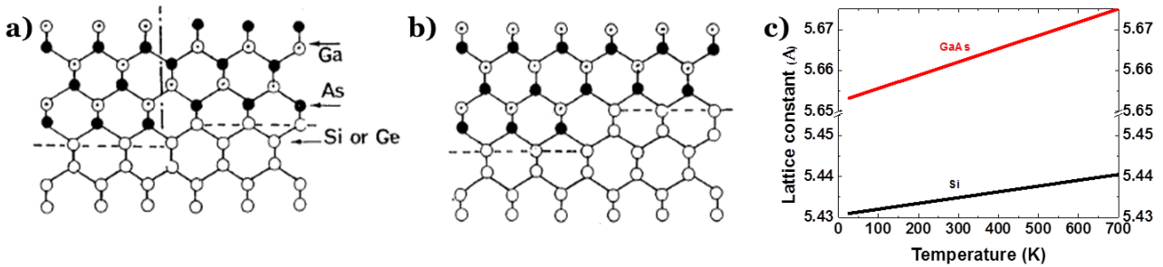
Figure 1.8 - (a) Mechanism of APB formation during the growth of zinc blende structure on (100) non polar surface presenting single-atomic high step, (b) Growth of a single domain zinc blende structure on a (100) non polar surface presenting double-atomic high step (from Freundlich 23 ) (c) lattice constant of GaAs and Si as a function of temperature
