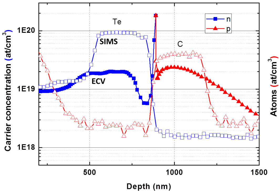
Figure 4.19 - ECV measurements (full symbols) as compared with SIMS analyses (open symbols) of a n on p GaAs/GaAs tunnel junction doped with Te and C.
