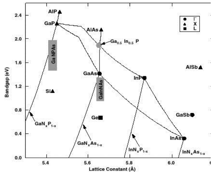
Figure 1.12 - Bandgap versus lattice constant including dilute nitride materials
