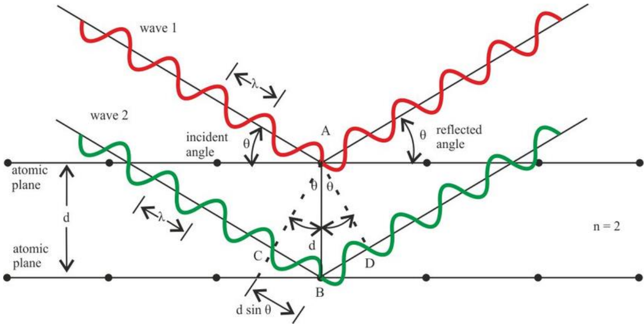
Figure 2.5 - Schematic representation of Bragg's law
