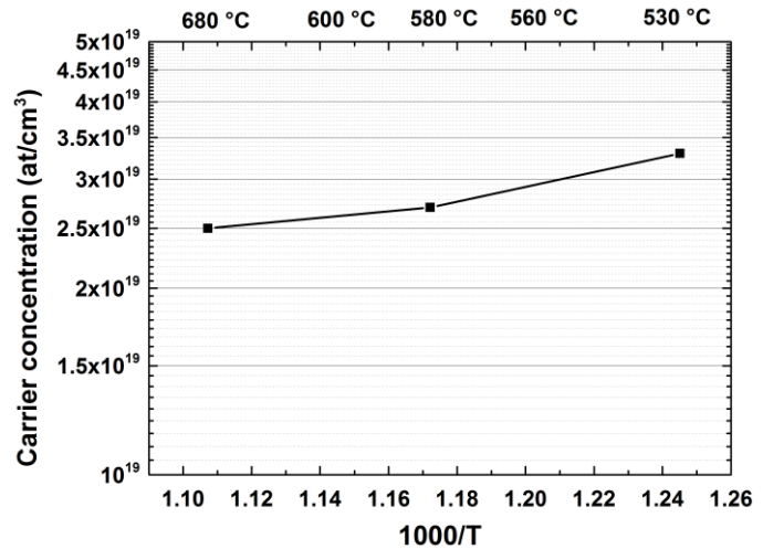
Figure 4.13 - Carrier concentration as a function of temperature
