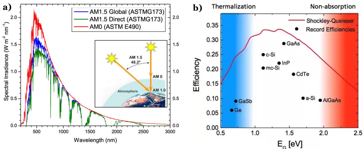
Figure 1.1 - a) Incident spectral irradiance from the sun for terrestrial applications (AM1.5G and AM1.5D) and space applications (AM0). b) Shockley-Queisser limit: maximum theoretical efficiency of a solar cell as a function of its bandgap, along with the best experimental efficiencies
