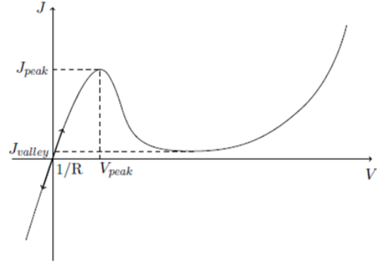
Figure 4.2- Typical J-V curve of a tunnel junction, and main parameters
