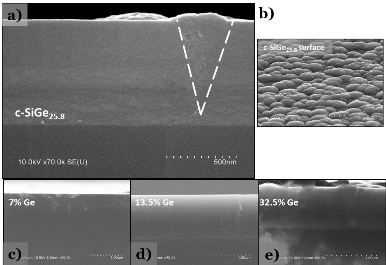
Figure 2.29 -SEM images of a)b) the cross-section and surface of SiGe 25.8 c)d)e) the cross-section for x = 7%, 13.5% and 32.5%.
