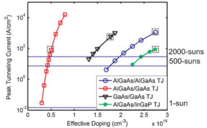
Figure 4.3- Peak tunnelling current as a function of the effective doping level for various TJ material combinations. (Simulation and experimental, from Wheeldon et al. 158 )
