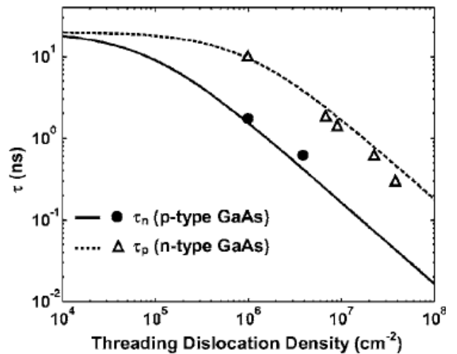
Figure 1.9 - minority carrier lifetime in GaAs as a function of threading dislocation density (Andre et al. 26 )
