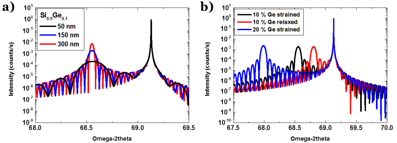
Figure 2.6 - Simulation with Leptos software of a) \text{Si}_{0.9}\text{Ge}_{0.1} layer with various thicknesses on a (100) Si substrate: the oscillation period and the peak intensity and FWHM are strongly dependent on the thickness b) Comparison of a strained \text{Si}_{0.8}\text{Ge}_{0.2} layer with a strained \text{Si}_{0.9}\text{Ge}_{0.1} and a relaxed one : the peak is shifted to the right when relaxed.
