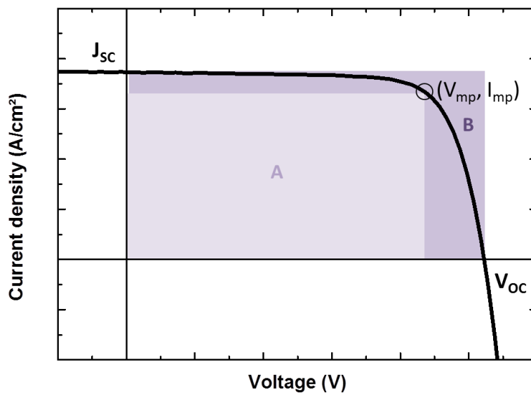
Figure 2.21 - J-V characteristics of a solar cell under illumination.
