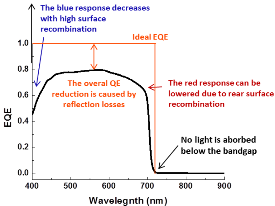
Figure 2.22 - Measured quantum efficiency of a AlGaAs solar cell, along with the main contributions responsible for possible EQE reductions.
