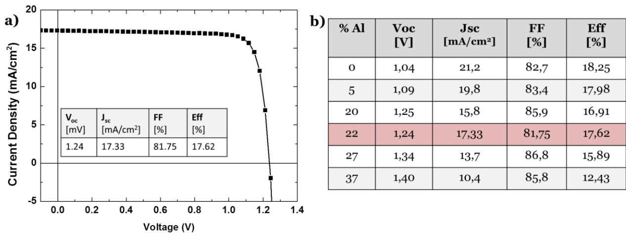
Figure 5.8 - a) J-V characteristics of the \text{Al}_{0.22}\text{Ga}_{0.78}\text{As} solar cell, b) detailed characteristics of the same cell as compared with results from Heckelmann et al. 207
