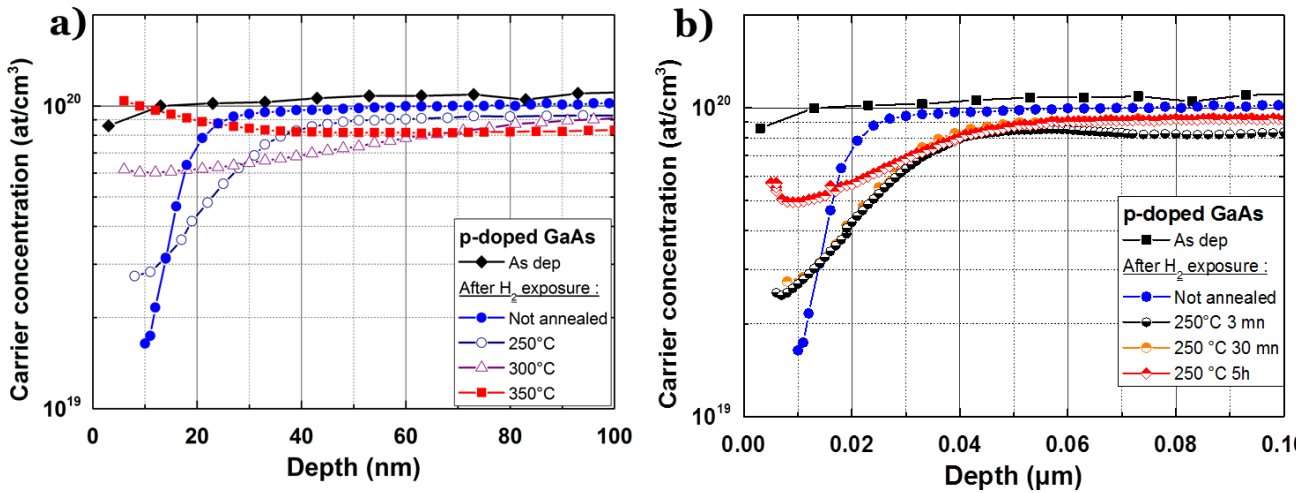
Figure 3.11 -ECV profiling of GaAs :C before H 2 exposure, after H 2 exposure and after a) 3-minutes annealing at various temperatures, b) annealing at 250 °C for various durations
