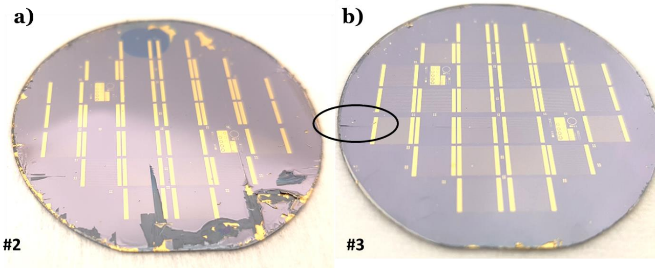
Figure 5.17 - a) Wafer #2 after metal lift-off: the active layer has been removed where the previous bubbles were present. b) Wafer #3 after metal lift-off: the previous cracks have been enlarged.
