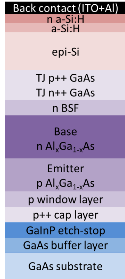
Figure 5.11 - Structure of the tandem device before bonding
