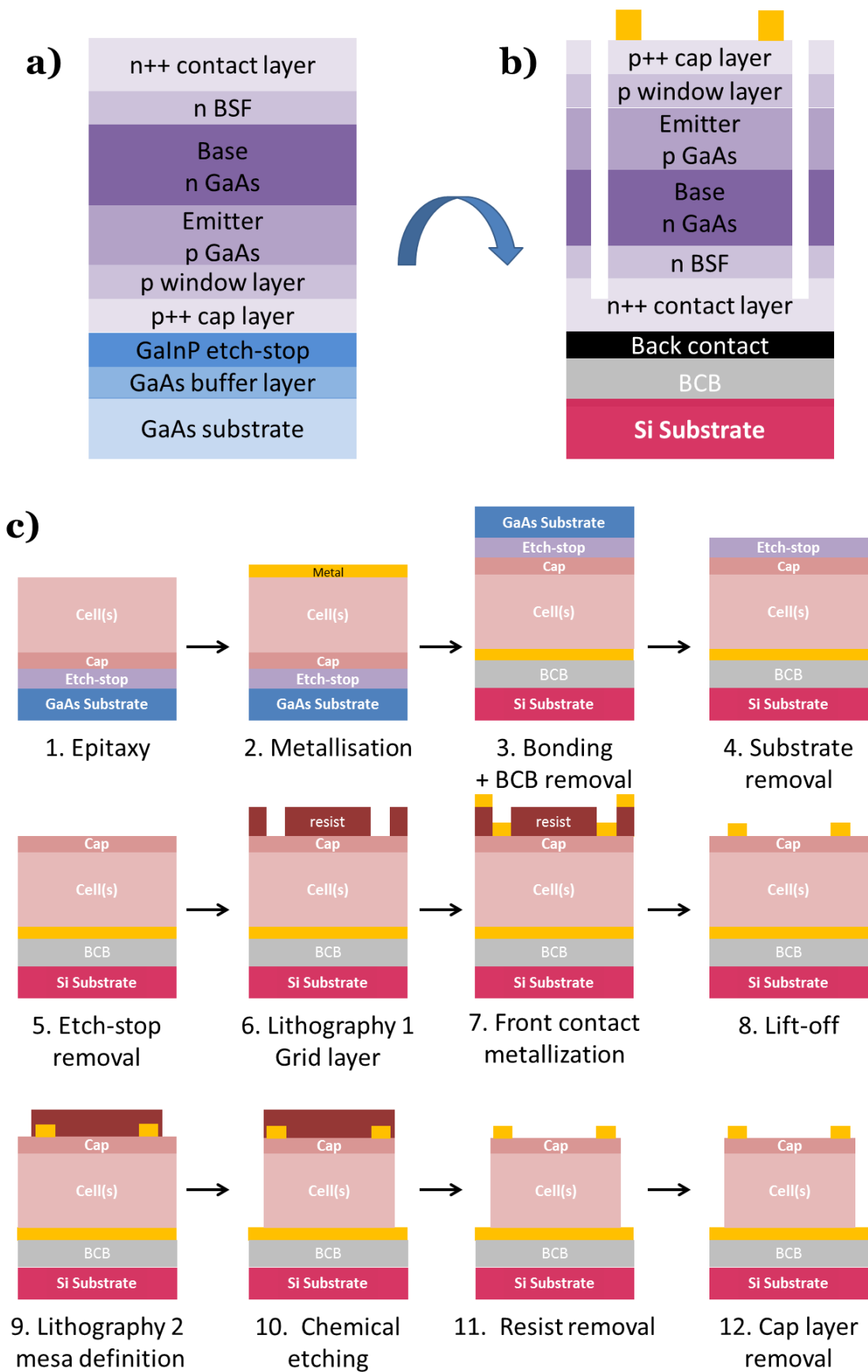
Figure 5.13 - Structure of a single GaAs (a) before and (b) after bonding an processing. c) Cross-section schematics of the process flow of inverted single or tandem solar cells
