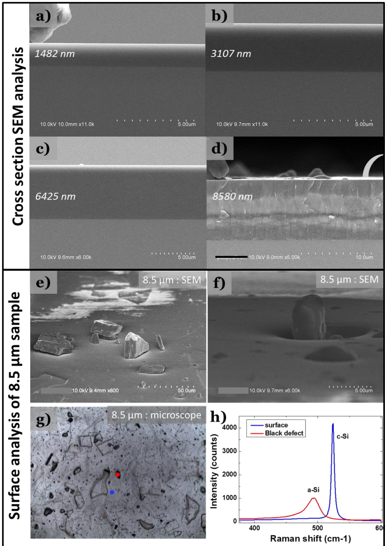
Figure 2.14 - a)b)c)d) cross-section SEM analysis of samples with thicknesses of 1.5 μm, 3.1 μm, 6.4 μm, 8.5 μm, along with the thickness measured thanks to this image. e)f) SEM images of the surface of the 8.5 μm sample, g)h) Raman spectroscopy spectra of the material on different surface spots : a defect, and the smooth surface of the film
