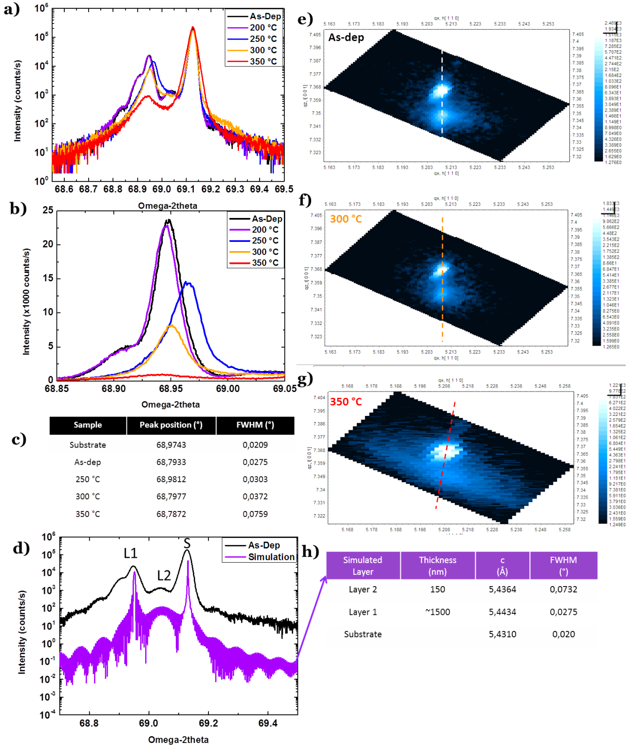
Figure 2.11 - \omega -2 \theta XRD scans of the samples before and after annealing at different temperatures a) in logarithmic scale, b) zoom on the film peak in a linear scale. c) Peak position and FWHM for each sample, d) Leptos simulation of the as-deposited sample. Reciprocal space mappings of {224} planes on e) as-dep sample, f) 300 °C annealed sample, g) 350 °C annealed sample. h) fit parameters obtained from simulation of as-deposited sample.
