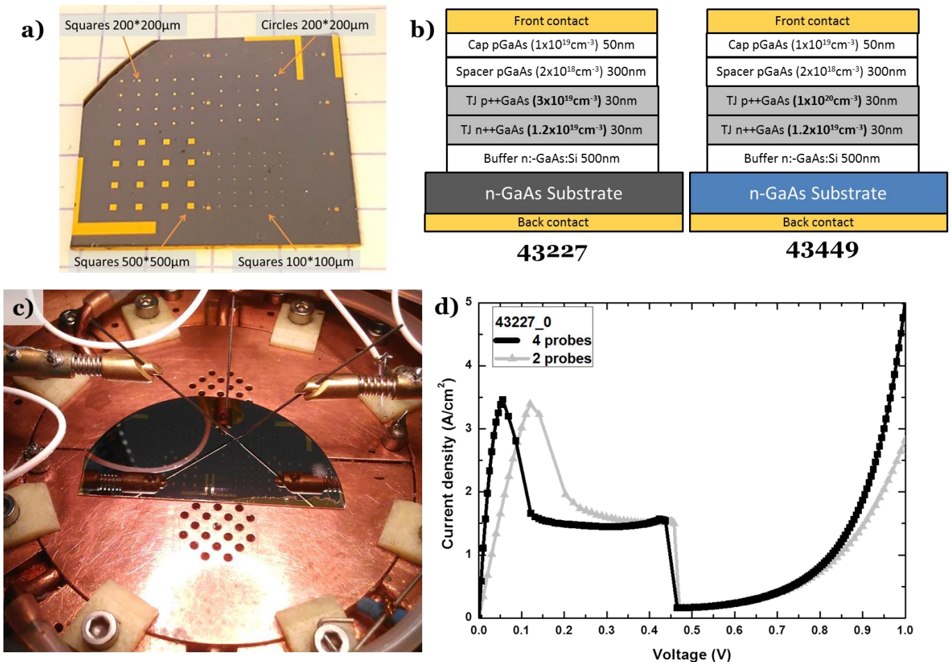
Figure 4.7- a) Picture of a tunnel junction after processing b) material and device of the two considered tunnel junctions, c) picture of the 4 probe characterization tool, d) comparison between 2-probe and 4-probe measurement
