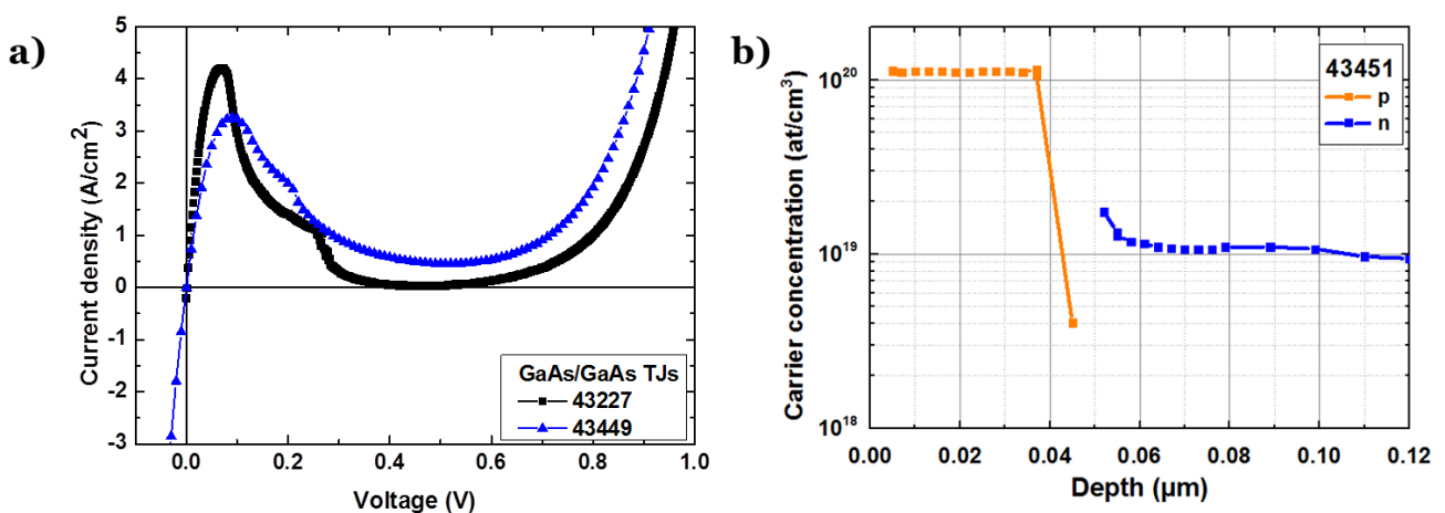
Figure 4.8 - a) J-V curves of GaAs/GaAs tunnel junctions, b) ECV measurement of a p-GaAs/n-GaAs structure
