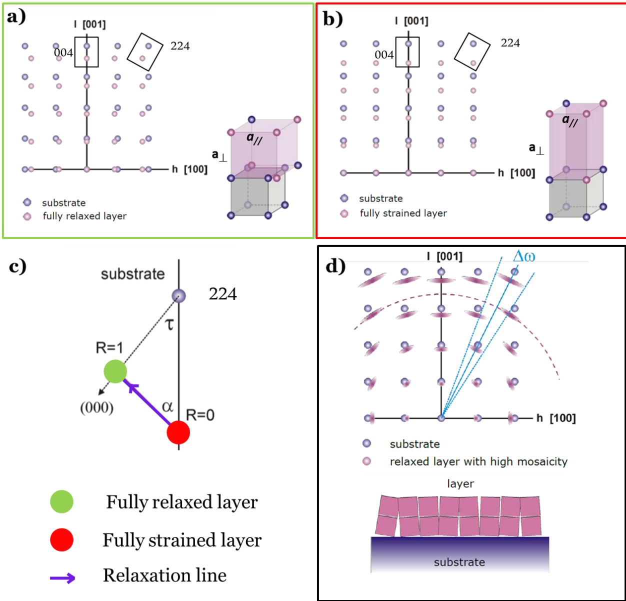
Figure 2.7 - Schematic of the reciprocal space of an hetero-epitaxy considering a substrate with lower lattice parameter than the layer. Rectangles show the area that corresponds to reciprocal space mapping (RSM) along \{004\} planes and \{224\} . a) In the relaxed configuration, b) in the fully strained configuration. c) The arrow represents the relaxation line for partly relaxed layer on along \{224\} planes. d) Reciprocal space schematics in case of relaxed layer with high mosaicity. (images: Bruker)
