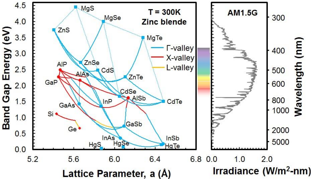
Figure 1.5 - Bandgap versus lattice constant at room temperature for various materials including Si, Ge, GaAs.
