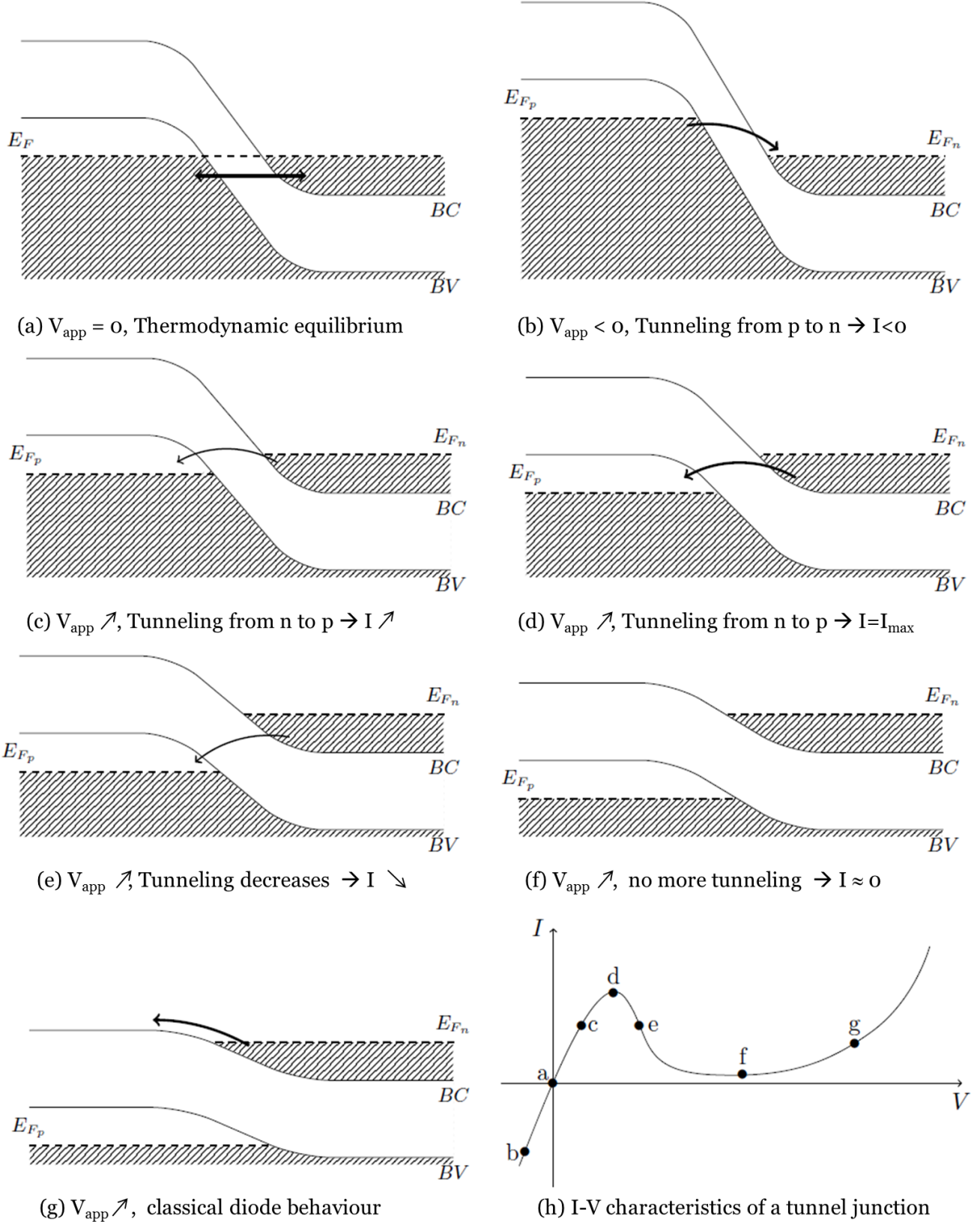
Figure 4.1 - Evolution of the band diagram of a tunnel junctions as a function of the applied Voltage (a to g), and corresponding I-V characteristics (h)
