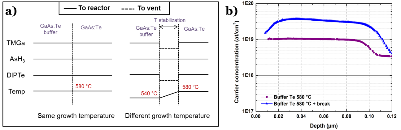
Figure 4.15 - a) Switching sequences of precursors in case of no temperature change (left) and with a temperature change (right) b) Doping profile of the upper doped layer grown directly after the buffer layer (purple circles), and grown after an annealing (blue triangles)
