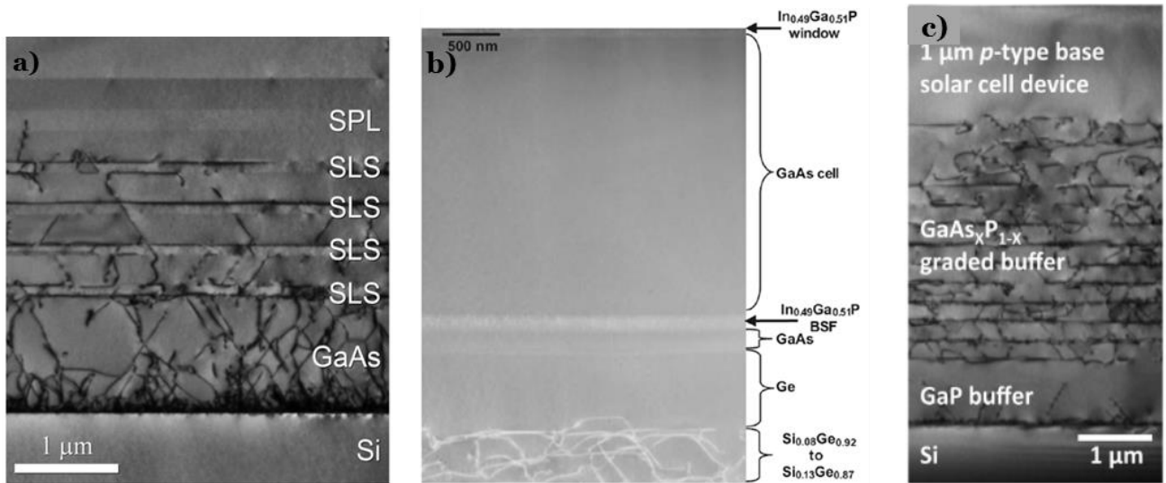
Figure 1.10 - TEM analysis of a) direct growth of GaAs on Si (Luxmoore et al. 30), b) SiGe graded layers (Andre et al. 37) (c) GaP buffer layer (Lang et al. 39)
