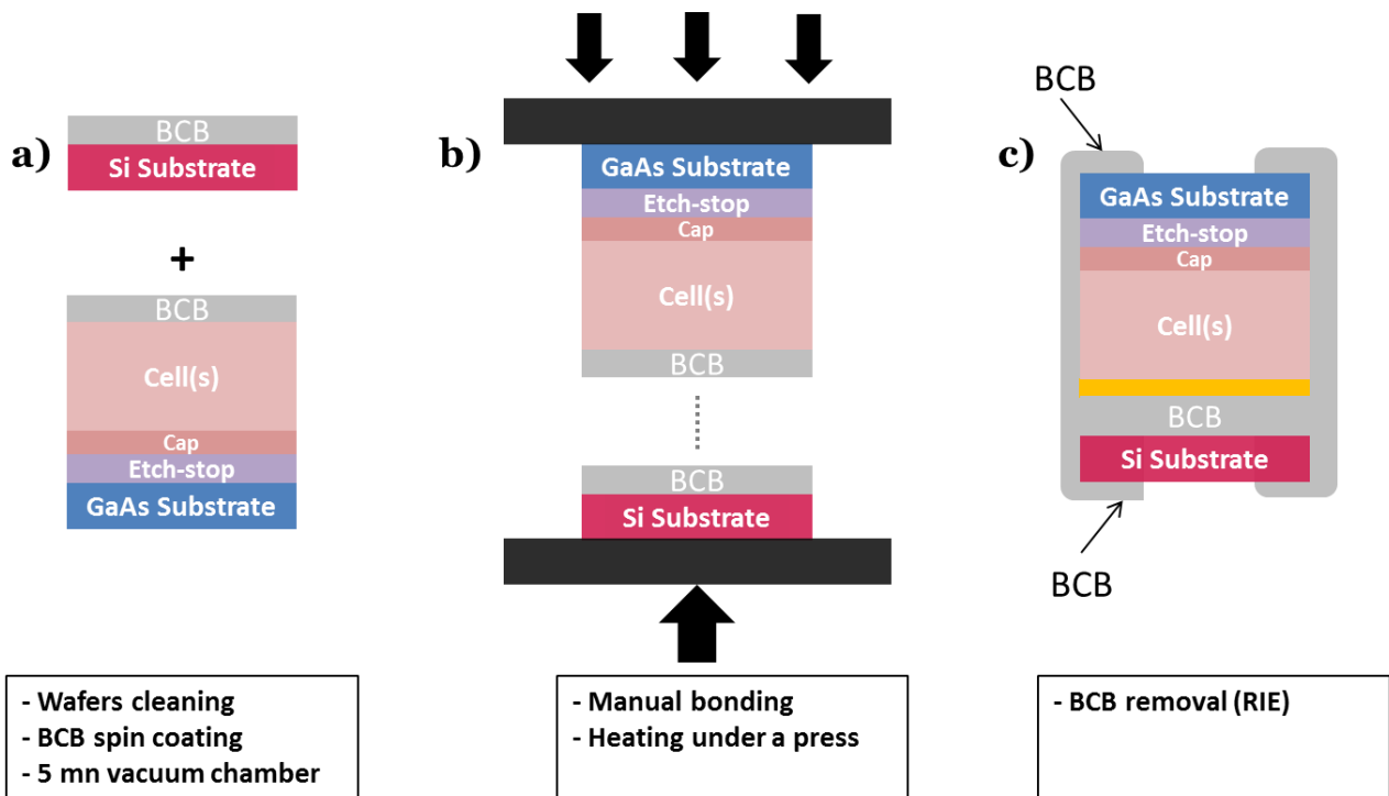
Figure 5.12- Schematics of the main technological steps of bonding with BCB
