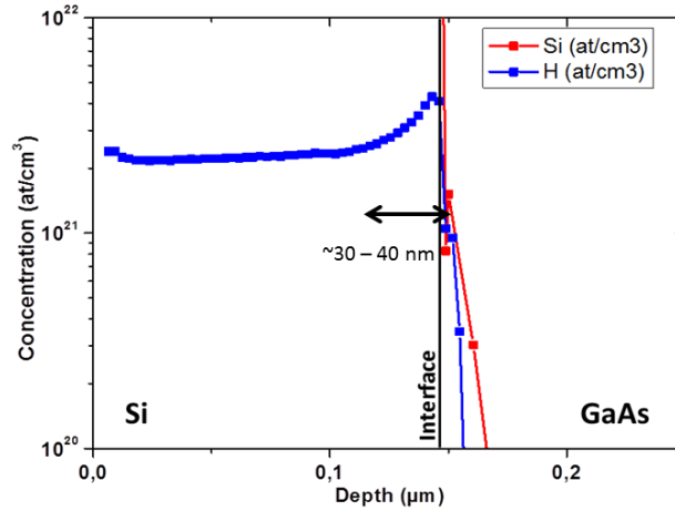
Figure 3.6 - SIMS analysis of a 150 nm-thick epi-Si layer on GaAs.
