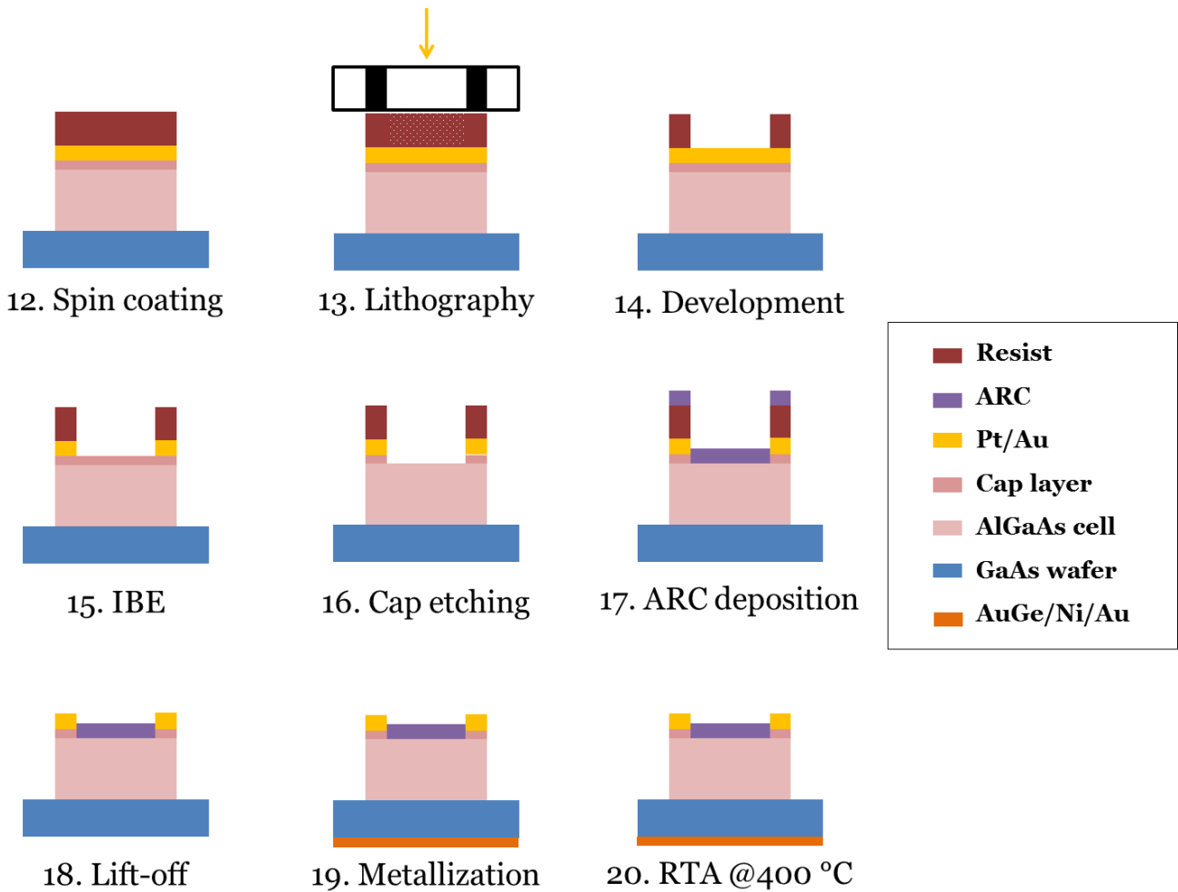
Figure 5.7 - Cross section schematics of the solar cell process flow: grid definition and ARC deposition
