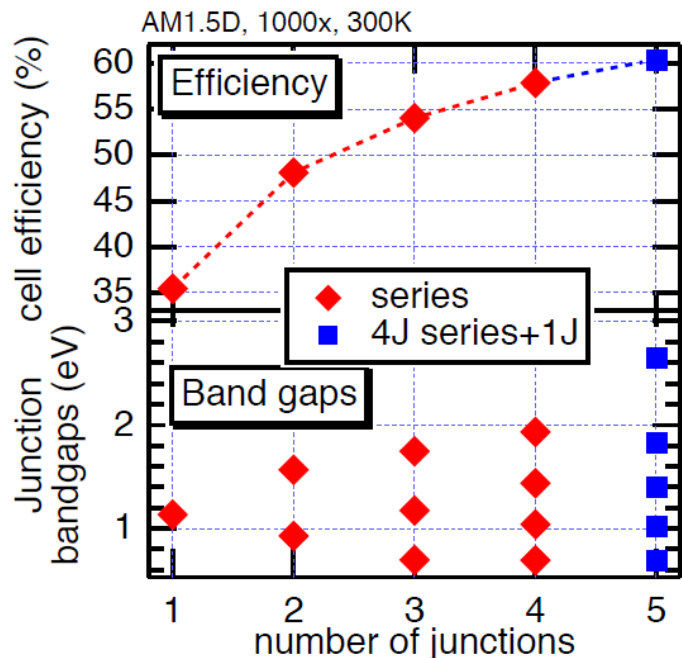
Figure 1.4 - Theoretical maximum efficiency of a multijunction as a function of the number of junctions, along with the corresponding bandgaps (NREL) 11
