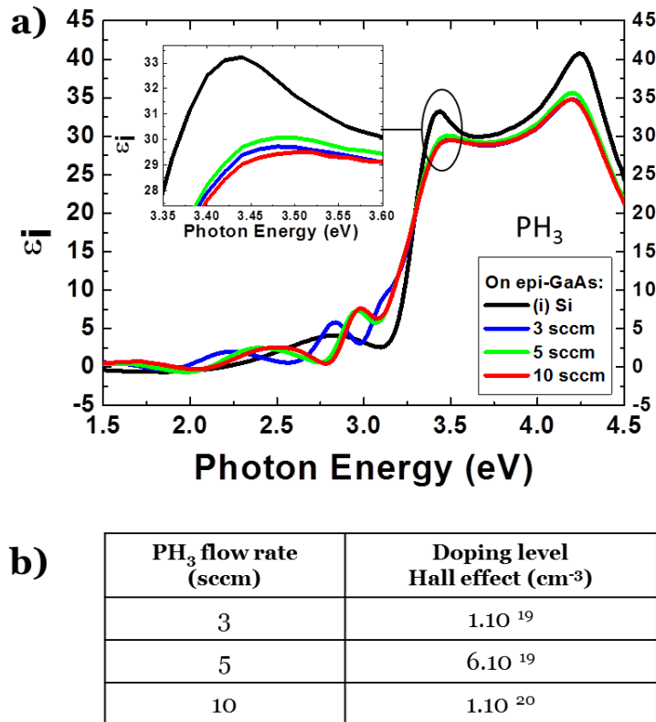
Figure 4.23 - Ellipsometric spectra of silicon thin films grown on epi-GaAs with various PH 3 flow rates
