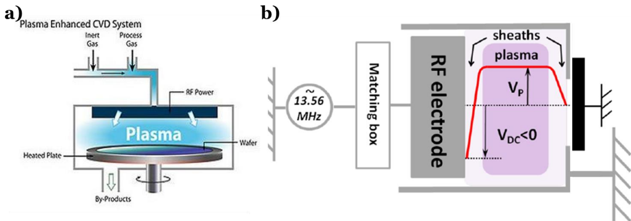
Figure 2.1 - a) Schematics of a PECVD reactor b) Schematic of the potential distribution in a RF discharge where the substrate is grounded and the RF voltage applied to the RF electrode
