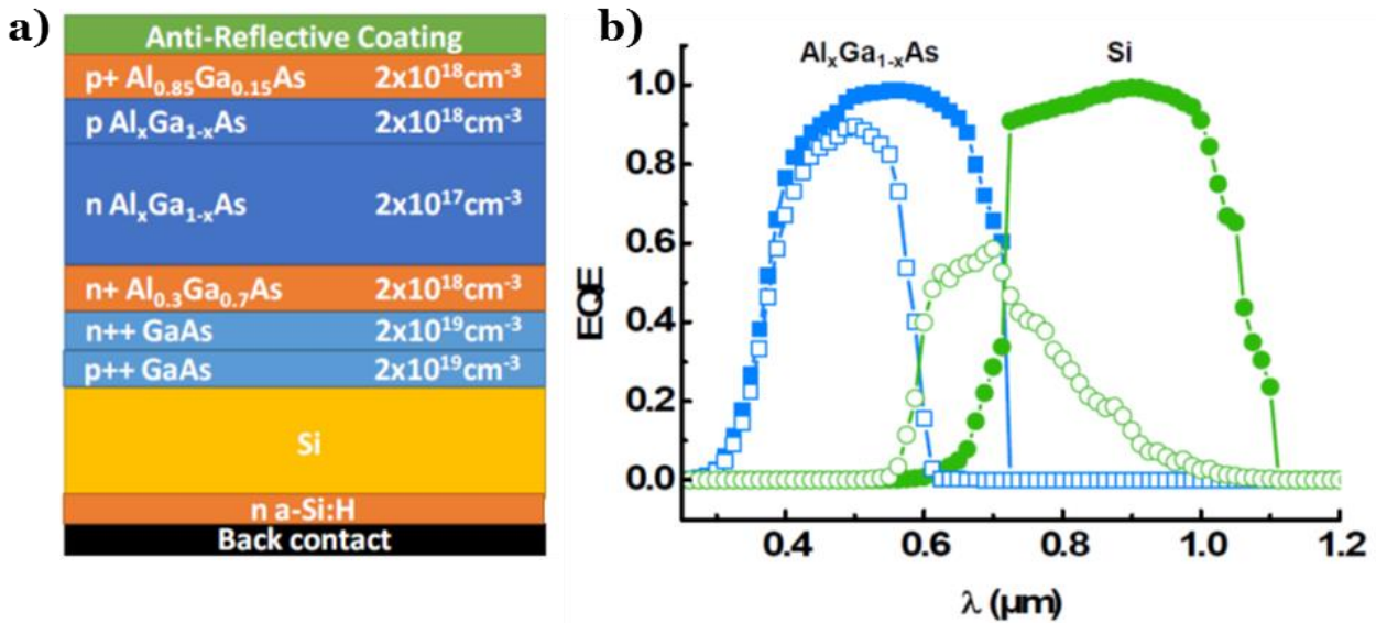
Figure 1.16 - a) Details of the simulated tandem solar cell b) External Quantum Efficiency (EQE) of current-matched AlGaAs/Si tandem solar cell with thick Si (full symbols) and thin Si (open symbols).
