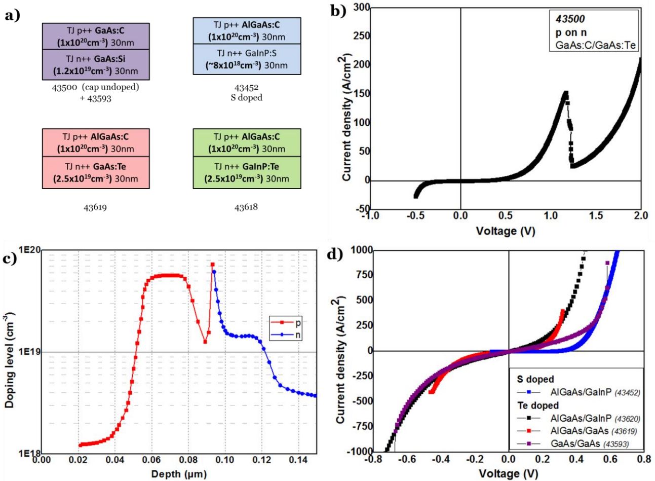
Figure 4.21 - a) structure of 4 tunnel junctions b) J-V characteristics of a p on n GaAs/GaAs tunnel junction with lowly doped cap layer. c) ECV measurement on the same GaAs/GaAs TJ, d) J-V characteristics of 4 different p on n tunnel junctions with highly doped cap layer
