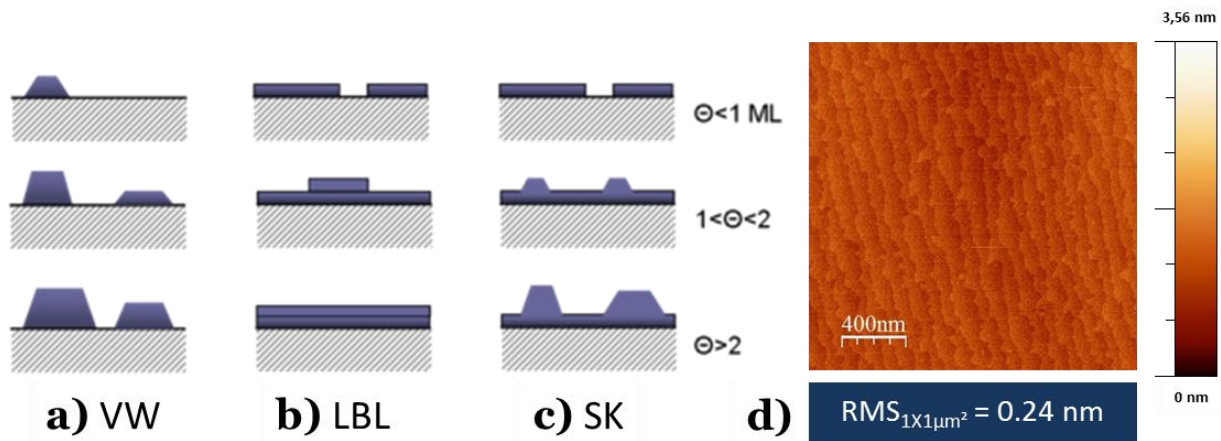
Figure 2.3 - Illustration of the three main growth modes: a) Volmer-Weber mode (VW) b) Frank-van der Merwe mode (Layer-By-Layer) c) Stranski-Krastanov (SK) d) Atomic Force Microscopy mapping of the surface of an GaAs layer grown by MOVPE
