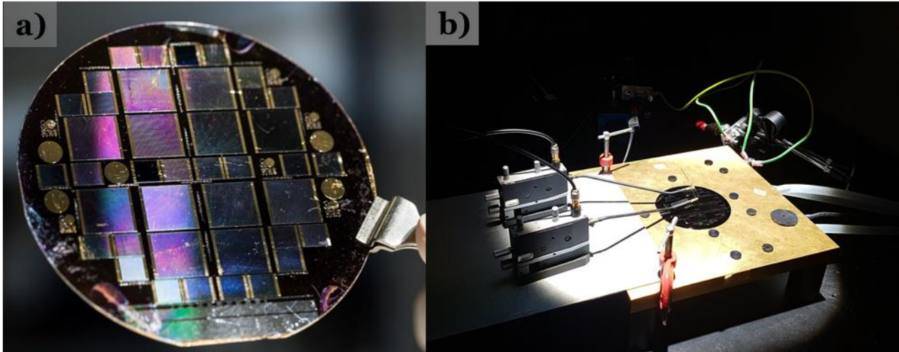
Figure 5.9 - a) Picture of the wafer after processing, b) picture of the measurement under AM1.5G spectrum
