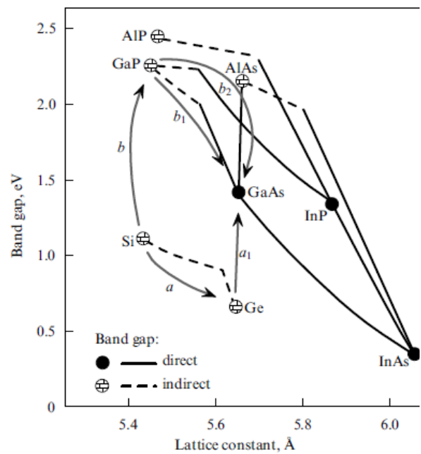
Figure 1.11 - Bandgap versus lattice constant for Si, Ge, and III-V compounds. Arrows indicate the possible pathways for integrating III-V on Si.
