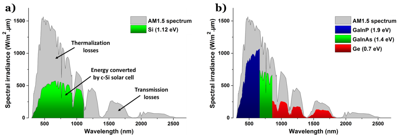
Figure 1.3- AM1.5G spectrum and the fraction theoretically converted by a) a Si solar cell, b) a triple junction GaInP/GaInAs/Ge (from ref 9 )
