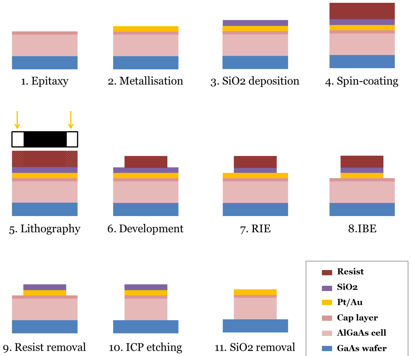
Figure 5.6 - Cross section schematics of the solar cell process flow detailing the 11 first steps required for the mesa etching
