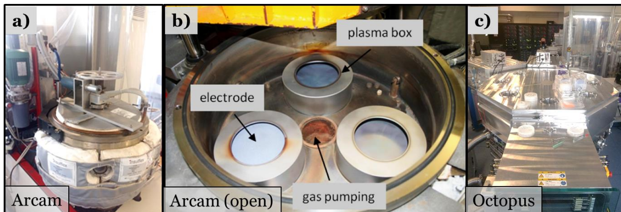
Figure 2.2 - a) Picture of Arcam reactor, b) picture of the inside of Arcam reactor with the three separated plasma boxes. c) picture of the Octopus reactor from IndeoTec.
