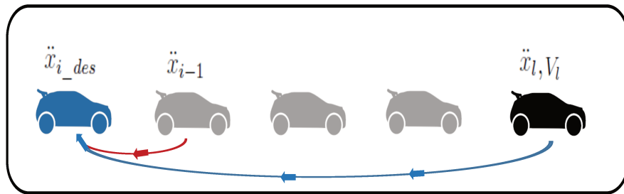
Figure 2.9: Platoon's communication information flow, a broadcasted CAM periodic messages is required to pass the leader vehicle speed and acceleration together with any DENMs, where a point-to-point link is required to pass the proceeding vehicle acceleration for string stability desired acceleration by the i th vehicle CAMs
