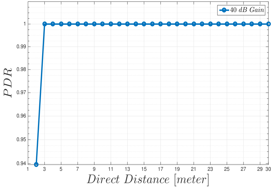
Figure 4.28: Packet Delivery Ratio (PDR) of the VLC platform for 40 dB gain.
