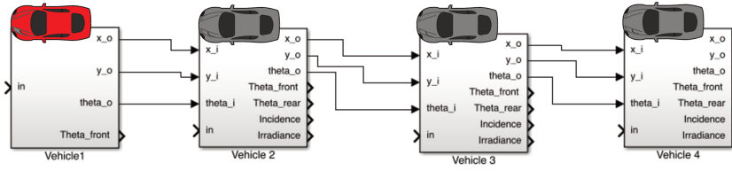
Figure 3.10: VLC-based Platoon SIMULINK model for four vehicles, each vehicle consist of longitudinal controller, lateral controller, VLC model for path loss calculation and an a FOV enhancement controller.
