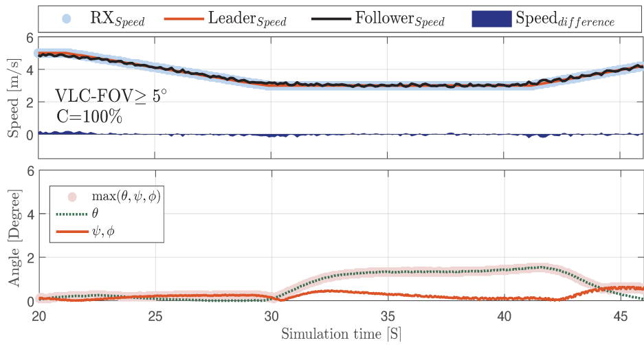
Figure 5.9: Simulation results of Straight driving platoon scenario. laser based detection confidence C=100\% .
