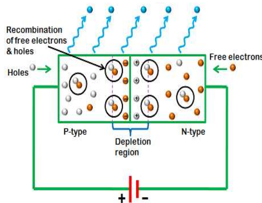
Figure 4.5: The basic structure of an LED
