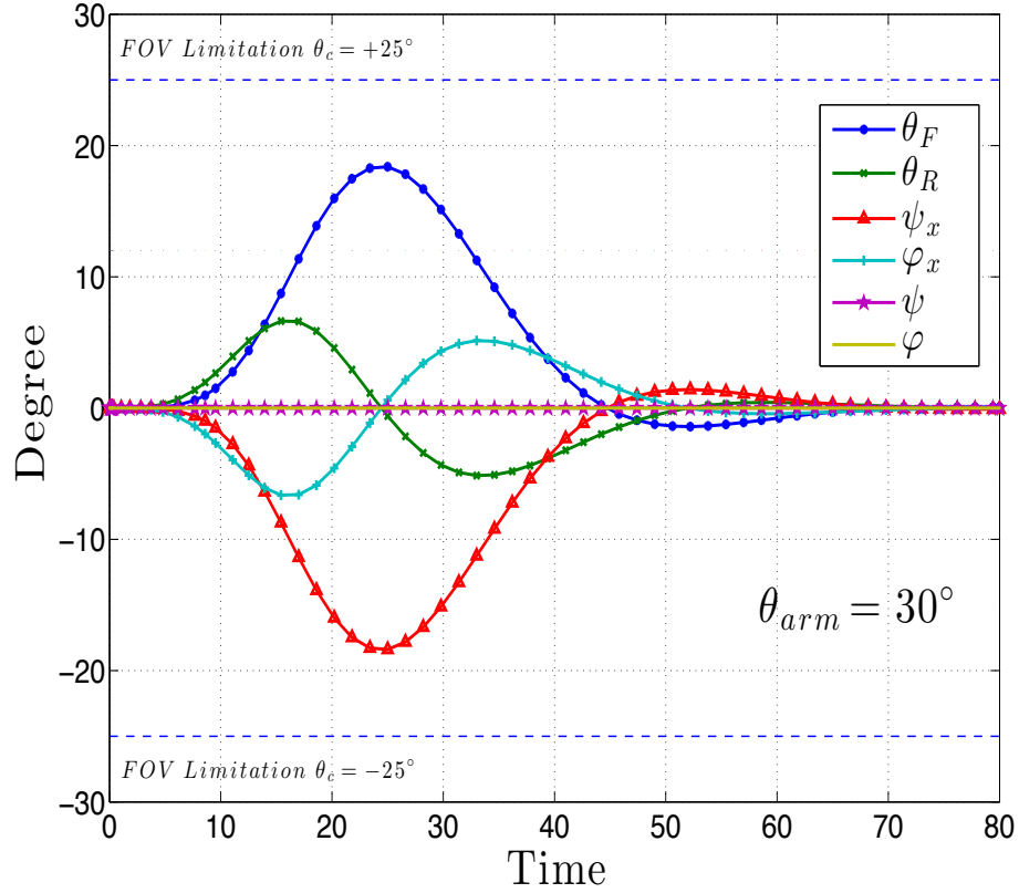
Figure 3.11: The angular variation of the vehicle front ( \theta_F ), vehicle rear ( \theta_R ), incidence compensation angle ( \psi_x ), irradiance compensation angle ( \varphi_x ), incidence angle ( \psi ) and irradiance angle ( \varphi ) between every two members in the VLC-based platoon and following trajectory 2 in Figure 3.12.
