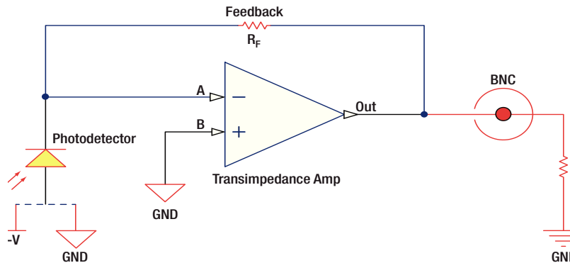
Figure 4.16: PDA10A device from THORLABS, Photodetector combined with a transimpedance amplifier.
