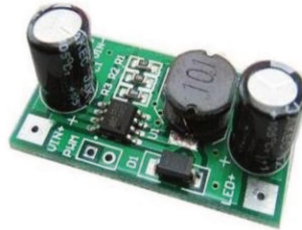
Figure 4.10: DC to DC Step-down 700mA current driver
