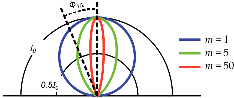
Figure 4.6: LED lambertian emission pattern and the FOV represented by the angle \phi and the index m
