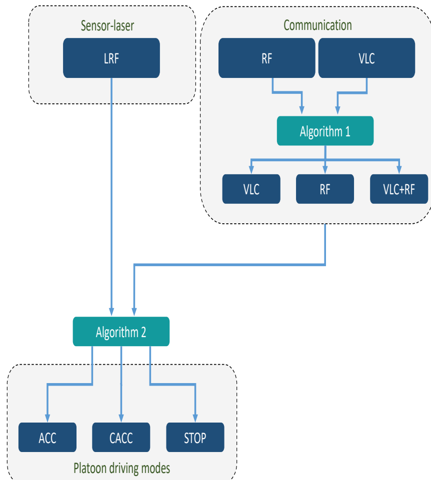
Figure 5.2: General flow chart of the two main handover algorithms used to enable platoon control using LRF, VLC and RF technologies.
