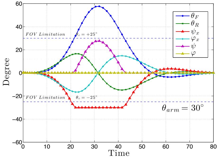
Figure 3.12: The angular variation of the vehicle front ( \theta_F ), vehicle rear ( \theta_R ), incidence compensation angle ( \psi_x ), irradiance compensation angle ( \varphi_x ), incidence angle ( \psi ) and irradiance angle ( \varphi ) between two members in the VLC-based platoon following trajectory 3 in Figure 3.12.
