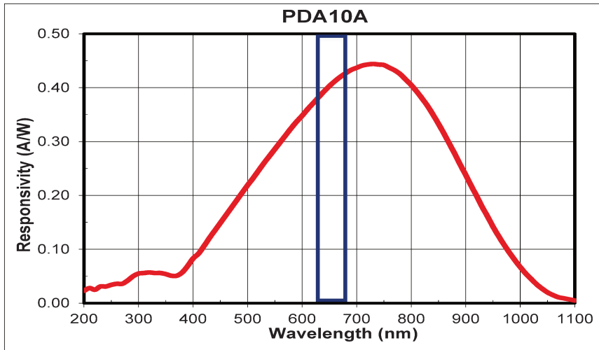
Figure 4.13: Response curve of the PDA10A Photo detector
