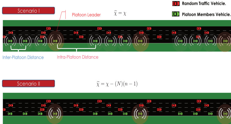
Figure 5.17: Four lanes simulation scenarios in NS3: Scenario I enables RF communication broadcast for all vehicles. Scenario II enables RF broadcast for all vehicles except platoon followers, assuming VLC is used as IVC between platoon members.
