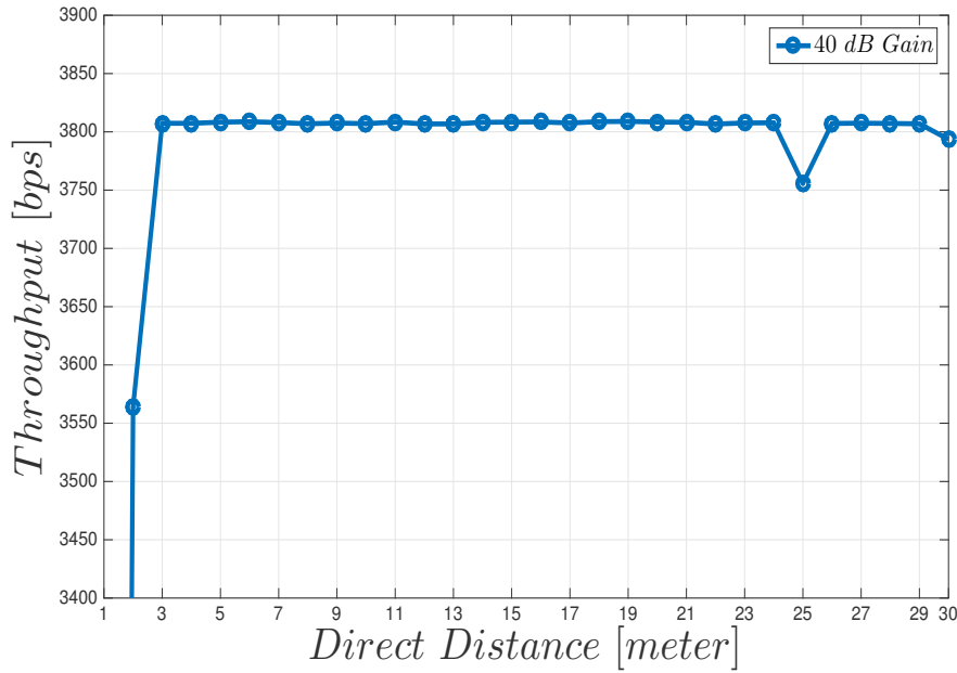
Figure 4.30: The throughput performance of the VLC platform for 40 dB gain.
