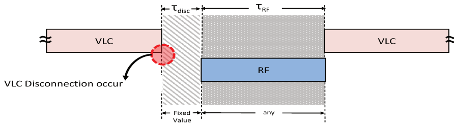
Figure 5.16: D-VHO switching stages between VLC and RF.
