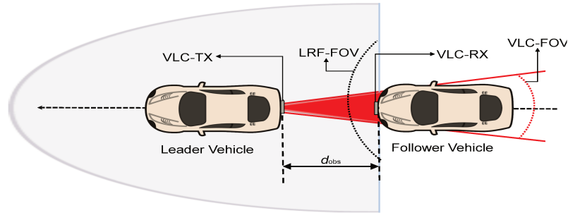
Figure 5.4: LRF-VLC system configuration for a platoon of autonomous vehicles.
