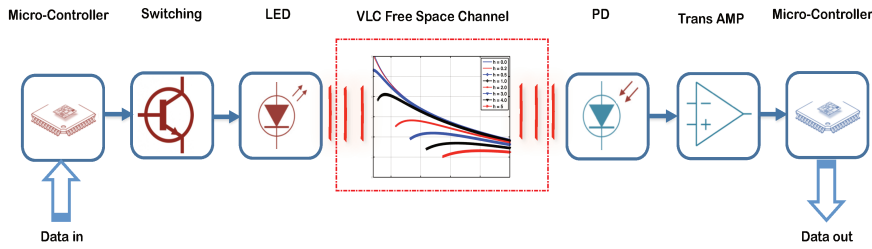
Figure 3.1: General illustration of the VLC concept.
