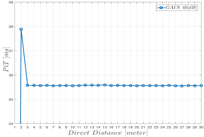
Figure 4.29: The packet inter-reception time (PiT) performance of the VLC platform for 40 dB gain.
