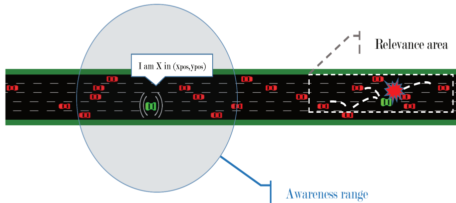
Figure 2.2: CAMs and DENMs delivery in IEEE 802.11p, messages are regionally broadcast through V2V communication
