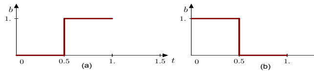
Figure 4.18: (a). Manchester bit representation for digit 1 (b). Manchester bit representation for digit 0.
