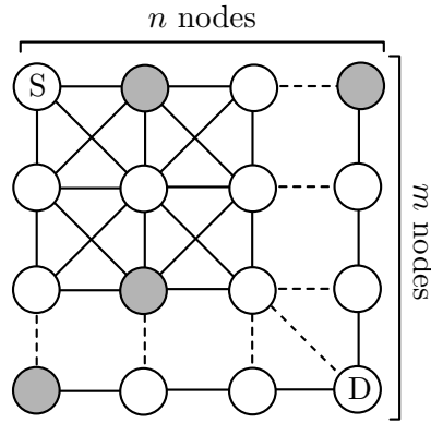
Figure 4.5: Grid topology with n \times m nodes
