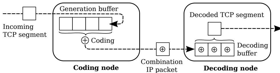
Figure 5.1: TCP over pipeline coding
