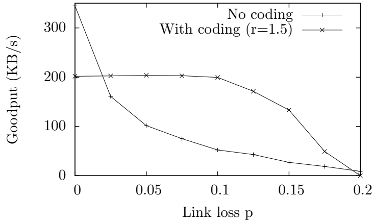
Figure 6.5: Application goodput for MPTCP on two links given loss rate p with 100ms RTT (generation size 8)
