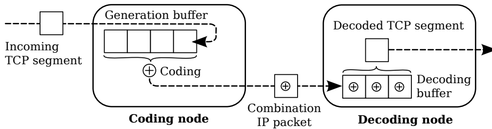
Figure 6.4: Pipeline coding as implemented in ns-3 nodes
