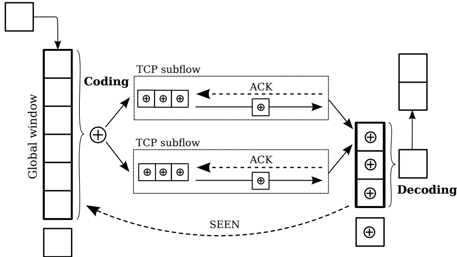
Figure 7.5: Overview of the coding/decoding principle with two subflows
