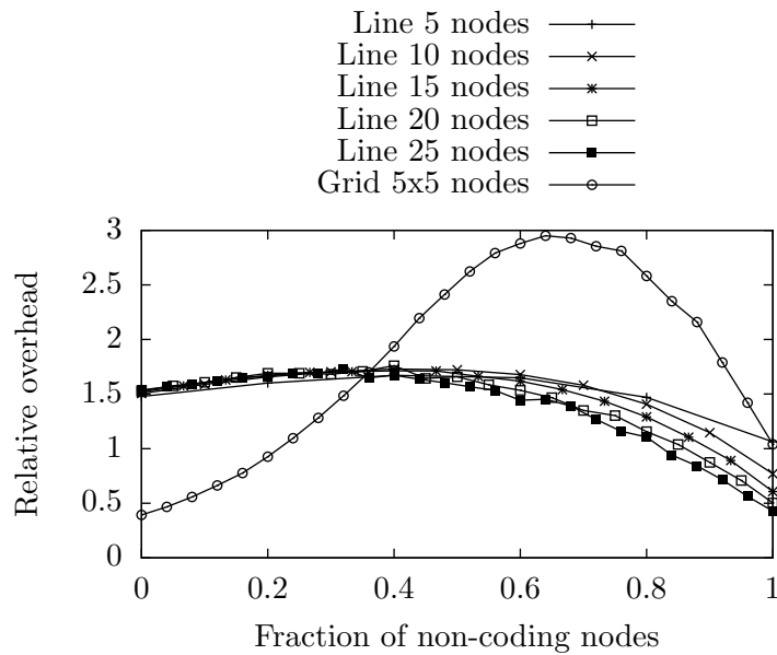
Figure 3.12: Network overhead in different topologies given the fraction of non-coding nodes
