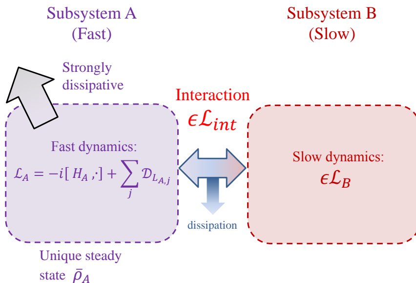
Figure 3.1: We consider a fast system A with stable dynamics \mathcal{L}_A converging towards a unique steady state \bar{\rho}_A . It is coupled through the super-operator \epsilon\mathcal{L}_{int} to the slow subsystem B with internal dynamics \epsilon\mathcal{L}_B . We investigate the perturbative effect of this coupling on the system of interest B by performing adiabatic elimination of the fast variables associated to the subsystem A . We particularly pay attention to the standard Hamiltonian and cascaded coupling in the next sections.
