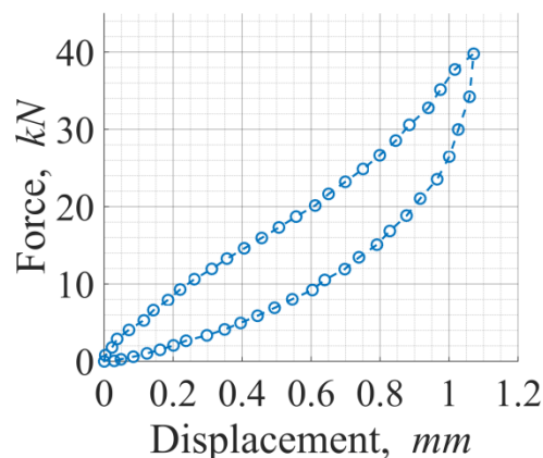
Figure 2.22: Force vs Displacement curve obtained during QS compression experiment of a rail pad in the second cycle
