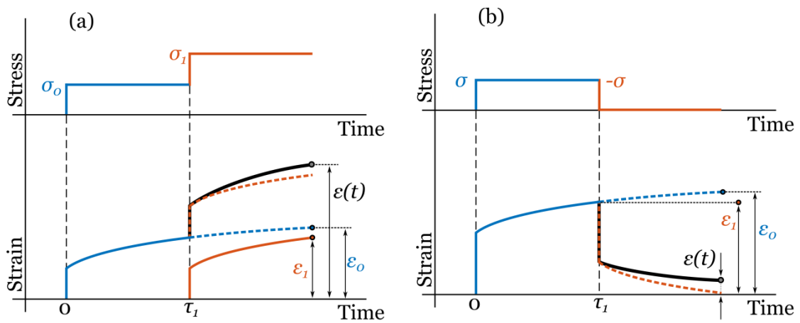
Figure 1.6: Illustration of the two-step (a) loading and (b) loading-unloading experiment (from [17])
