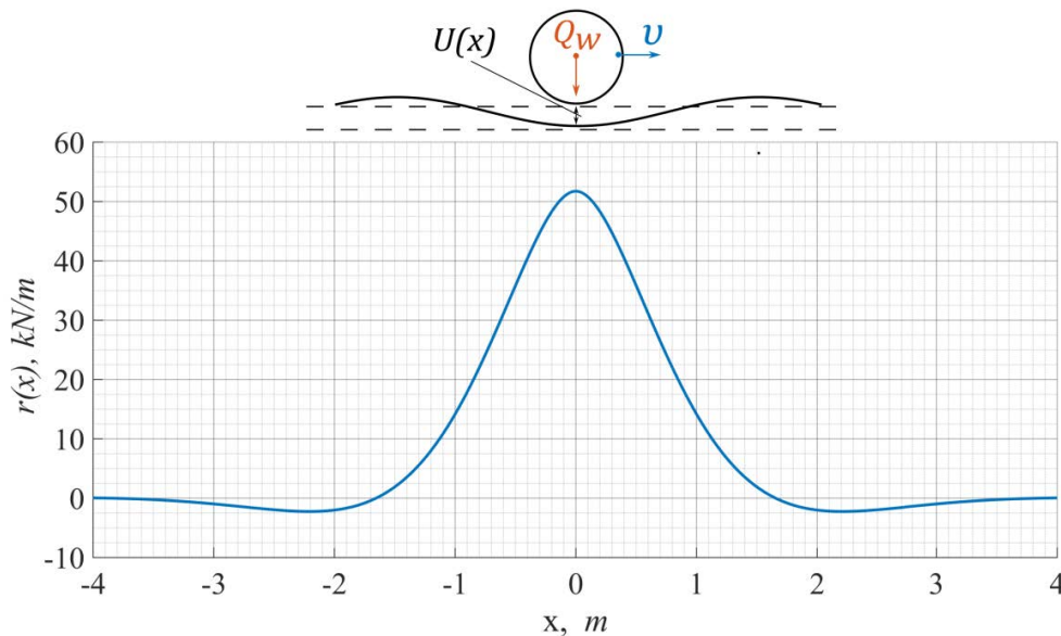
Figure 2.11: Dependence of distributed reaction force r(x,t) on distance x from a wheel load moving with the speed v = 87.8 m/s
