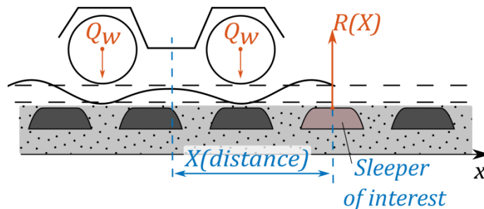
Figure 2.14: Reaction force of a sleeper of interest depends on a distance between centres of this sleeper and approaching bogie
