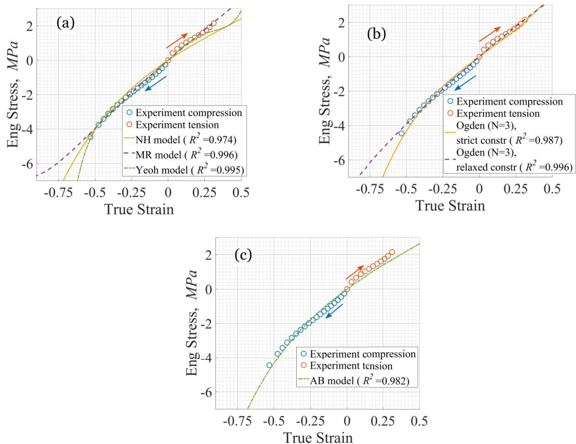
Figure 2.20: Fitting of different hyperelastic models to experimental data: (a) Neo-Hookean, Mooney-Rivlin and Yeoh models; (b) Ogden models with strict and relaxed condition (Eq. 2.11); (c) Arruda-Boyce model
