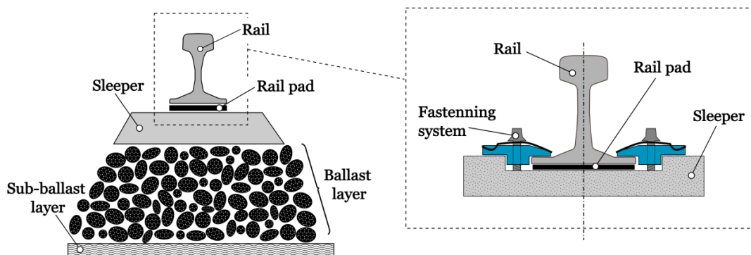
Figure 2.1: Rail pad location on the ballasted railway track
