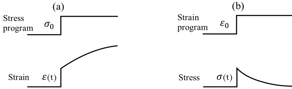
Figure 1.4: Two load programs to represent (a) creep effect at applied constant stress and (b) relaxation effect at applied constant strain
