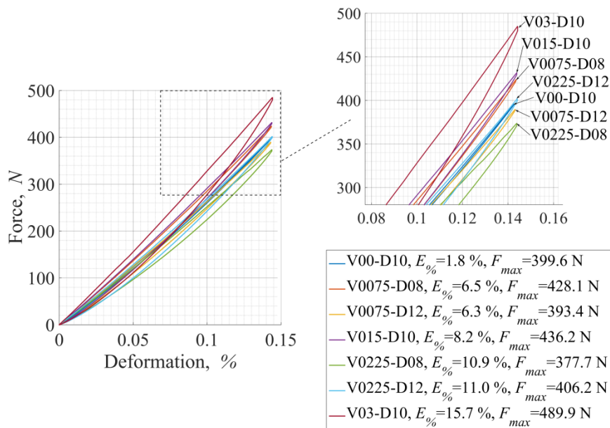
Figure 3.13: Force vs Macroscopic strain curves obtained during experimental investigation of VM specimens subjected to compression load in the Y-direction
