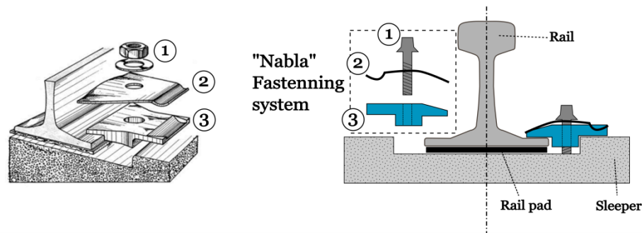
Figure 2.8: Construction of a fastening system “Nabla” [1]
