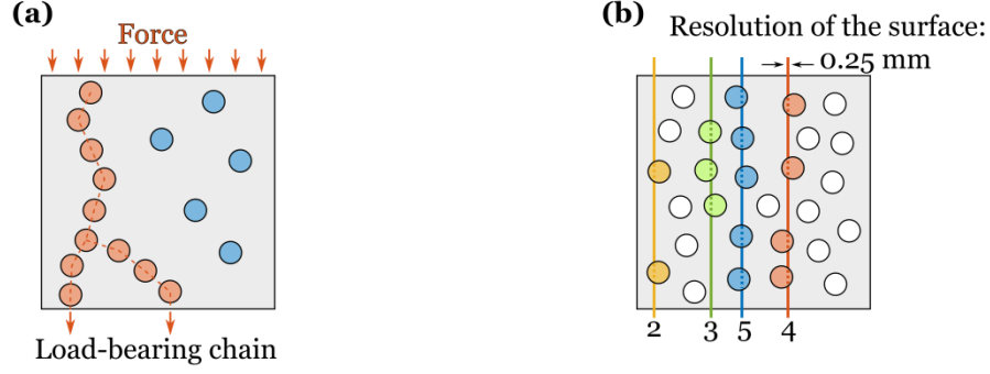
Figure 3.18: Schematic representation of a load-bearing chain in a composite material (a); construction of a surface of projections (b)
