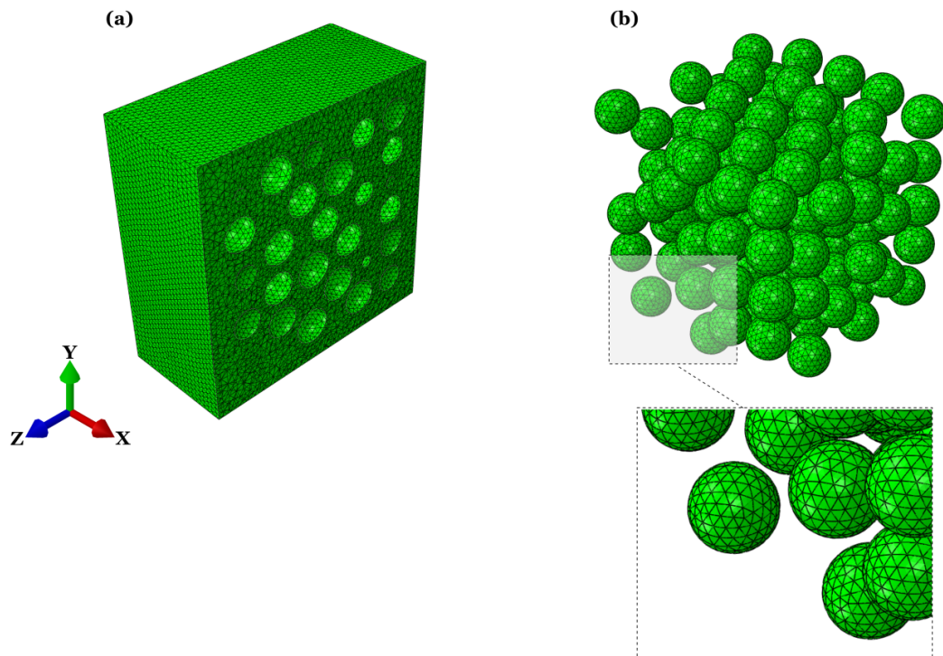
Figure 3.23: Meshing of the matrix (a) and the inclusions skeleton (b) of VO 3 -D10 specimen
