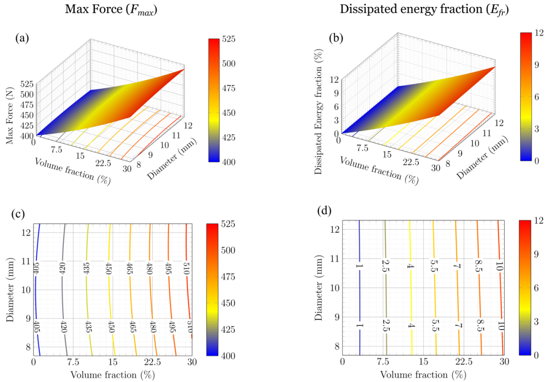
Figure 3.26: F_{max} (a) and E_{fr} (b) output parameters obtained during FE simulations as functions of inclusions' volume fraction and diameter
