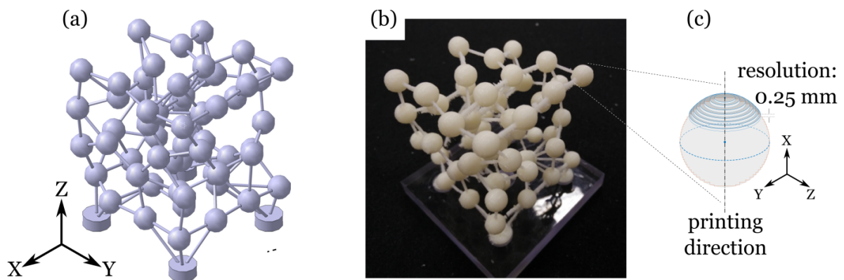
Figure 3.7: Inclusions skeleton of the specimen V7.5-Do8: numerical (a) and printed using ABS plastic material (b). Stair-like surface of a 3D printed geometry (c)
