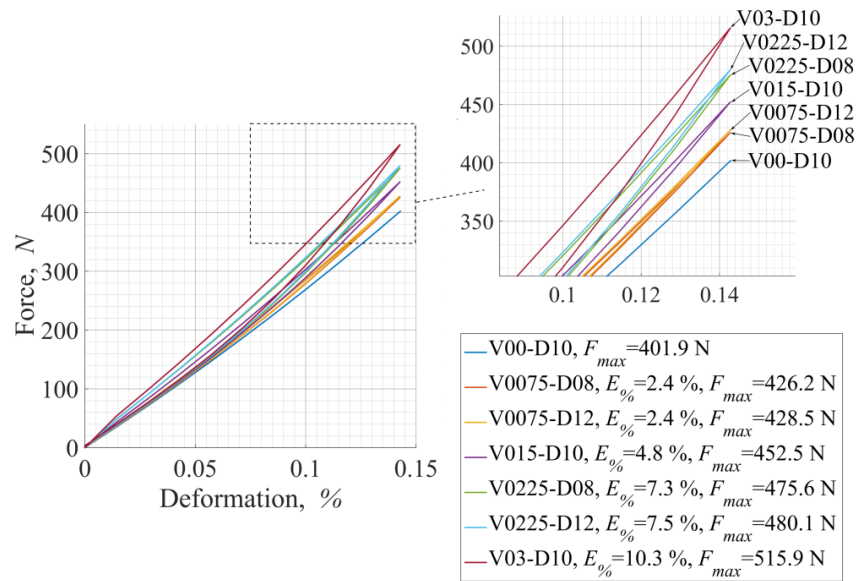
Figure 3.27: Force vs Macroscopic strain curves obtained during FE simulations of VM specimens subjected to compression load in the Y-direction
