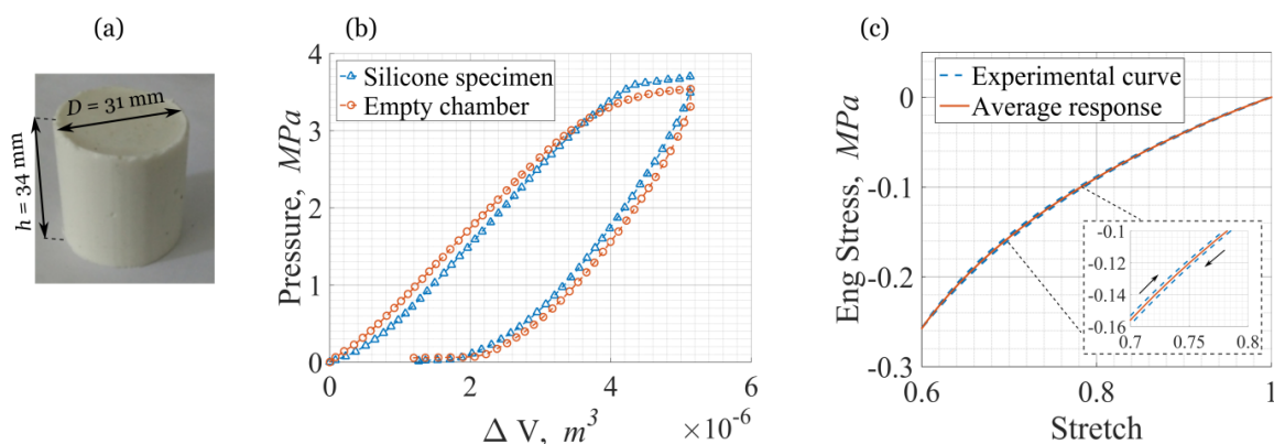
Figure 3.9: Experimental investigation of the mechanical behaviour of silicone material: (a) Cylindrical specimen; (b) Pressure dependences on change in volume during hydrostatic compression experiment; (c) Stress vs Stretch curve obtained during QS compression experiment
