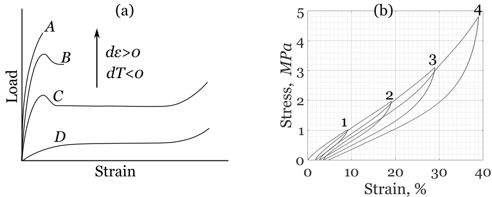
Figure 1.2: (a) Typical load-elongation curves for a polymer at different temperatures/strain rates[17]; (b) Stress-strain curves illustrating Mullins softening effect (numbers indicate a cycle number and location of maximum load for this cycle)
