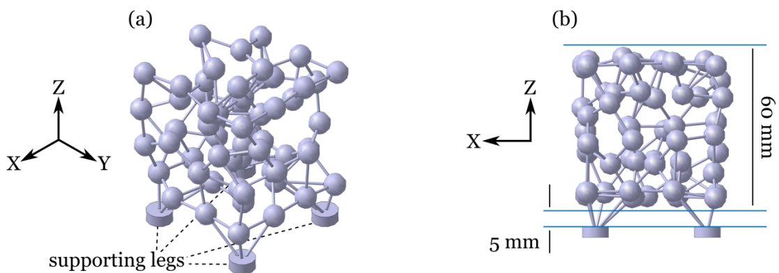
Figure 3.6: Inclusions skeleton designed for 3D printing of the specimen V0075-Do8 reinforced by links: (a) isometric view, (b) XZ-plane view
