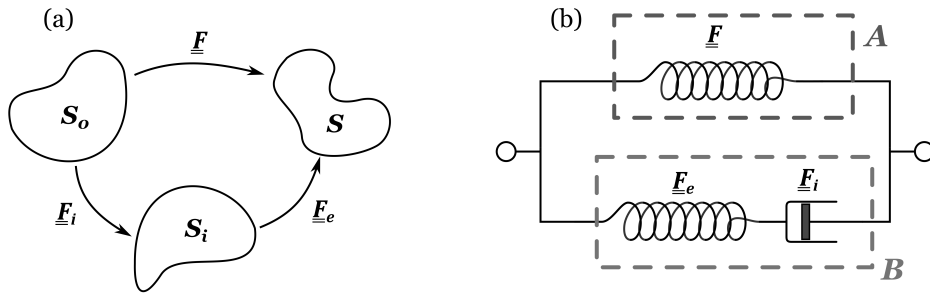
Figure 1.11: Schematic representation of deformation split in IV-model approach
