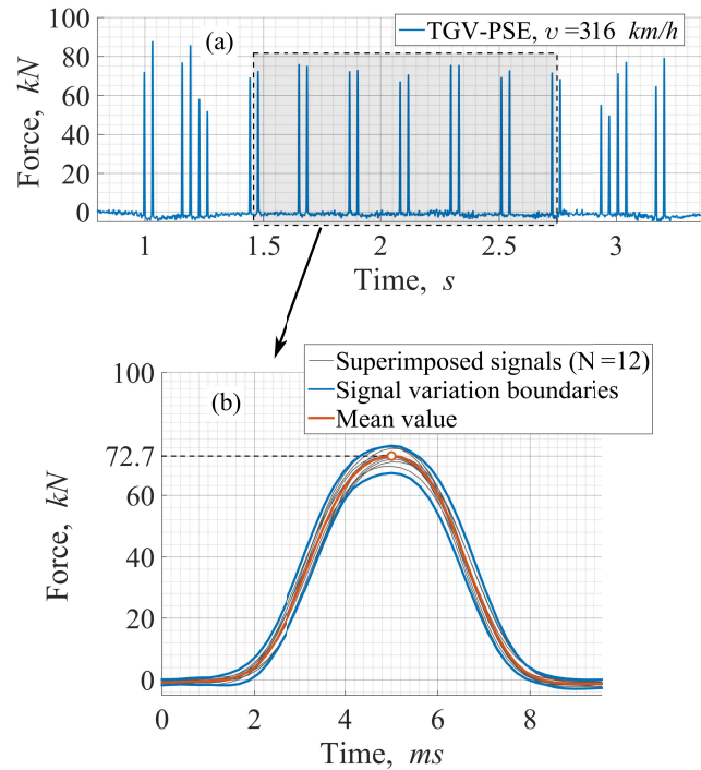
Figure 2.4: The common wheel force signal caused by passing of a TGV-PSE train plotted in a time domain (a); superimposed peaks of a wheel force signal (b)
