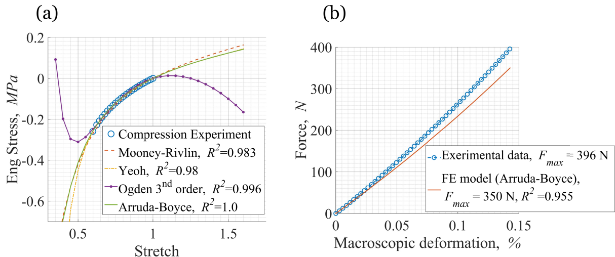
Figure 3.21: (a) Fitting of different hyperelastic models to QS compression data of a cylindrical silicone specimen; (b) prediction by FE simulation of the mechanical behaviour of V00-D10 specimen using previously fitted Arruda-Boyce hyperelastic model
