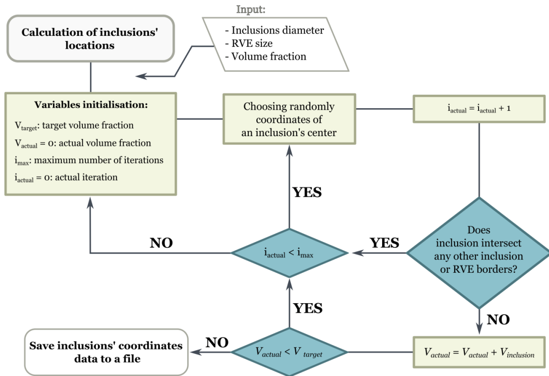
Figure 3.4: Scheme representing algorithm of inclusions locations calculation
