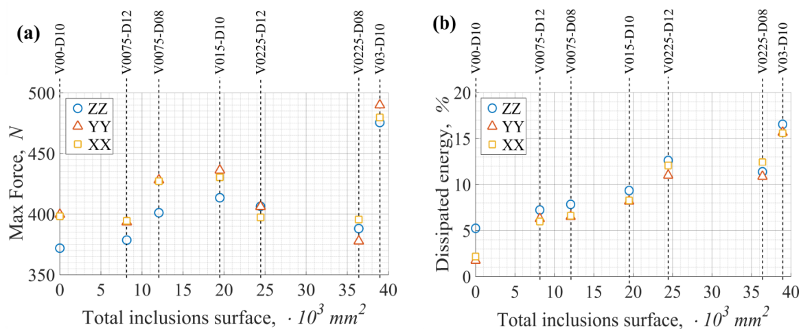
Figure 3.15: Dependences of F_{max} (a) and E_{\%} (b) on total inclusions' surface area
