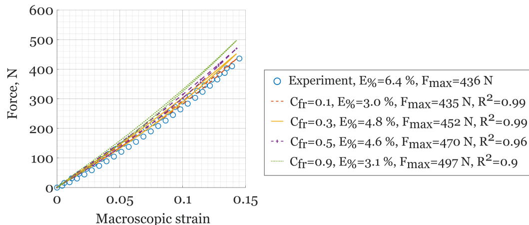
Figure 3 25: Influence of a friction coefficient value on the mechanical response of the FE model of V15-D10 specimen
