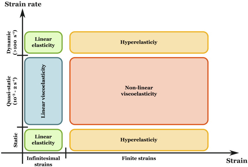
Figure 1.12: Applicability domains for constitutive approaches, appropriate for the modelling of the mechanical behaviour of elastomers (from [44])
