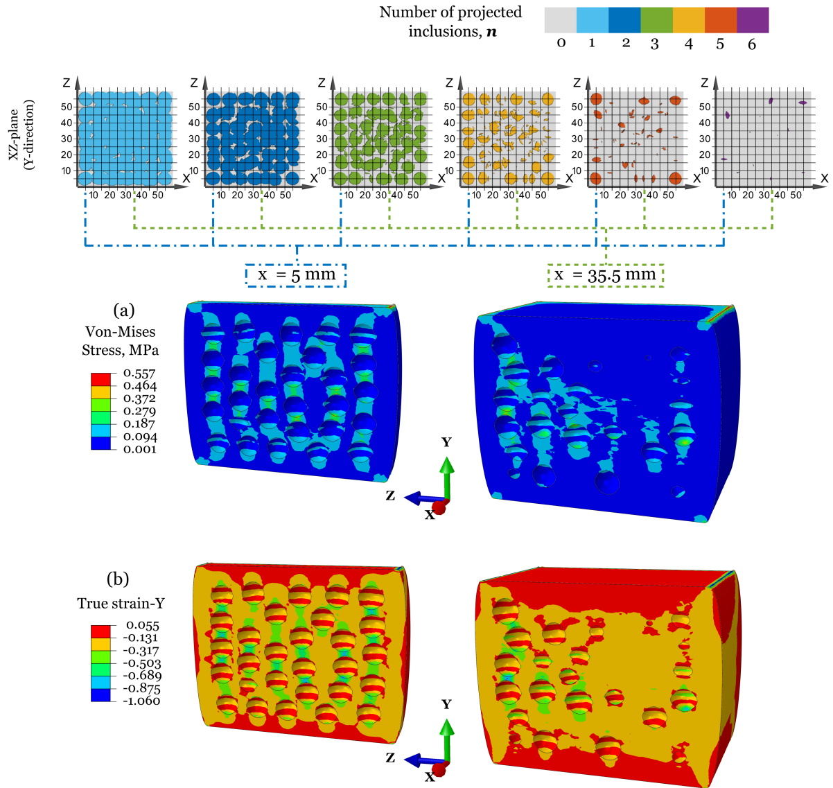
Figure 3.28: Maps of (a) Von Mises stress and (b) Y-uniaxial true strain at x = 5 mm and x = 35.5 mm cross sections (relatively to the central, 60 \times 60 \times 60 mm 3 , part) of V22.5-D8 FE model subjected to compression displacement of 10 mm
