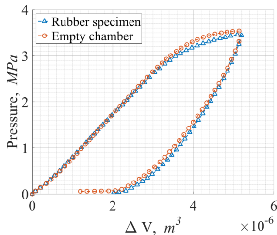
Figure 2.18: Pressure dependences on change in volume during hydrostatic compression experiment
