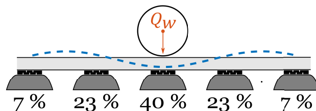
Figure 2.9: Distribution of the wheel load among the sleepers (from [58])
