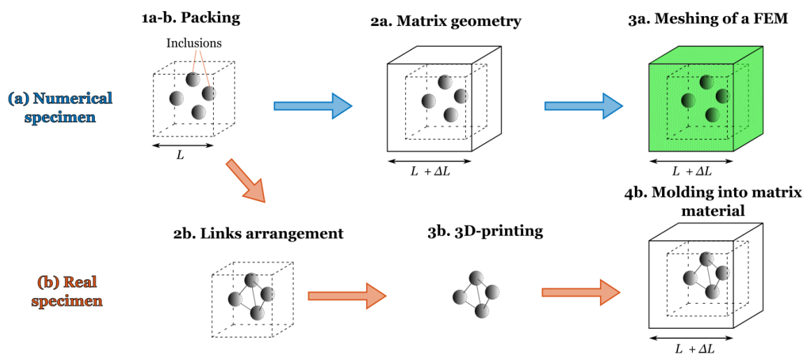
Figure 3.2: Schematic representation of process of development of numerical and real specimens
