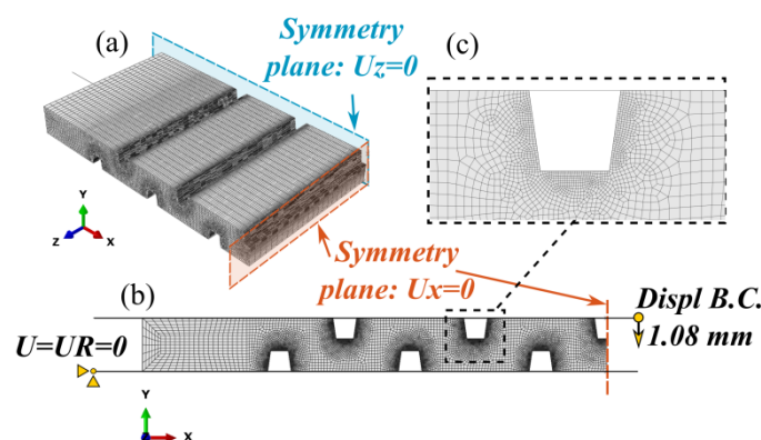
Figure 2.23: 3D and 2D FE models of the rail pad (a-b); planes of symmetry (a-b); boundary conditions applied on rigid compression plates (b); mesh refinement near groove (c)
