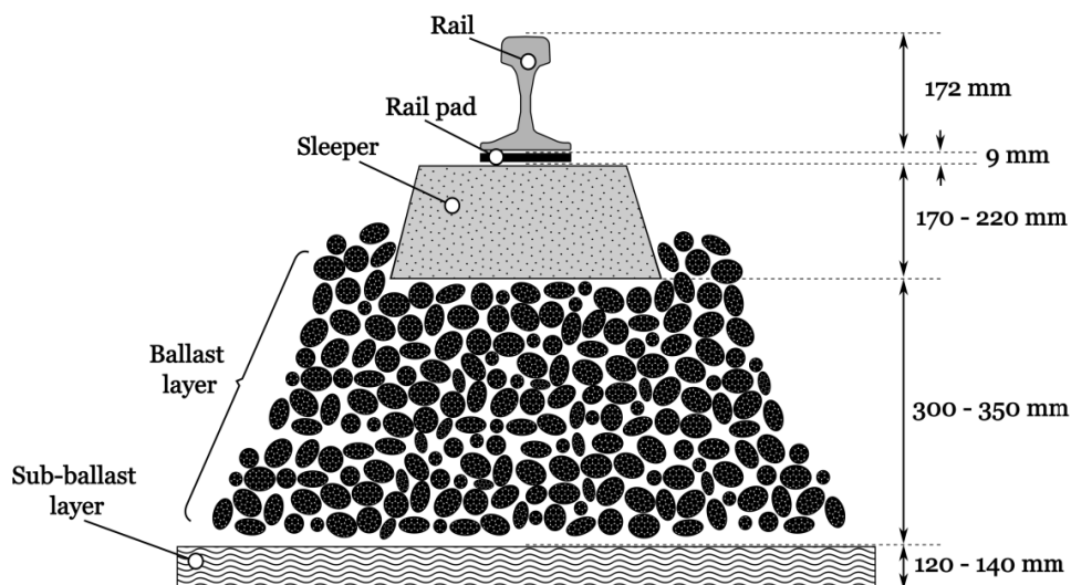
Figure 1: Schematic representation of the TGV ballasted railway track structure
