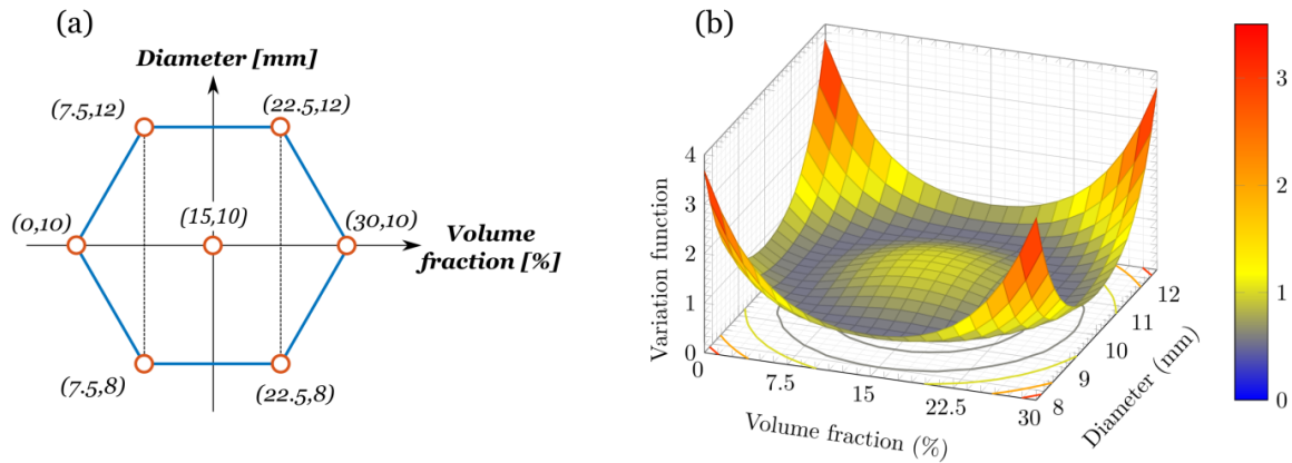
Figure 3.3: Parameters of specimens on the scale of the Doehlert diagram (a); variation function for the Doehlert experimental design (b)
