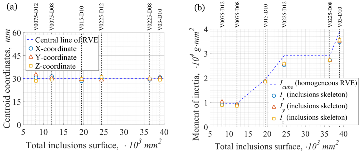
Figure 3 17: The values of coordinates of centroid of spherical inclusions (a) and moment of inertia of inclusions set in relation to the three main axes of the cube (b) as function of total inclusions surface. Results obtained for inclusions arrangements were compared to the central line of the cube (a) and the moment of inertia of an equivalent homogeneous solid (b)
