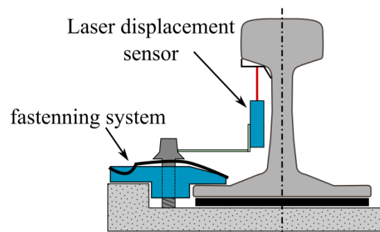
Figure 2.5: Experimental setup for the measurement of a rail pad compression displacement
