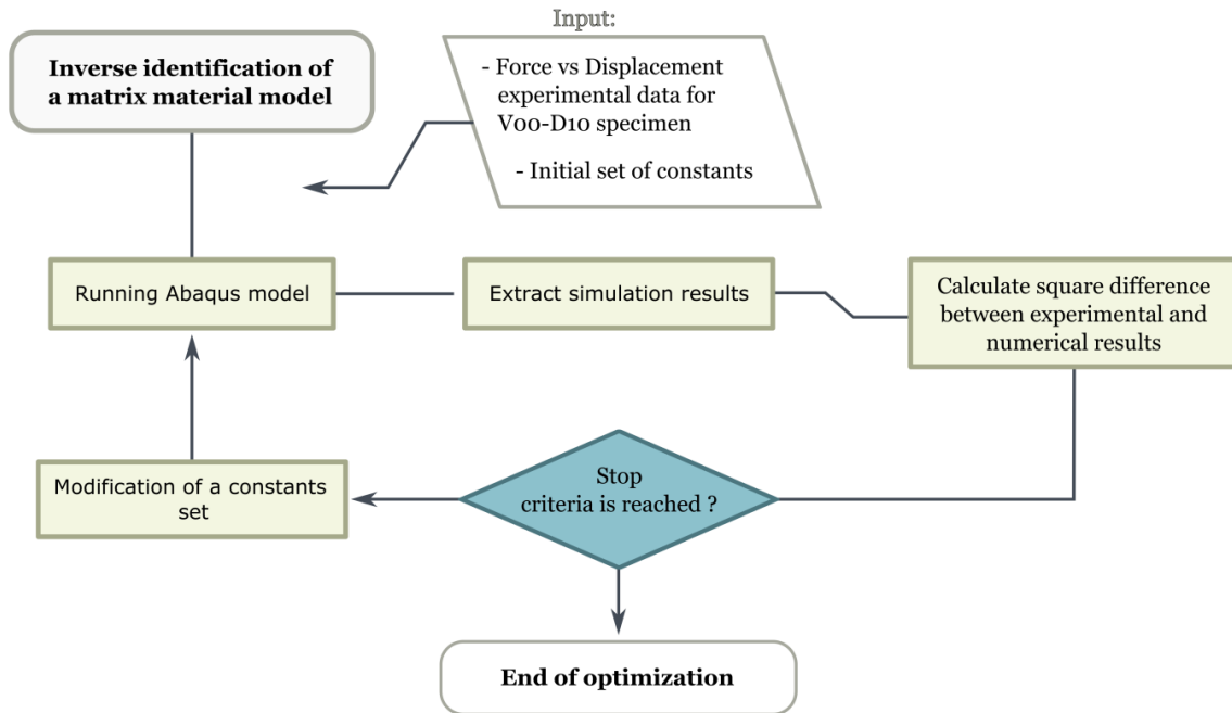
Figure 3.22: Scheme of inverse identification process
