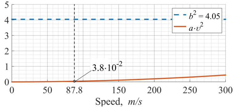
Figure 2.12: Dependence of av^2 on the value of a train speed compared with the value of b^2
