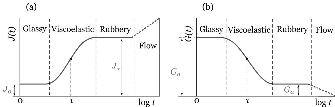
Figure 1.5: The creep compliance J(t) (a) and the relaxation modulus G(t) (b) as functions of time t (from [17])
