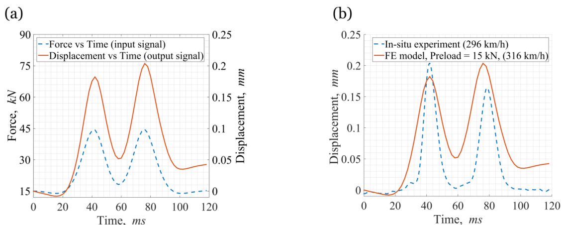
Figure 2.29: Force vs Time curve of a dynamic impact, applied on the numerically studied structure, and Displacement vs Time curve obtained as a result of FE simulation (a); and comparison between dependences of the compression displacement value on time obtained from FE simulation results and by averaging in-situ experimental data (b)
