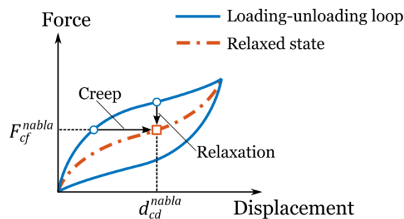
Figure B.1: The same “relaxed” state can be reached either by force relaxation at a constant displacement d_{cd}^{nabla} or by creep at a constant force F_{cf}^{nabla}
