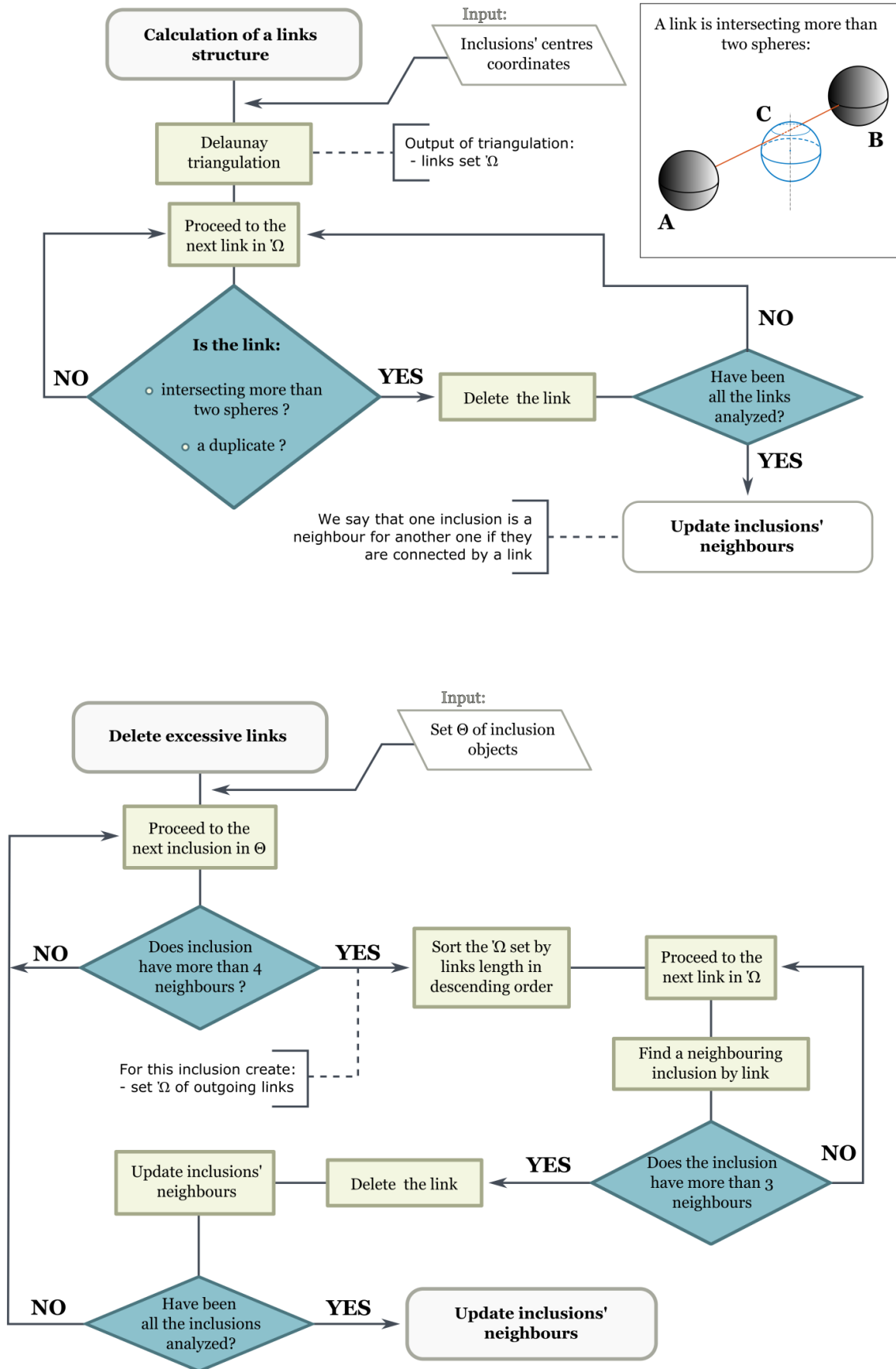
Figure 3.5: Optimization schemes for links number and length
