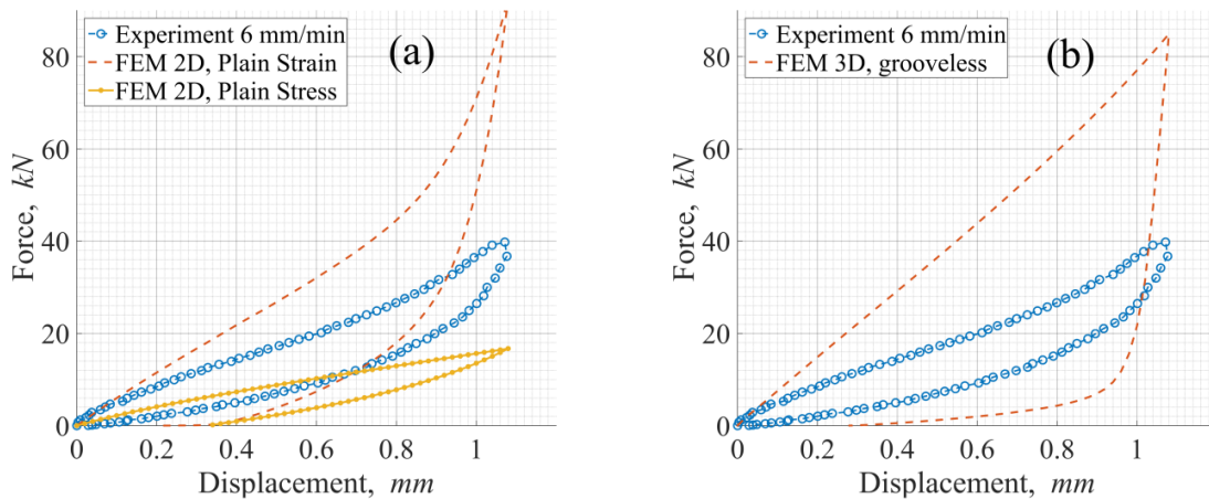
Figure 2.28: Comparison between experimental data and response from FE model of a rail pad: (a) 2D plane strain and plane stress; (b) 3D grooveless
