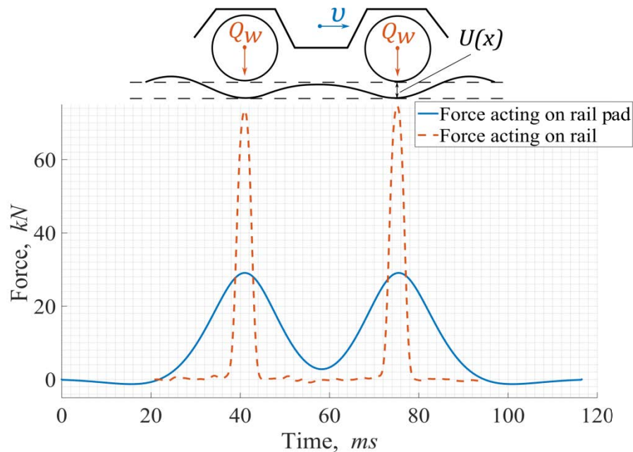
Figure 2.15: Time signals of the forces acting on a rail and a rail pad generated by a bogie passing with the speed v = 87.8 m/s
