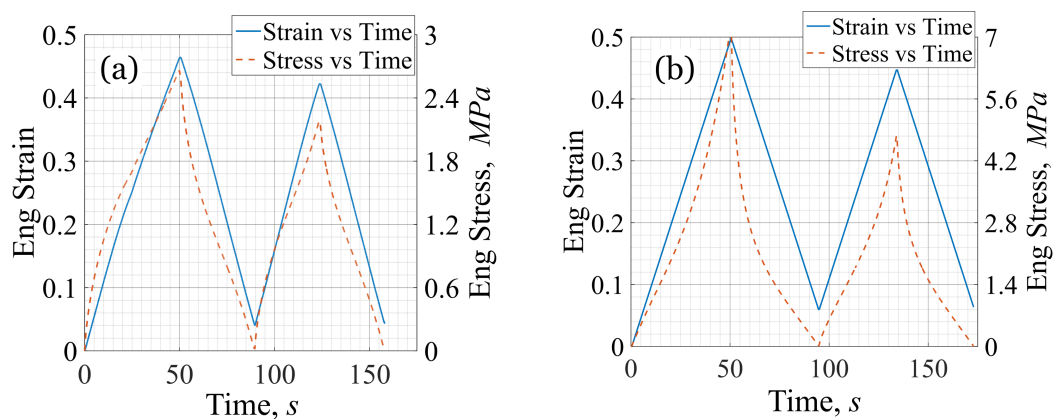
Figure 2.19: Profiles of the Engineering Stress and Strain vs Time in compression (a) and tension (b) experiments
