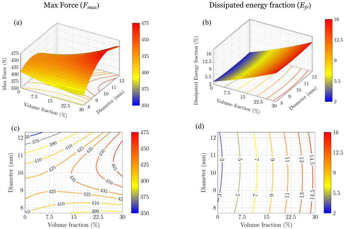
Figure 3.14: F_{max} (a,c) and E_{\%} (b,d) output parameters obtained during QS-compression experiment as functions of inclusions' volume fraction and diameter
