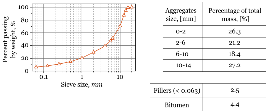
Figure 3.1: Grading curve and composition by mass for a GB3 mixture [4]
