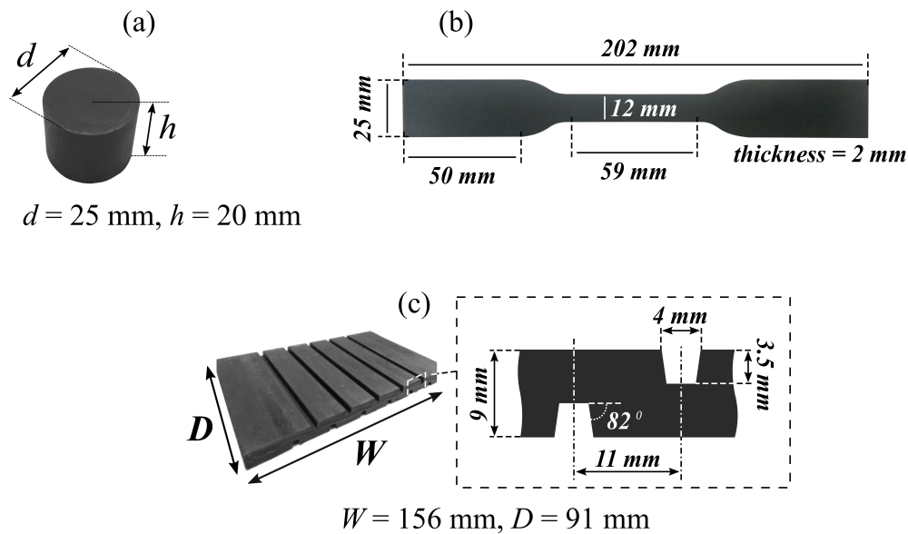
Figure 2.16: Dimensions of: (a) a cylindrical specimen; (b) a dumbbell specimen [112]; (c) a rail pad specimen
