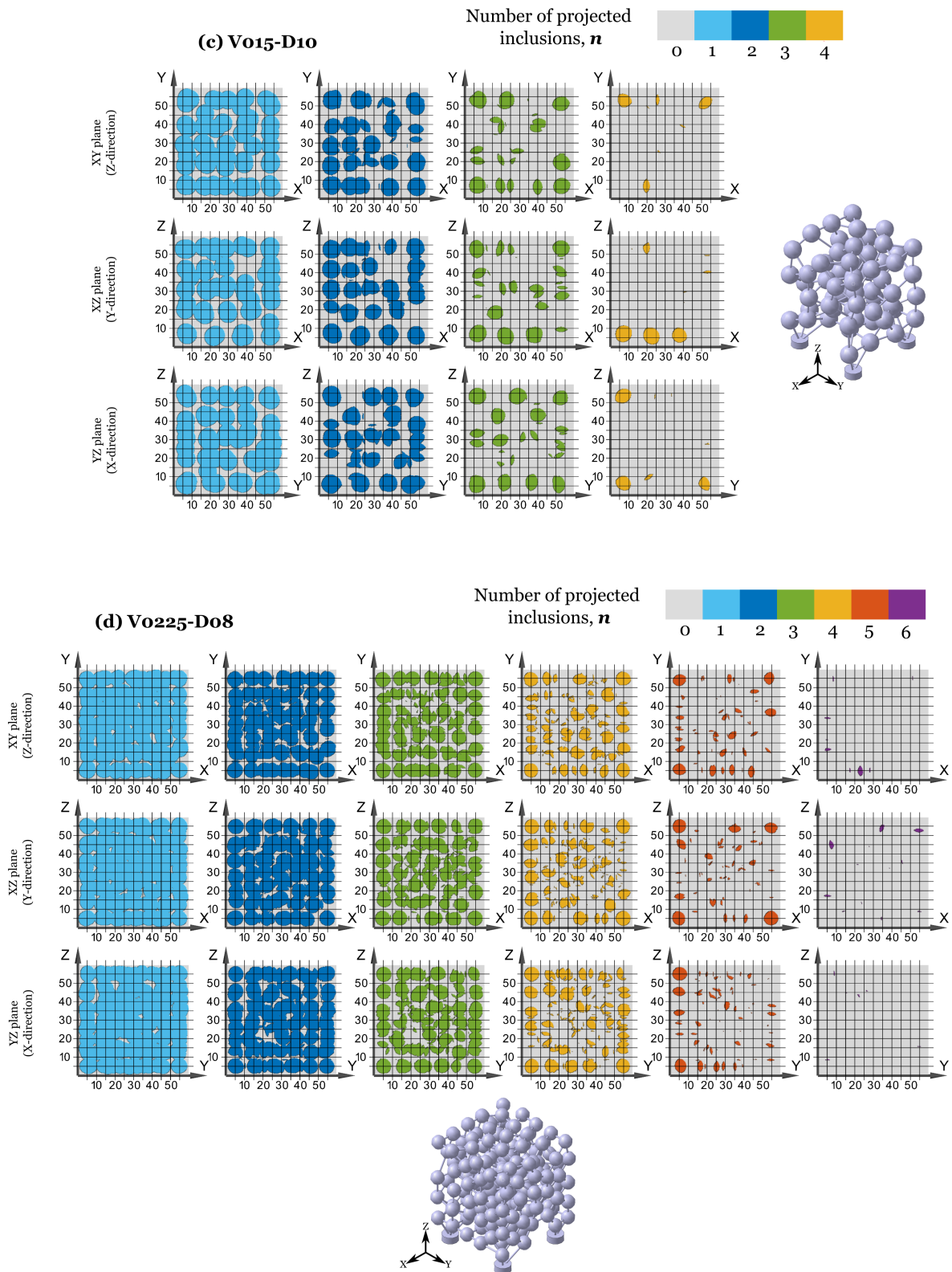
Figure 3.20 c-d: Surfaces of projections for specimens Vo15-D10 (c) and Vo225-Do8 (d)
