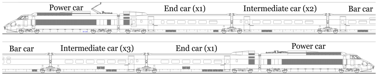
Figure 2.2: TGV train with two power cars, bar/restaurant car, two end and five intermediate passenger cars
