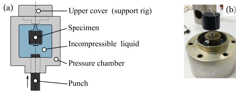
Figure 2.17: Hydrostatic compression experiment testing set: (a) schematic representation of a hydrostatic chamber; (b) specimen on a supporting rig
