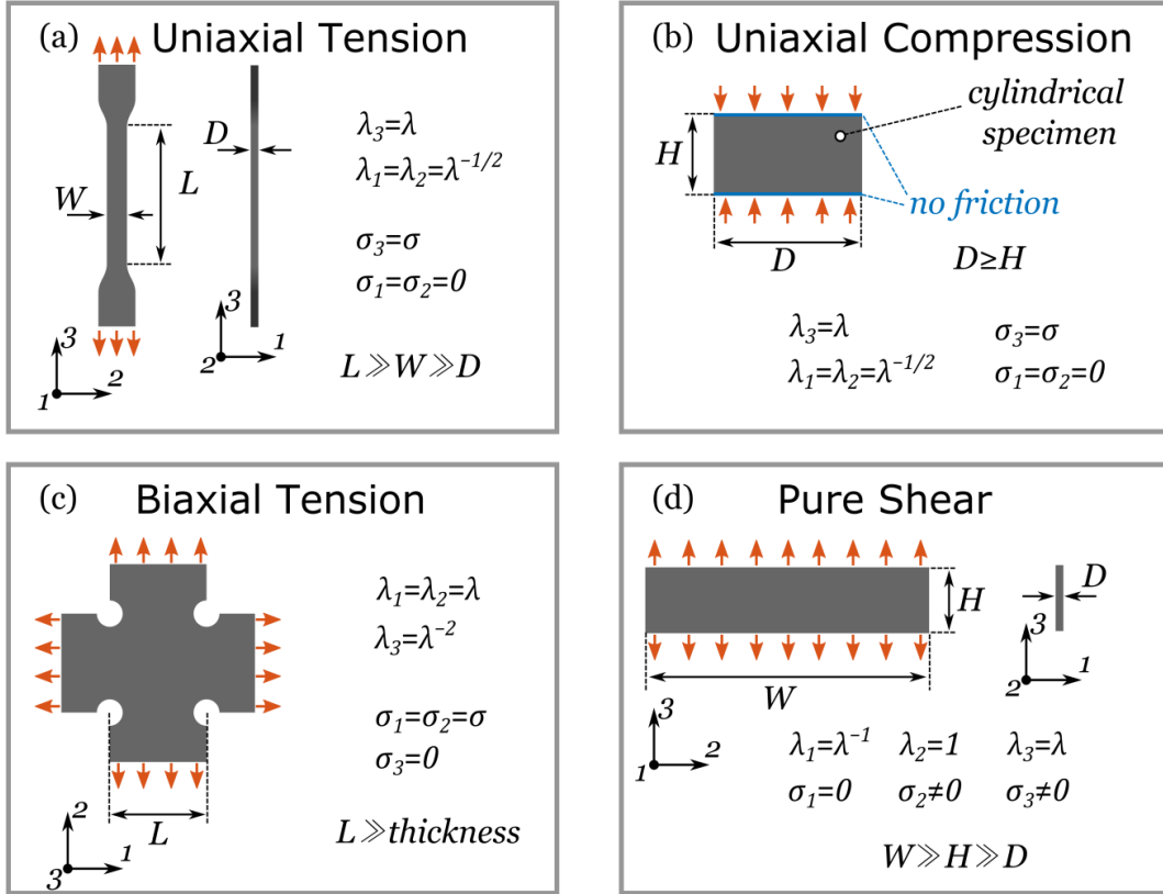
Figure 1.3: Typical tests which provide pure homogeneous deformations for incompressible material: (a) uniaxial tension, (b) uniaxial compression, (c) biaxial tension, (d) pure shear [37].
