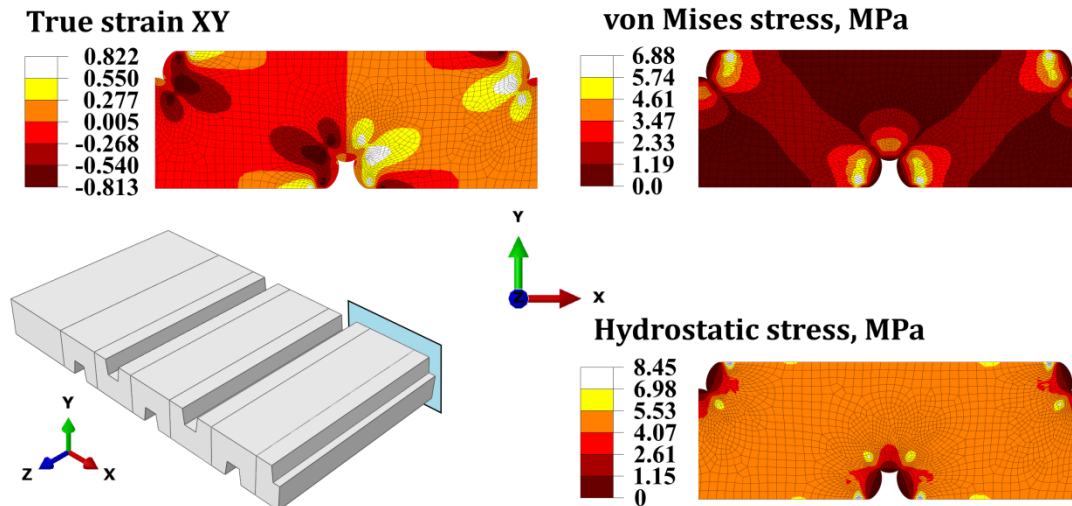
Figure 2.27: True shear strain (XY), von Mises stress and hydrostatic stress maps calculated at the cross-section located in the middle of the specimen. Rail pad is under compressive displacement of 1.08 mm
