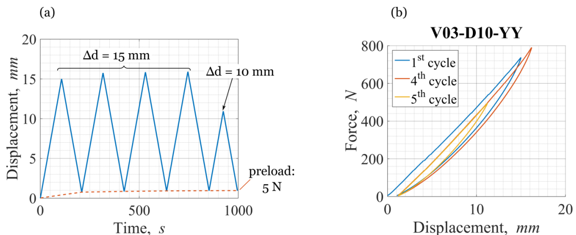
Figure 3.10: VM loading scheme (a) and cycling influence (b)
