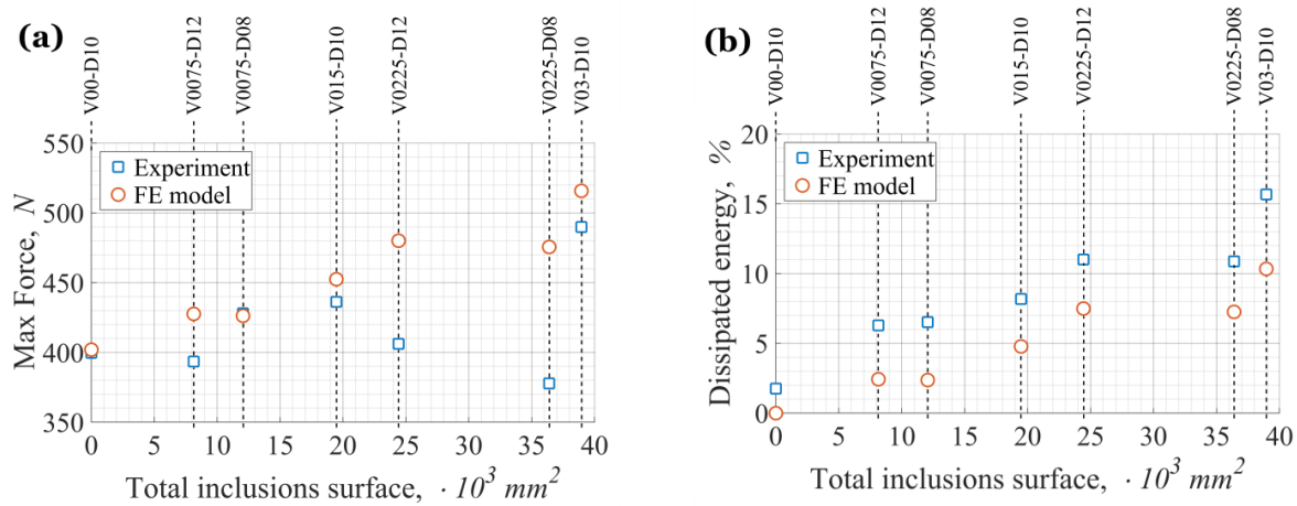
Figure 3.29: Dependences of F_{max} (a) and E_{\%} (b) on total inclusions' surface area obtained during experimental and FE investigations
