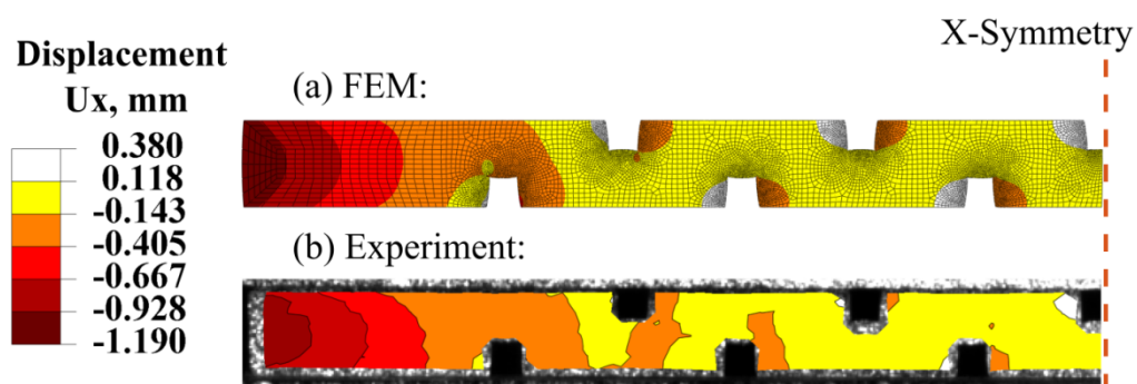
Figure 2.25: Comparison between displacement maps in horizontal direction obtained in FE simulation (a) and experiment (b)
