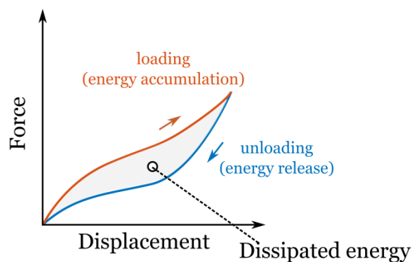
Figure 3.11: Calculation of dissipated energy
