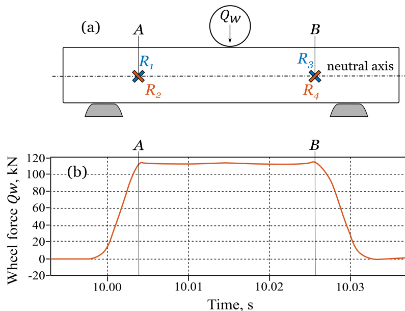
Figure 2.3: Measurement of a wheel force using the set of strain gauges connected to a Wheatstone bridge: (a) location of strain gauges on a rail; (b) an example of signal of one wheel obtained using data from strain gauges
