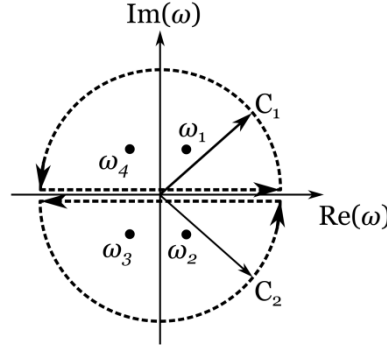
Figure A.1: Contours C_1 and C_2 on the complex plane around poles \omega_i of a complex function F(\omega)
