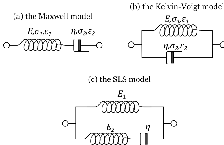
Figure 1.8: Classical mechanical models of linear viscoelasticity
