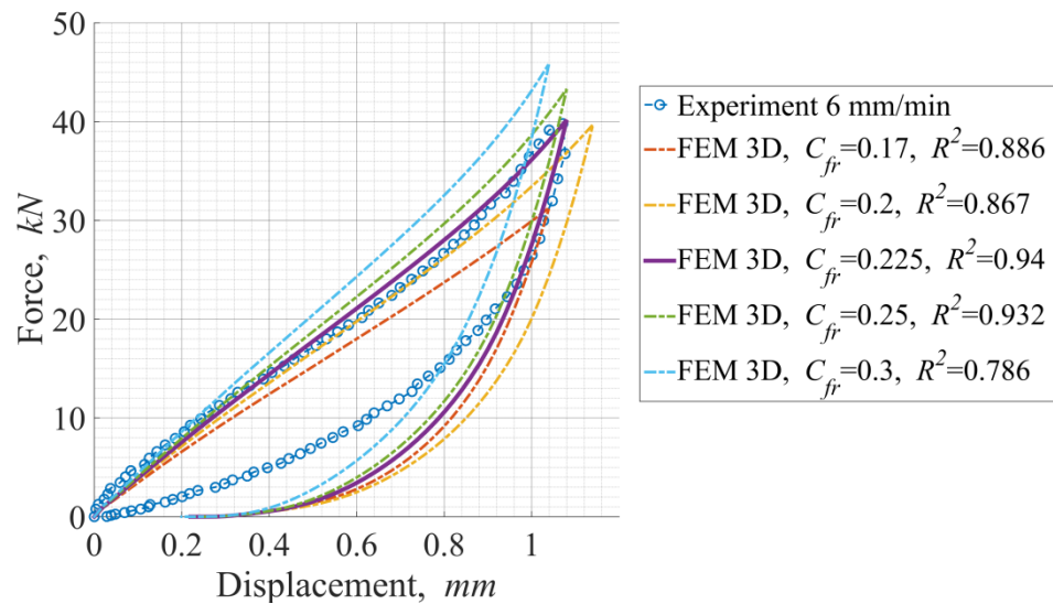
Figure 2.24: Force vs Displacement curves obtained in the experiment and calculated by FE simulation using values of friction in the range of 0.17 to 0.3
