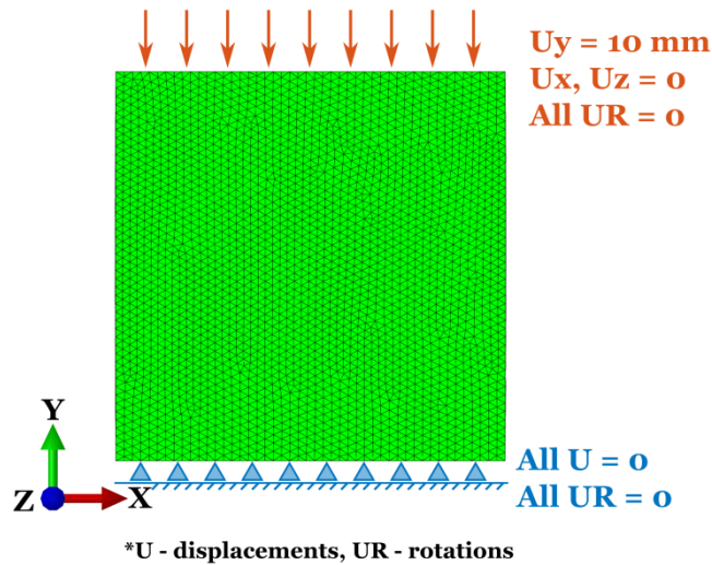
Figure 3.24: Boundary conditions for VM finite element model
