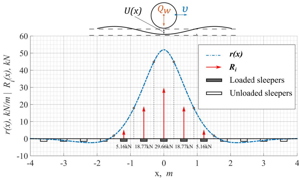
Figure 2.13: Dependence of distributed reaction force r(x, t) (blue curve) on position of a wheel load moving with the speed v = 87.8 m/s and sleepers' reaction forces R_i (red arrows)
