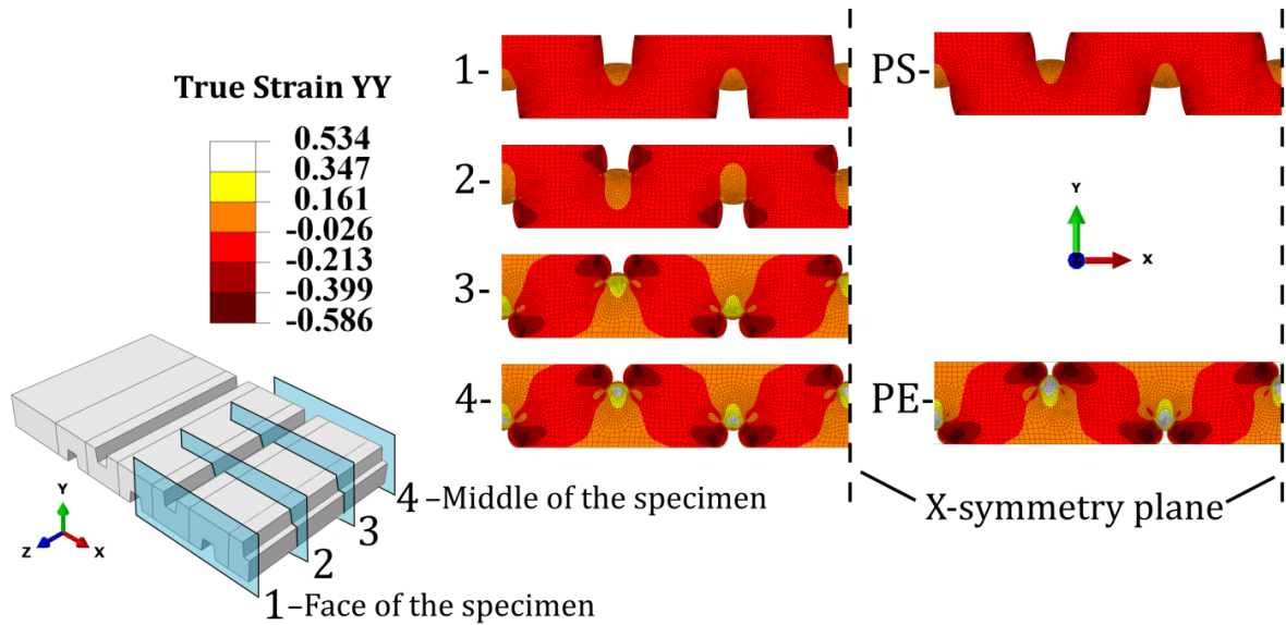
Figure 2.26: True strain YY-field calculated in different cross-sections in the Z-direction (from face to the middle of the specimen) and true strain fields obtained in 2D plane strain (PE) and plane stress (PS) models. Rail pad is under compressive displacement of 1.08 mm
