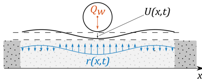
Figure 2.10: Rail on a Winkler foundation subjected to concentrated load Q_w
