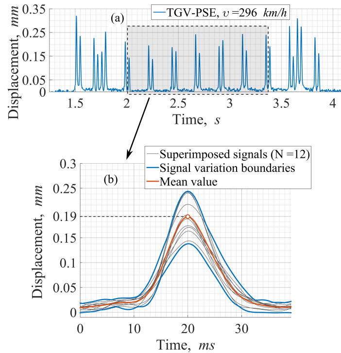
Figure 2.6: The common rail pad compression displacement signal caused by passing of a TGV-PSE train plotted in a time domain (a); superimposed peaks of a rail pad compression displacement signal (b)
