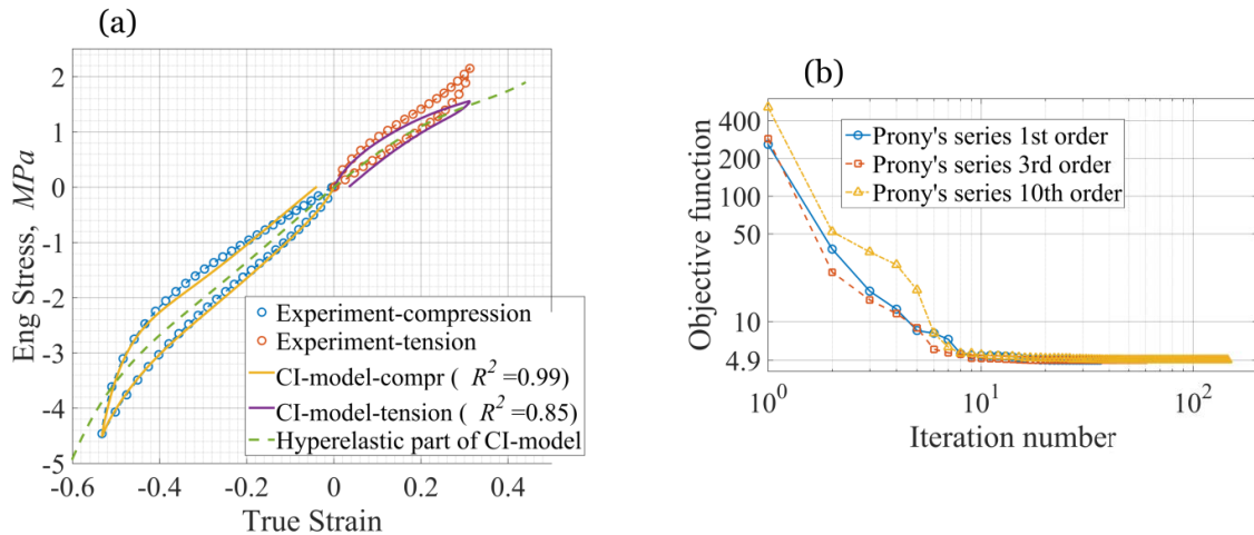
Figure 2.21: (a) Comparison between experimental data and prediction of fitted CI-model; (b) convergence curves for different values of the Prony's series order
