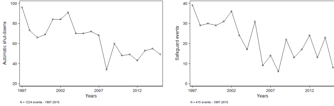
Figure 3.3: Historical occurrences of automatic shut-downs (left) and safeguard events (right) in the French fleet between 1997 and 2015.
