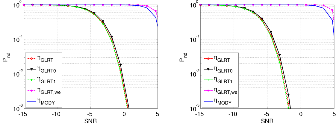
(a) |\alpha_{12}|^2 = 0, |\alpha_{1I}|^2 = 0.262, |\alpha_{2I}|^2 = 0.728
