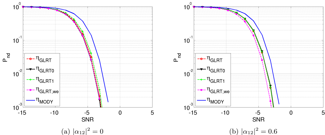
Figure 2.1: P_{\text{ND}} as a function of SNR, N = 32 , K = M = 2 , P_{\text{FA}} = 10^{-3} , No interference, Orthogonal sequences, Deterministic channel
