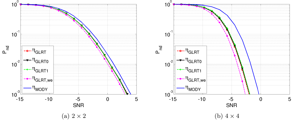
Figure 2.2: P_{ND} as a function of SNR, N = 32 , P_{FA} = 10^{-3} , No interference, Orthogonal sequences, Random channel
