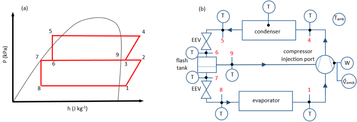
Figure 1.6. Refrigeration cycle P - h diagram (a) and schematic with required measurements (b) of FT injection cycle
