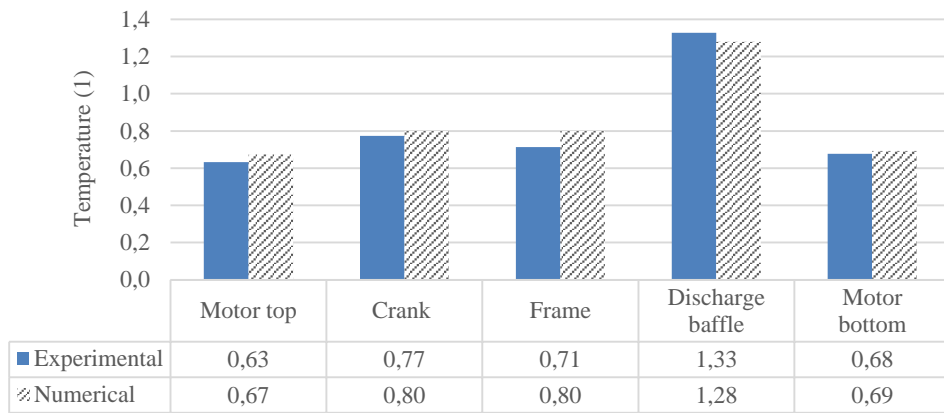
Figure 3.9. Experimental and numerical component temperatures in scroll compressor at T_{cond} = 40\text{ }^{\circ}\text{C} , T_{evap} = 15\text{ }^{\circ}\text{C} , and T_{amb} = 25\text{ }^{\circ}\text{C} , 30 rps (operating condition 4)
