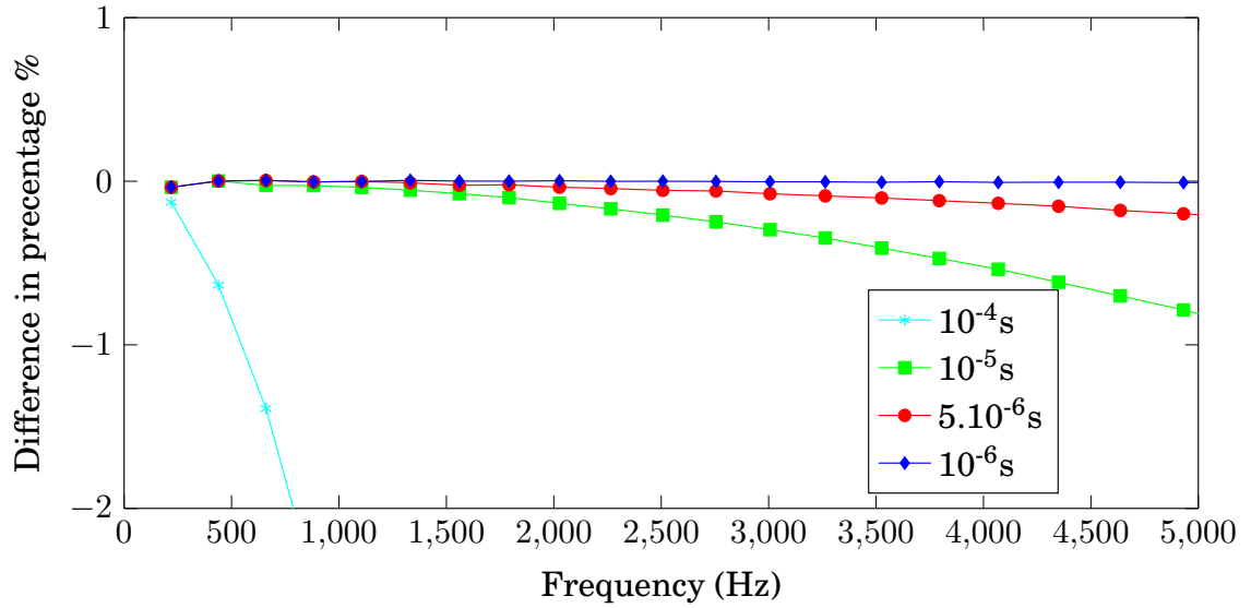
Figure 2.4: Difference in percentage between the theoretical eigenfrequencies and computed frequencies as observed from FFT plots when the simulations are done in time steps of 10^{-4} , 10^{-5} , 5 \cdot 10^{-6} and 10^{-6} seconds.
