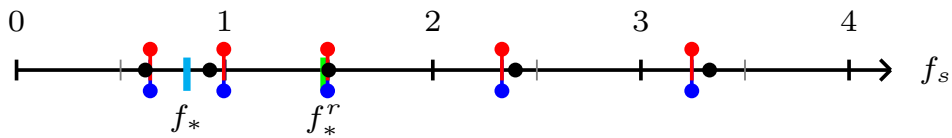
Figure 5.13: Eigenfrequencies plotted on a number line for Case I in units of the fundamental string mode, f_s = 238.2\text{Hz} . The blue and red markers represent the eigenfrequencies as determined from Equation (5.90b) and (5.91b) respectively while the black markers display the eigenfrequencies for the complete system, i.e. from Equation (5.88).
