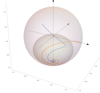
Figure 4.3: Decaying system. Two different trajectories of system (4.33) with E = 1 , a = 0 , b_+ = 0 , b_- = 1 . In transparency the ellipsoid (4.36).
