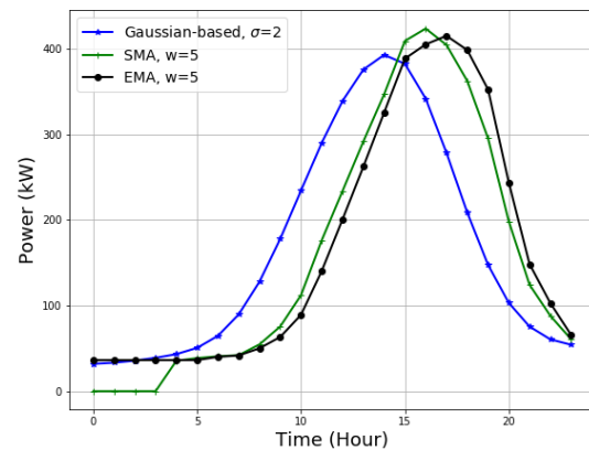
3.17.4: When \gamma = 25\%
