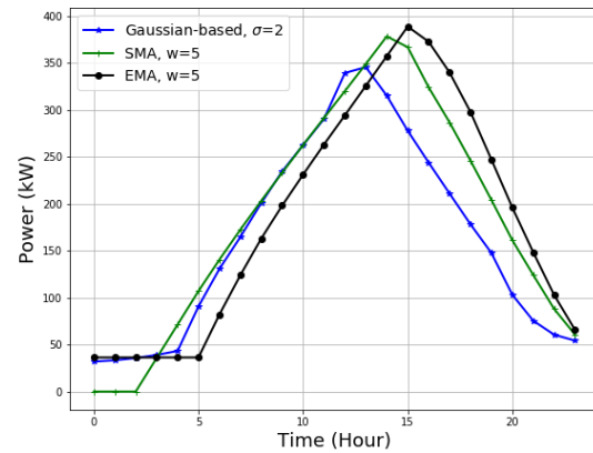
3.17.2: When \gamma = 10\%
