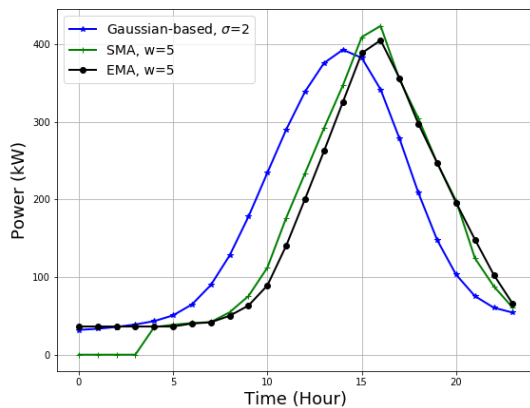
3.17.3: When \gamma = 15\%
