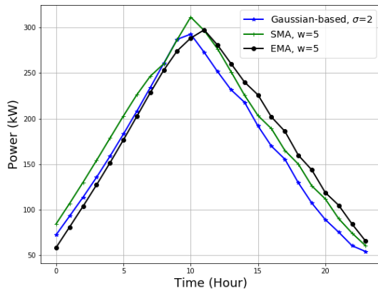
3.17.1: When \gamma = 5\%
