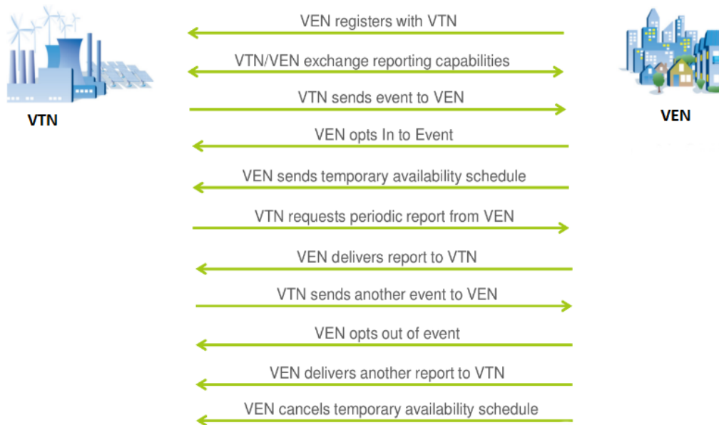
Figure 2.11 – VTN and VEN communications using OpenADR services [Haa13].
