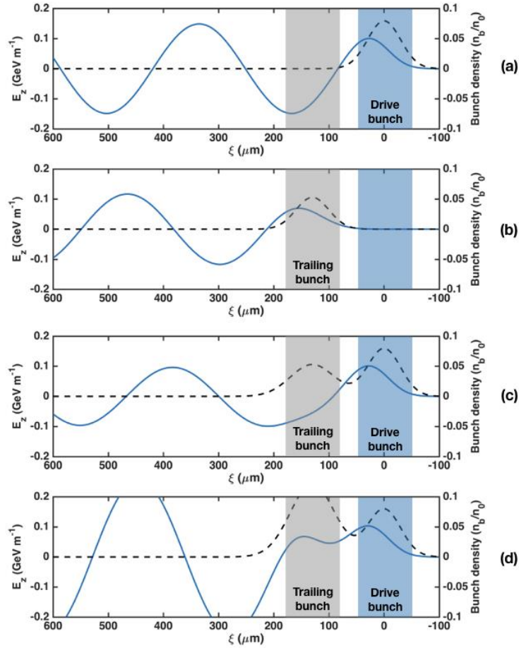
Figure 5.8: (a) E_z field on axis, in the linear regime of positron driven wakefield. n_0 = 10^{16} cm^{-3} , N_{drive} = 3 \cdot 10^8 particles. Drive beam at \xi = 0 . (b) E_z field on axis. n_0 = 10^{16} cm^{-3} , N_{trailing} = 2 \cdot 10^8 particles. Trailing beam initially at \xi = 130 \mu m . (c) E_z field on axis, with a loaded wakefield. n_0 = 10^{16} cm^{-3} . Drive beam at \xi = 0 \mu m and trailing beam at \xi = 130 \mu m , the total wakefield is the superposition of the previous two. The wake is still accelerating at the trailing position (grey area), the wake is not optimally loaded. N_{drive} = 3 \cdot 10^8 particles and N_{trailing} = 2 \cdot 10^8 particles. (d) E_z field on axis, with an overloaded wakefield: the wake becomes decelerating at the trailing position. n_0 = 10^{16} cm^{-3} . Drive beam at \xi = 0 \mu m and trailing beam at \xi = 130 \mu m . N_{drive} = 3 \cdot 10^8 particles and N_{trailing} = 4.5 \cdot 10^8 particles.
