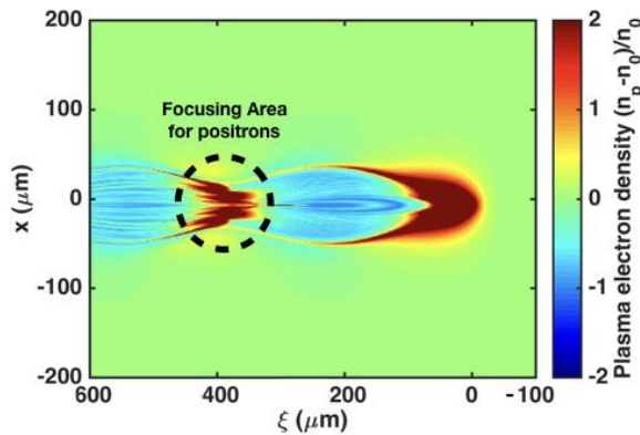
Figure 4.1: Plasma electron density in a positron wakefield from a PIC simulation. The code QuickPIC was used, with n_0 = 10^{16} \text{ cm}^{-3} , and a drive bunch of charge Q_{drive} = 480 \text{ pC} and dimensions (\sigma_x, \sigma_y, \sigma_z) = (35 \text{ } \mu\text{m}, 25 \text{ } \mu\text{m}, 30 \text{ } \mu\text{m}) . The focusing and accelerating area is very limited, by contrast, the large blue area is very defocusing for positrons.
