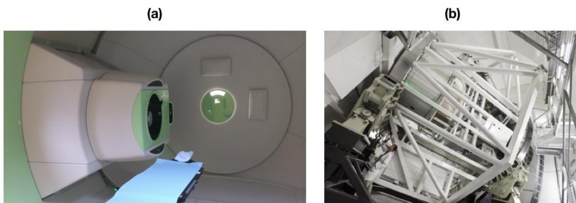
Figure 1.3: (a) Gantry of the proton therapy center in Orsay, France. The patient lies on the bed (center), the ionizing radiations flow from the mobile green and white device (left). (b) Moving structure of the gantry. The chamber (a) is inside the circular shape on the top left. The grey device on the bottom of the picture is one of the brake of the moving structure. Its total height is approximately 4m. Courtesy of E. Bayard
