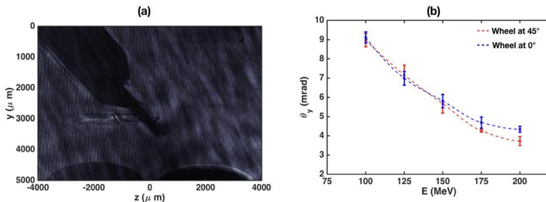
Figure 6.11: (a) Side-view image that displays the 45^\circ oriented wheel. (b) Plot of the divergence of the beam as a function of the energy of the particle. No effect of the 45^\circ wheel is seen, compared to the 0^\circ usual one.
