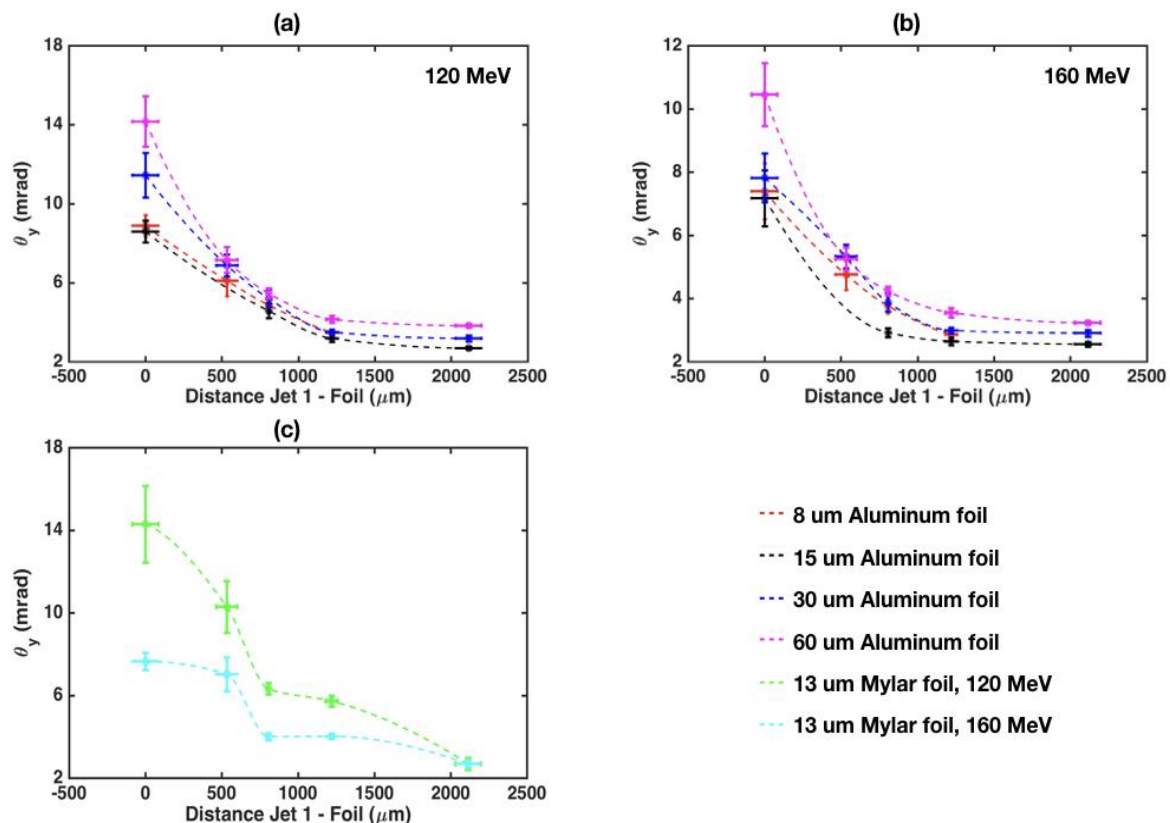
Figure 6.13: Plots of the divergence evolution for different materials and thicknesses of the foil in the wheel. (a) Aluminum foil of different thicknesses. The divergence is measured at 120 MeV. (b) Aluminum foil of different thicknesses. The divergence is measured at 160 MeV. (c) Mylar foil, divergence at 120 MeV and at 160 MeV.
