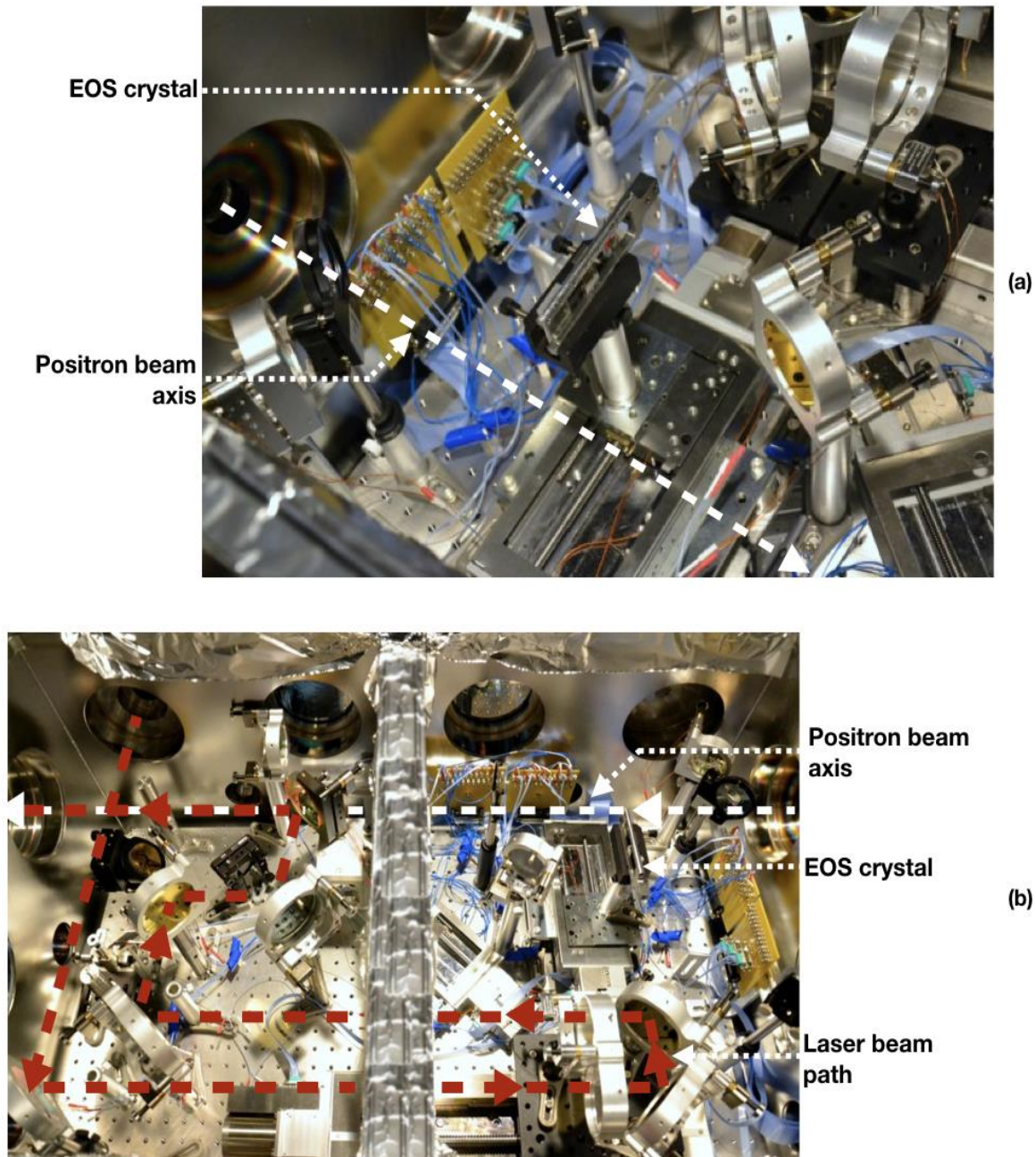
Figure 5.4: (a) EOS crystal and titanium wedge mount in the picnic basket. (b) Overview of the picnic basket with the positron beam and laser beam paths.
