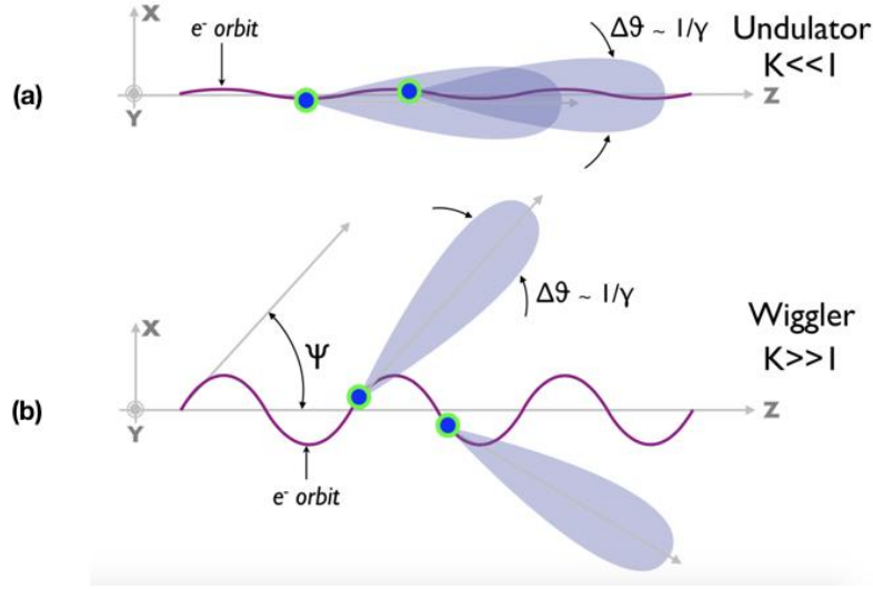
Figure 7.2: (a) Electron trajectory and X-ray emission cone in the undulator regime. (b) Electron trajectory and X-ray emission cone in the wiggler regime. Figure from [Corde 13].
