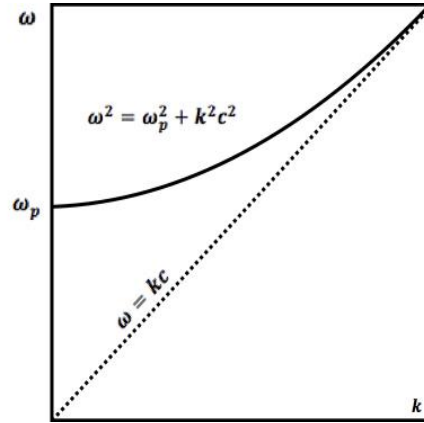
Figure 2.4: Dispersion diagram for electromagnetic waves in a plasma. \omega_p appears as the cut-off frequency. Waves of frequency inferior to \omega_p cannot propagate in the plasma [Rax 05].
