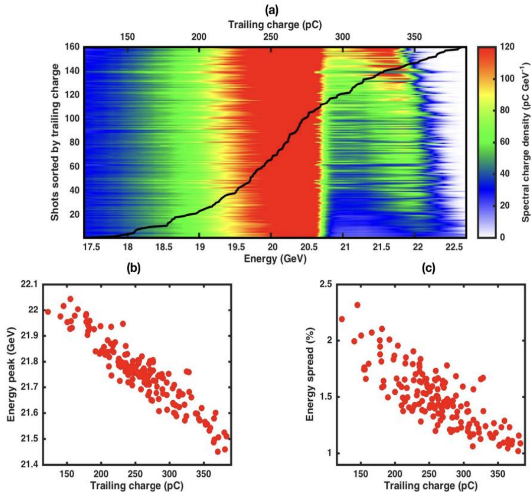
Figure 5.9: (a) Waterfall plot of the 160 spectra in which the beam loading effects are particularly visible. Each line is an integrated spectrum from the Cherenkov spectrometer. (b) Correlation between the trailing bunch charge and the peak energy of the accelerated bunch. (c) Correlation between the trailing bunch charge and the energy spread of the accelerated bunch.
