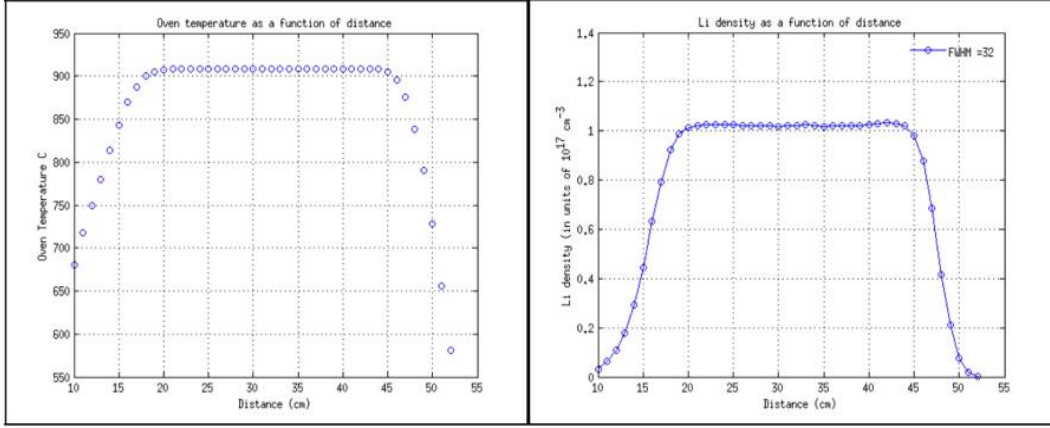
Figure 4.5: A plasma oven temperature profile (left) and density profile (right), from [Vafaei-Najafabadi 12]
