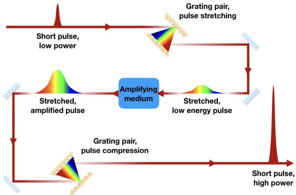
Figure 1.6: Schematic of the chirped pulse amplification technique.
