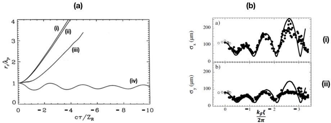
Figure 3.1: (a) Laser spot size as a function of the normalized propagation distance in the plasma. (i) Vacuum diffraction (ii) L = \frac{\lambda_p}{4} (iii) L = \frac{\lambda_p}{4} , P = P_c , a_0 = 0.9 and \lambda_p = 0.03 cm (iv) Guiding in a preformed plasma channel, from [Sprangle 92, Esarey 09] (b) Betatron oscillations of the drive beam of an electron driven PWFA experiment. Transverse beam dimensions as a function of the phase advance (i) Beam spot size in the horizontal plane ( \sigma_x ) (ii) Beam spot size in the vertical plane ( \sigma_y ), from [Clayton 02].
