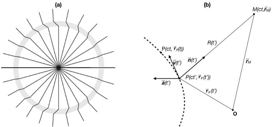
Figure 7.1: (a) Perturbation of the electric field propagating from a charged particle. (b) Definition of the retarded time t' and of various notations.
