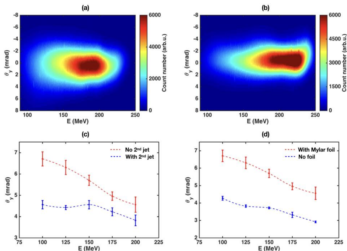
Figure 6.9: (a) Example of an electron bunch spectra, for a shot with a Mylar window to block the laser, but no gas in the second jet. (b) Same, but with gas in the second jet. (c) Divergence of the beam on the spectrometer as a function of the particles energy. The focusing effect of the second gas jet is visible. (d) Divergence of the beam on the spectrometer as a function of the particles energy. This is an evidence of the defocusing effect of the Mylar foil.
