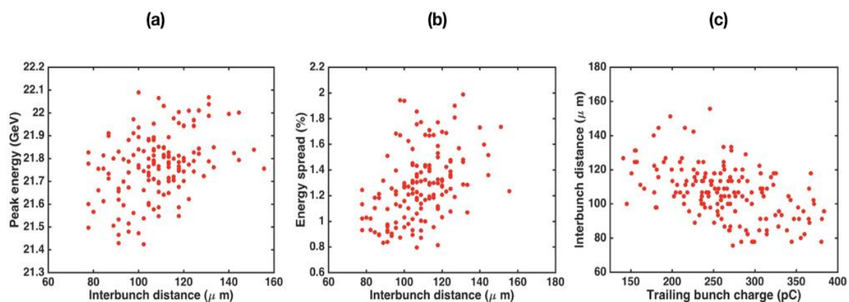
Figure 5.10: Absence of correlations with the interbunch distance. Plot of the peak energy of the accelerated bunch as a function of the interbunch distance (a), plot of the energy spread of the accelerated bunch as a function of the interbunch distance (b), plot of the interbunch distance of the accelerated bunch as a function of the trailing bunch charge (c).
