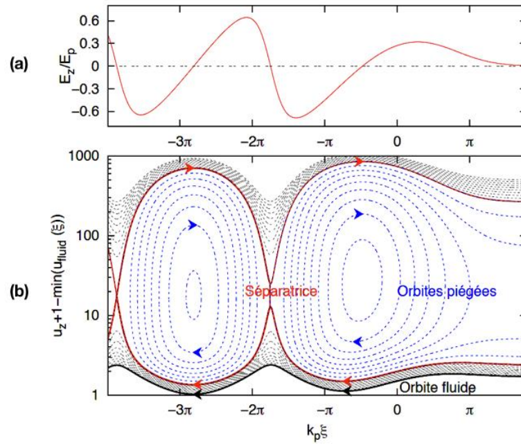
Figure 6.1: (a) Longitudinal electric field of a nonlinear laser driven wakefield (b) Phase portrait of the particles in the plasma. The separatrix (red line) distinguishes the trapped particles from the particles traversing the wakefield. The vertical coordinate is the speed. Figure from [Réchatin 10].
