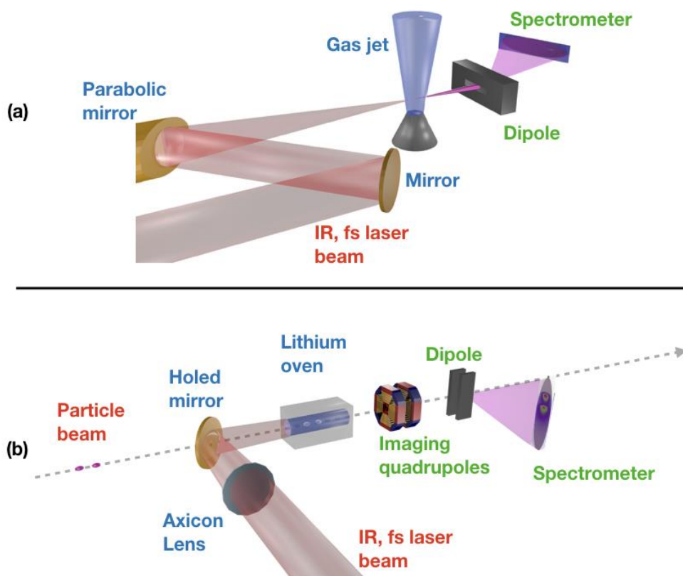
Figure 0.2: (a) A typical laser wakefield experiment, a parabolic mirror focuses a laser beam into a gas jet. The emerging electron beam is characterized by a spectrometer. (b) A plasma wakefield experiment, in which two particle bunches are sent into a laser pre-ionized plasma. A spectrometer displays the energy of the particle bunch emerging from the plasma. This experiment can be carried out with electron or positron bunches.
