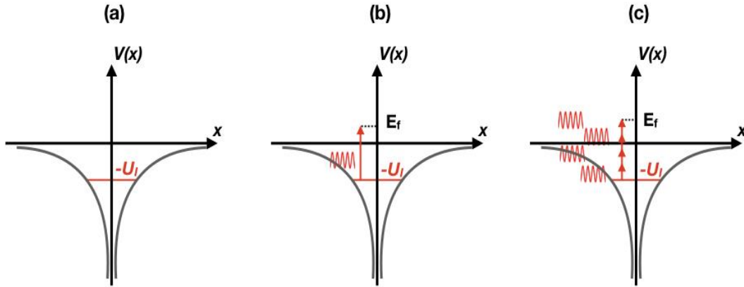
Figure 2.2: Ionization processes (a) Coulomb potential of an atom, the valence electron has an ionization energy U_I . (b) Low-Field Ionization process, the energy of the incoming photon is high enough to ionize the atom. (c) Multi-Photon Ionization: the atom is ionized under the combined effect of multiple photons. When the total energy of the photons is U_I the process is called Multi-Photon Ionization. In the specific case where the total energy is higher than U_I , the process is called Above-Threshold Ionization, case (c).
