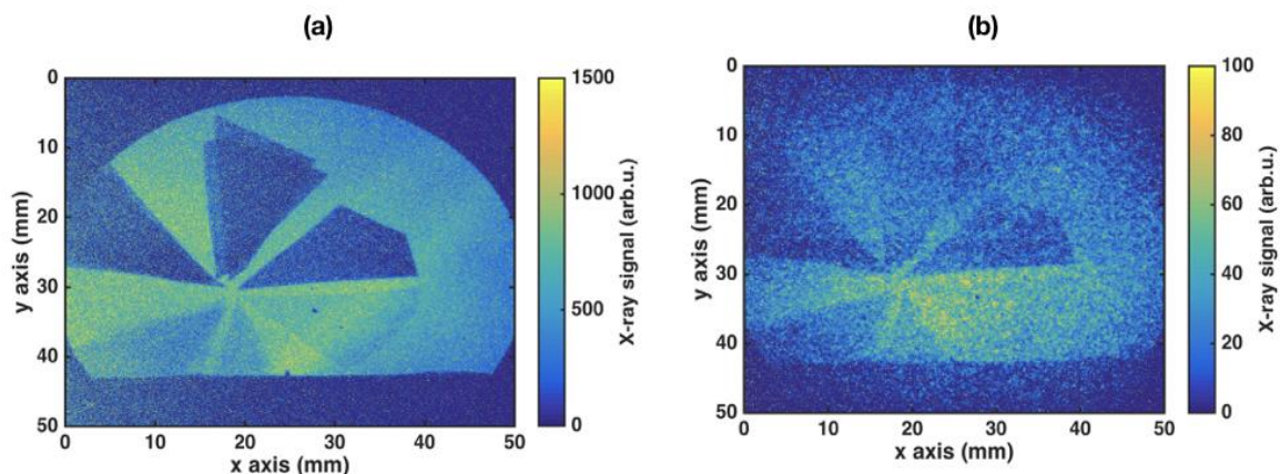
Figure 7.5: (a) X-ray signal on the CCD chip, parameters for this shot were P_1 = 17 bars and P_2 = 40 bars (highest signal in Fig.7.4). (b) X-ray signal on the CCD chip, parameters for this shot were P_1 = 17 bars and P_2 = 0 bars (reference signal in Fig.7.4).
