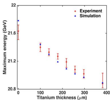
Figure 5.12: Maximum energy of the accelerated particles as a function of the titanium thickness.
