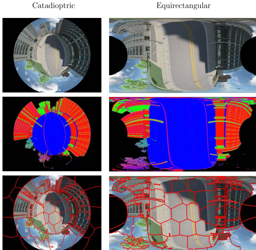
Figure 6.7 – OmniSLIC superpixel segmentations of an RGB-D catadioptric image. Observe that adherence to the boundaries of the superpixels takes into account the normal map (second row images) and the color images. The values used in the segmentation are k = 50 , m = 30 and the tradeoff between the intensity and normal images is set to \lambda = 1 .
