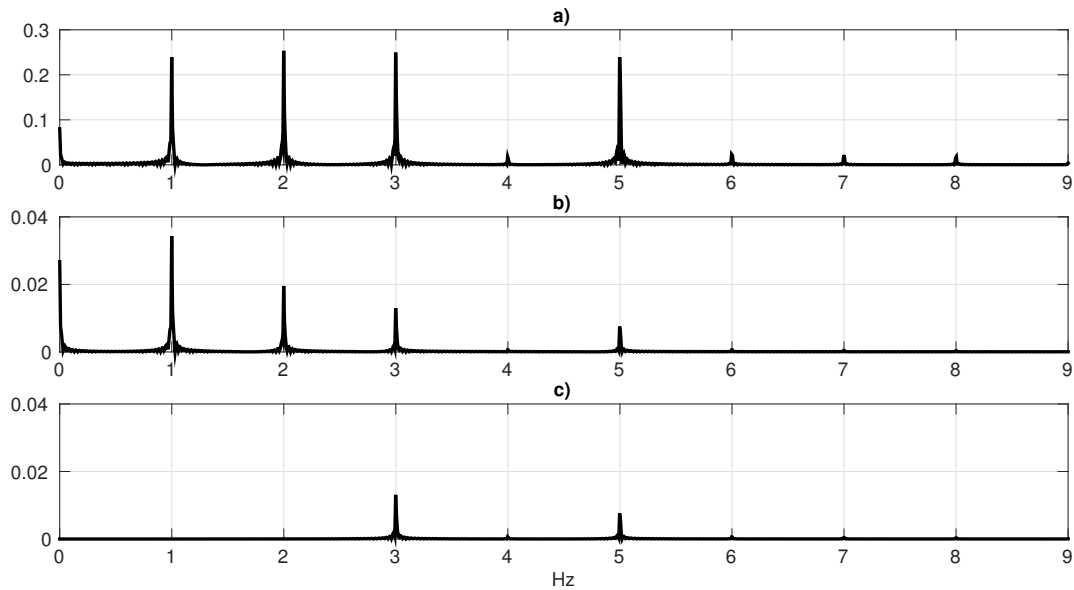
Figure 5.1: Plot a) shows the spectrum of the friend \psi(t) . Plot b) shows the spectrum of the output steady-state e(t) when there is no internal model (namely v = 0 ). Plot c) shows the spectrum of the output steady-state e(t) when the dimension of the internal model is L = 2 .
