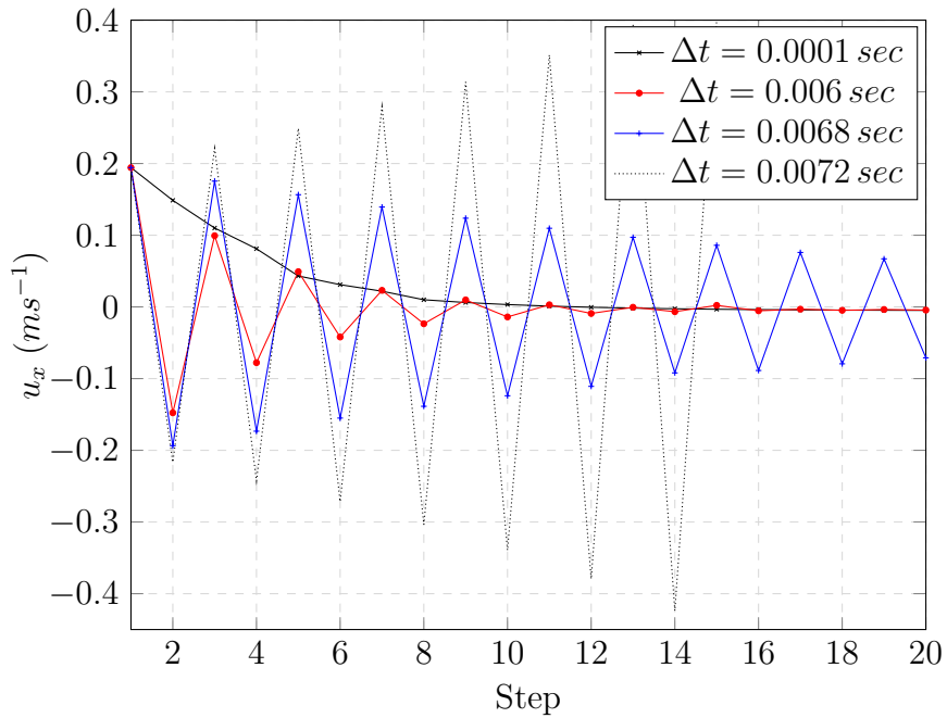
Figure 4.21: Evolution of the horizontal velocity at P(0.5;0.75) with different time-steps and \Delta t^* = 0.0035 sec.
