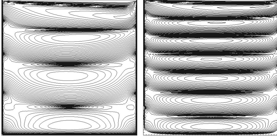
(a) Velocity magnitude isocontour: Re = 5000, N = 5 (b) Velocity magnitude isocontour: Re = 5000, N = 30
