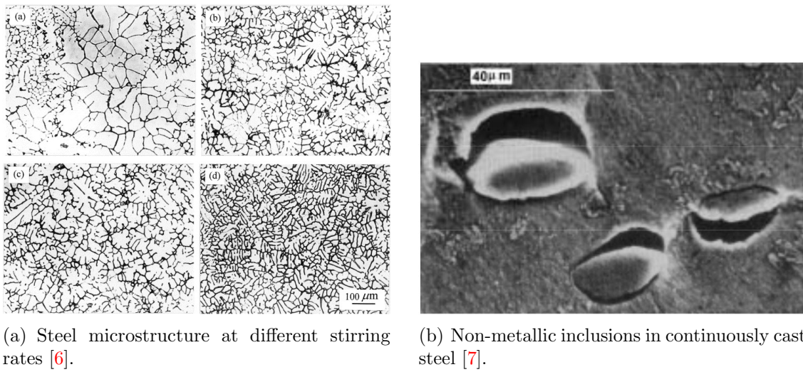
Figure 1.5: Microscopic structure and inclusions in steel.
