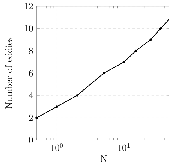
Figure 4.8: Number of horizontal eddies with respect to the magnetic interaction parameter.
