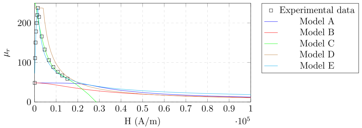
(b) \mu -H magnetization curve
