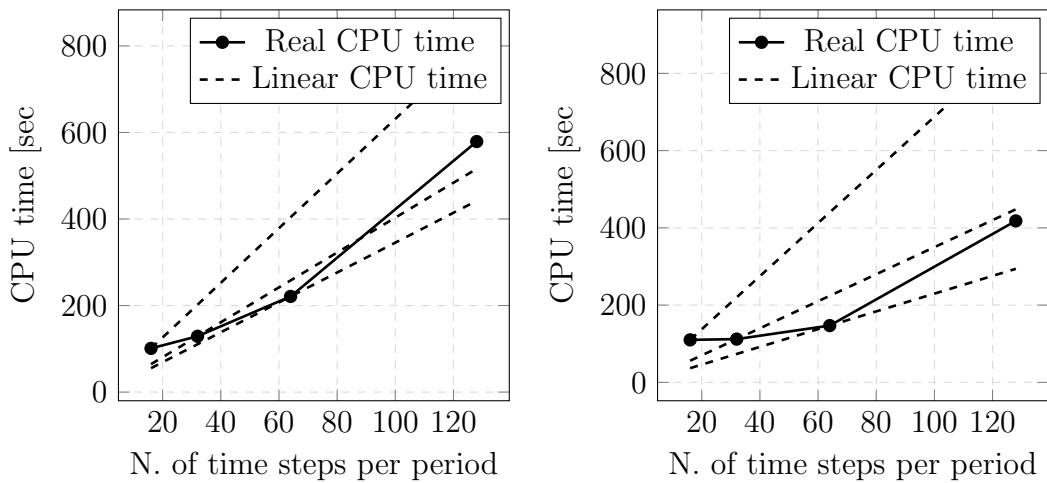
(a) Comparison between actual CPU time and its potentially linear evolution with explicit Euler scheme
