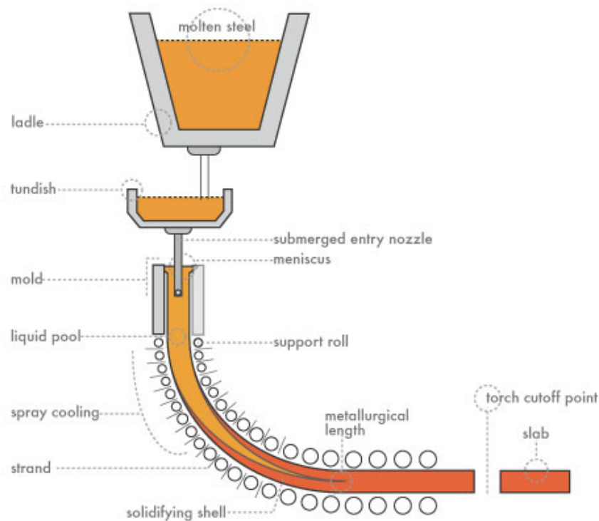
Figure 1.2: Continuous casting machine
