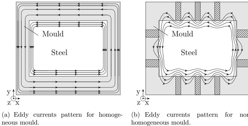
Figure 5.13: Electrical eddy current patter with (b) and without (a) insulating layers in the mould.
