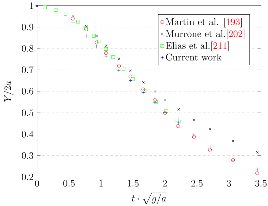
Figure 4.25: Non-dimensional column height evolution.
