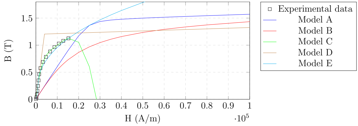
(a) B-H magnetization curve
