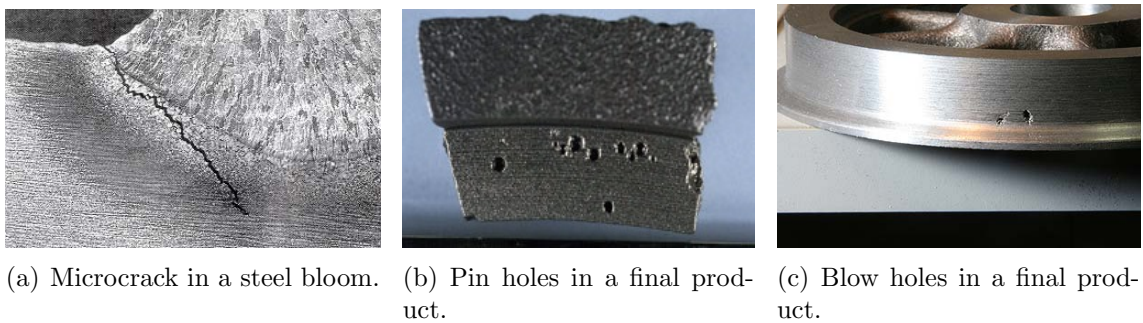
Figure 1.6: Examples of defects in the casting product.
