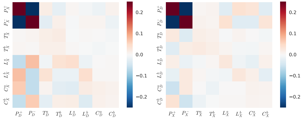
Figure V.10: Submatrices of the Kernel norm matrix \mathbf{G} corresponding to the effect of DAX events on EUROSTOXX STOXX events (left) and vice versa (right). These two submatrices correspond to the ones lying on the antidiagonal on the Figure V.9
