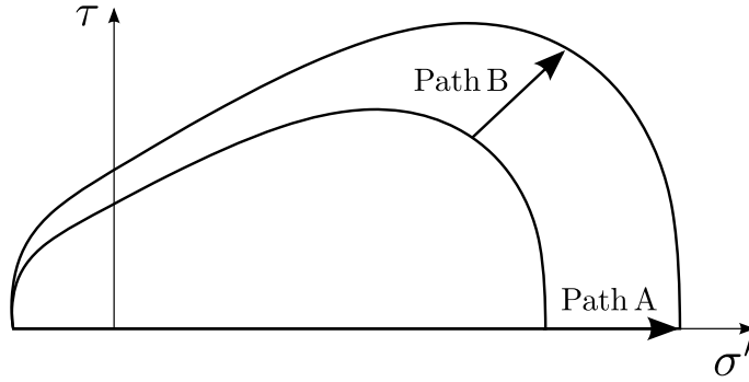
Figure 5.11: Two different stress paths with equal plastic energy increase.
