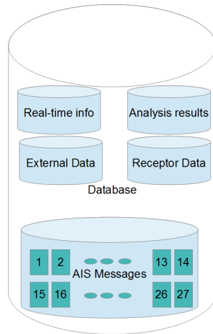
Figure 5.6: Database composition
