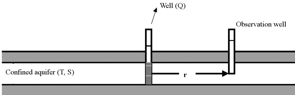
FIGURE A.15 – Geometry for the Theis' solution (modified from Hunt (2008).)
