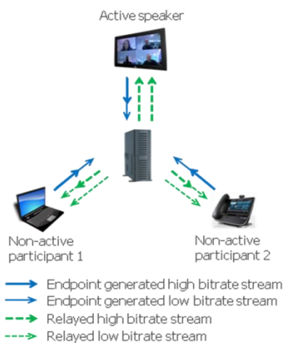
Figure 2.9: Logic of SFU based on Scalable Video Coding
