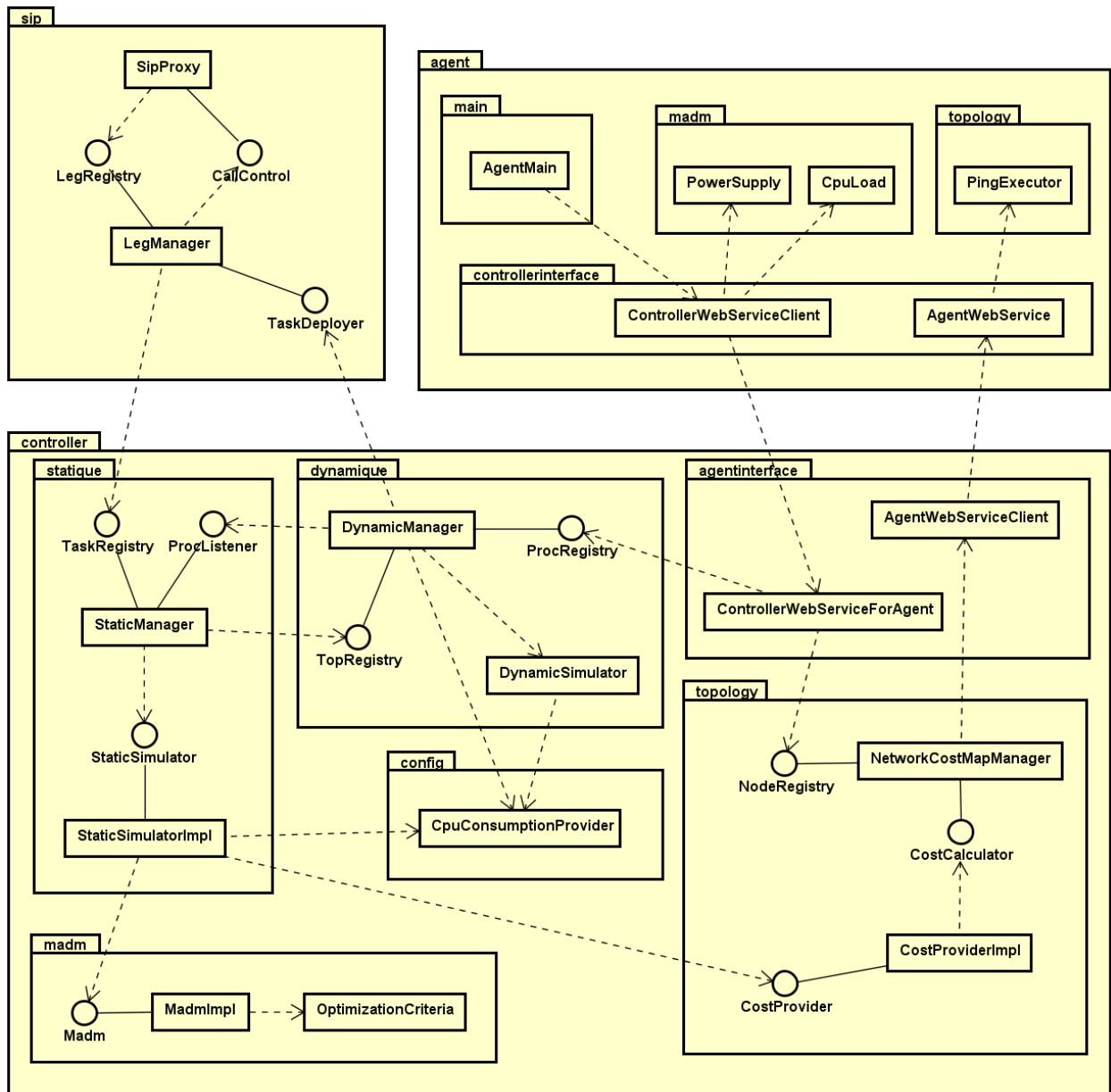
Figure A.1: Packages, interfaces and classes structure
