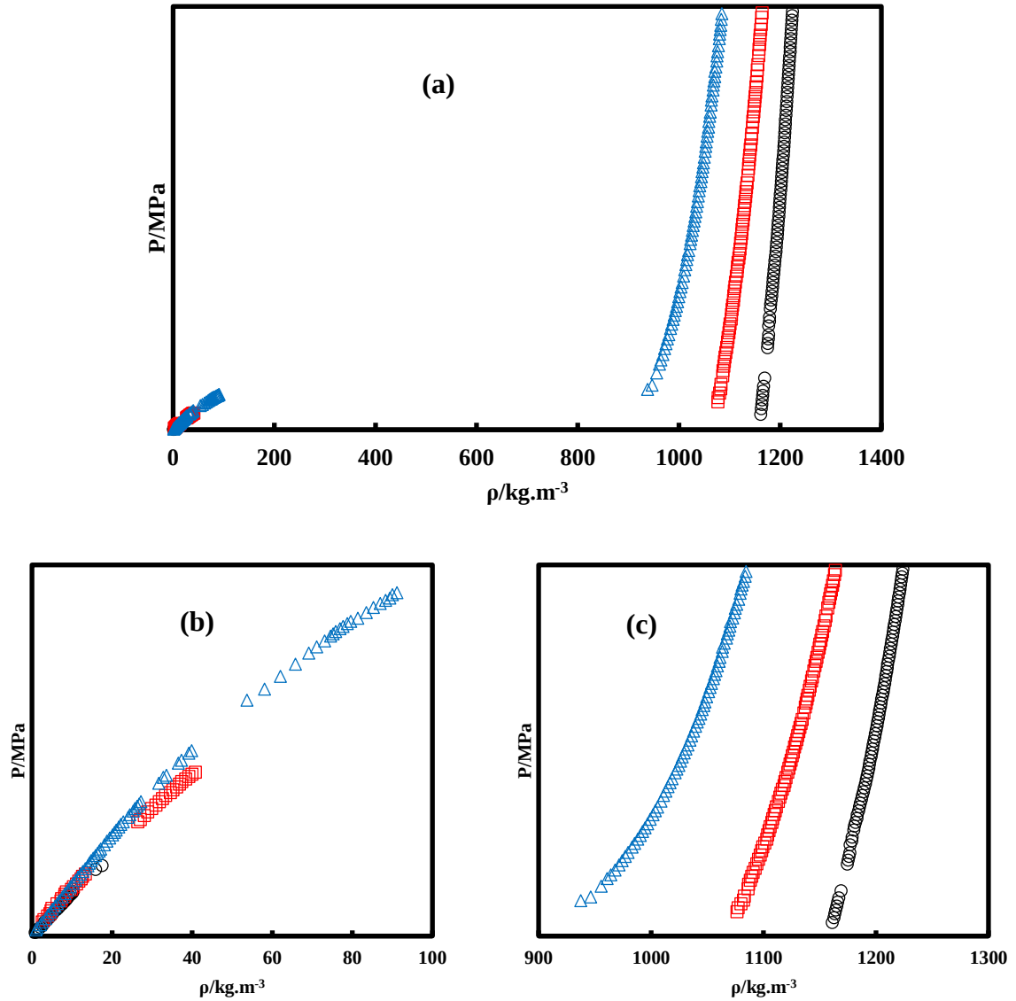
Figure 3.27 Experimental densities of (R134a + R152a + R1234yf) (2 nd composition). (a): Both phases. (b): Vapour phase. (c): Liquid phase. ( \circ ): 278.15 K; ( \square ): 303.15 K; ( \triangle ): 333.15 K. U(T) = 0.04 K; U(P) = 0.007 MPa; U(\rho^V)/\rho^V = 2\% ; U(\rho^L)/\rho^L = 0.2\% .
