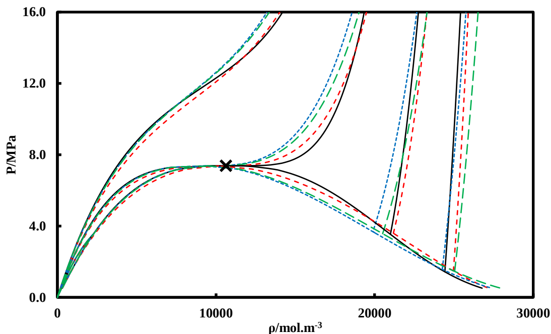
Figure 5.8 P- \rho diagram out of saturation for CO 2 . (—) REFPROP; (×) Critical Point: REFPROP ( T_c=304.13\text{K} ); (---) NéoS; (.....) PT-EoS; (- - -) PR-EoS. Out of saturation: T_r = 0.8, 0.9, 1.0 , and 1.1 .
