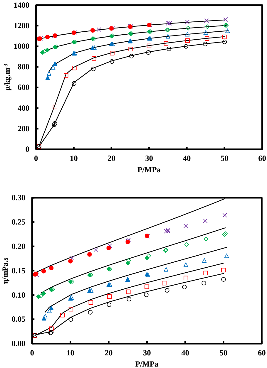
Figure 8.10 Densities and viscosities of the R1234yf. This work: (x) 303.65 K; (◇) 333.20 K; (△) 362.71 K; (□) 394.16 K; (○) 423.06 K. (Meng et al. 2013): (●) 303.15 K; (◆) 333.16 K; (▲) 363.16 K. (—) REFPROP 9.0 (Lemmon et al. 2010).
