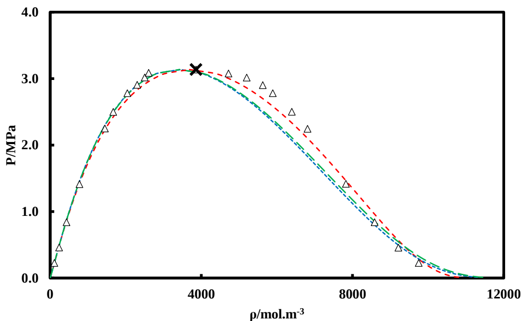
Figure 5.4 P- \rho diagram at saturation for R1216. ( \Delta ) Experimental data (Coquelet et al. 2010); ( \times ) Critical Point: Experimental ( T_c=358.9 K) (Coquelet et al. 2010); (---) NEdS; (.....) PT-EoS; (—) PR-EoS.
