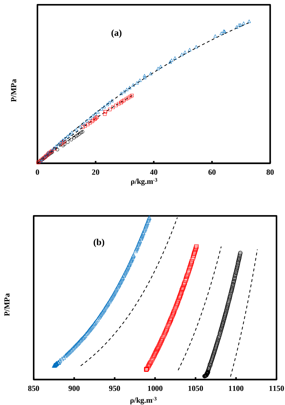
Figure 6.29 Density prediction for (R1234yf + R152a), 1 st composition. (a): Vapour phase. (b): Liquid phase. (○): 278.15 K; (□): 303.15 K; (△): 333.15 K; (- - -) N 2 O 2 S.
