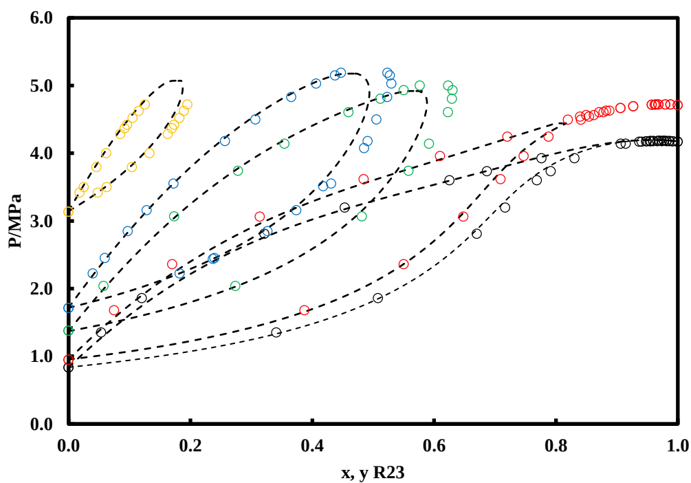
Figure 6.25 VLE prediction for binary mixture (R23 + Propane). ( \circ ) 293.15 K; ( \circ ) 298.15 K; ( \circ ) 313.15 K; ( \circ ) 323.15 K; ( \circ ) 353.15 K; (---) NéoS.
