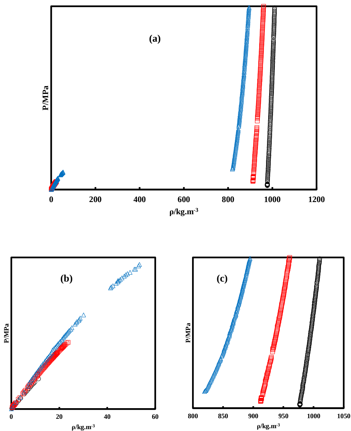
Figure 3.25 Experimental densities of R1234yf + R152a (3 rd composition). (a): Both phases; (b): Vapour phase; (c): Liquid phase. ( \circ ): 278.15 K; ( \square ): 303.15 K; ( \triangle ): 333.15 K. U(T) = 0.04 K; U(P) = 0.007 MPa; U(\rho^V)/\rho^V = 2\% ; U(\rho^L)/\rho^L = 0.2\% .
