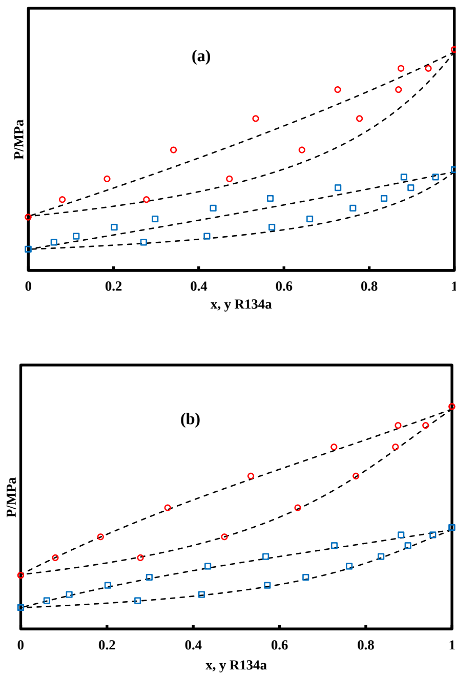
Figure 6.14 VLE prediction for binary mixture (R134a + R1233zd(E)). (a): With k_{ij} = 0 . (b): With k_{ij} adjusted. ( \square ) 303.07 \text{ K} ; ( \circ ) 333.23 \text{ K} ; (---) N 2 O-S.
