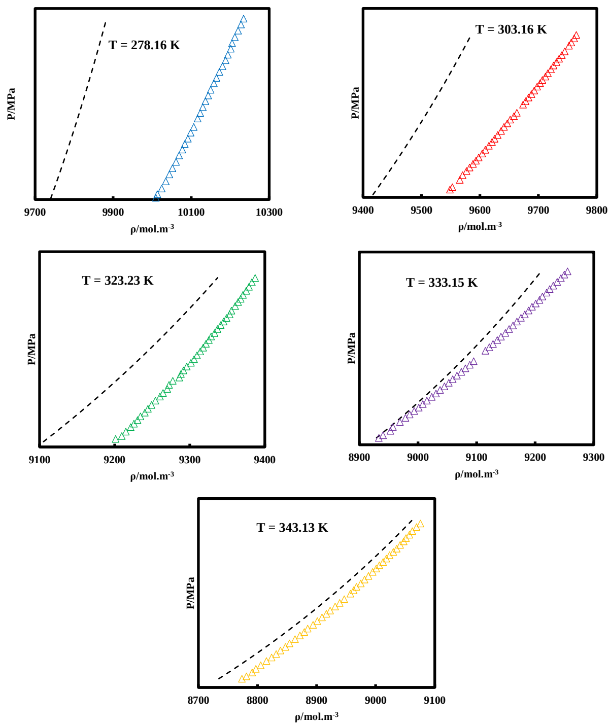
Figure 5.22 Liquid density prediction for pure compound R1233zd(E). (Δ) Experimental data; (- - -) N EOS.
