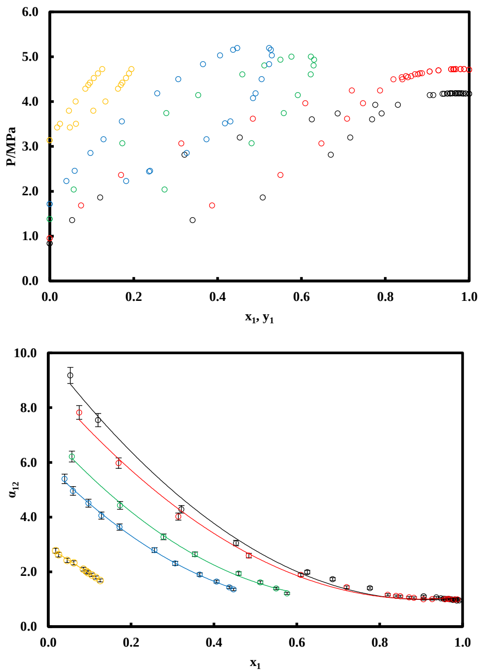
Figure 3.17 VLE results and relative volatility for R23 (1) + Propane (2). ( \circ ) 293.15 K; ( \odot ) 298.15 K; ( \oplus ) 313.15 K; ( \oplus ) 323.15 K; ( \triangle ) 353.15 K. U(T) = 0.08 K; U(P) = 0.0008 MPa; U(x_1) = 0.009 ; U(y_1) = 0.009 . Error bars: \pm 3.2\% .
