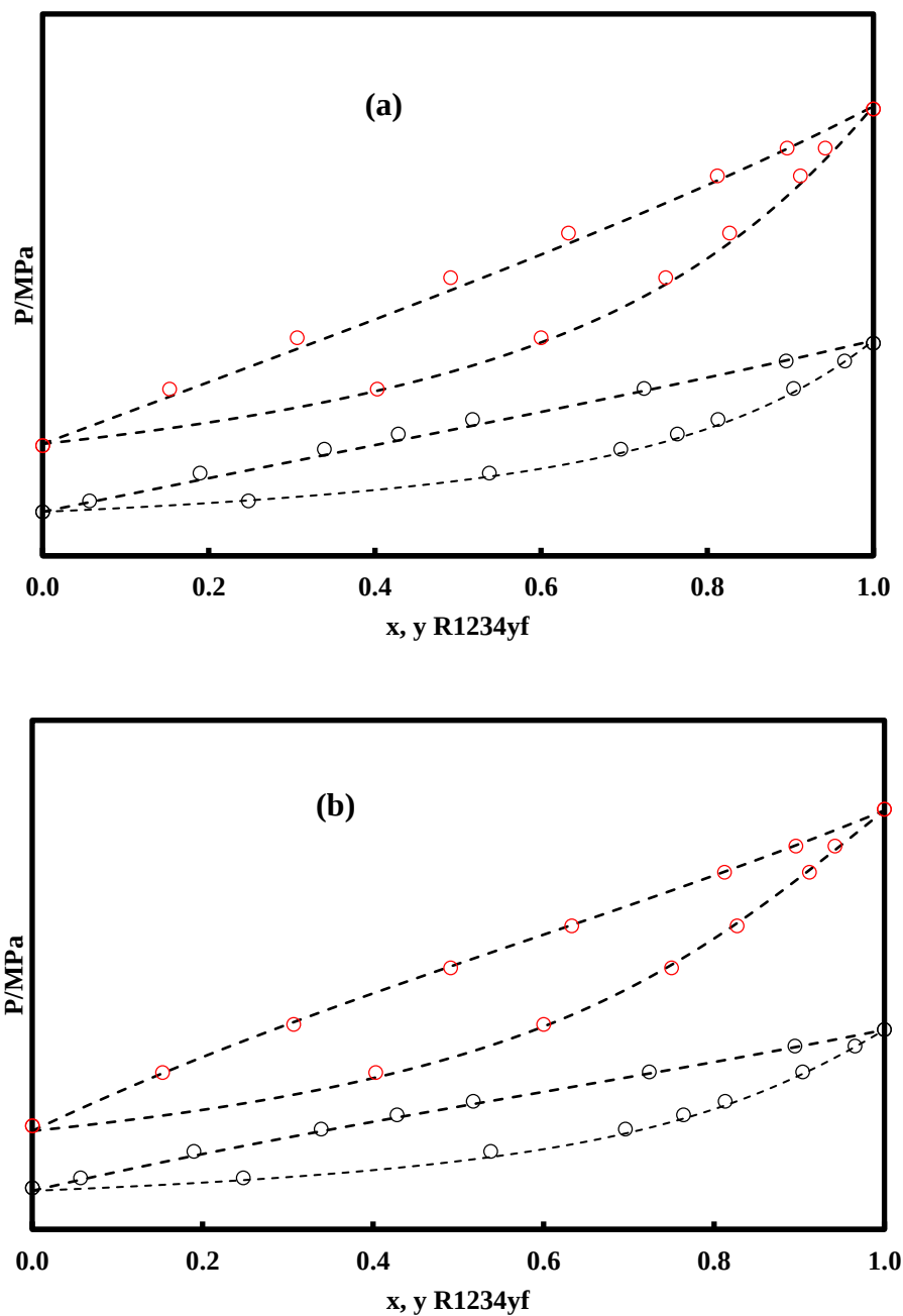
Figure 6.18 VLE prediction for binary mixture (R1234yf + R1233zd(E)). (a): With predictive parameters. (b): With adjusted parameters. ( \circ ) 303.22 \text{ K} ; ( \circ ) 333.27 \text{ K} ; (---) N EoS.
