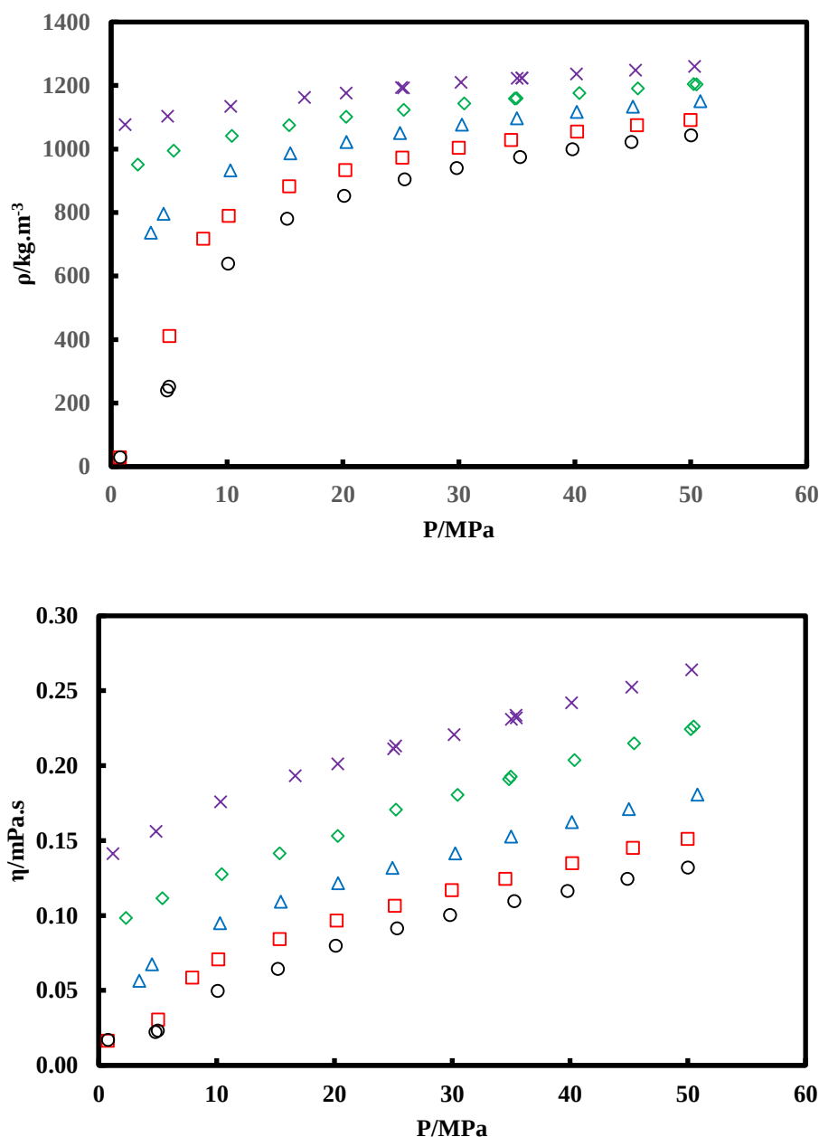
Figure 8.8 Experimental densities and viscosities for the R1234yf. (×) 303.65 K; (◇) 333.20 K; (△) 362.71 K; (□) 394.16 K; (○) 423.06 K. U(T) = 0.1 K; U(P) = 0.05 MPa; U(\rho)/\rho = 0.2\% ; U(\eta)/\eta = 2\% .
