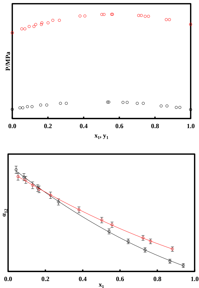
Figure 3.15 VLE results and relative volatility for R245fa (1) + R1233xf (2). (○) 323.40 K; (◐) 353.27 K. U(T) = 0.08 K; U(P) = 0.0004 MPa; U(x_1) = 0.0086 ; U(y_1) = 0.0085 . Error bars: \pm 1.8\% .
