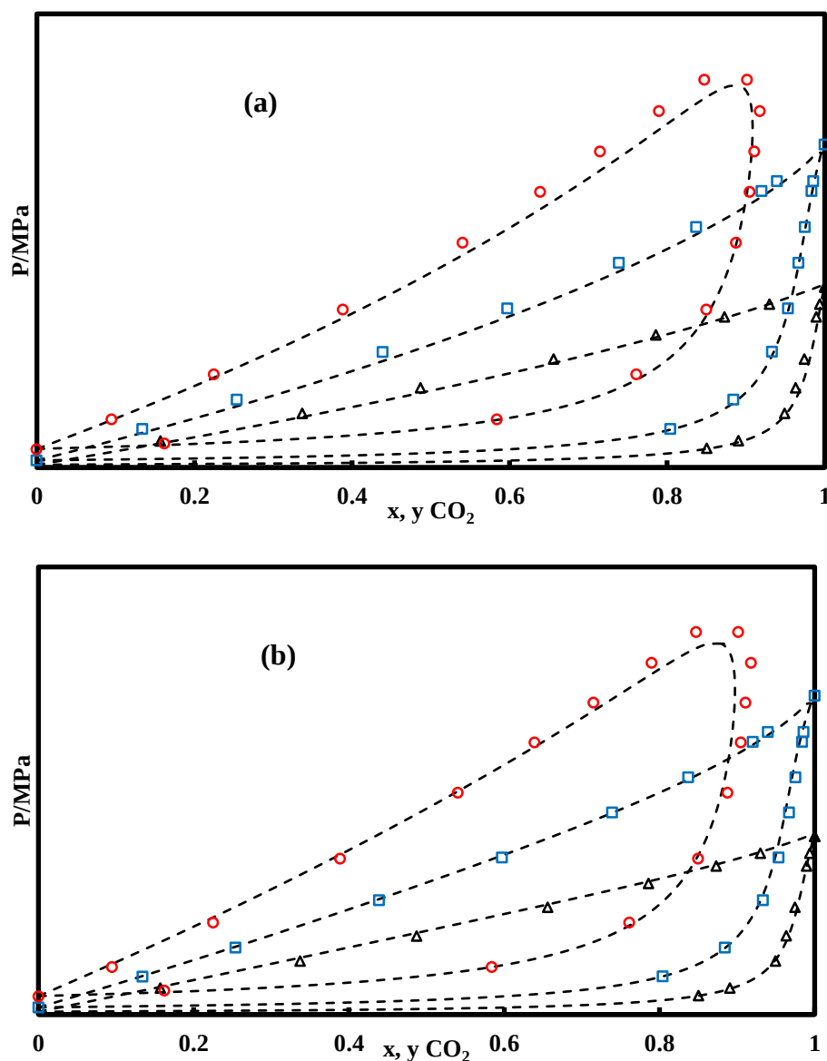
Figure 6.20 VLE prediction for binary mixture (CO 2 + R1233zd(E)). (a): With k_{ij} = 0 . (b): With k_{ij} = 0.0285 . ( \Delta ) 278.18 K; ( \square ) 303.16 K; ( \circ ) 333.29 K; (---) NEOS.
