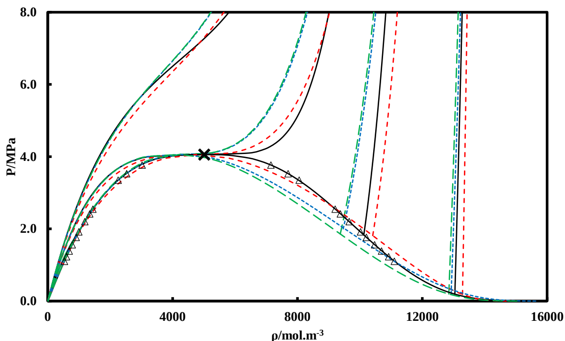
Figure 5.9 P- \rho diagram out of saturation for R134a. (Δ) Experimental data (Niesen et al. 1994); (—) REFPROP; (×) Critical Point: REFPROP ( T_c=374.21\text{K} ); (---) NéoS; (.....) PT-EoS; (- - -) PR-EoS. Out of saturation: T_r = 0.7, 0.9, 1.0 , and 1.1 .
