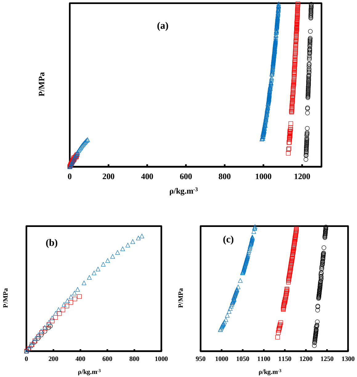
Figure 3.20 Experimental densities of R1234yf + R134a (1 st composition). (a): Both phases; (b): Vapour phase; (c): Liquid phase. ( \circ ): 278.34 K; ( \square ): 302.45 K; ( \triangle ): 332.55 K. U(T) = 0.04 K; U(P) = 0.007 MPa; U(\rho^V)/\rho^V = 2\% ; U(\rho^L)/\rho^L = 0.2\% .
