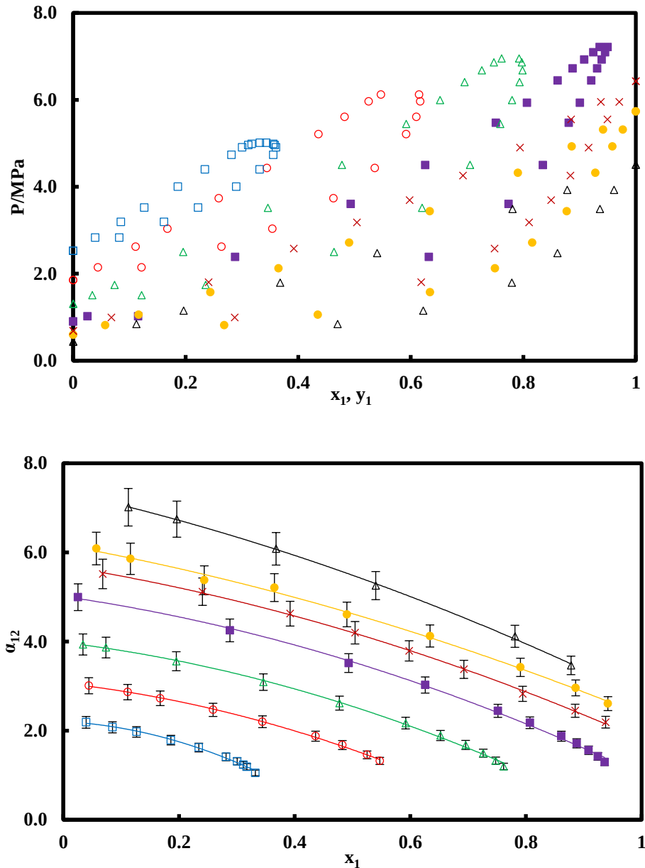
Figure 3.11 VLE results and relative volatility for CO 2 (1) + R1234yf (2). ( \Delta ) 283.21 K; ( \bullet ) 293.18 K; ( \times ) 298.11 K; ( \blacksquare ) 308.20 K; ( \triangle ) 323.18 K; ( \circ ) 338.24 K; ( \square ) 353.25 K. U(T) = 0.06 K; U(P) = 0.0008 MPa; U(x_1) = 0.008 ; U(y_1) = 0.008 . Error bars: \pm 6\% .
