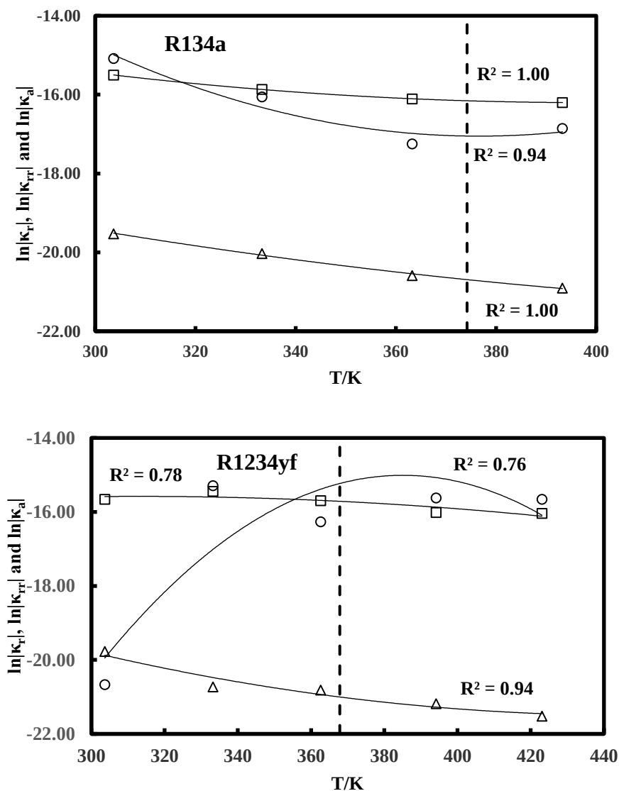
Figure 8.14 Parameters \ln|\kappa_r| , \ln|\kappa_{rr}| and \ln|\kappa_a| in function of the temperature. ( \circ ) \ln|\kappa_r| ; ( \triangle ) \ln|\kappa_{rr}| ; ( \square ) \ln|\kappa_a| ; (---) Critical temperature: 374.21 K for R134a and 367.85 K for R1234yf.
