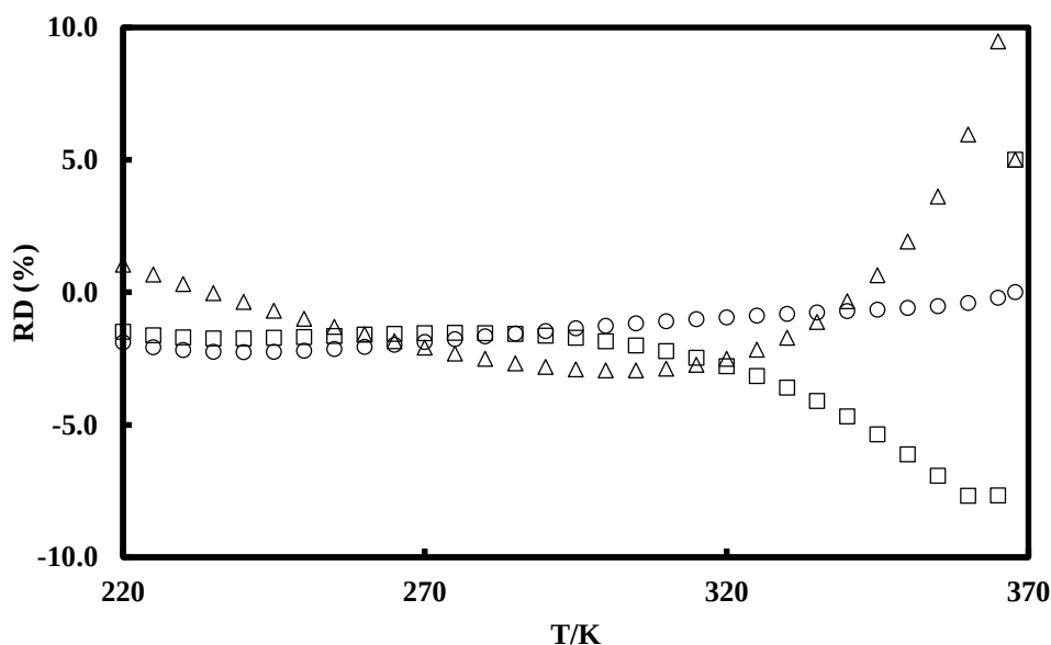
Figure 5.2 Relative deviation (RD) for R1234yf with NEdS using the calculated parameters. (○) RD of vapour pressure; (Δ) RD of saturated liquid density; (□) RD of saturated vapour density.
