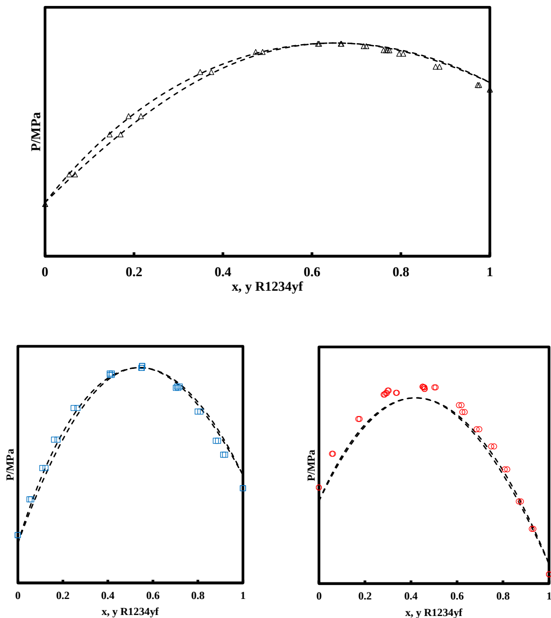
Figure 6.21 VLE prediction for binary mixture (R1234yf + R134a). ( \Delta ) 278.17 K; ( \square ) 303.16 K; ( \circ ) 333.17 K; (- - -) NEoS.
