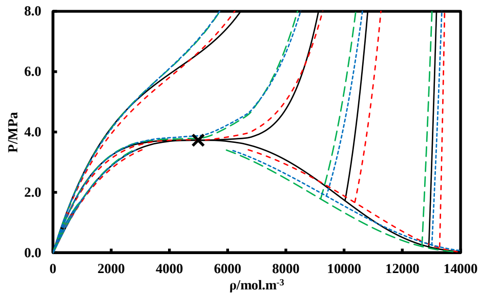
Figure F.5 P- \rho diagram for ternary mixture R-404A. (—) REFPROP; (x) Critical Point: REFPROP ( T_c=345.2\text{K} ); (- - -) NéoS; (.....) PT-EoS; (- . -) PR-EoS. Out of saturation: T_r = 0.7, 0.9, 1.0, 1.1 .
