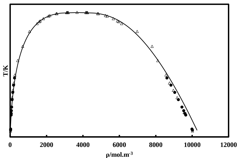
Figure 7.7 T- \rho diagram for R-1233zd(E). (Δ) This work; (●) (Kondou et al. 2015); (—) Correlation.
