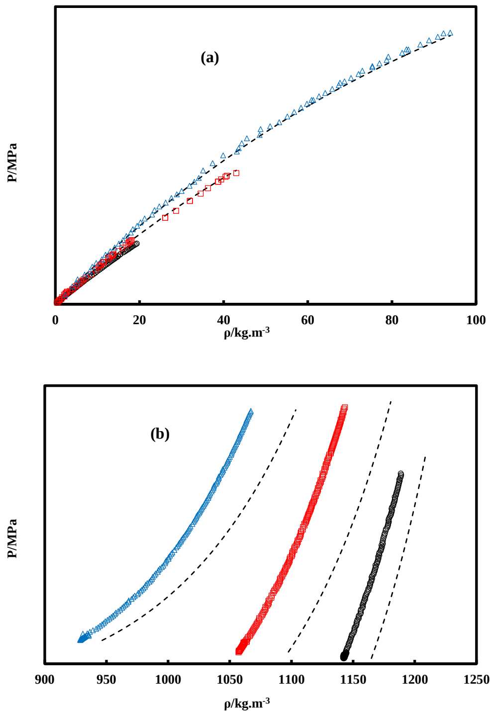
Figure 6.30 Density prediction for (R1234yf + R152a), 2 nd composition. (a): Vapour phase. (b): Liquid phase. (○): 278.15 K; (□): 303.15 K; (△): 333.15 K; (---) NEdS.
