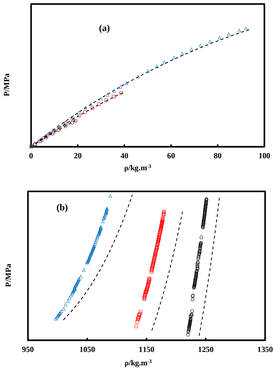
Figure 6.26 Density prediction for (R1234yf + R134a), 1 st composition. (a): Vapour phase. (b): Liquid phase. ( \circ ): 278.34 K; ( \square ): 302.45 K; ( \triangle ): 332.55 K; (- - -) NEdS.
