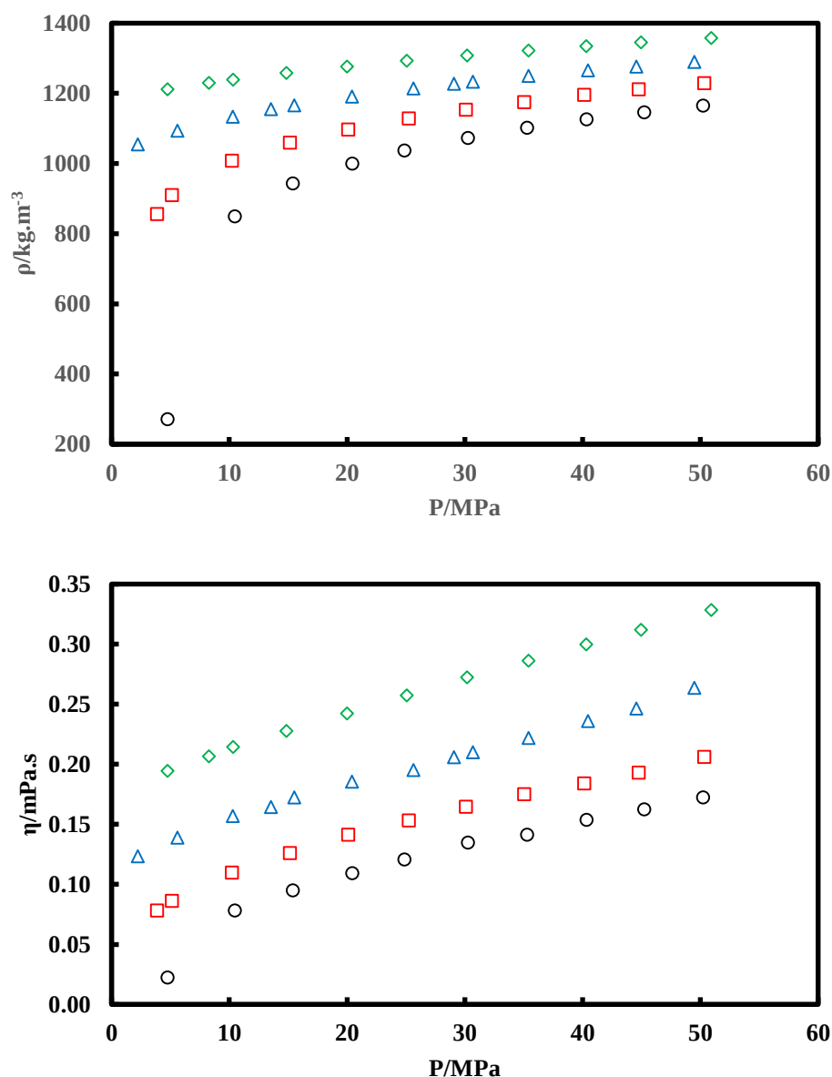
Figure 8.7 Experimental densities and viscosities for the R134a. ( \diamond ) 303.67 K; ( \triangle ) 333.27 K; ( \square ) 363.27 K; ( \circ ) 393.26 K. U(T) = 0.1 K; U(P) = 0.05 MPa; U(\rho)/\rho = 0.2\% ; U(\eta)/\eta = 2\% .
