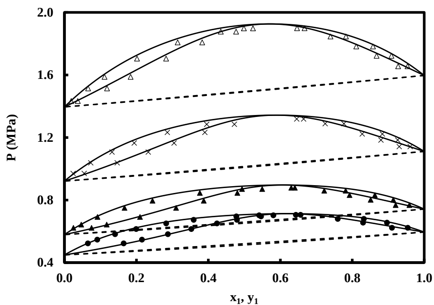
Figure 6.6 VLE prediction for Isopentane (1) + R365mfc (2). Experimental data (ElAhmar et al. 2012): (●) 363.12 K; (▲) 373.20 K; (×) 393.22 K; (Δ) 413.09 K. NEEoS: (---) k_{ij} = 0 ; (—) k_{ij} adjusted.
