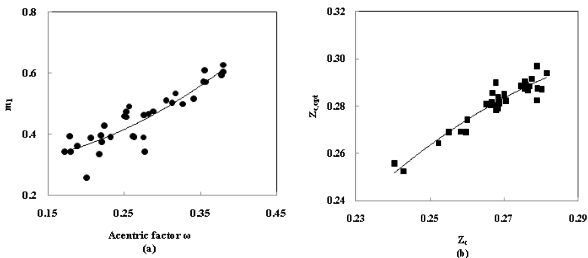
Figure F.2 Correlations obtained with the N EOS. (a): the parameter m_1 as a function of the acentric factor \omega (coefficient of determination R^2 = 0.82 ); (b): the optimized critical compressibility factor Z_{c,opt} as a function of the experimental critical compressibility factor (coefficient of determination R^2 = 0.89 ).
