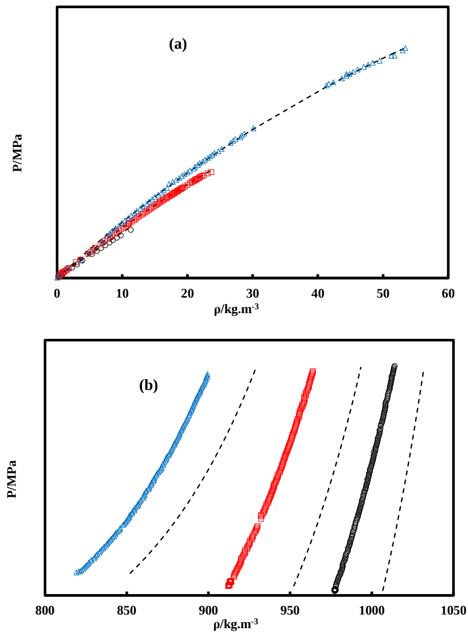
Figure 6.31 Density prediction for (R1234yf + R152a), 3 rd composition. (a): Vapour phase. (b): Liquid phase. ( \circ ): 278.15 K; ( \square ): 303.15 K; ( \triangle ): 333.15 K; (- - -) NEEoS.
