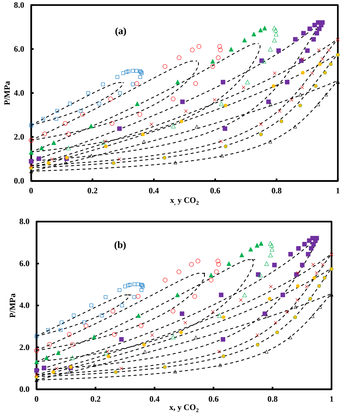
Figure 6.19 VLE prediction for the binary mixture ( \text{CO}_2 + \text{R1234yf} ). (a): With k_{ij} = 0 . (b): With an adjusted k_{ij} . ( \Delta ) 283.21 K; ( \bullet ) 293.18 K; ( \times ) 298.11 K; ( \blacksquare ) 308.20 K; ( \triangle ) 323.18 K; ( \circ ) 338.24 K; ( \square ) 353.25 K; (---) NEOs.
