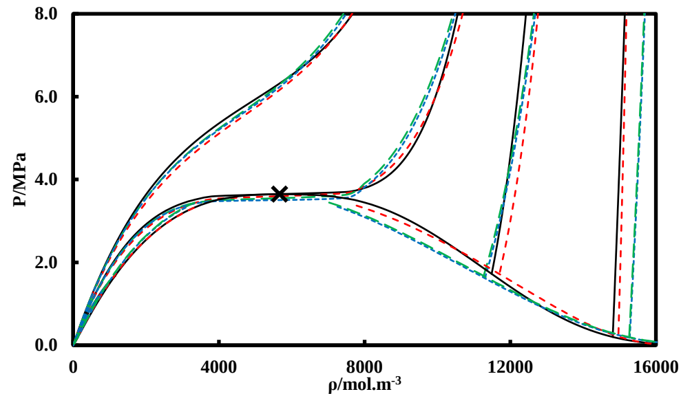
Figure F.3 P- \rho diagram for binary mixture R-508A. (—) REFPROP; (x) Critical Point: REFPROP ( T_c = 283.34\text{K} ); (- - -) NéoS; (.....) PT-EoS; (- . -) PR-EoS. Out of saturation: T_r = 0.7, 0.9, 1.0, 1.1 .
