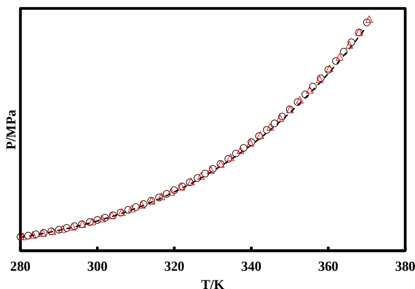
Figure 5.18 Vapour pressures of pure compound R245fa. (○) Experimental data (This work); (Δ) Experimental data (NIST); (---) N EoS .
