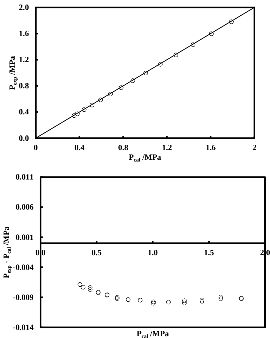
Figure 5.13 Experimental and calculated vapour pressures of the pure compound R1234yf.
