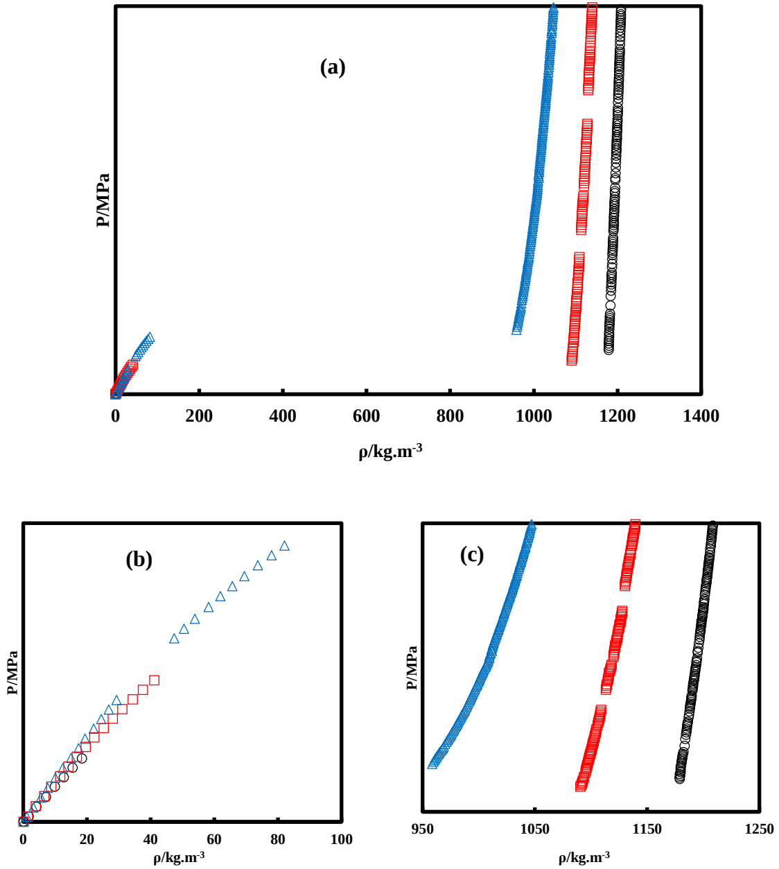
Figure 3.21 Experimental densities of R1234yf + R134a (2 nd composition). (a): Both phases; (b): Vapour phase; (c): Liquid phase. ( \circ ): 278.36 K; ( \square ): 302.74 K; ( \triangle ): 332.54 K. U(T) = 0.04 K; U(P) = 0.007 MPa; U(\rho^V)/\rho^V = 2\% ; U(\rho^L)/\rho^L = 0.2\% .
