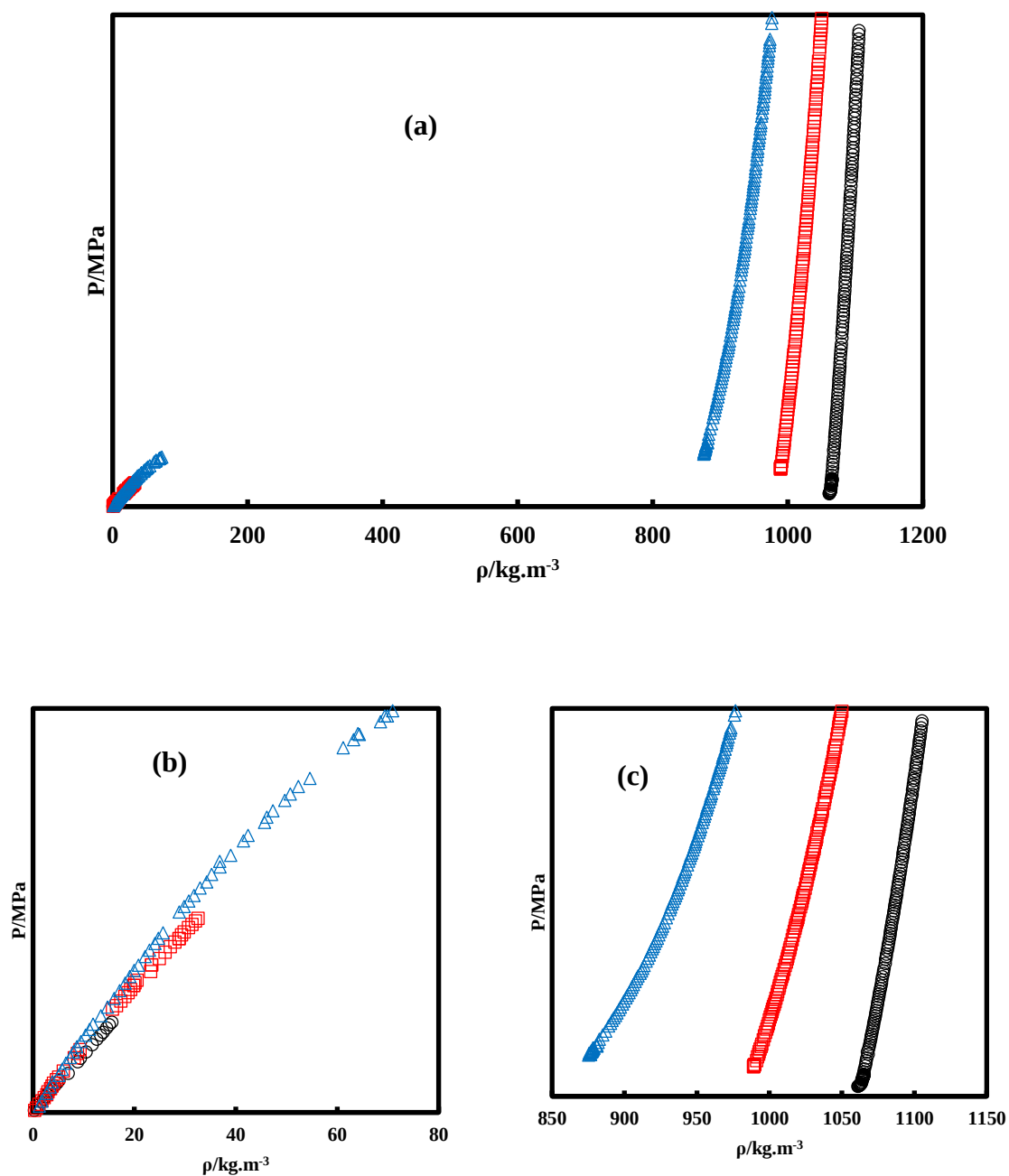
Figure 3.23 Experimental densities of R1234yf + R152a (1 st composition). (a): Both phases; (b): Vapour phase; (c): Liquid phase. ( \circ ): 278.15 K; ( \square ): 303.15 K; ( \triangle ): 333.15 K. U(T) = 0.04 K; U(P) = 0.007 MPa; U(\rho^V)/\rho^V = 2\% ; U(\rho^L)/\rho^L = 0.2\% .
