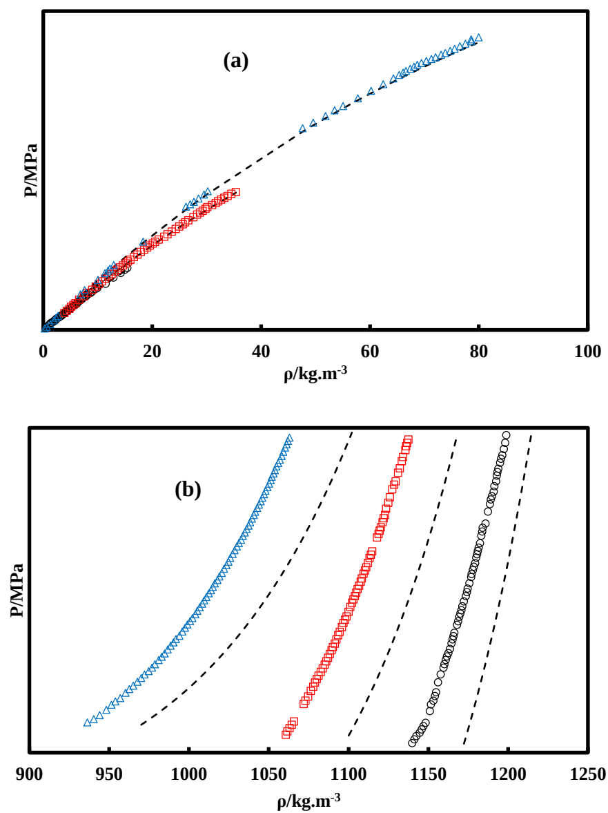
Figure 6.34 Density prediction for (R134a + R152a + R1234yf), 3 rd composition. (a): Vapour phase. (b): Liquid phase. (○): 278.15 K; (□): 303.15 K; (△): 333.15 K; (---) NEdS.
