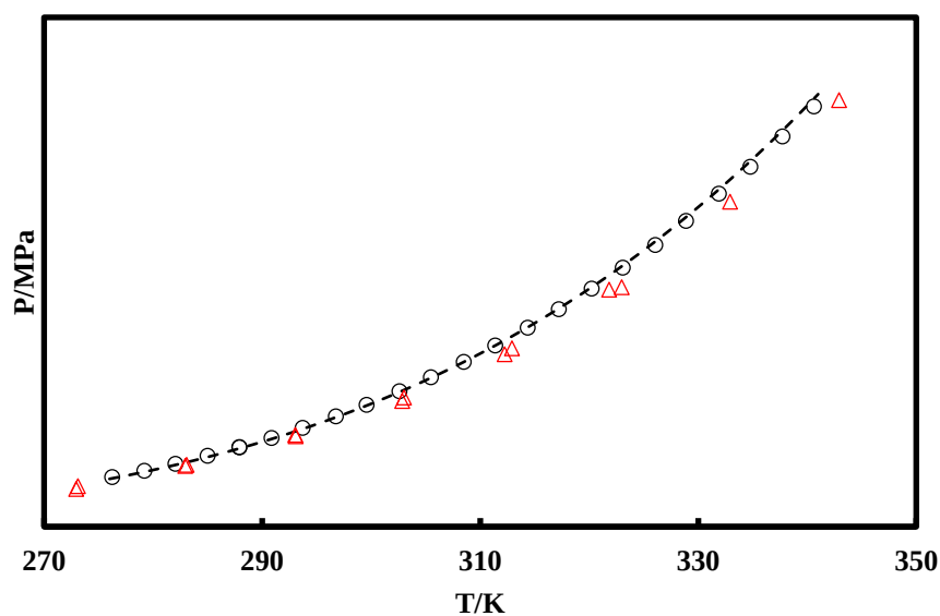
Figure 5.14 Vapour pressures of the pure compound R1233zd(E). (○) Experimental data (This work); (Δ) Experimental data (Hulse et al. 2012); (---) NéoS.
