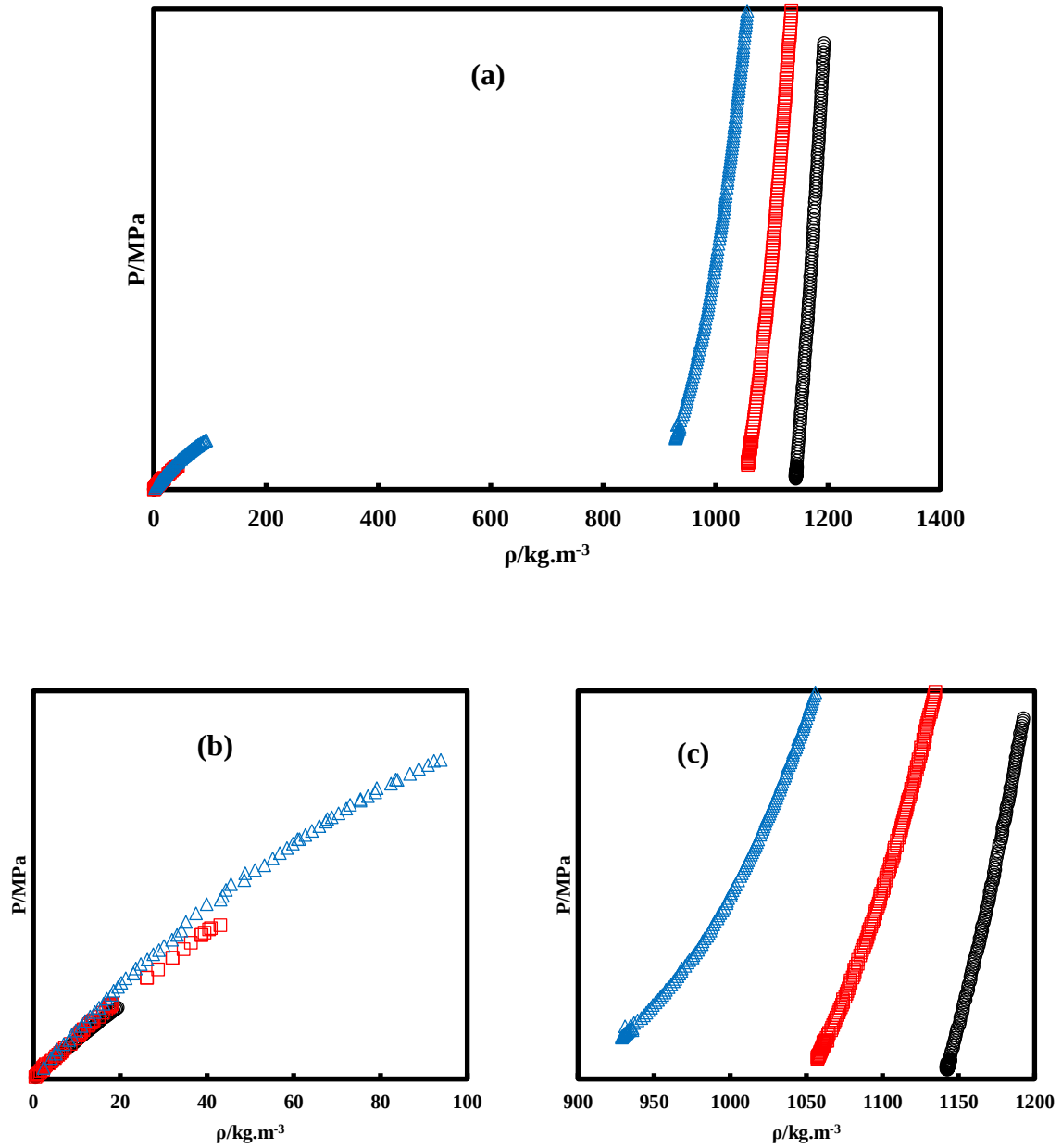
Figure 3.24 Experimental densities of R1234yf + R152a (2 nd composition). (a): Both phases; (b): Vapour phase; (c): Liquid phase. ( \circ ): 278.15 K; ( \square ): 303.15 K; ( \Delta ): 333.15 K. U(T) = 0.04 K; U(P) = 0.007 MPa; U(\rho^V)/\rho^V = 2\% ; U(\rho^L)/\rho^L = 0.2\% .
