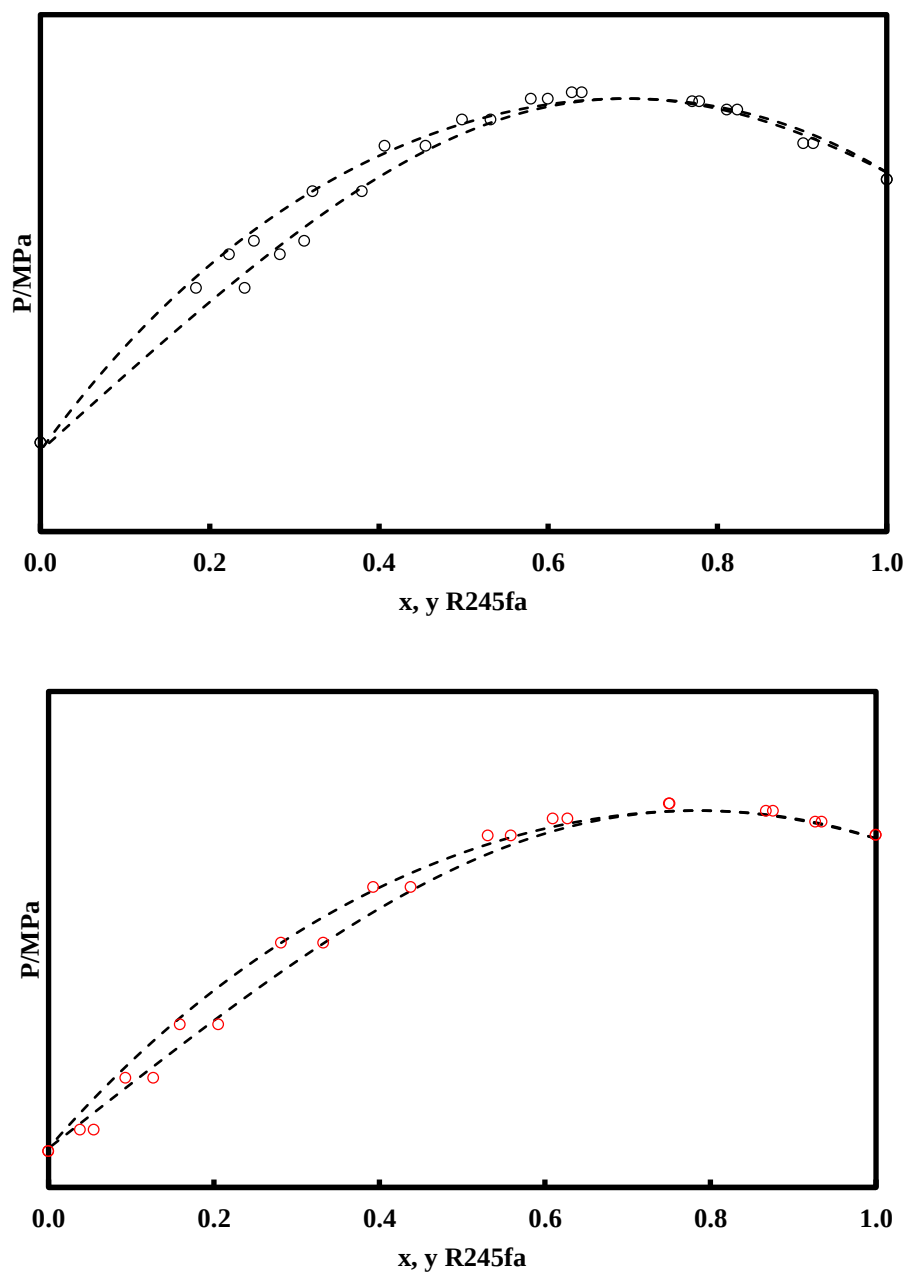
Figure 6.24 VLE prediction for binary mixture (R245fa + R1233zd(E)). (○) 323.23 K; (○) 353.27 K; (---) N EOS.
