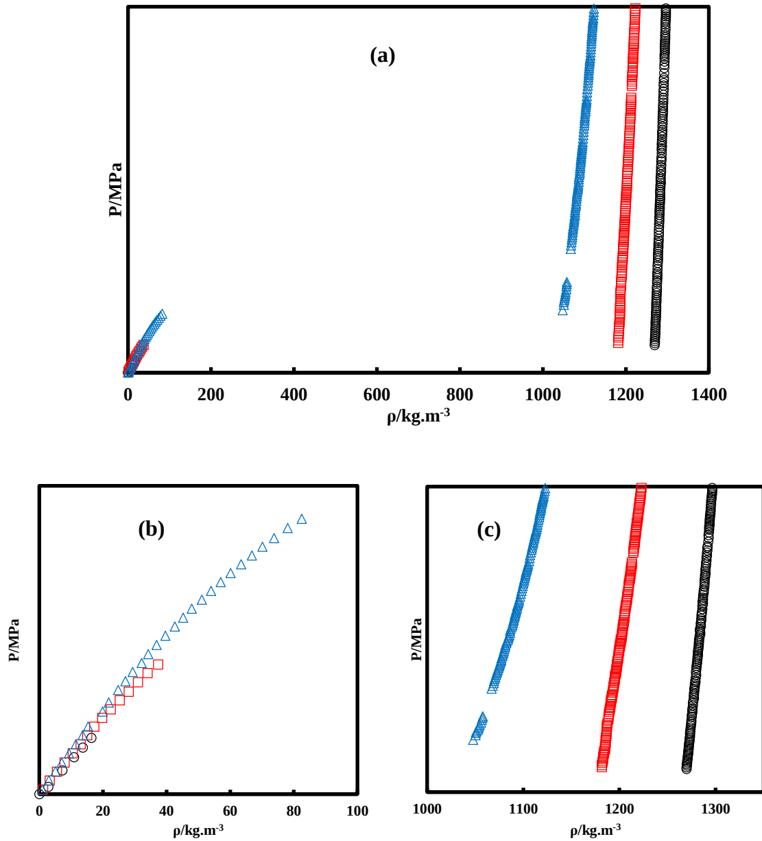
Figure 3.22 Experimental densities of R1234yf + R134a (3 rd composition). (a): Both phases; (b): Vapour phase; (c): Liquid phase. ( \circ ): 278.40 K; ( \square ): 302.93 K; ( \triangle ): 332.53 K. U(T) = 0.04 K; U(P) = 0.007 MPa; U(\rho^V)/\rho^V = 2\% ; U(\rho^L)/\rho^L = 0.2\% .
