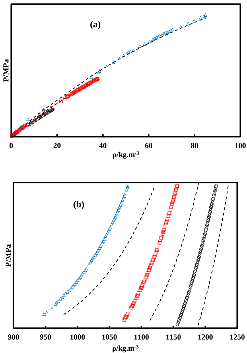
Figure 6.32 Density prediction for (R134a + R152a + R1234yf), 1 st composition. (a): Vapour phase; (b): Liquid phase. (○): 278.15 K; (◻): 303.15 K; (△): 333.15 K; (---) N EOS.
