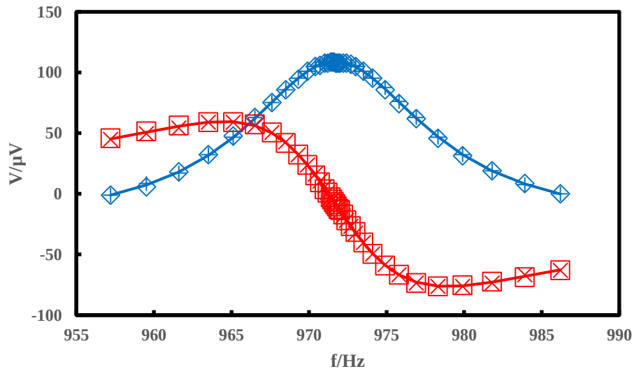
Figure 8.6 Typical response of the viscometer cell. ( \square ) In-phase voltage (up); ( \times ) In-phase voltage (down); ( \diamond ) Quadrature voltage (up); ( + ) Quadrature voltage (down), (—) Fitted in-phase voltage; (—) Fitted quadrature voltage.
