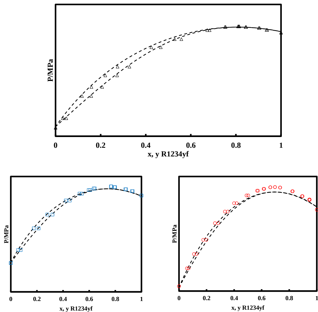
Figure 6.22 VLE prediction for binary mixture (R1234yf + R152a). ( \Delta ) 278.18 K; ( \square ) 303.16 K; ( \circ ) 333.29 K; (---) NEEoS.
