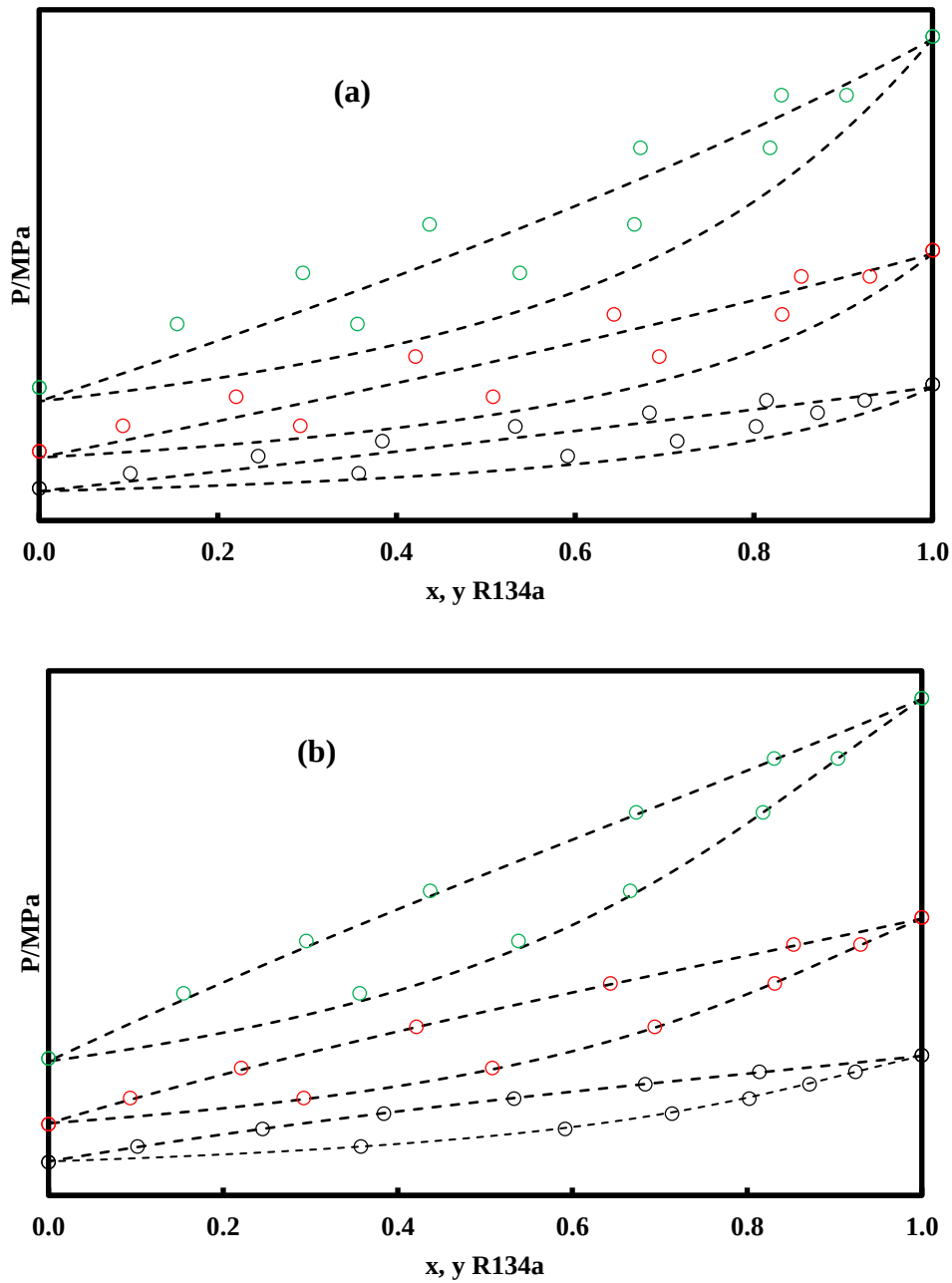
Figure 6.16 VLE prediction for binary mixture (R134a + R1233xf). (a): With predictive parameters. (b): With adjusted parameters. (○) 298.30 K; (○) 323.38 K; (○) 348.27 K; (---) NEOs.
