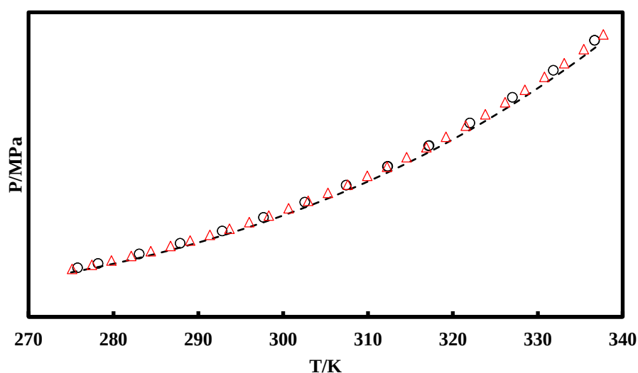
Figure 5.10 Vapour pressures of pure compound R152a. ( \circ ) Experimental data (This work); ( \Delta ) Experimental data (NIST); (---) NEOs.
