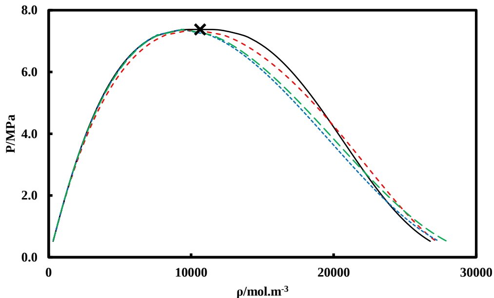
Figure 5.5 P- \rho diagram at saturation for CO 2 . (—) REFPROP; ( \times ) Critical Point: REFPROP ( T_c=304.13 K); (---) NEdS; (.....) PT-EoS; (—) PR-EoS.
