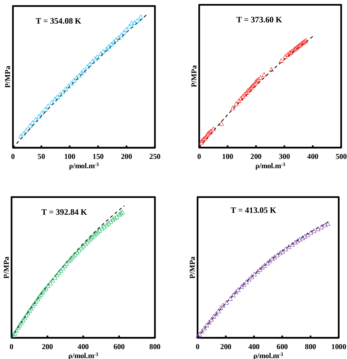
Figure C.1 Vapour densities of pure compound R1233zd(E) at high temperatures. ( \Delta ) Experimental data; (---) N EO S.
