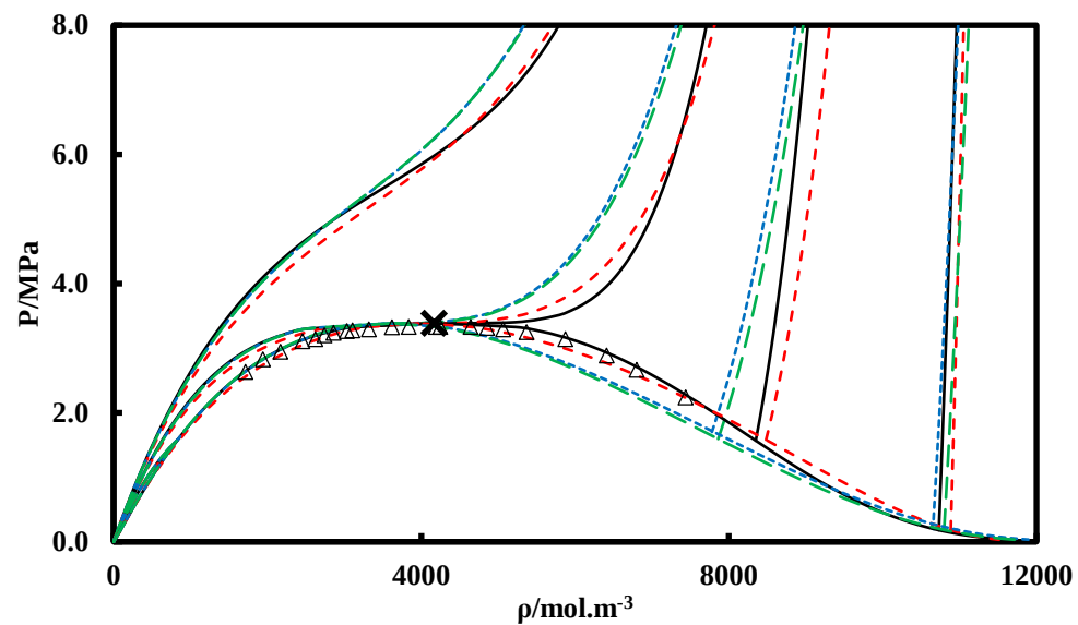
Figure F.4 P- \rho diagram for pure compound R-1234yf. ( \Delta ) (Tanaka & Higashi 2010b); (—) REFPROP; (x) Critical Point: REFPROP ( T_c = 367.85\text{K} ); (- - -) NéoS; (.....) PT-EoS; (- . -) PR-EoS. Out of saturation: T_r = 0.7, 0.9, 1.0, 1.1 .
