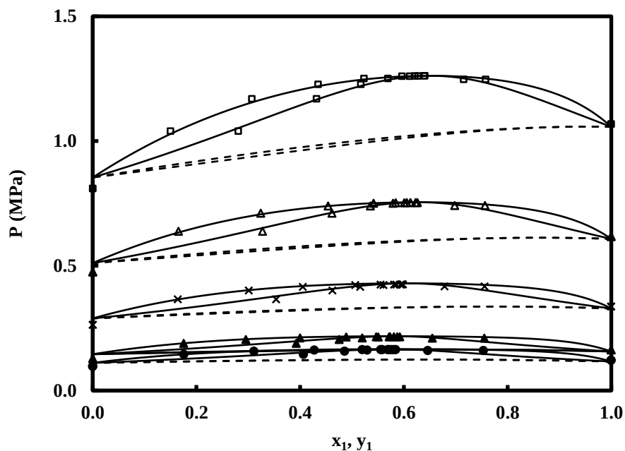
Figure 6.5 VLE prediction for R23 (1) + R116 (2). Experimental data (Zhang et al. 2008): (●) 194.33 K; (▲) 199.71 K; (×) 214.19 K; (Δ) 229.63 K; (□) 244.94 K. NEEoS: (---) k_{ij} = 0 ; (—) k_{ij} adjusted.
