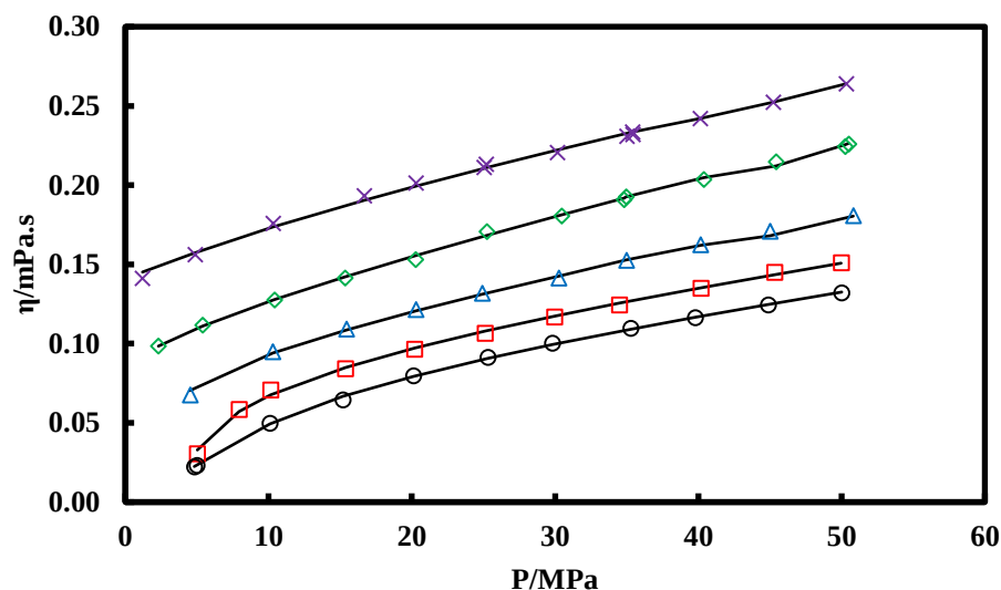
Figure 8.12 Viscosities of the R134a. This work: (◇) 303.67 K; (△) 333.27 K; (□) 363.27 K; (○) 393.26 K. (—) Friction theory model.
