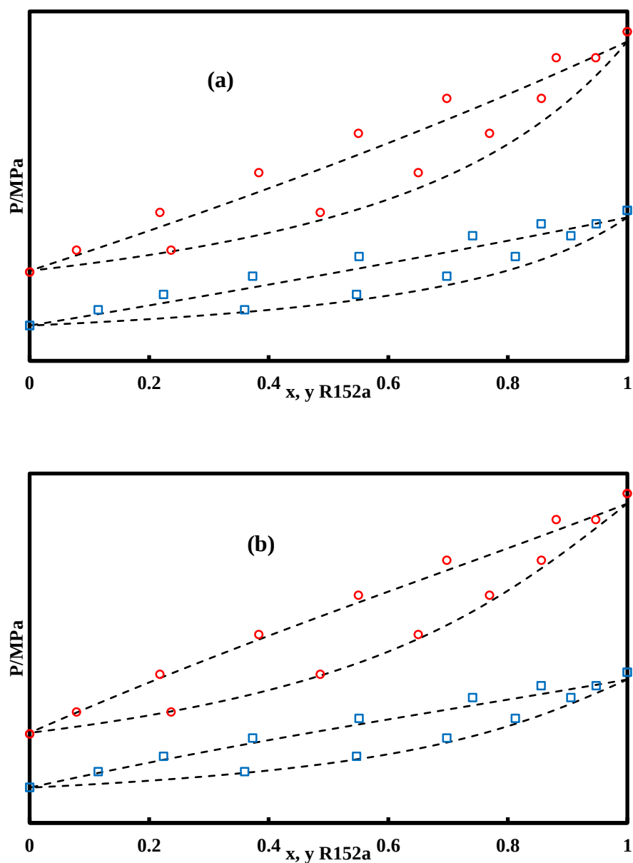
Figure 6.15 VLE prediction for binary mixture (R152a+ R1233zd(E)). (a): With k_{ij} = 0 . (b): With k_{ij} adjusted. ( \square ) 303.10 K; ( \circ ) 333.23 K.; (- - -) NRTL.
