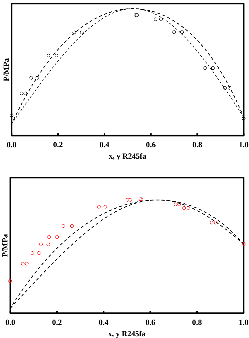
Figure 6.23 VLE prediction for binary mixture (R245fa+ R1233xf). ( \circ ) 323.40 K; ( \circ ) 353.27 K; (- - -) NéoS.
