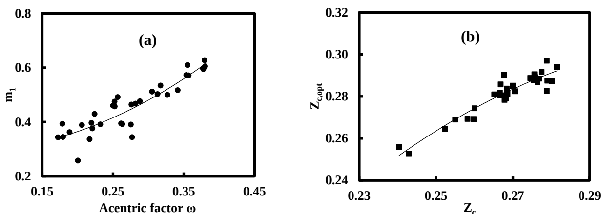
Figure 4.2 Correlations obtained with the N EOS. (a): The parameter m_1 as a function of the acentric factor \omega (coefficient of determination R^2 = 0.82 ); (b): The optimized critical compressibility factor Z_{c,opt} as a function of the experimental critical compressibility factor Z_c (coefficient of determination R^2 = 0.89 ).
