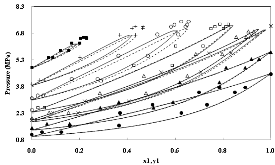
Figure F.9 VLE prediction for CO 2 (1) + R-32 (2). (Rivollet et al. 2004): (●) 283.12 K; (▲) 293.11 K; (×) 303.13 K; (Δ) 305.15 K; (□) 313.30 K; (○) 323.34 K; (+) 333.33 K; (■) 343.23 K. NEoS: (---) k_{ij} = 0 ; (—) k_{ij} adjusted.
