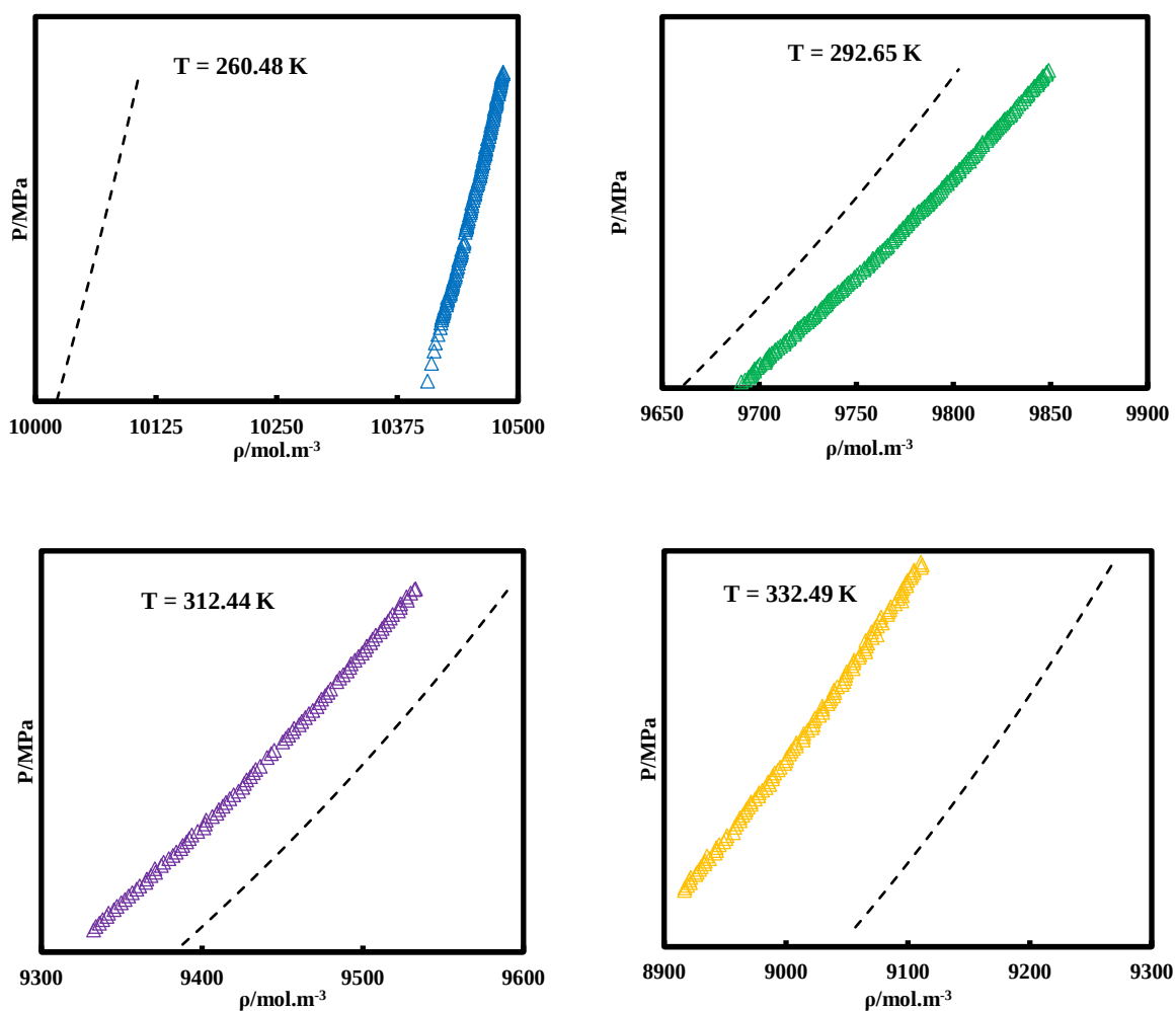
Figure 5.20 Liquid density prediction for pure compound R1233xf. (Δ) Experimental data; (- - -) NEoS.
