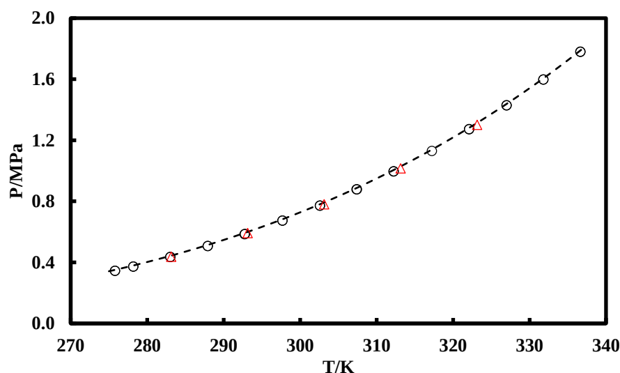
Figure 5.12 Vapour pressures of pure compound R1234yf. (○) Experimental data (This work); (Δ) Experimental data (Hu, L.-X. Chen, et al. 2013); (- - -) N EoS .
