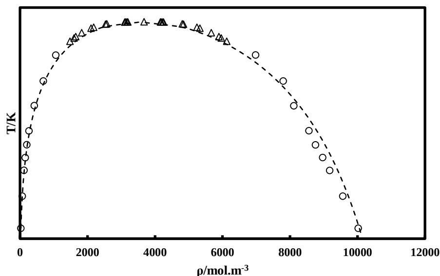
Figure C.3 Densities of pure compound R1233zd(E) at saturation. (Δ) Experimental data; (○) Data obtained using the graphical method; (---) N EOS.
