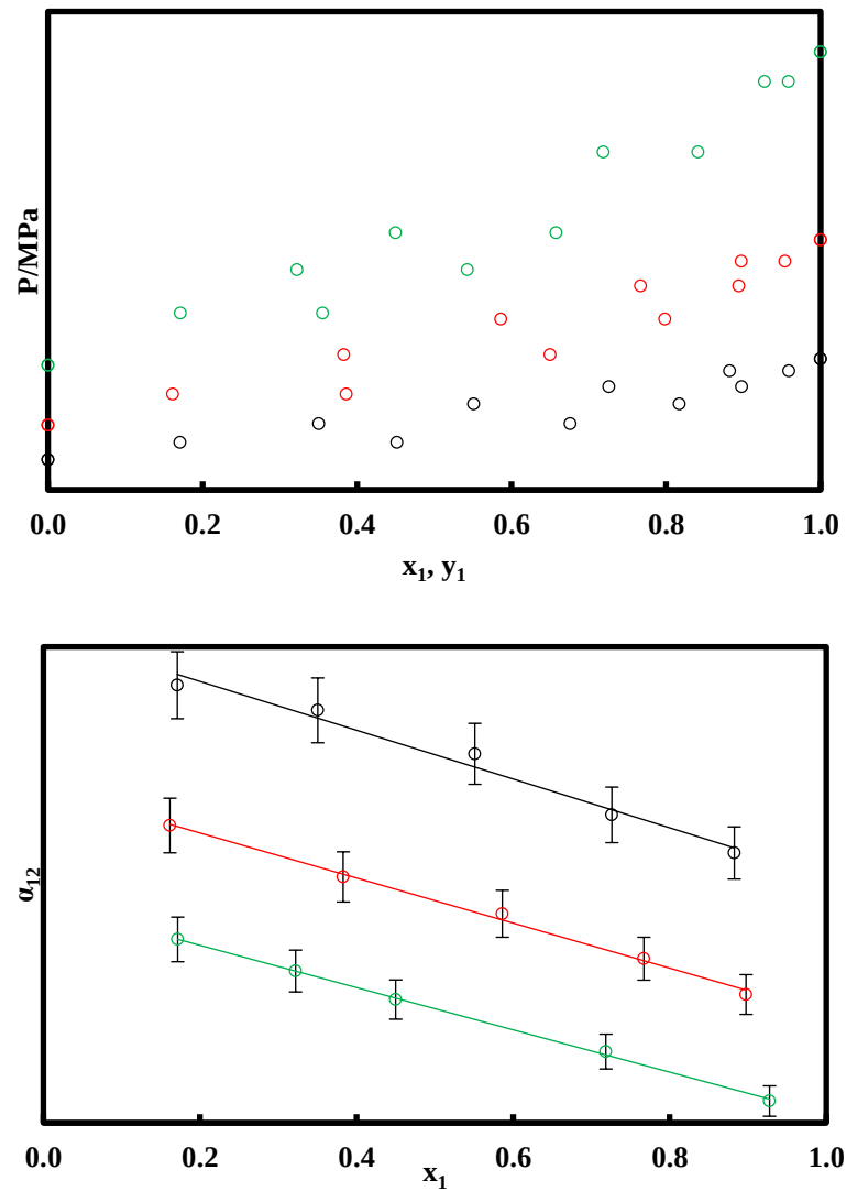
Figure 3.9 VLE results and relative volatility for R1234yf (1) + R1233xf (2). ( \circ ) 298.31 K; ( \circ ) 323.27 K; ( \circ ) 348.25 K. U(T) = 0.08 K; U(P) = 0.0005 MPa; U(x_1) = 0.0086 ; U(y_1) = 0.0087 . Error bars: \pm 4.4\% .
