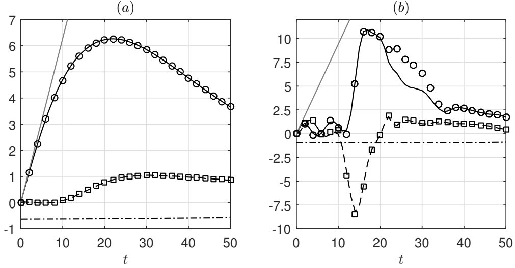
Figure 5.6: Time evolution of \partial \bar{u} / \partial z (black dash-dotted lines), \partial u^* / \partial z (black dashed lines), and \partial v^* / \partial z (black solid lines) at the vortex center x_c = 9 , y_c = 9 , z_c = l_z/2 for (a) F_h = 0.1 , k_z = \pi , and (b) F_h = 0.5 , k_z = 3\pi/2 for U_S = 0.2 and Re = 6000 . The straight grey lines represent the law k_z U_S t . The symbols show the horizontal vorticity components -\omega_x^* (circles) and \omega_y^* (squares).
