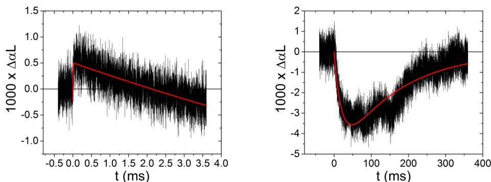
Figure 6.11: Dynamics of ns T-jump experiment on TBA G4. FWHM(probe) = 80 \mu\text{m} , FWHM(pump) = 300 \mu\text{m} , quartz cuvette, l = 100 \mu\text{m} . Left: First couple of ms, time resolution: 40 \mu\text{s} . Fit curve is in red. Decreasing time constant was fixed at 20 ms. Rising time constant was determined to be 6 \mu\text{s} . Right: First 360 ms after. First time constant was fixed at 20 ms. Relaxation time yielded 160 ms. T_{in} = 49^\circ\text{C} , \Delta T = 6^\circ\text{C} .
