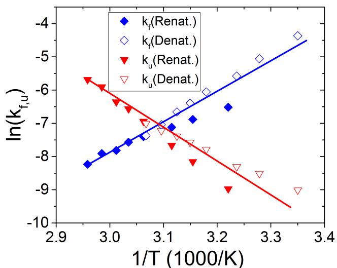
Figure 6.4: Arrhenius plot of \ln(k(T)) against 1/T . Values extracted from folding are depicted with filled dots, values from unfolding are shown with empty dots. Values of k_f are blue, values of k_u are red. Straight lines indicate tendencies.
