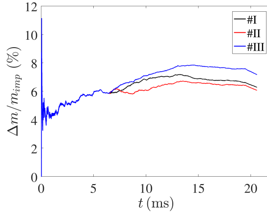
Figure 5.21: Mass deviation in the three simulation cases of multi-track deposition. Note that pass #1 is the same for all, so the 3 curves are overlaid between t = 0 and 6.5 ms.
