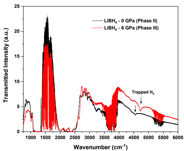
Figure S8 : IR transmission spectra of \text{LiBH}_4 before and after the phase transition II/III.
