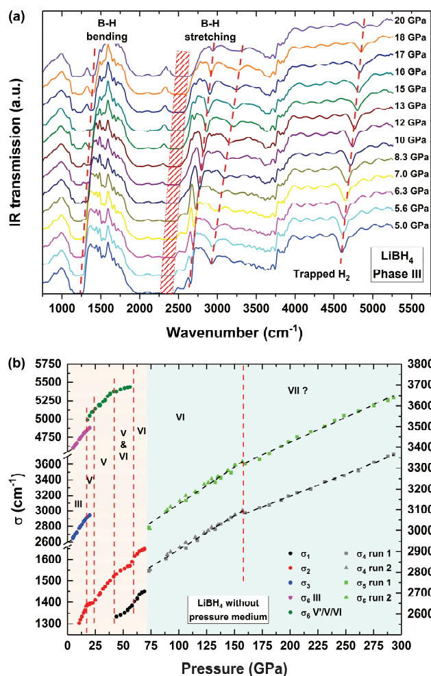
Fig. 6 (a) IR transmission spectra of \text{LiBH}_4 in phase III at selected pressures and 300 K. Followed absorption bands are indicated by red lines. Red rectangles indicate the saturated main stretching bands of \text{LiBH}_4 . (b) Pressure evolution of the followed absorption bands. The Y axis of the data in red background is on the left (single run with 300- \mu\text{m} culets) and the Y axis of the data in green background is on the right (two runs with 40- \mu\text{m} culets).
