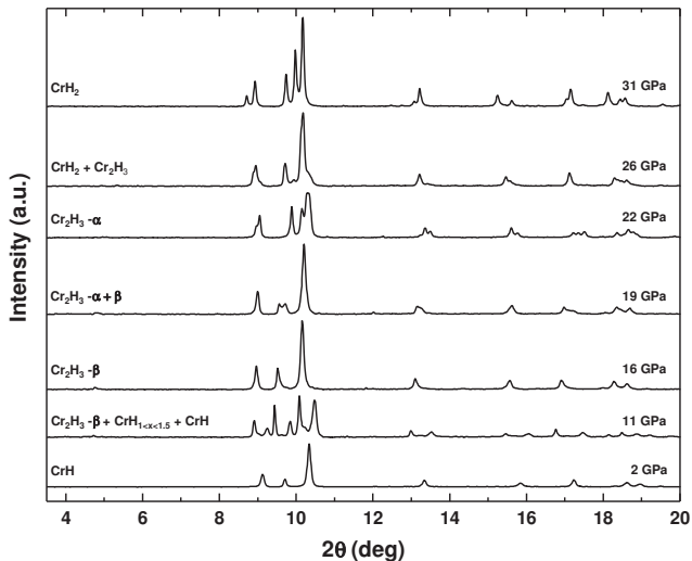
FIG. 3. Diffraction pattern during decompression of the second run with their corresponding chromium hydride phases. \lambda=0.3738 \text{ \AA} .
