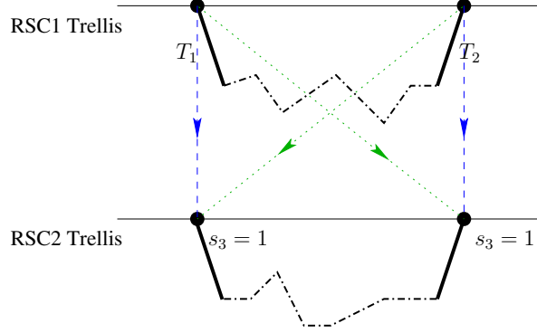
Figure 2.13: Trellis error events for input weight \omega = 2 . The two interleaving configurations are indicated. Diversity is guaranteed by full-span transitions.
