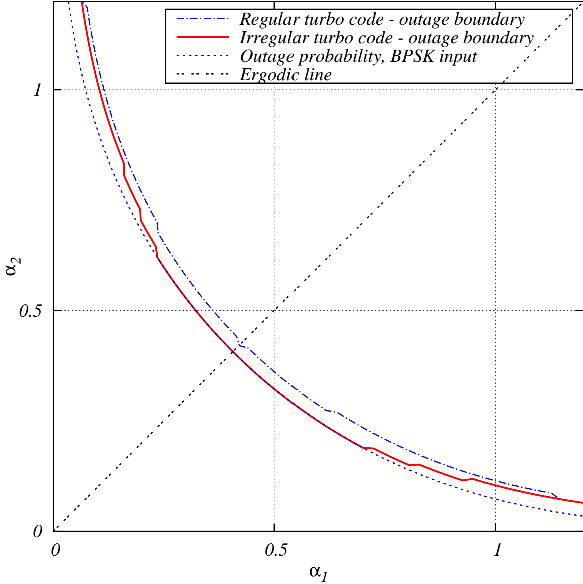
Figure 4.5: Outage boundary of regular and irregular turbo codes under h- \pi -diagonal multiplexing and with the RSC (13, 15)_8 constituent code at E_b/N_0 = 8\text{dB} . Circles filled with crosses correspond to the fading pairs in which irregular turbo codes outperform regular codes. Although the two codes have similar performance with largely unbalanced fading pairs, the irregular code outperforms the regular code in the vicinity of the ergodic line.
