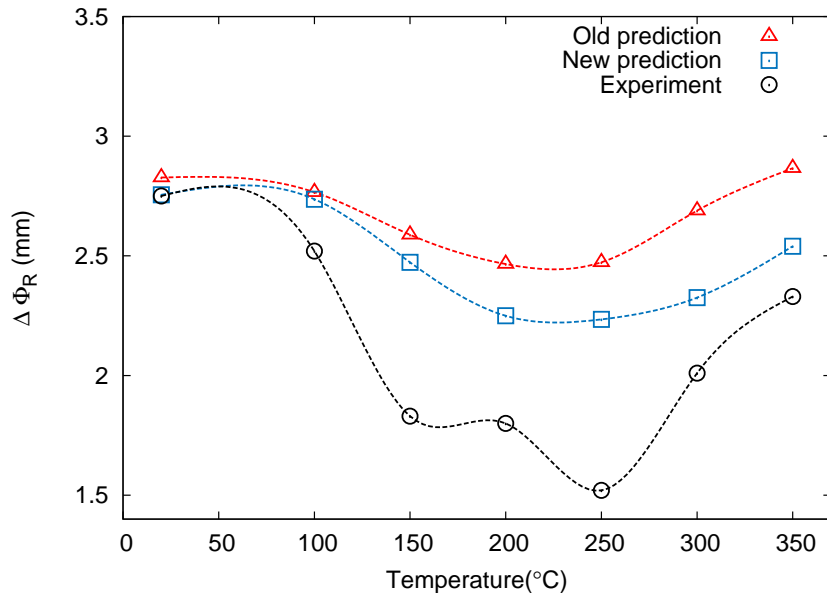
Figure A.2 – Prediction of fracture for AE4 in terms of diameter variation \Delta\phi_R : experimental measurement, old prediction by Wang [2011] and new prediction.
