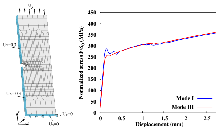
Figure 5.26 – FEM simulation of mode III loading.
