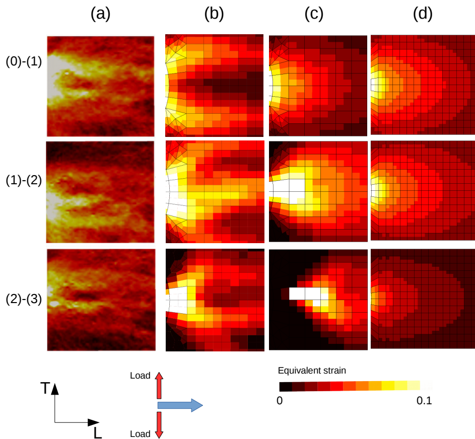
Figure A.8 – Incremental von Mises equivalent strain field in the T-L plane of ROI 2. (a) Laminography-DVC analysis at z = 0 mm [Buljac et al., 2016]; (b) Current full coupled model ( z = -0.25 mm); (c) without PLC term at z = -0.125 mm (polycrystalline+damage+Coulomb); (d) Tresca (approximated using Bron) plasticity ( z = 0 mm).
