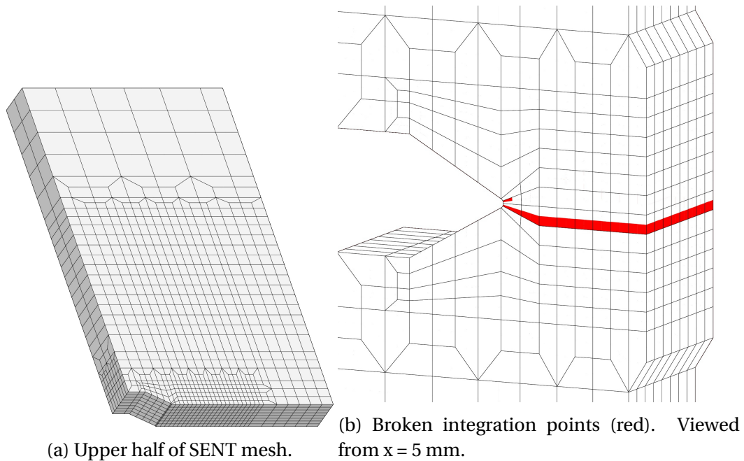
Figure 6.8 – Simulations of SENT test at 175 °C with fast nucleation and DSA.
