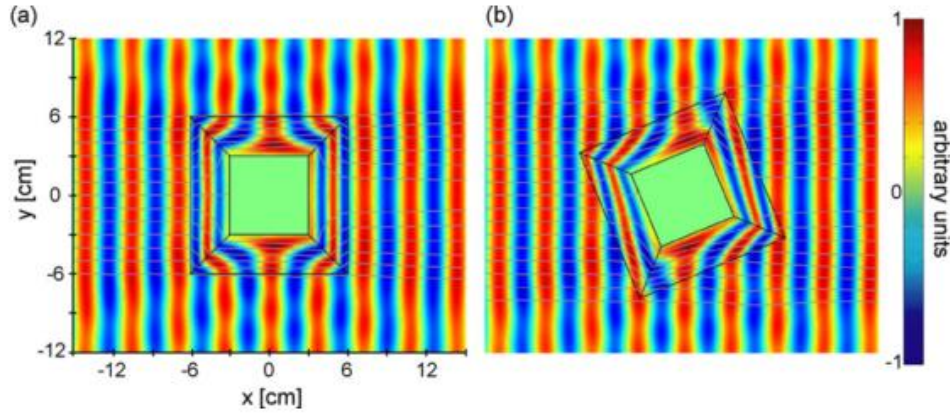
Fig. 2.14 Square cloak with of anisotropic material profile: (a) Cloak parallel to the incident wavefront (b) Cloak rotated by 22.5° [45].
