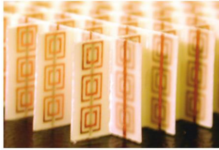
Fig. 2.2 Left-handed material for achieving a negative index of refraction [9].
