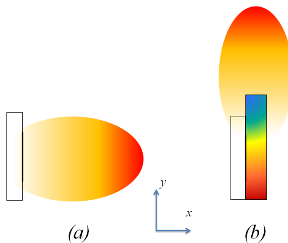
Fig. 5.13 Radiation patterns: (a) antenna alone, (b) antenna with dielectric superstrate for reorientation in single direction in azimuth.
