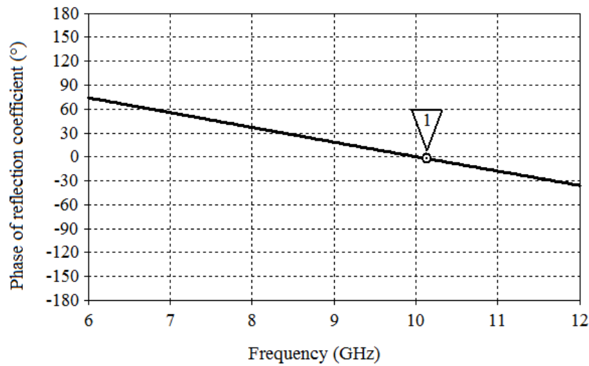
Fig. 5.34 Phase of reflection coefficient of the unit cell for a plane wave incident at 80^\circ .
