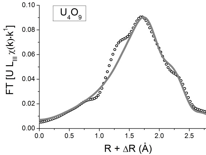
Fig. 4.16: Refinement of the U L III EXAFS Fourier transform of U 4 O 9 ( 3.5\text{--}14 \text{ Å}^{-1} , dk = 2 \text{ Å}^{-1} ).
