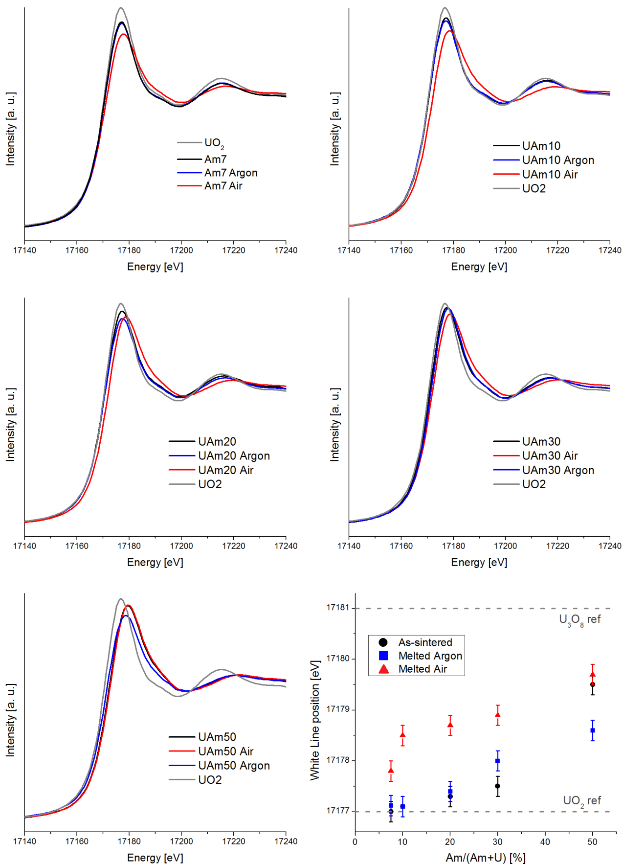
Fig. 6.19: XANES spectra collected at the U-L 3 edge of Am on (U,Am)O 2 oxides, before and after melting. Bottom right: observed white lines.
