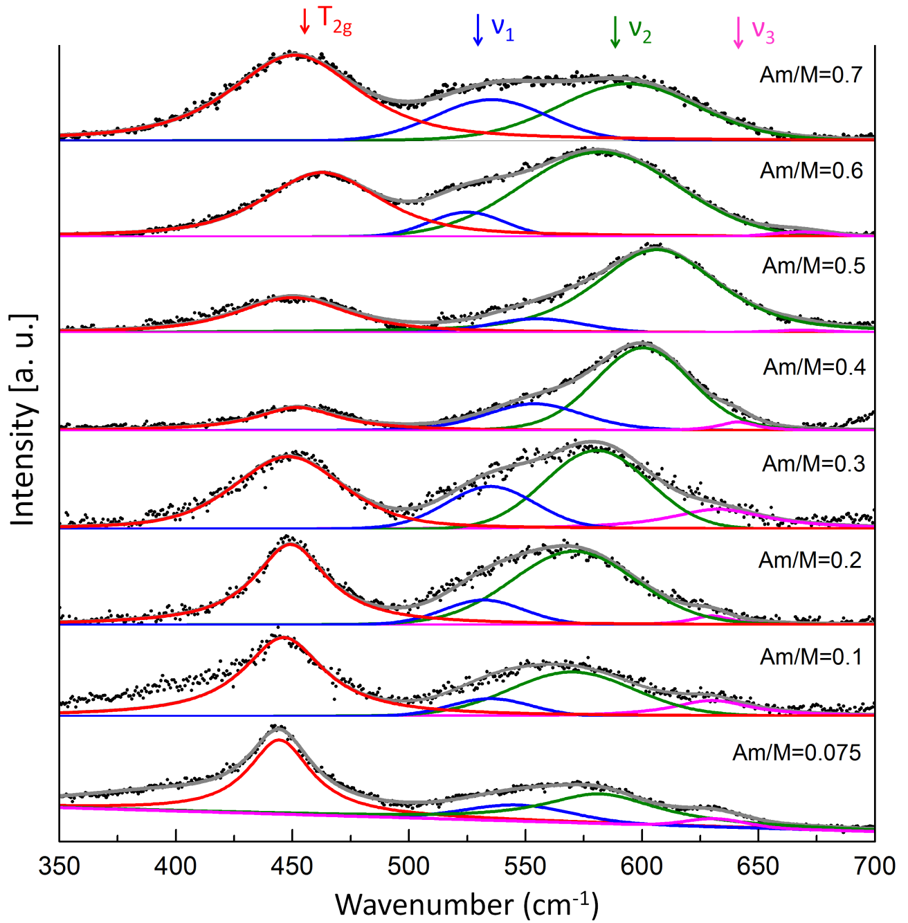
Fig. 4.18: Raman spectra of (U,Am)O 2 oxides with Am/(Am+U)=0.075, 0.1, 0.2, 0.3, 0.4, 0.5, 0.6 and 0.7. • = experimental points; – = deconvolution. The 4 bands used for the deconvolution ( T_{2g} , \nu_1 , \nu_2 , \nu_3 ) are also indicated.
