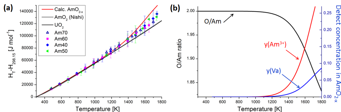
Fig. 6.5: The enthalpy increment function of AmO 2-x in air calculated from the CALPHAD model (—) (a) and the corresponding O/Am and defect fractions (b) as a function of temperature. The function is compared to the experimental data obtained in this work and the literature data of UO 2 [25] and stoichiometric AmO 2 [145].
