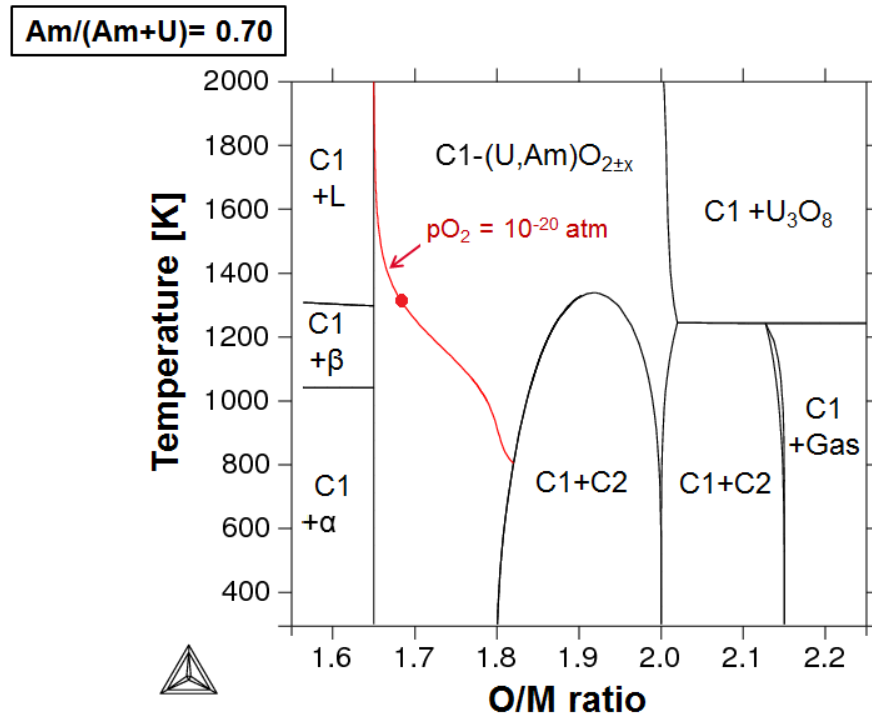
Fig. 7.6: Isopleth section of the U-Am-O phase diagram, for \text{Am}/\text{M}=0.70 and equilibria points (red line) calculated for p\text{O}_2 = 10^{-20} atm.
