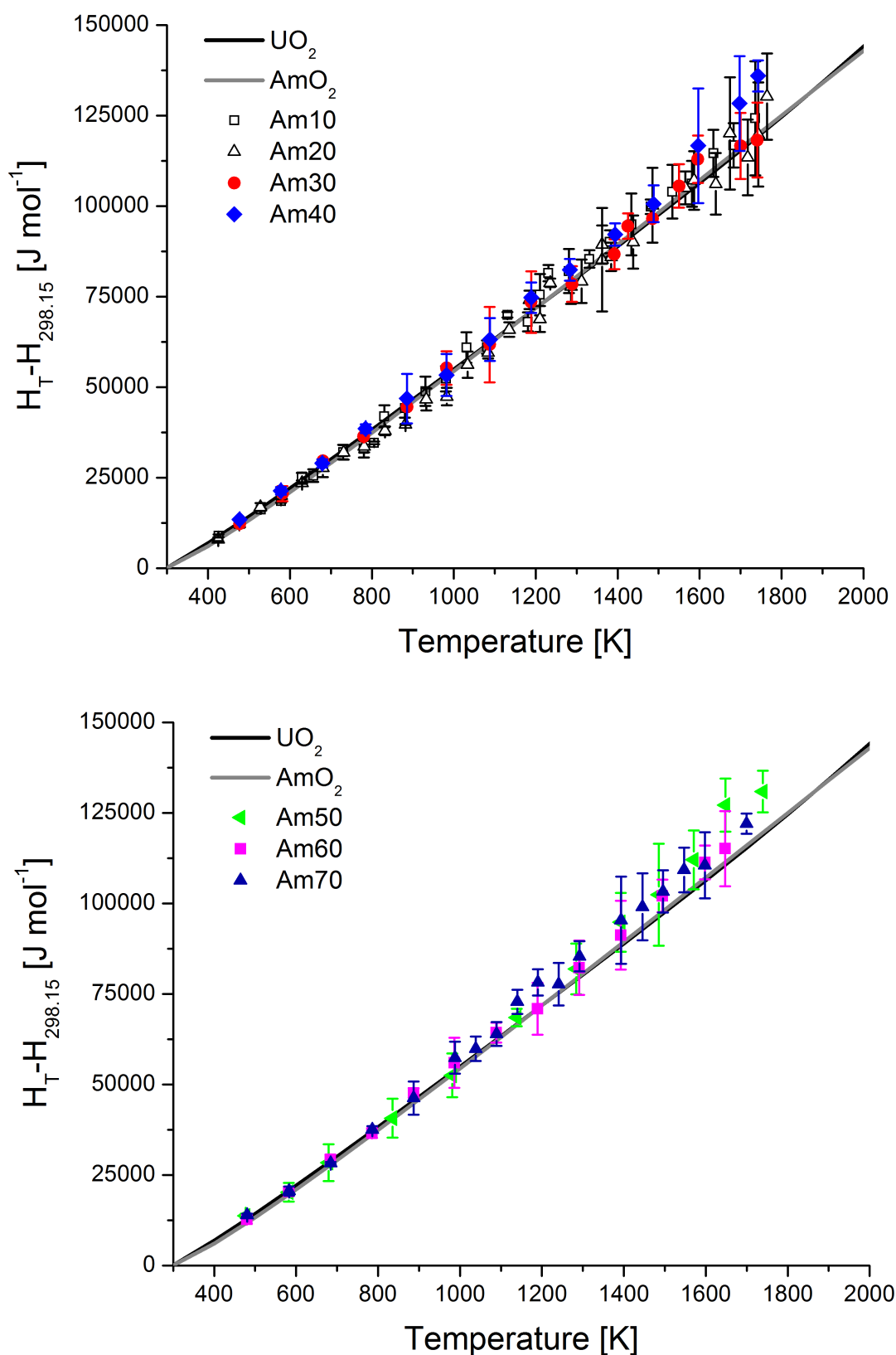
Fig. 6.2: Enthalpy increments of (U,Am) \text{O}_2 oxides measured in this work: in (a), Am30, Am40; in (b), Am50, Am60, Am70. The data from Valu et al. [203] for Am10 and Am20 are reported in (a), whereas the data of \text{UO}_2 and \text{AmO}_2 (extrapolated for T > 1100 K) are represented in both graphs.
