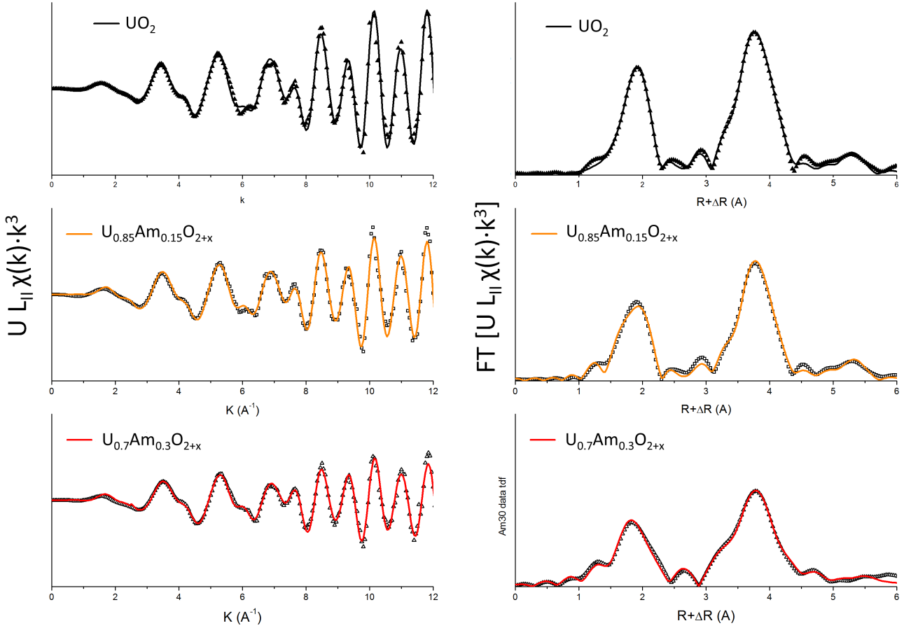
Fig. 4.15: Refinement of the U L II EXAFS spectra and their Fourier transforms for UO 2 , U 0.85 Am 0.15 O 2+x , U 0.7 Am 0.3 O 2+x (FT boundaries 3.5–11.5 Å -1 , dk = 2 \text{ Å}^{-1} ).
