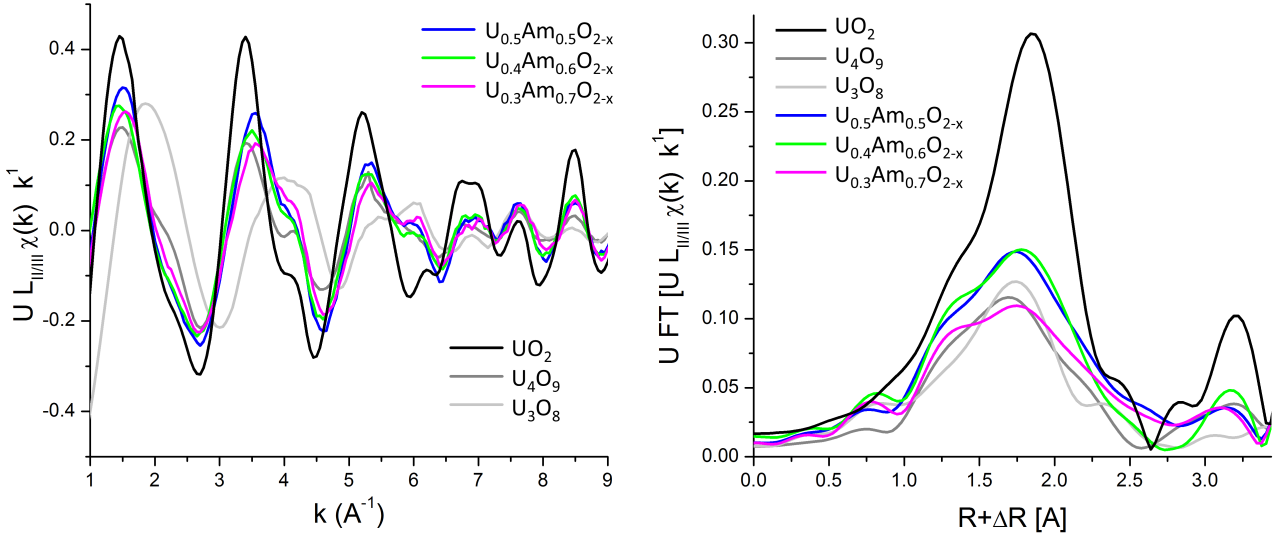
Fig. 4.11: k^1 -weighted EXAFS spectra at the U L_{II} edge and their Fourier transforms for the (U,Am)O 2 samples with Am/(Am+U)=0.5, 0.6 and 0.7. The U L_{II} spectrum of UO 2 and the U L_{III} spectra of U 4 O 9 and U 3 O 8 are also reported. FT boundaries: 3.5-11.5 \text{\AA}^{-1} , dk = 2\text{\AA}^{-1} .
