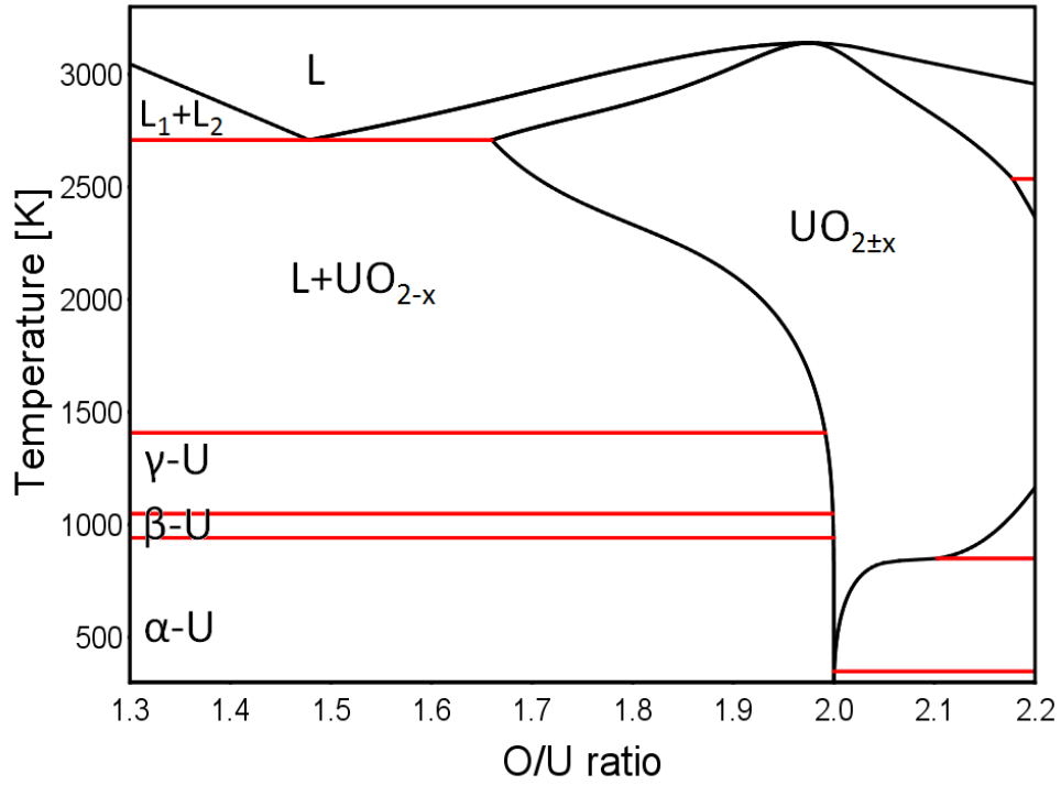
Fig. 2.2: The U- \text{UO}_{2+x} domain of the U-O phase diagram according to Guéneau et al. [27]
