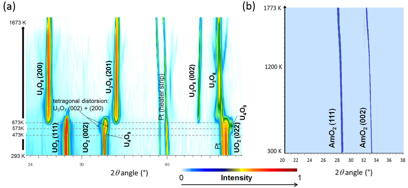
Fig. 5.1: Iso-intensity map of HT-XRD measurements in air on (a) UO 2 (figure extracted from [199]) and (b) AmO 2 .
