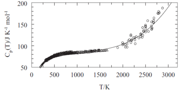
Fig. 2.24: Heat capacity of \text{UO}_2 [41, 139–142].
