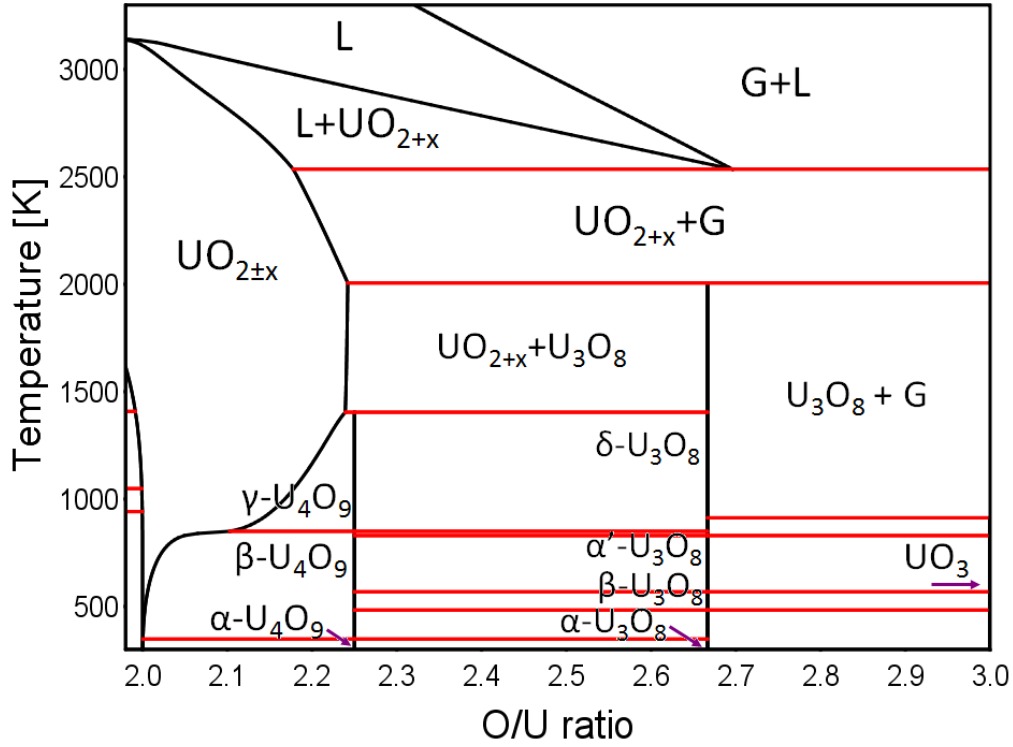
Fig. 2.3: The \text{UO}_2\text{-UO}_3 domain of the U-O phase diagram according to Guéneau et al. [27]
