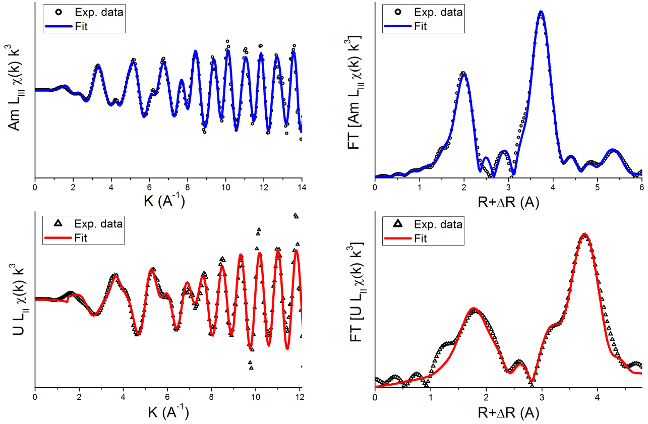
Fig. 5.19: Am L 3 and U L 2 EXAFS spectra and Fourier transforms of the Am50ox sample. FT boundaries: 3.5-13.5 Å -1 , dk = 2\text{Å}^{-1} for Am L 3 ; 3.5-11.2 Å -1 , dk = 2\text{Å}^{-1} for U L 2 .
