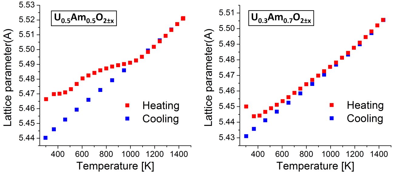
Fig. 5.13: Lattice parameter variation as a function of temperature for \text{U}_{0.5}\text{Am}_{0.5}\text{O}_{2\pm x} and \text{U}_{0.3}\text{Am}_{0.7}\text{O}_{2\pm x} oxider in air. (The lattice parameter uncertainty coincides with the symbol size).
