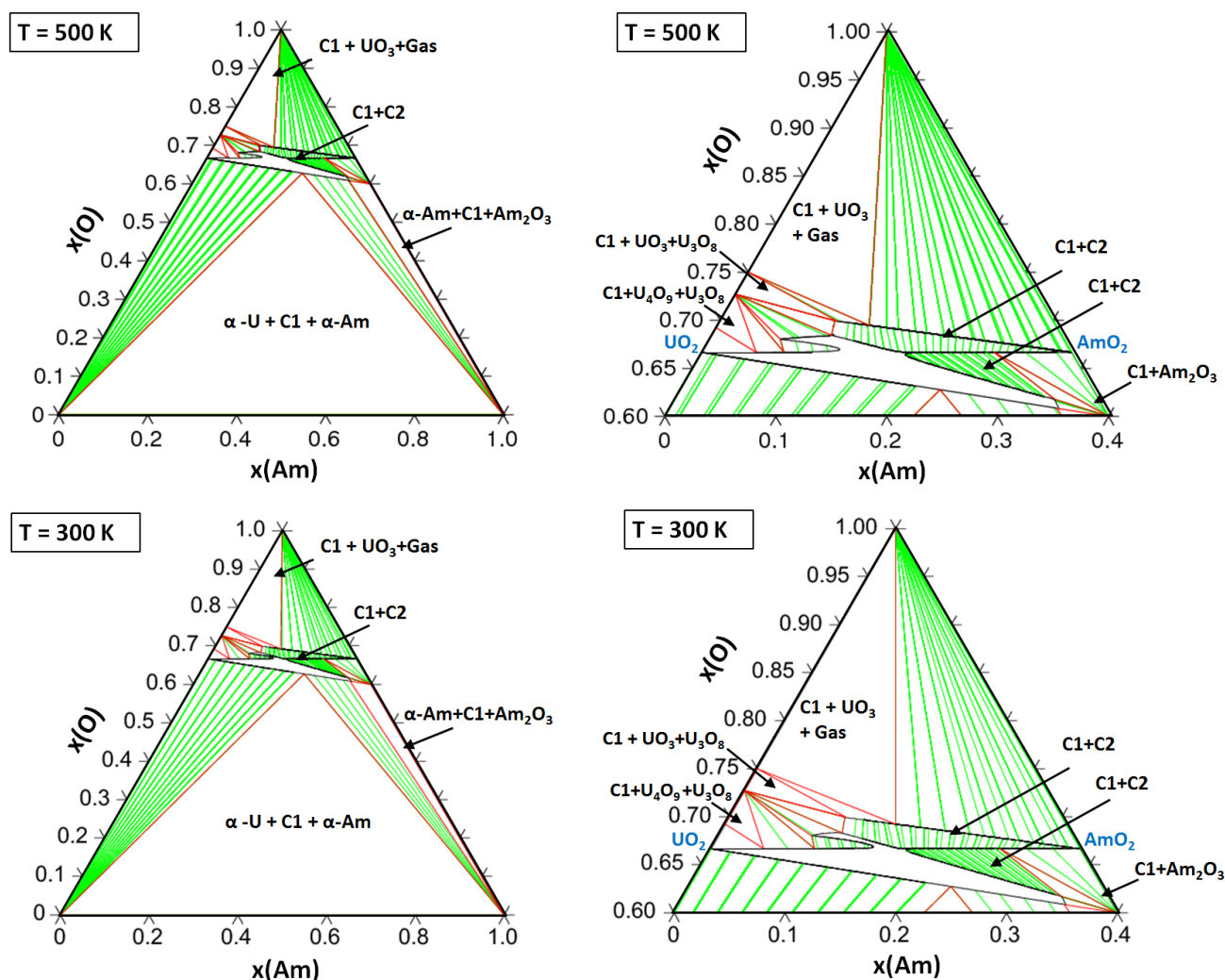
Fig. 7.5: Isothermal sections of the U-Am-O phase diagram for T = 300, 500 K, with zooms on the oxide domain (right).
