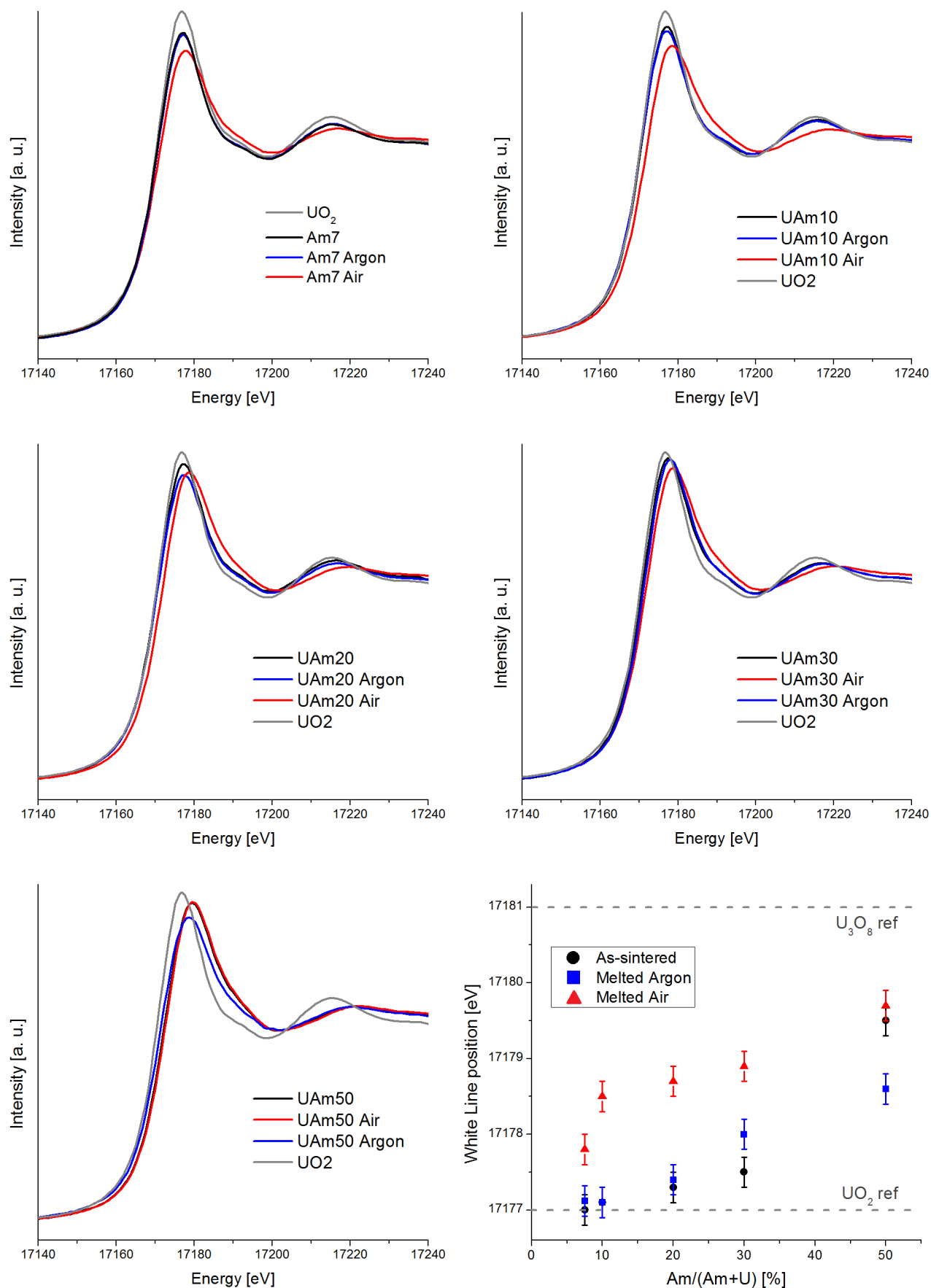
Fig. 6.19: XANES spectra collected at the U-L 3 edge of Am on (U,Am)O 2 oxides, before and after melting. Bottom right: observed white lines.
