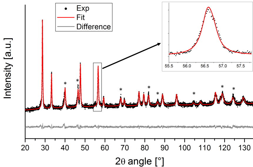
Fig. 3.4: XRD pattern acquired on the aged AmO 2 sample at room temperature and Pawley refinement (* indicate the diffraction peaks due to the Pt sample holder).
