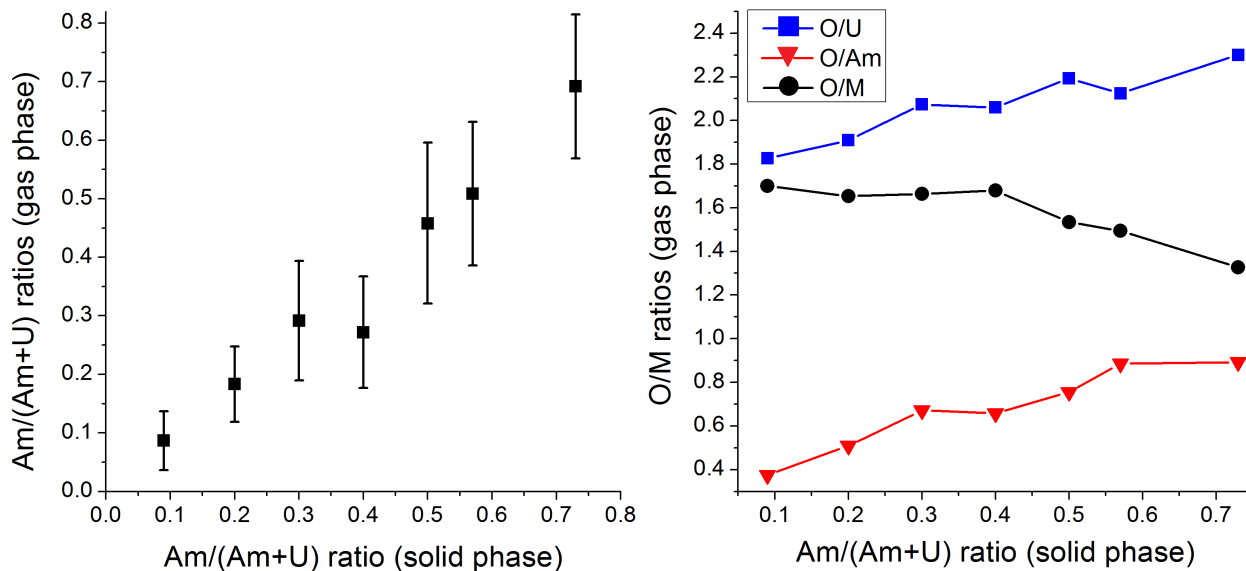
Fig. 6.11: Composition of the gas phase vs the Am/M of the solid phase: (a) Am/(Am+U) ratio; (b) O/U, O/Am and O/M ratio; these data are given with an uncertainty of 0.5, error bars not represented for visual clarity.
