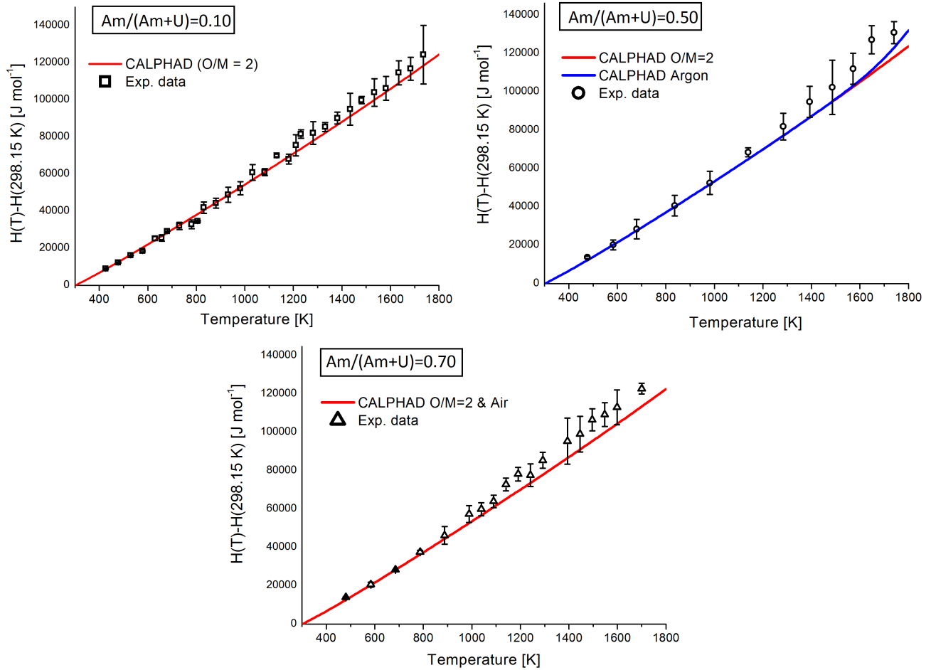
Fig. 7.12: Calculated enthalpy functions compare to experimental data for Am/(Am+U)=0.10 , 0.50 and 0.70.
