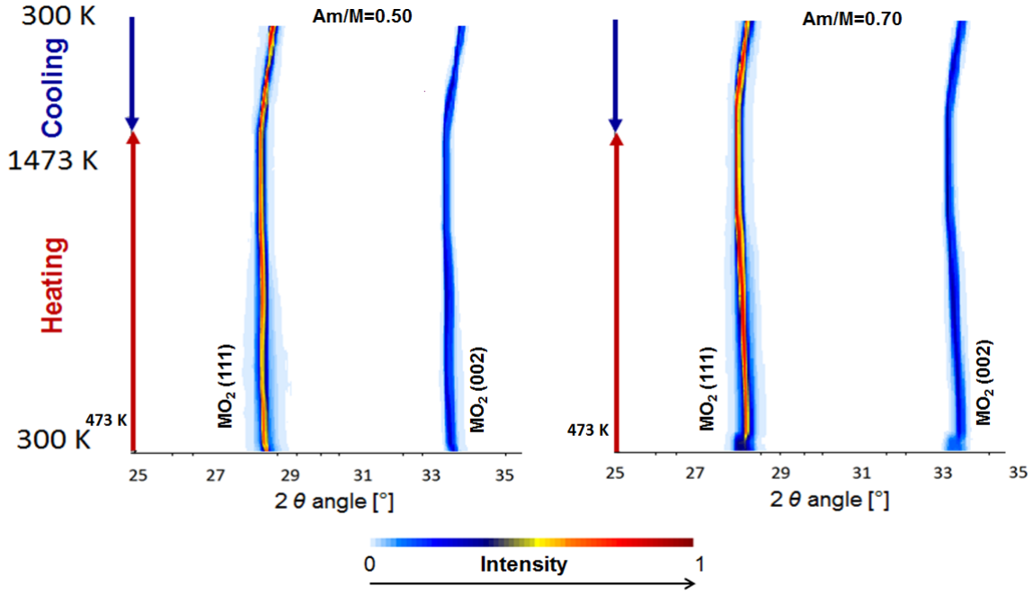
Fig. 5.12: Isointensity maps of HT-XRD measurements in air on (\text{U,Am})\text{O}_2 with \text{Am}/(\text{Am}+\text{U})=0.5 and 0.7 .
