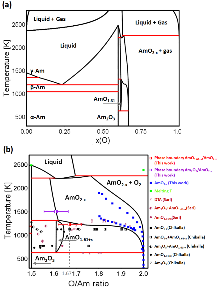
Fig. 3.17: (a) Am-O phase diagram calculated with the CALPHAD model of this work; (b) magnification in the stoichiometry range 1.49 < O/Am < 2.01 . The experimental data are from [56,58,63] and this work.
