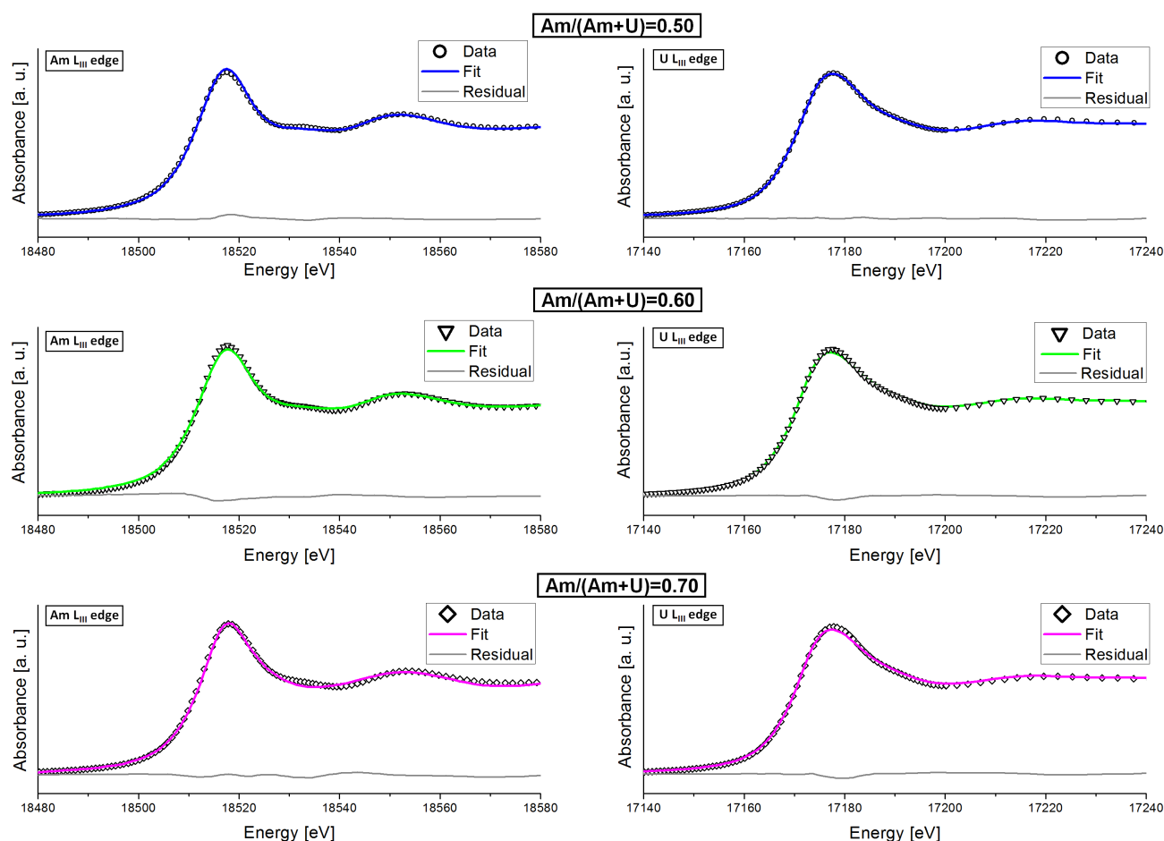
Fig. 4.7: Experimental XANES spectra and linear combination fits at the L 3 edge of Am (left) and U (right) for the (U,Am)O 2 samples with Am/(Am+U) ratio equal to 50, 60 and 70 mol.%.
