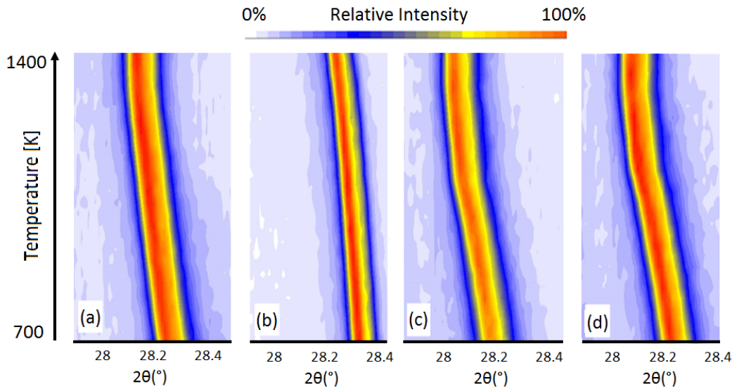
Fig. 3.11: Iso-intensity maps of the main fluorite-structure peak (111) collected during fast cooling under different atmospheres: pO 2 = 10 -5 atm (a), 10 -6 atm (b), 10 -7 atm (c), 10 -8 atm (d).
