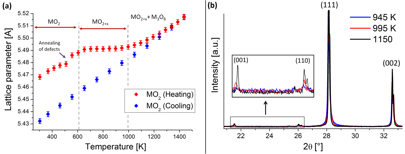
Fig. 5.8: Behaviour of the \text{U}_{0.7}\text{Am}_{0.3}\text{O}_2 sample in air: (a) evolution of the lattice parameter of the cubic structure as a function of the temperature; (b) extracts of the XRD patterns, for selected temperatures (heating), showing the (111), (002) reflections of the Fm\bar{3}m structure and the (001) (110) reflections of the P\bar{6}2m structure.
