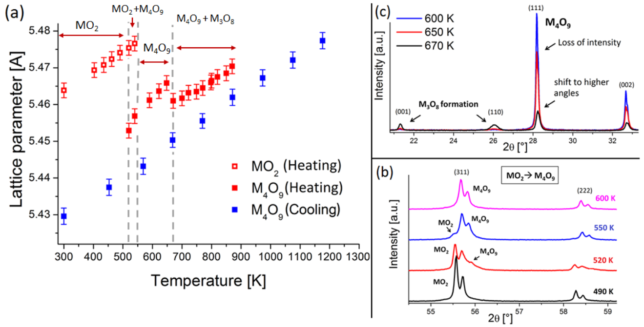
Fig. 5.3: Behaviour of the U 0.9 Am 0.1 O 2 sample in air: (a) evolution of the lattice parameter of the cubic structure as a function of the temperature; (b) extracts of the XRD patterns, for selected temperatures, showing the (311) and (222) reflections of the Fm \bar{3} m structure; (c) extracts of the XRD patterns, for selected temperatures, showing the (111), (002) reflections of the Fm \bar{3} m structure and the (001) (110) reflections of the P \bar{6} 2 m structure.
