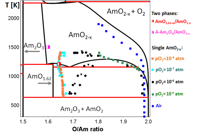
Fig. 3.15: The O/Am-T points observed in this work according to our composition assessment are reported on the phase diagram of Gotcu-Freis et al.
