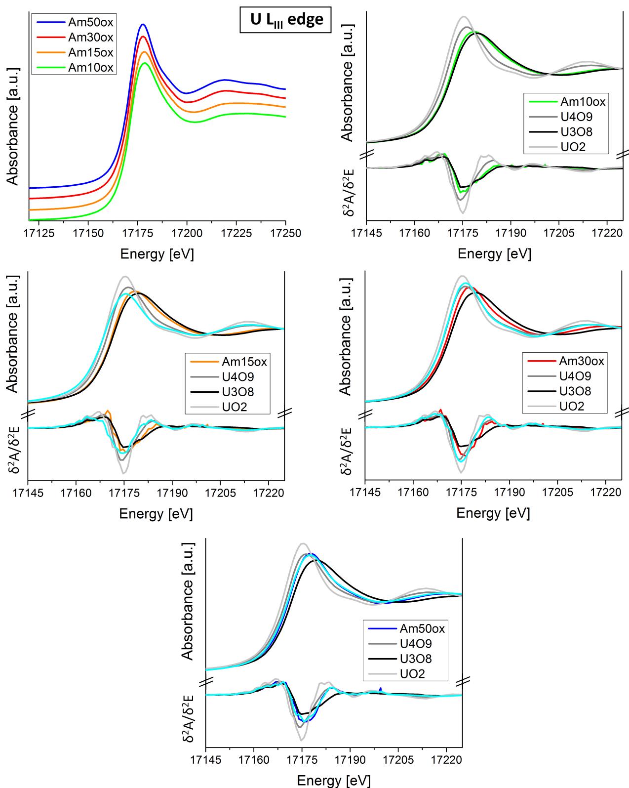
Fig. 5.15: XANES spectra collected at the L_3 edge of U and their second derivatives for the (U,Am)O_2 samples before and after oxidation in air.
