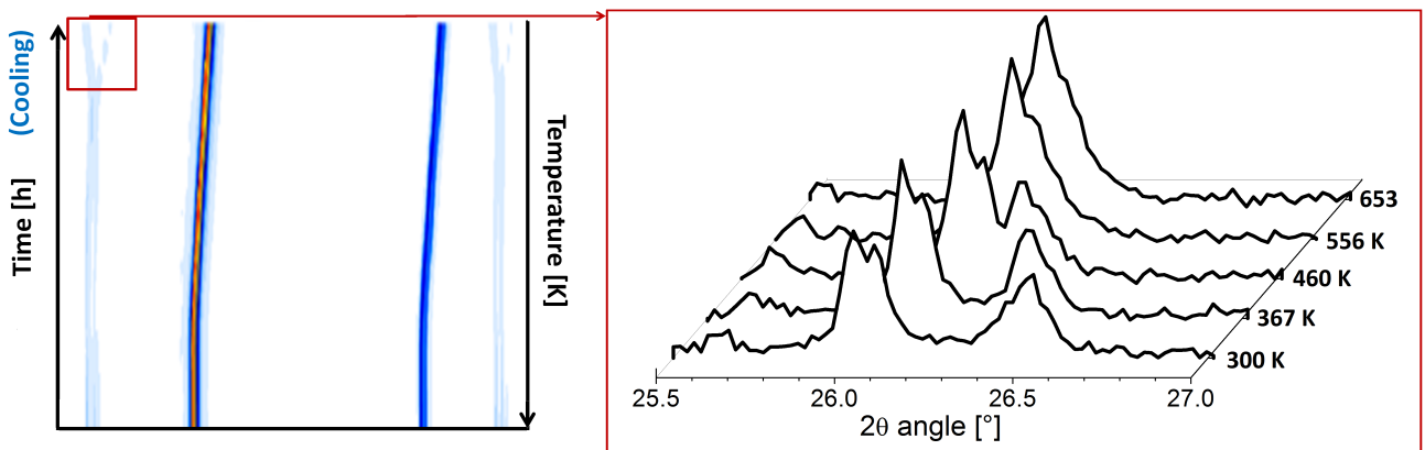
Fig. 5.9: Cooling in air of the \text{Am}/(\text{Am}+\text{U})=0.30 composition: zoom on the 25.5 < 2\theta < 27^\circ range of the XRD patterns. The doubling of the XRD peak indicates the transition from the hexagonal P\bar{6}2m to the orthorhombic C2mm structure for \text{M}_3\text{O}_8 .
