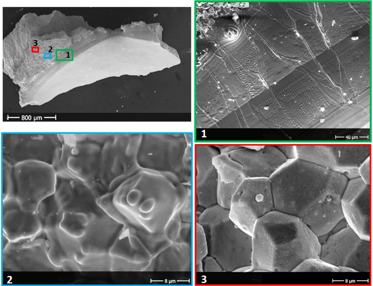
Fig. 6.15: SEM images acquired on the the \text{U}_{0.5}\text{Am}_{0.5}\text{O}_{2\pm x} oxide melted in argon.
