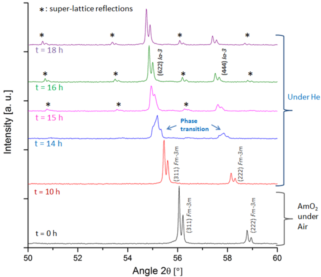
Fig. 3.8: XRD patterns sections between 50° and 60° 2\theta during iso-T measurements at 1220 K during reduction. After 14 h, the BCC structure (super-lattice reflections) appears.
