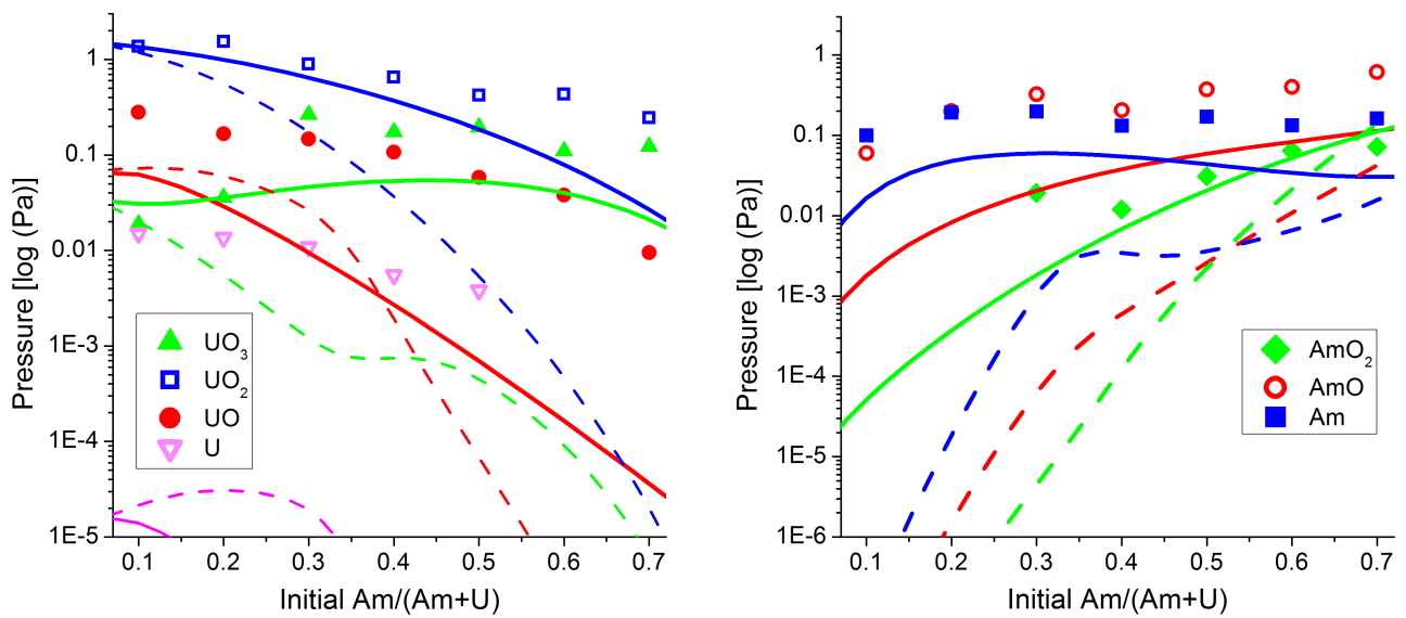
Fig. 7.8: Calculated and measured partial pressures of the U (left) and Am (right) species at 2320 K, imposing \text{O}/\text{M}(\text{solid}) = \text{O}/\text{M}(\text{gas}) . Dotted lines: CALPHAD- Lebreton; solid lines: CALPHAD- this work
