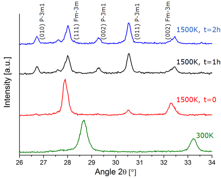
Fig. 3.6: Diffraction patterns collected at 300 K and 1500 K for 2 hours under controlled atmosphere ( p_{O_2} \simeq 2 \cdot 10^{-5} atm). The characteristic diffraction peaks of the Fm\bar{3}m ( AmO_2 ) and P\bar{3}m1 ( Am_2O_3 ) structures are identified.
