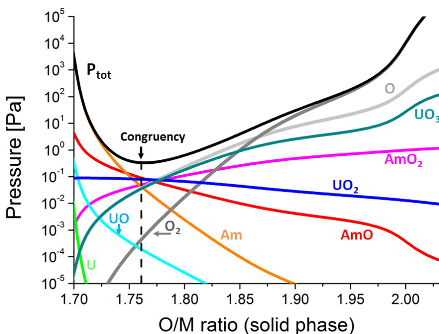
Fig. 7.10: Calculated pressures as a function of the O/M ratio at 2320 K, for an Am/(Am+U) ratio equal to 0.60.
