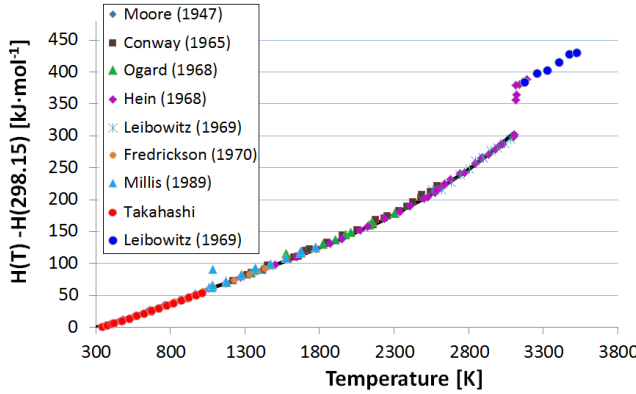
Fig. 2.23: High temperature enthalpy increments of \text{UO}_2 [130–138].
