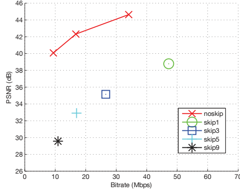
Figure 4.19: Bitrate variations with PSNR measured on light-field slices (Champagne sequence)
