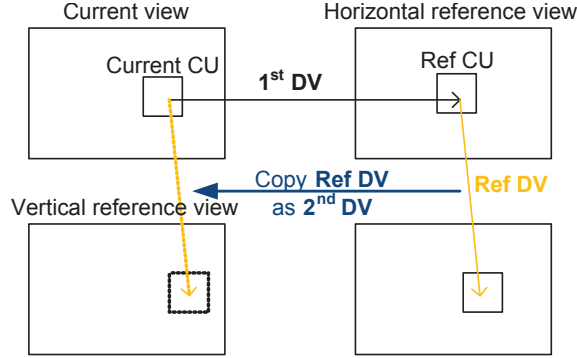
Figure 5.7: Inter-view derivation of a second DV
