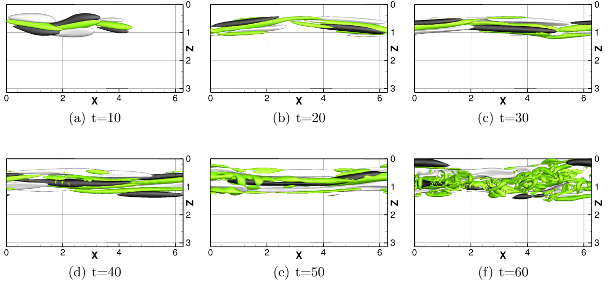
Figure II.16: Snapshots of the time evolution of the highly nonlinear optimal perturbation computed for T_{opt} = 30 and E_0 = 2.5 \times 10^{-7} . Isosurface of Q -criterion ( Q = 0.01Q_{max} ) colored by streamwise vorticity, and isosurfaces of streamwise velocity disturbance ( u = \pm 0.5u_{max} , black negative and white positive).
