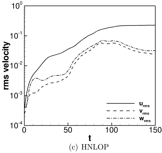
Figure II.15: Time evolution of the rms of the velocity (left) and vorticity (right) components for the 50-norm LOP (top frames) and the HNLOP (bottom frames) with E_0 = 2.5 \times 10^{-7} , computed for T_{opt} = 30 .
