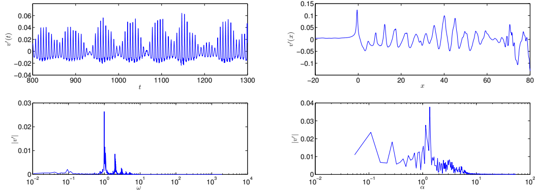
Figure V.12: A probe in (10, 1.5, 0) is used to catch the temporal signal and its spectrum with the main pulsation at \omega = 1.02 (left). Instantaneous wall-normal velocity on a line located at y = 1.5 and z = 0 shows a dominant spatial wavenumber \alpha = 1.3 (right). For both signals the Fourier spectrum is also reported. For the temporal signal the main harmonic is at \omega = 1.02 and for the spatial signal the main spatial wavelength is equal to 1.3.
