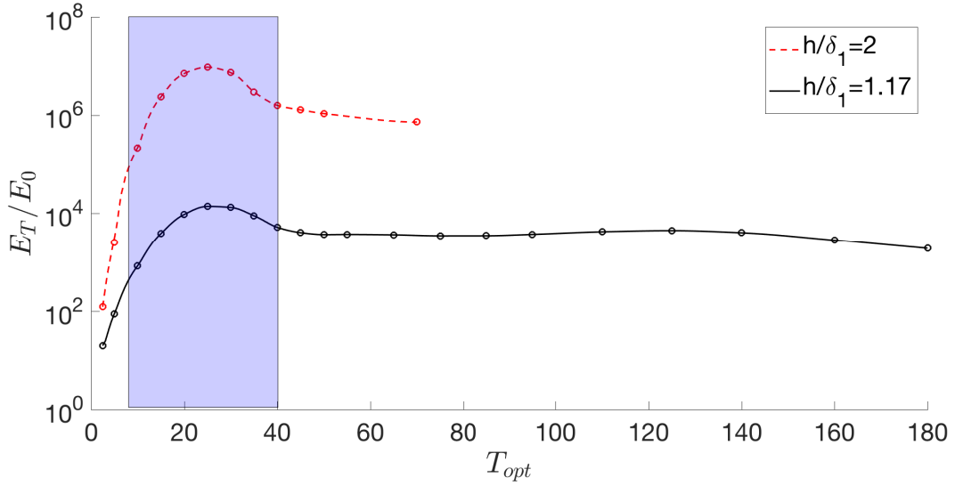
Figure VII.27: Transient energy growth comparison between h/\delta_1 = 1.17 (black continuous line) and \delta_1 = 2 (red dashed line). Blue region highlight T_{opt} range for which the optimal perturbation is antisymmetric.
