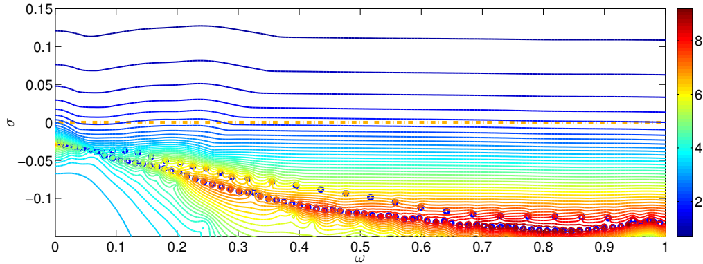
Figure VII.8: Pseudospectrum evaluation on the Hessenberg matrix. Iso-lines represent pseudospectrum given by \log_{10} \epsilon contour.
