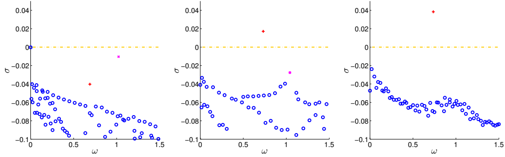
Figure VI.3: Eigenspectrum for Re = 700, 900 and 1200 . Red (+) marker represents the varicose mode, magenta (x) marker the sinuous one.
