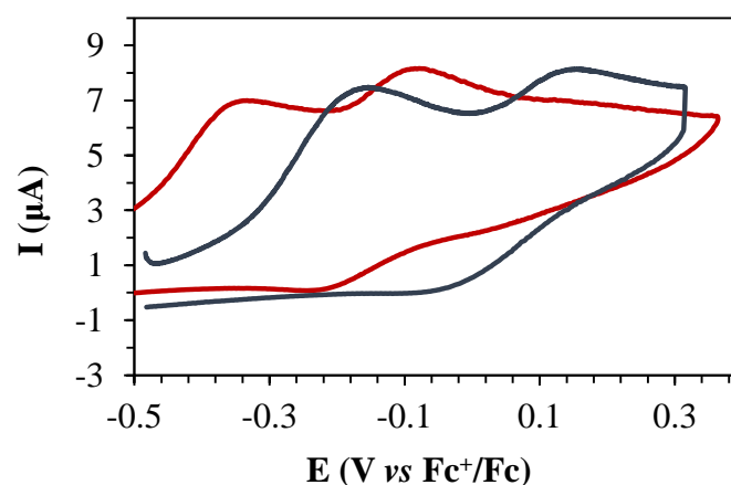
Figure 16. Cyclic voltammograms of the potassium salts of the ligands Psalen tBu (blue) and Psalen OMe (red) in CH 2 Cl 2 (containing 0.12 M of TBAPF 6 ) at carbon electrode. The curve of Psalen OMe has been normalized.
