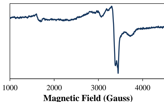
Figure 93. X-band EPR spectrum of [\text{Cu}(\text{Psalophen})]^+\text{SbF}_6^- in a dichloromethane solution at 10 K. Conditions: Frequency: 9.641 GHz; Power: 2.002 mW; modulation frequency: 100 kHz; amplitude: 0.8 mT. This spectrum was recorded under saturated conditions.
