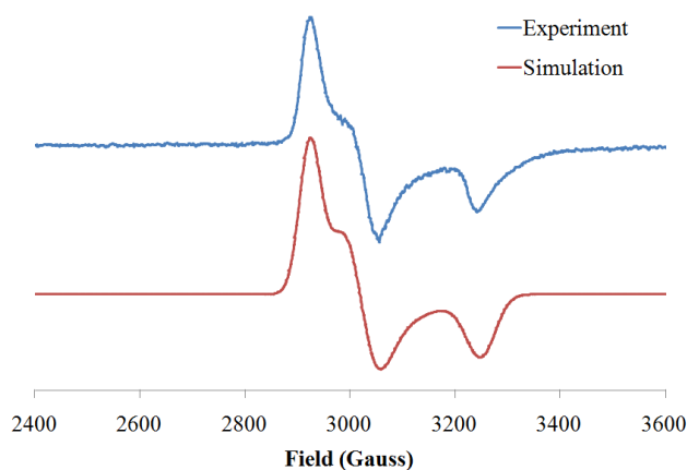
Figure 27. Experimental and simulated EPR spectrum of [Ni(Psalen tBu )] + in dichloromethane at 5K. [1]
