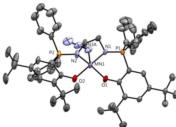
Figure 172. ORTEP of [Mn(Psalent tBu )(N 3 )] with thermal ellipsoids at 50 % probability. Hydrogen atoms and a molecule of THF have been removed for clarity.
