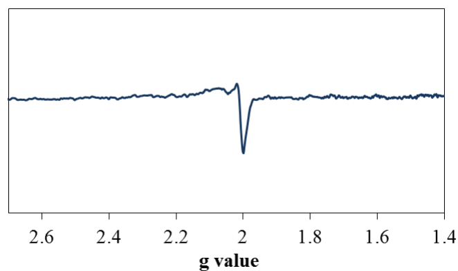
Figure 90. X-band EPR spectrum of [[\text{Ni}(\text{Psalophen})]]+\text{SbF}_6^-)_2 in the solid state at 10 K. Conditions: Frequency: 9.640 GHz; Power: 0.5029 mW; modulation frequency: 100 kHz; amplitude: 0.8 mT.
