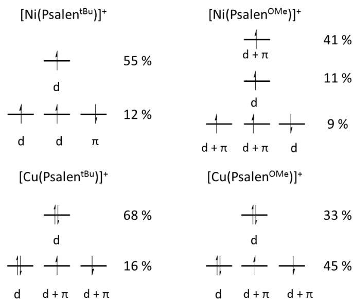
Chart 1. Electronic structure of [\text{Ni}(\text{Psalen}^{\text{tBu}})]^+\text{SbF}_6^- , [\text{Ni}(\text{Psalen}^{\text{OMe}})]^+\text{SbF}_6^- , [\text{Cu}(\text{Psalen}^{\text{tBu}})]^+\text{SbF}_6^- and [\text{Cu}(\text{Psalen}^{\text{OMe}})]^+\text{SbF}_6^- computed from CASSCF/TZVP state-average calculations.
