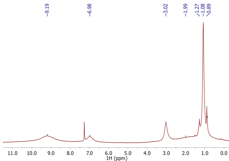
Figure 129. ^1\text{H} NMR spectrum of [\text{Cu}(\text{Psalophen}^{\text{OMe}_2})] in \text{CDCl}_3 at 20^\circ\text{C} . Signals present around 1.27 and 0.89 ppm correspond to pentane.
