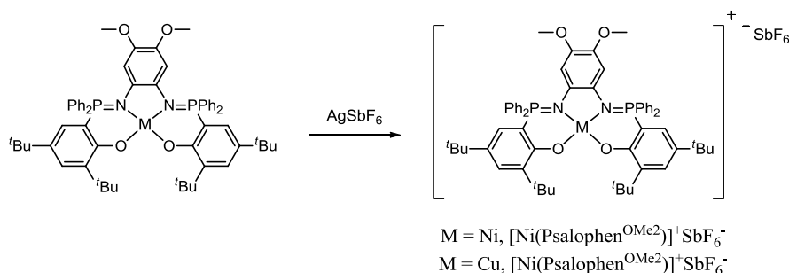
Scheme 74. Chemical oxidation of [Ni(Psalophen OMe2 )] and [Cu(Psalophen OMe2 )] complexes.
