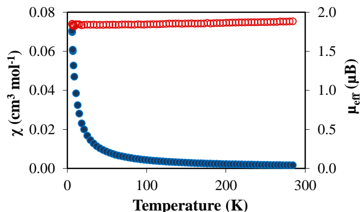
Figure 14. Plot of magnetic susceptibility (blue circles) and effective magnetic moment (red circles) vs. temperature for [Cu(Psalen tBu )].
