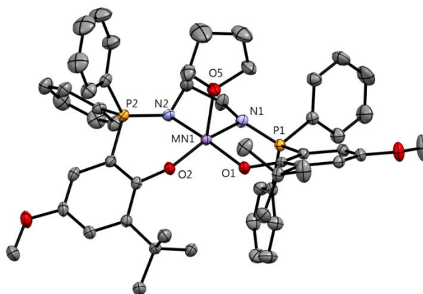
Figure 168. ORTEP of [\text{Mn}(\text{Psalen}^{\text{OMe}})(\text{THF})]\text{PF}_6 with thermal ellipsoids at 50 % probability. Hydrogen atoms and a molecule of THF and a molecule of \text{PF}_6 have been removed for clarity
