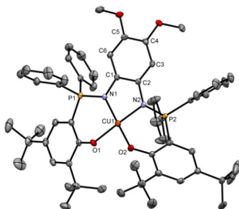
Figure 133. ORTEP of [Cu(Psalophen OMe2 )] with thermal ellipsoids at 50 % probability. Hydrogen atoms and a molecule of dichloromethane have been omitted for clarity.
