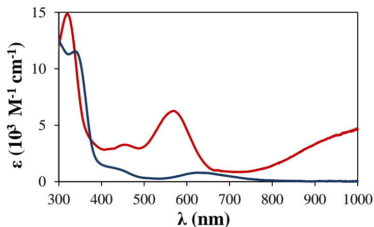
Figure 34. UV-vis spectra of [Cu(Psalen 0Me )] (blue line) and [Cu(Psalen 0Me )] + (red line) in CH 2 Cl 2 at 298 K.
