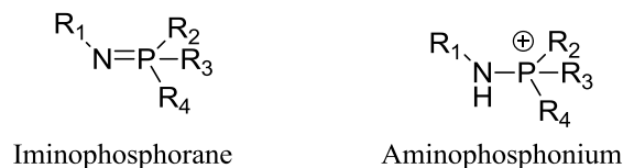
Scheme 26. Iminophosphorane and aminophosphonium functions.
