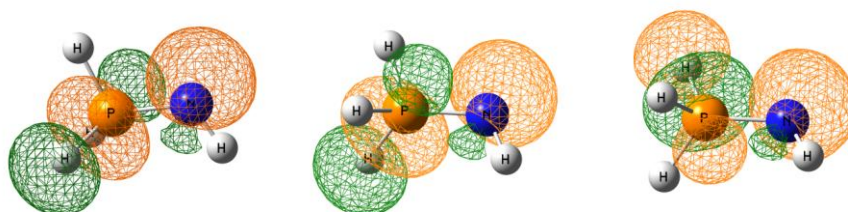
Figure 2. Stabilizing interactions between L1 and three \sigma^*(\text{P-H}) antibonding orbitals. [89]
