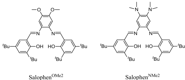
Scheme 55. \text{Salophen}^{\text{OMe2}} (left) and \text{Salophen}^{\text{NMe2}} (right) ligands. [3a,6]
