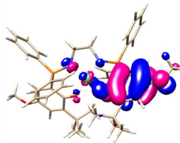
HOMO [Ni(Psalen OMe ) + ]
