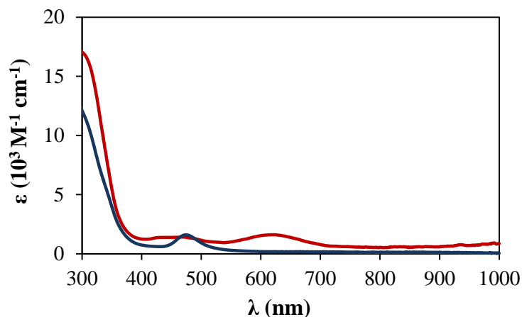
Figure 124. UV-vis spectra of [Cu(Psalophen CF3 )] (blue line) and [Cu(Psalophen CF3 )] + (red line) in dichloromethane.
