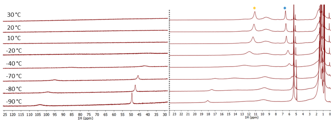
Figure 143. 1 H NMR spectra of [Cu(Psalophen OMe2 )] + in CD 2 Cl 2 at different temperatures.
