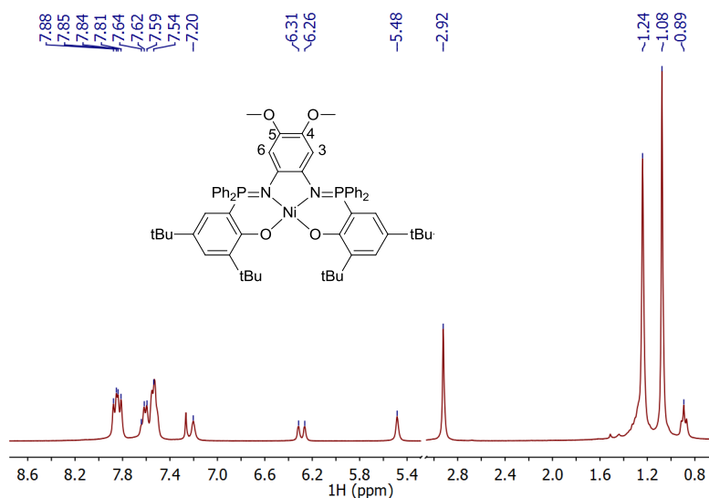
Figure 128. ^1\text{H} NMR spectrum of [\text{Ni}(\text{Psalophen}^{\text{OMe}_2})] in \text{CDCl}_3 . The signal at 0.89 ppm corresponds to pentane.
