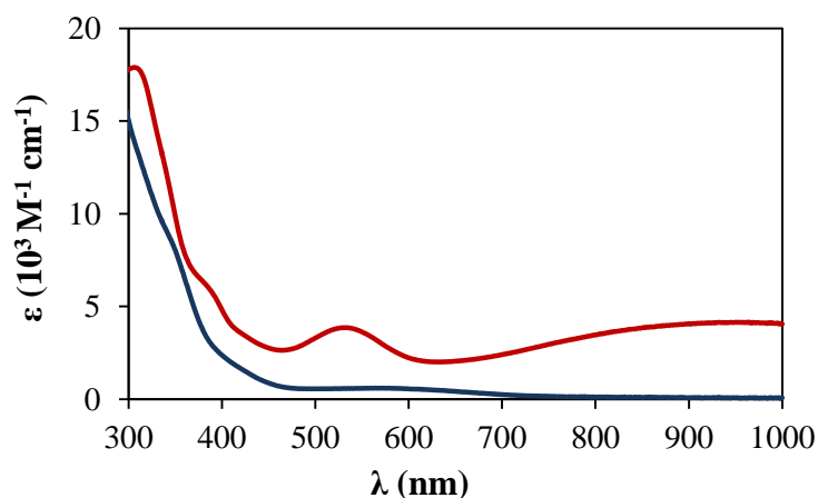
Figure 123. UV-vis spectra of [Ni(Psalophen CF3 )] (blue line) and [Ni(Psalophen CF3 )] + (red line) in dichloromethane.
