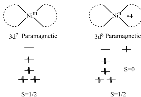
Scheme 18. Representation of the different electronic configurations for Ni oxidized complexes in a square-planar environment.
