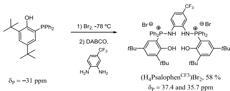
Scheme 69. Synthetic procedure for (H_4Psalophen^{CF_3})Br_2 and related ^{31}P chemical shifts in dichloromethane.
