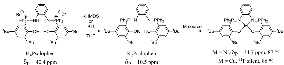
Scheme 60. Synthesis of the complexes and the related ^{31}\text{P} NMR signals in THF.
