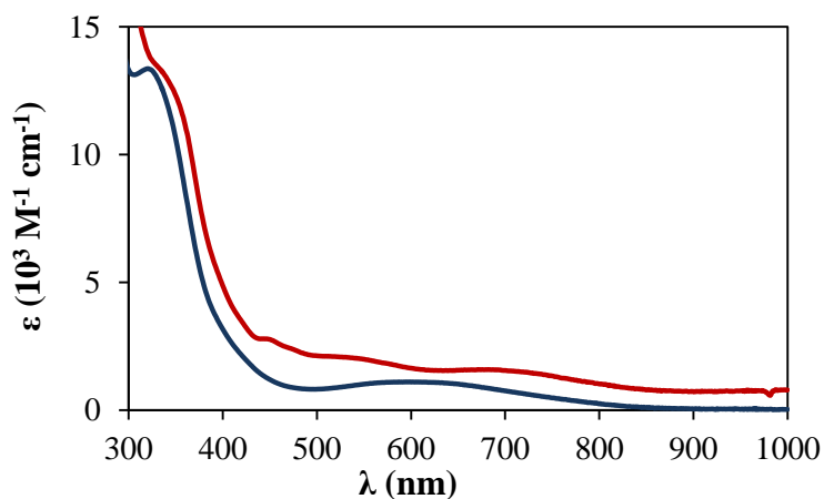
Figure 150. UV-vis spectra of [Ni(Psalophen OMe2 )] (blue line) and [Ni(Psalophen OMe2 )] + (red line) in dichloromethane.
