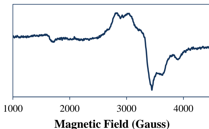
Figure 92. X-band EPR spectrum of [\text{Cu}(\text{Psalophen})]^+\text{SbF}_6^-_2 in the solid state at 40 K. Conditions: Frequency: 9.637 GHz; Power: 2.002 mW; modulation frequency: 100 kHz; amplitude: 0.8 mT.
