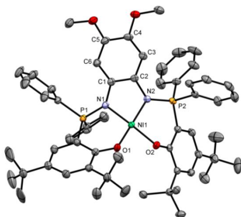
Figure 132. ORTEP of [Ni(Psalophen OMe2 )] with thermal ellipsoids at 50 % probability. Hydrogen atoms and a molecule of diethyl ether have been omitted for clarity.
