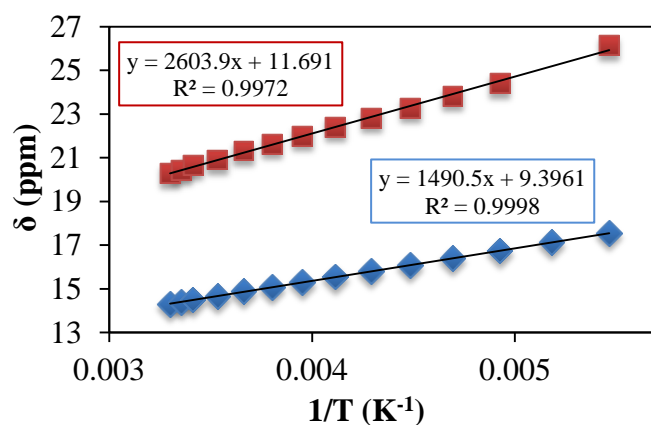
Figure 55. Plot of the chemical shifts of the phenoxide protons with the inverse of the temperature for compound [\text{Ni}(\text{iPrPsalen})]^+ .
