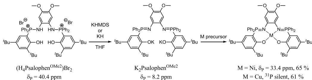
Scheme 73. Synthesis of [\text{Ni}(\text{Psalophen}^{\text{OMe}_2})] and [\text{Cu}(\text{Psalophen}^{\text{OMe}_2})] and their related ^{31}\text{P} NMR signals in THF.
