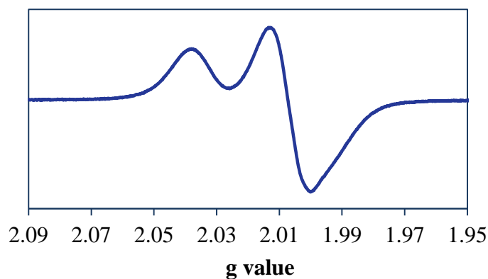
Figure 147. X-band EPR spectrum of [\text{Ni}(\text{Psalophen}^{\text{OMe}_2})]^+ in dichloromethane at 160 K. Conditions: Frequency: 9.387 GHz; Power: 1.006 mW; modulation frequency: 100 kHz; amplitude: 0.1 mT.
