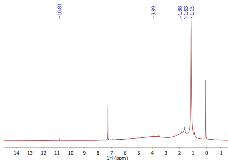
Figure 47. ^1\text{H} NMR of [\text{Cu}(\text{iPrPsalen})] in \text{CD}_2\text{Cl}_2 at 20\text{ }^\circ\text{C} . The signal around 0 ppm corresponds to silicon grease.
