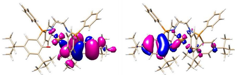
Figure 44. Active space molecular orbitals occupied by unpaired electrons with a “metal-ligand” character for [\text{Cu}(\text{Psalen}^{\text{tBu}})]^+ .
