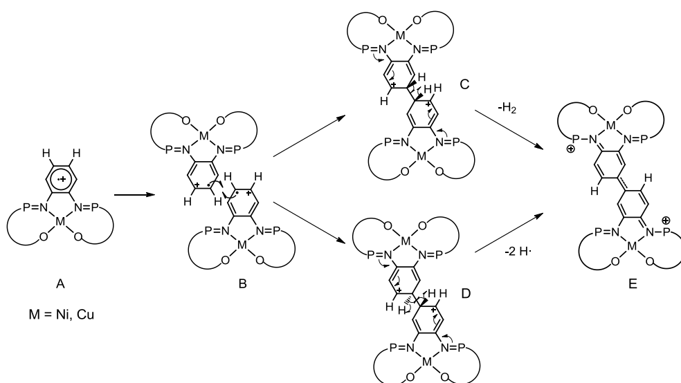
Scheme 63. Proposed dimerization mechanism for [Cu(Psalophen)] + and [Ni(Psalophen)] + complexes.
