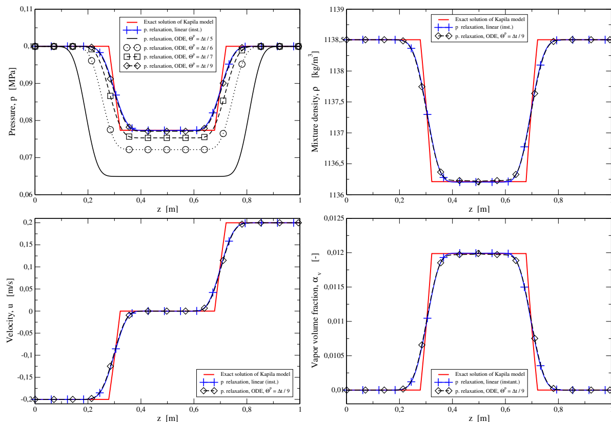
FIGURE 6.7. Numerical results for the water cavitation test with initial velocity |u| = 0.2 \text{ m/s} . Initial parameters are reported in Eq. (6.80), t_{output} = 0.2 \text{ ms} . Calculations made with 1000 cells, second order HLLC-type scheme for the hyperbolic operator and RK45 as ODE solver.
