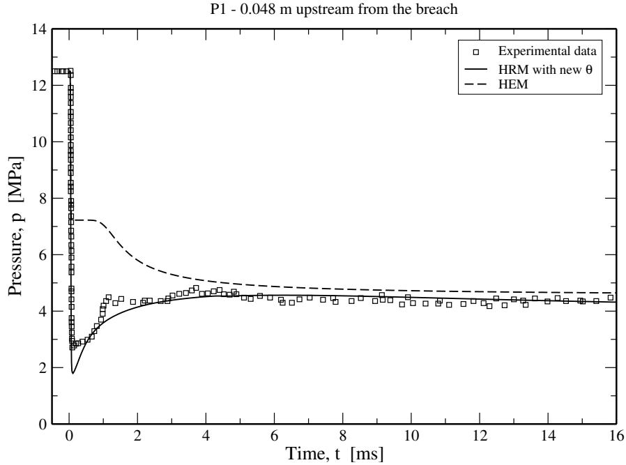
FIGURE 4.11. Pressure evolution in the first 16ms of the Bartak's experiment [16] ( 12.5\text{ MPa} , 563.15\text{ K} ). Assessment of HEM and HRM using the relaxation time correlation proposed in Eq. (4.62).
