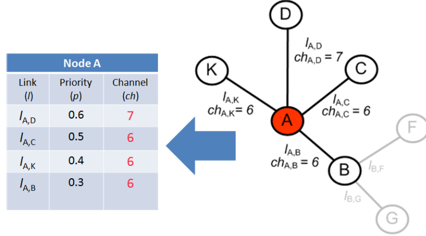
Figure 16: Allocated channels
