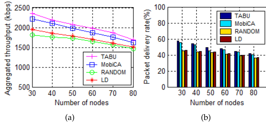
Figure 28: (a) Aggregated throughput \times number of nodes, (b) packet delivery rate \times number of nodes.
