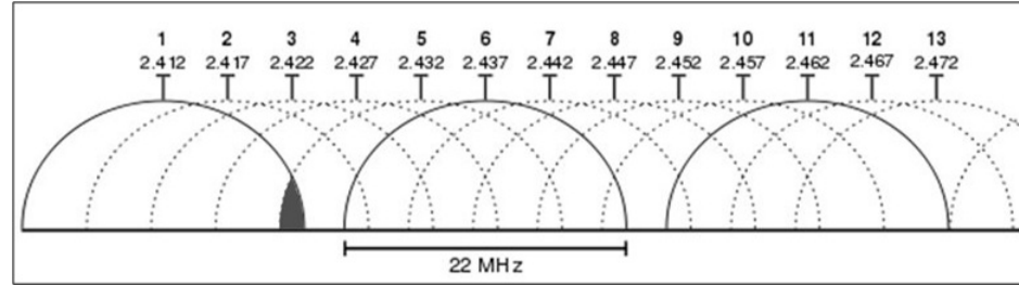
Figure 9: Channels overlapping in WiFi spectrum [98]
