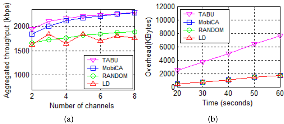
Figure 25: (a) Aggregated throughput x number of channels, (b) overhead x time.
