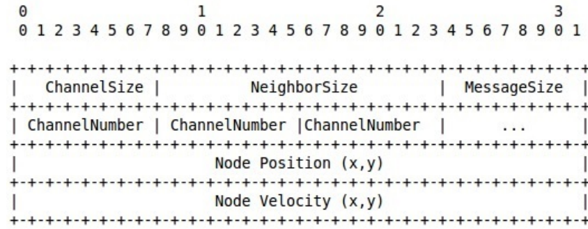
Figure 12: Hello message.
