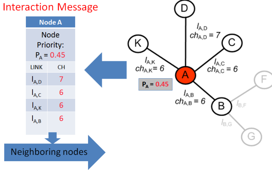
Figure 17: Interaction message
