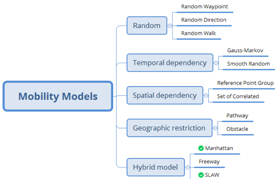
Figure 8: Mobility models
