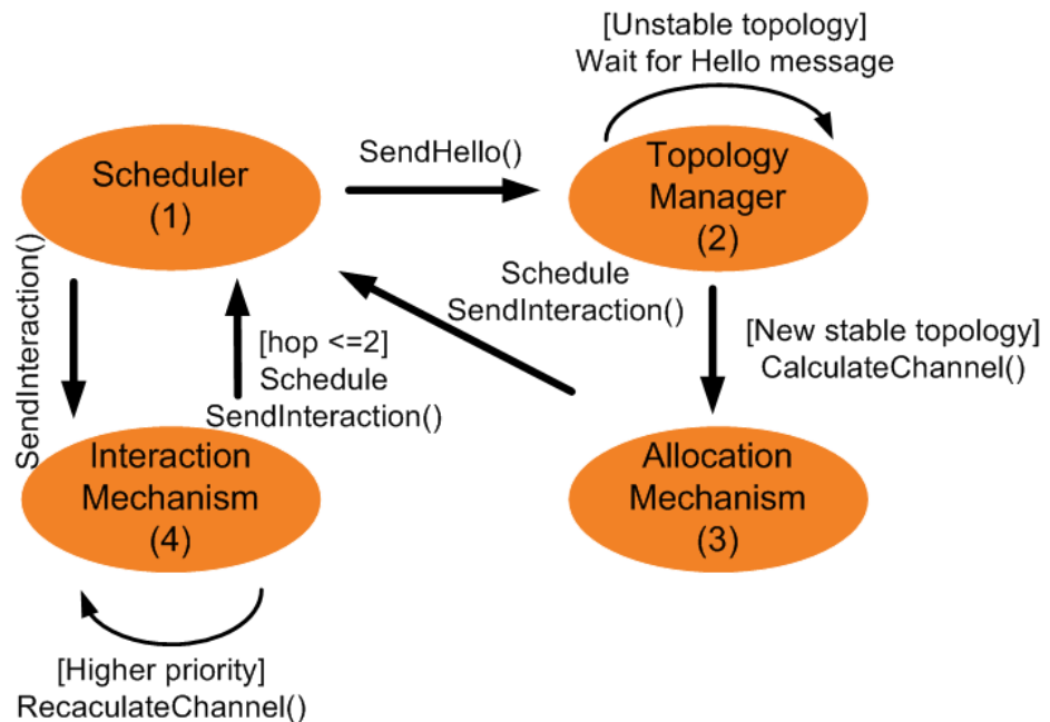
Figure 10: State machine.
