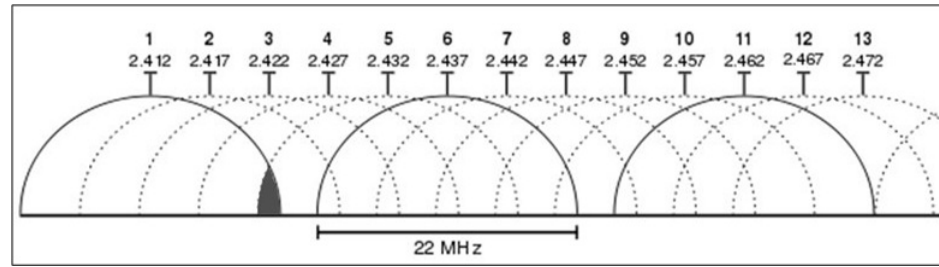
Figure 9: Channels overlapping in WIFI spectrum [98]
