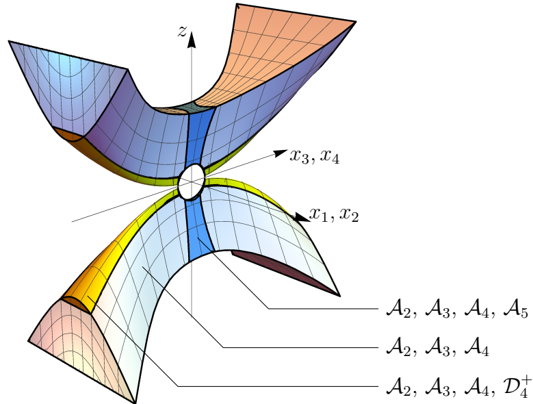
Figure 2.8 – Schematic representation of the three domains of the studied caustic, resulting in the classification.
