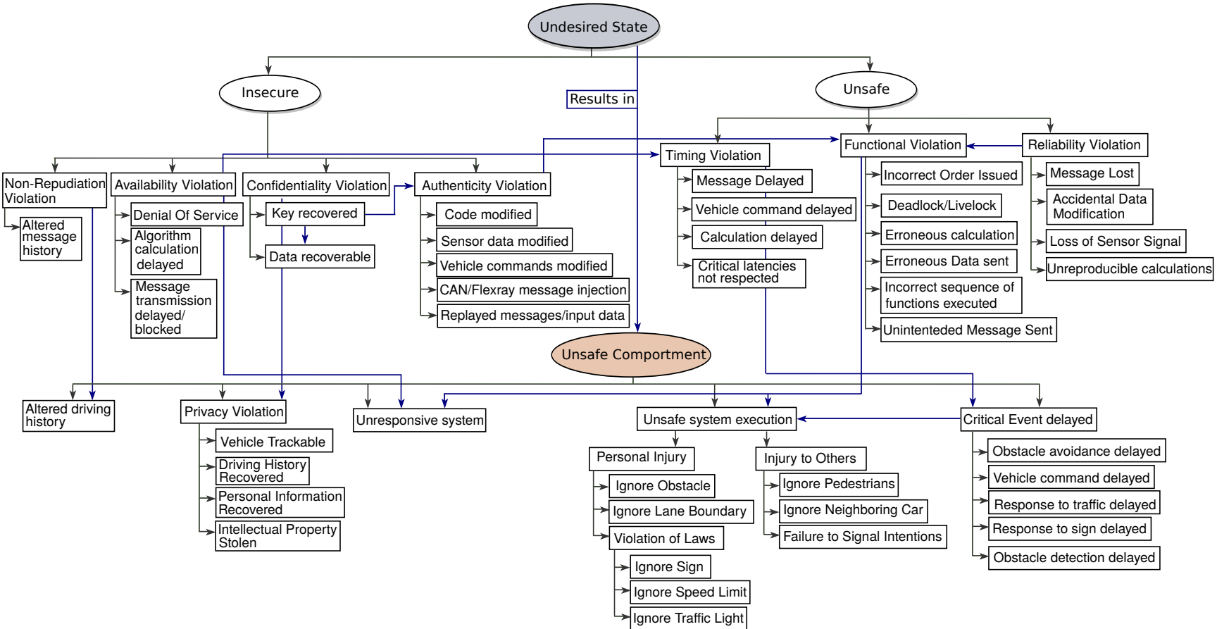
Figure 2-3: Taxonomy for Autonomous Vehicles Part 2
