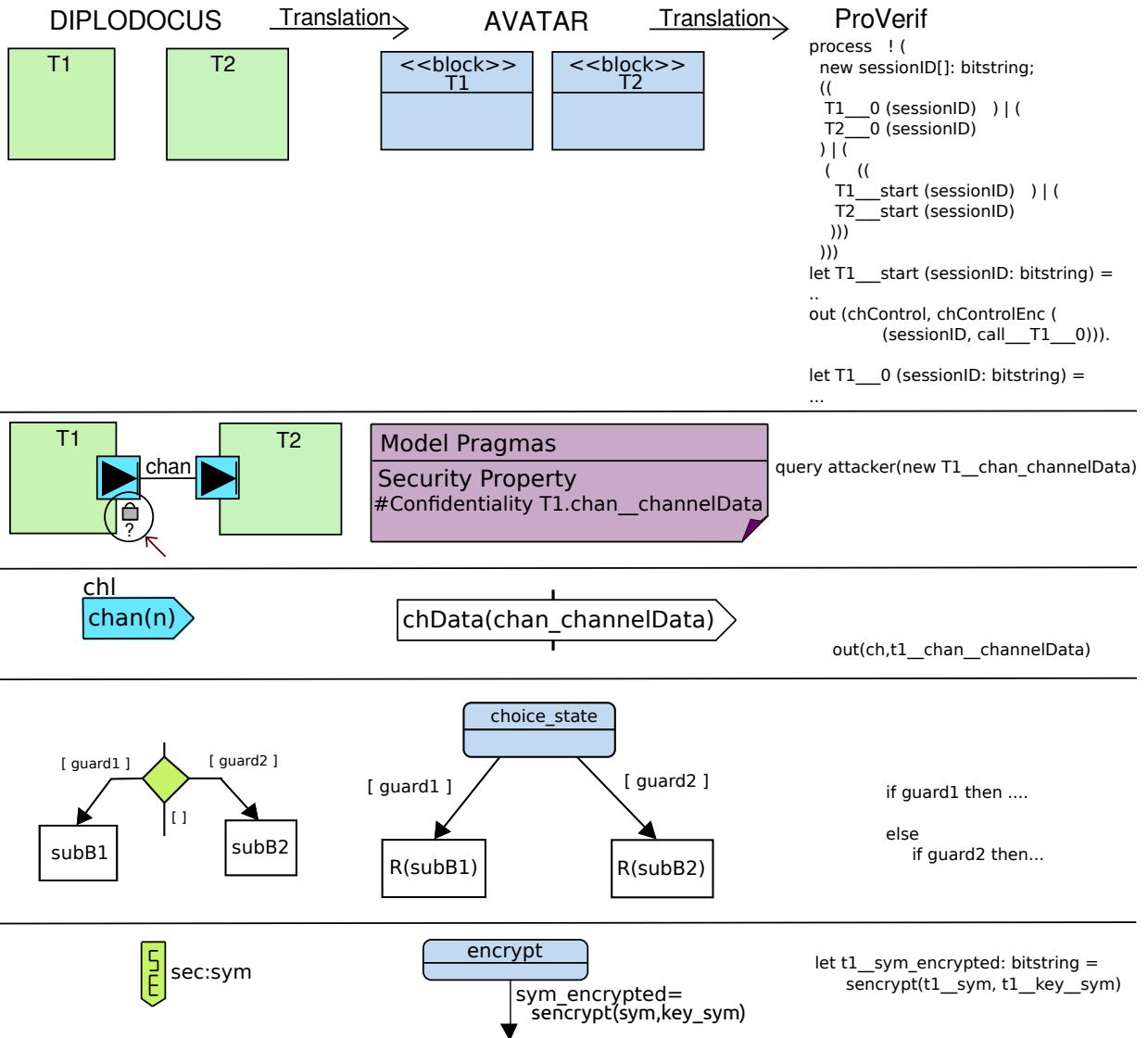
Figure 6-19: Translation of DIPLODOCUS to AVATAR to ProVerif
