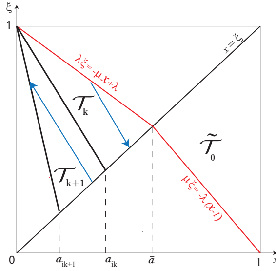
Figure 4.4: Representation of the triangles \mathcal{T}_k
