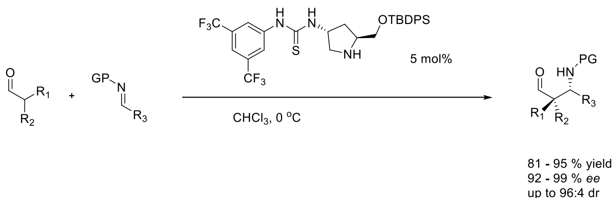
scheme 3-11 chiral bifunctional thiureas catalysed Mannich reaction
