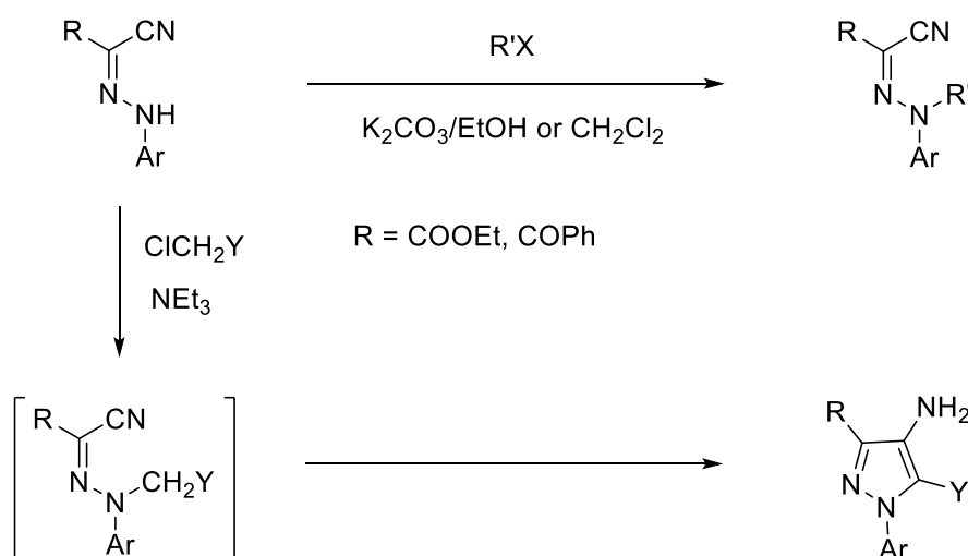
scheme 3-29 N-alkylation reaction
