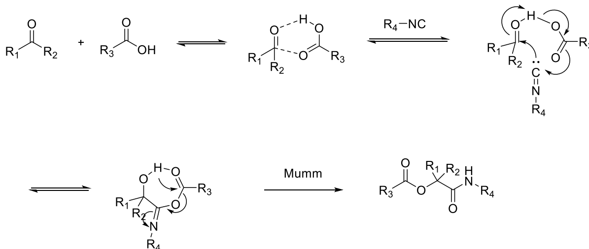
scheme 1-36 mechanism of Passerini reaction
