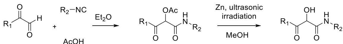
scheme 2-2 O-deacylation
