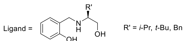
scheme 3-17 strecker reaction
