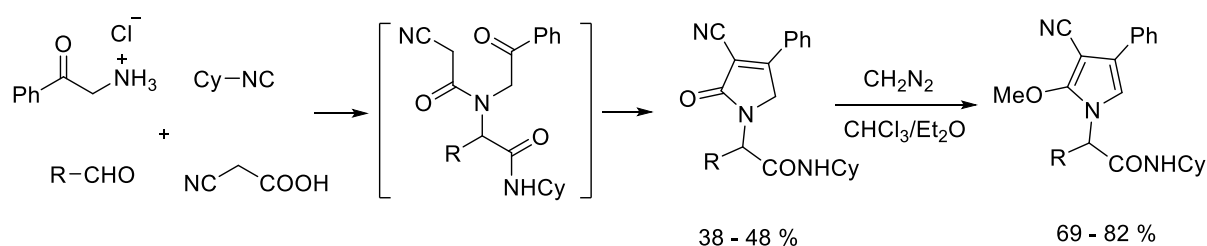
scheme 1-60
