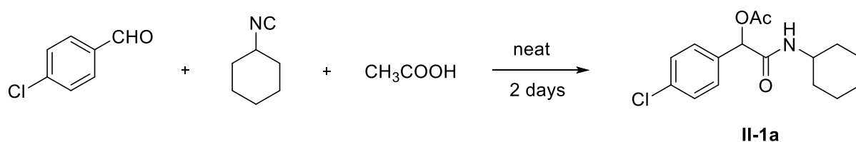
scheme 2-30
