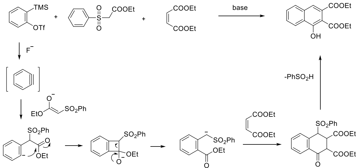
scheme 4-18
