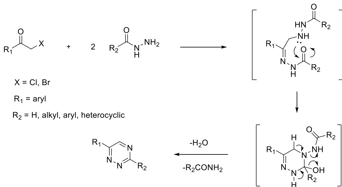
scheme 3-48
