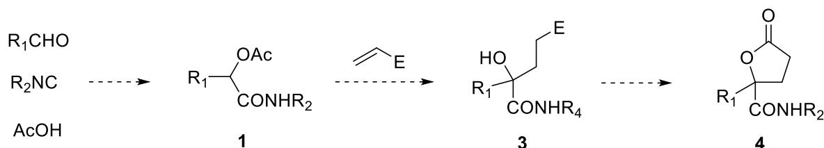
scheme 2-29
