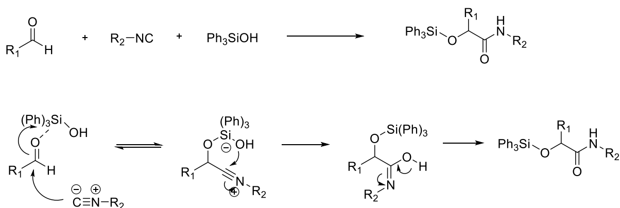
scheme 1-40 O-silylative Passerini reactions
