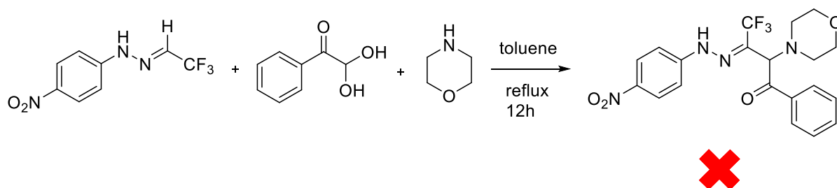
Scheme 3-40
