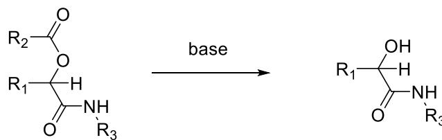
scheme 2-26
