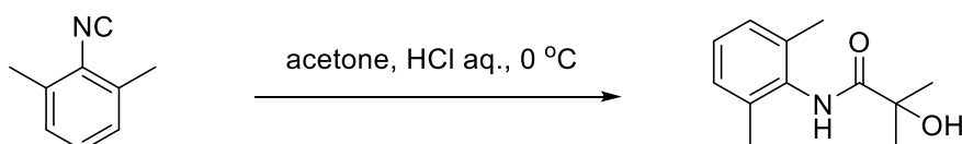
scheme 1-42
