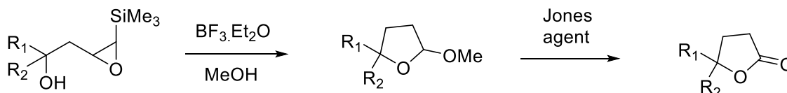
scheme 2-16
