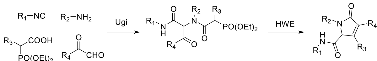
scheme 1-61
