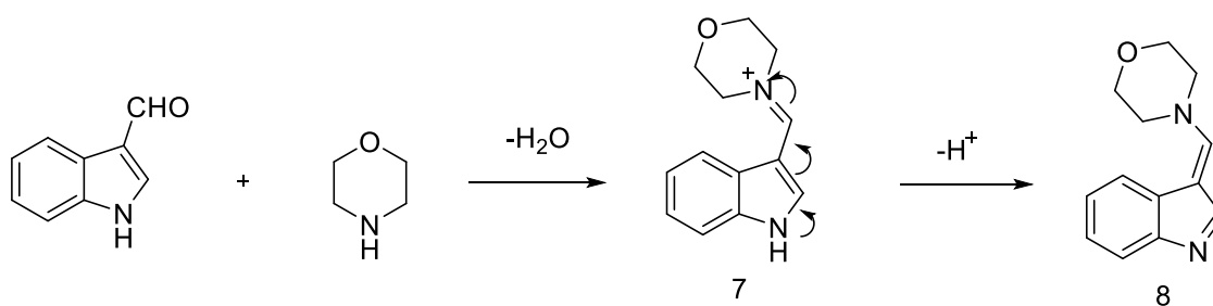
Scheme 3-42
