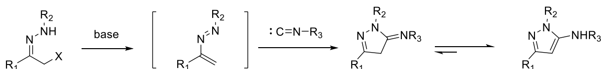
scheme 1-33
