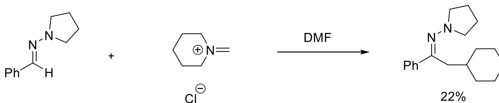
scheme 3-27
