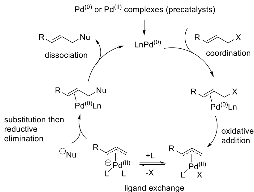
scheme 4-6
