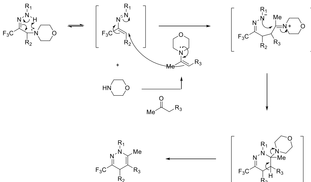
Scheme 3-68 proposed mechanism
