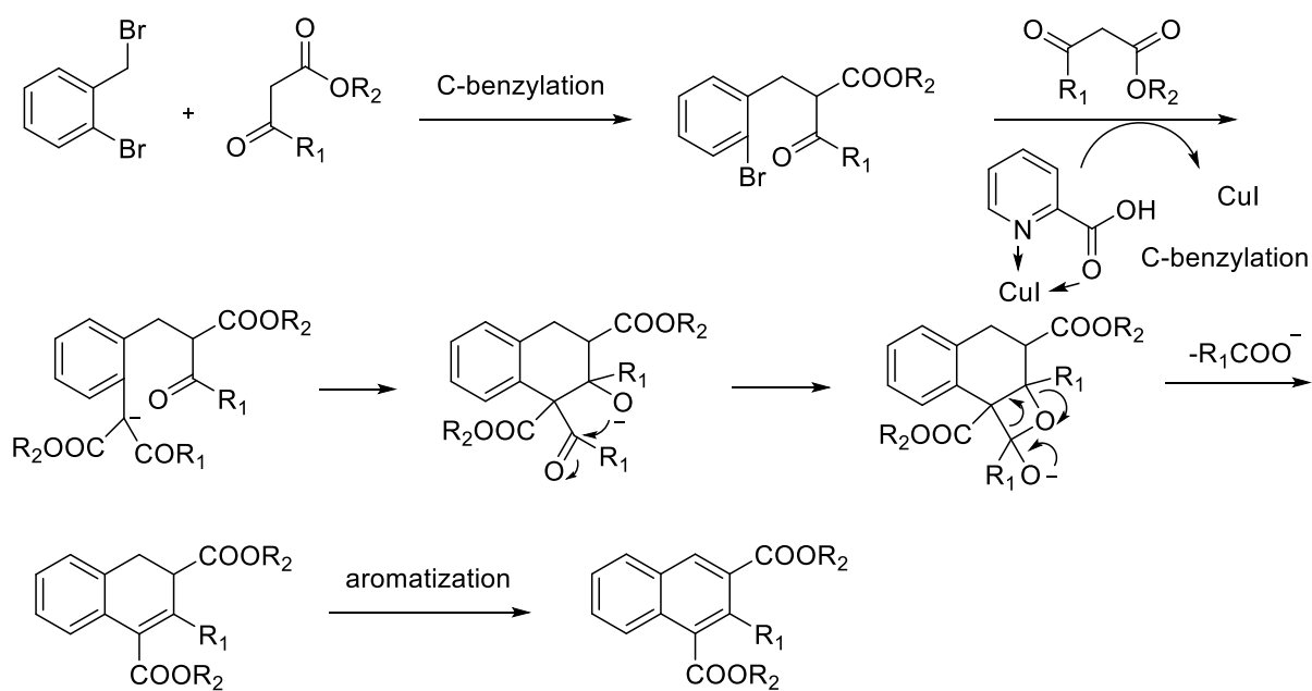
scheme 4-19
