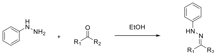
scheme 3-20
