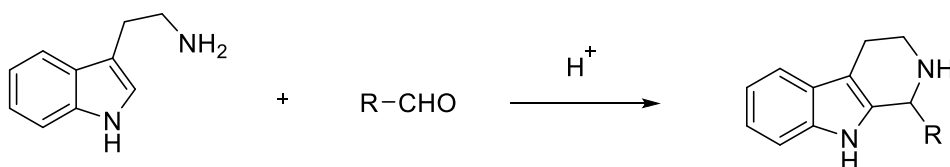
scheme 3-52 Pictet-Spengler type reaction
