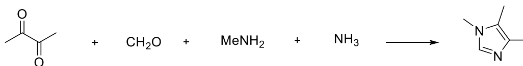
scheme 1-4
