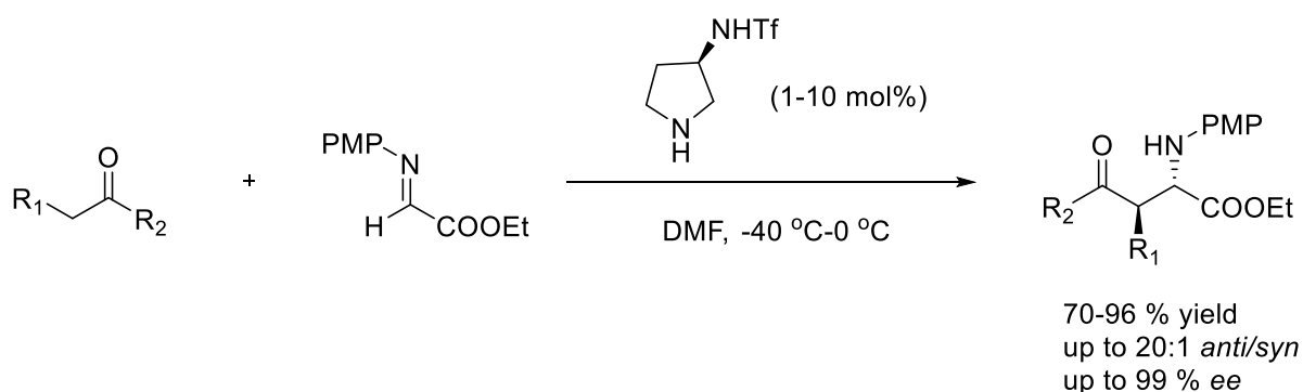
scheme 3-13
