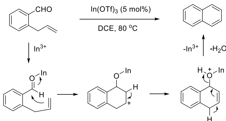
scheme 4-17
