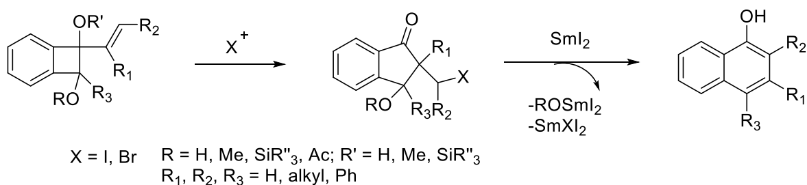
scheme 4-16
