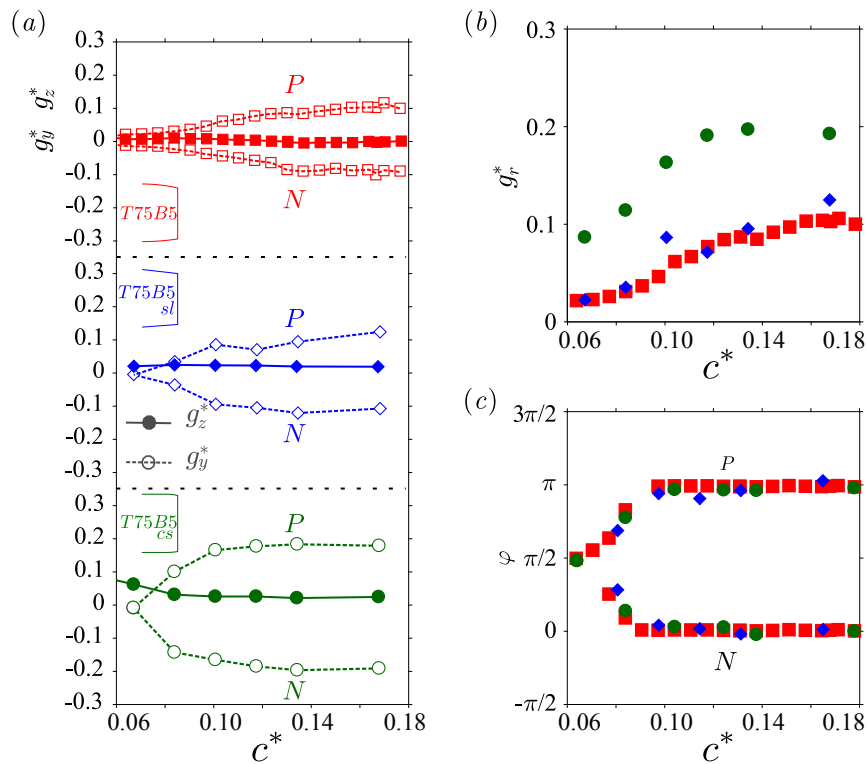
Figure C.9 – Most probable pressure gradients vs. ground clearance c^* for different boat-tails geometry with \theta_T = 7.5^\circ and \theta_B = 5^\circ detailed in table 5.1: g_y^* and g_z^* (a), g_r^* (b) and \varphi (c). The legend of the symbols is given in (a).
