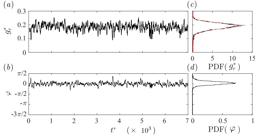
Figure 4.7 – Modulus g_r^*(t^*) (a) and phase \varphi(t^*) (b) time series of the base pressure gradient with corresponding probability density functions (c – d) for \beta = 1.0^\circ . The smooth red line superimposed to \text{PDF}(g_r^*) is a best fit of Rigas et al. (2015)’s PDF model.
