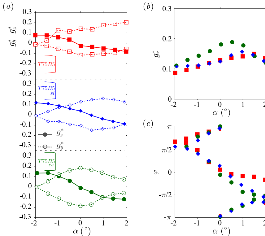
Figure C.11 – Most probable pressure gradients vs. pitch angle \alpha for different boat-tails geometry with \theta_T = 7.5^\circ and \theta_B = 5^\circ detailed in table 5.1: g_y^* and g_z^* (a), g_r^* (b) and \varphi (c). The legend of the symbols is given in (a).
