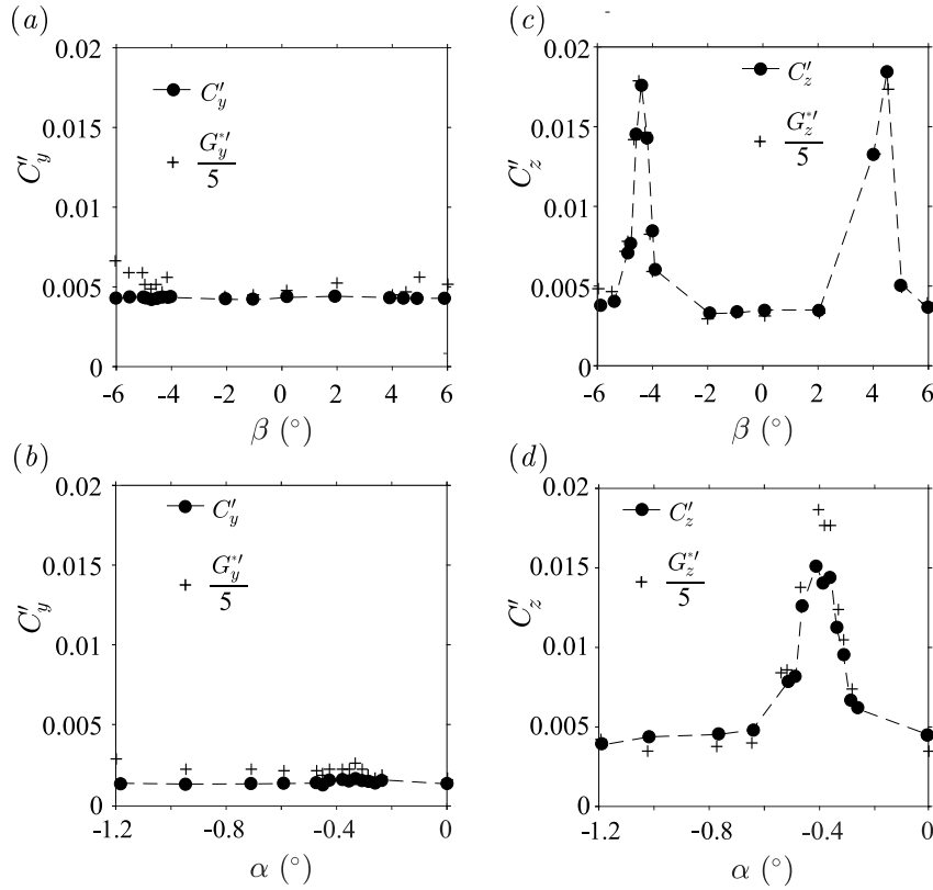
Figure 4.32 – Components of the fluctuating force coefficients C'_y and C'_z (filled circles) compared to the fluctuating base pressure gradient G_y^{*'} and G_z^{*'} (crosses) vs. yaw \beta (top row) and pitch angle \alpha (bottom row) for the boat-tailed geometry.
