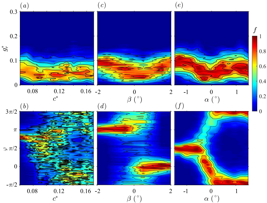
Figure 4.14 – Rear cavity d^* = 0.285 . Base pressure gradient response to ground clearance (a, b) f(c^*, \hat{g}^*) , yaw (c, d) f(\beta, \hat{g}^*) and pitch angle (e, f) f(\alpha, \hat{g}^*) . Sensitivity maps of the gradient modulus g_r^* (a, c, e) and phase \varphi (b, d, f).
