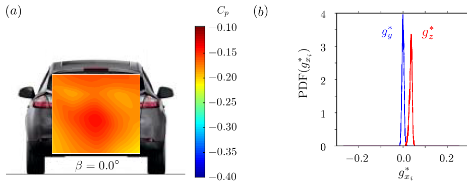
Figure 8.2 – Baseline configuration of the Renault Mégane: (a) Mean base pressure distribution C_p(y^*, z^*) and mean base suction coefficient C_b . (b) Probability Density Functions of the horizontal base pressure gradient g_y^* (in blue) and of the vertical base pressure gradient g_z^* (in red).
