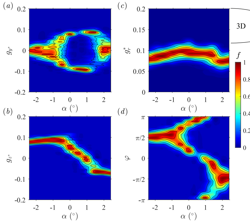
Figure C.19 – Base pressure gradient response to variations of the pitch angle \alpha . Sensitivity maps (a) f(\alpha, g_y^*) , (b) f(\alpha, g_z^*) , (c) f(\alpha, g_r^*) and (d) f(\alpha, \varphi) for the 3D configuration (see table 5.1).
