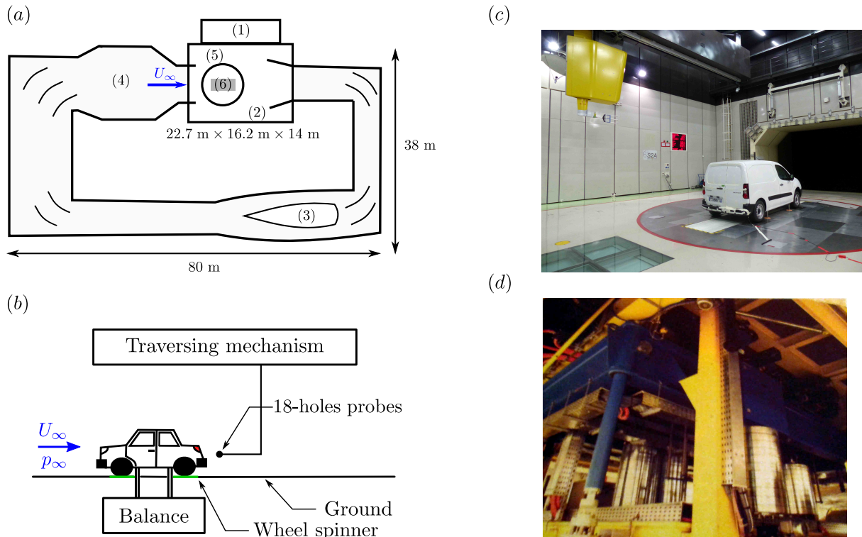
Figure 2.1 – Full-scale wind tunnel of the GIE-S2A: (a) schematic top view with characteristic dimensions. See text for numbers’ description. (b) Schematic side view of the test section with a vehicle and the force balance. (c) Photograph of the plenum with a Peugeot Partner during a test session. (d) The force balance of the full-scale wind tunnel (reproduced from Déleroy et al. (2017)).
