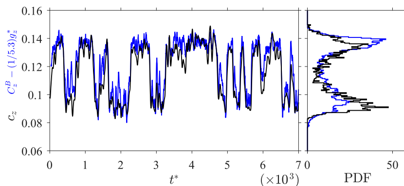
Figure 7.21 – Time series of the lift coefficient c_z(t^*) for the Citroën Berlingo in the bi-stable case under pitching conditions ( left ) with the corresponding probability density function ( right ). The black line is the value measured by the force balance and the blue line is the reconstructed value from equation (7.4b) using \xi = 1/5.3 .
