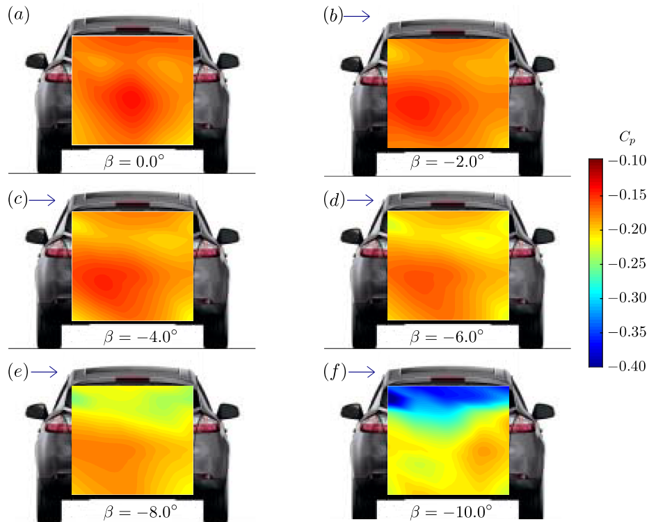
Figure 8.4 – Mean base pressure distributions C_p(y^*, z^*) for the Renault Mègane under yawing conditions: (a) Baseline \beta = 0.0^\circ , (b) \beta = -2.0^\circ , (c) \beta = -4.0^\circ , (d) \beta = -6.0^\circ , (e) \beta = -8.0^\circ , (f) \beta = -10.0^\circ . The horizontal arrow stands for the lateral component of the velocity U_\infty \sin(\beta) of the wind (not to scale).
