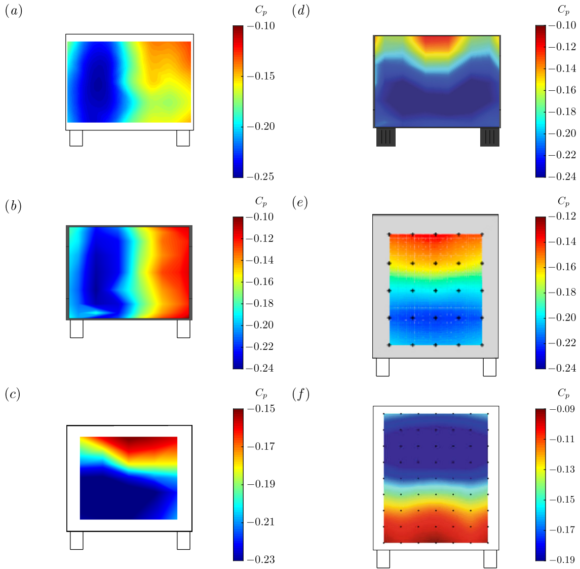
Figure 1.5 – Base pressure distributions of bluff bodies subject to static wake instabilities. y -wake asymmetry: (a) for the squareback Ahmed body at the industrial scale (adapted from Grandemange et al. (2015)) and (b) for a Windsor body (adapted from Perry et al. (2016b)). Only states P are shown. z -wake asymmetry: (c) for the squareback Ahmed body with underbody disturbances (adapted from Barros et al. (2017)) and (d) for a Windsor body with wheels (adapted from Pavia & Passmore (2018)). Only states P are shown. GTS model displaying (e) P state (adapted from Castelain et al. (2018)) and (f) N state (adapted from van Raemdonck et al. (2016)).
