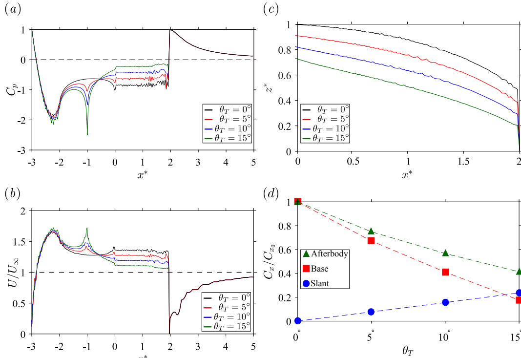
Figure 5.5 – Wake simulation based on the Free Streamline Theory with length of the recirculation bubble set to 2H and slant length to \ell_S = H . (a) Pressure distribution and (b) velocity magnitude along the body and the separating streamline; the dashed line stands for free-stream conditions. (c) Geometry of the separating streamline for \theta_T \in \{0^\circ, 5^\circ, 10^\circ, 15^\circ\} after the iterative process is terminated. (d) Contribution to the drag coefficient of the whole afterbody (green triangles), of the slant (blue dots) and of the vertical base (red squares) compared to the total drag of the squareback geometry C_{x_0} .
