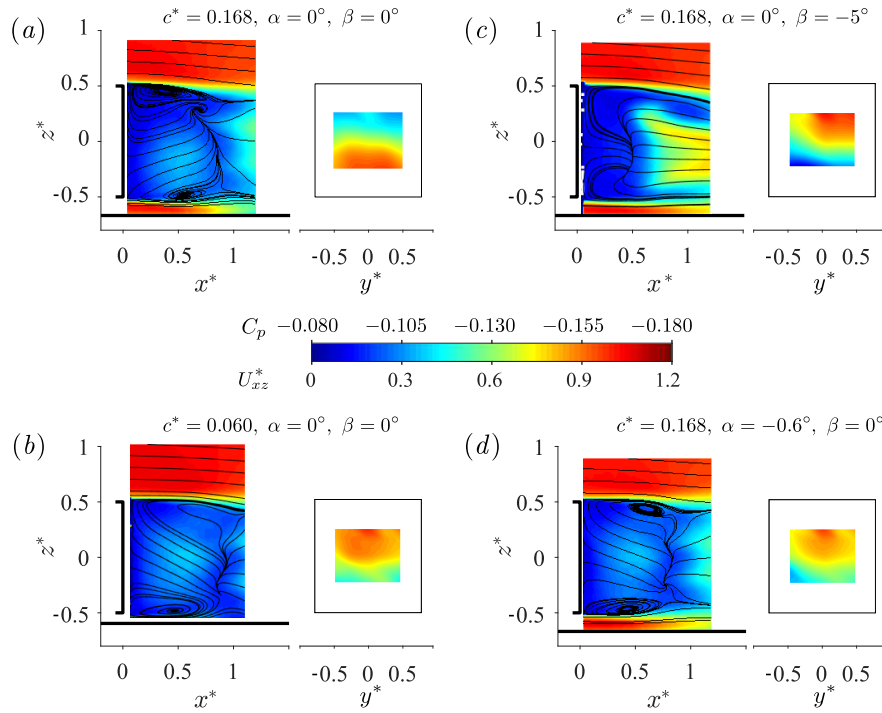
Figure 4.28 – Cross-sections of the mean velocity field visualized using streamlines superimposed to the modulus of the components in the vertical plane ( x^*, z^* ) for (a) baseline configuration ( \alpha = \beta = 0^\circ , c^* = 0.168 ), (b) \alpha = \beta = 0^\circ , c^* = 0.060 , (c) \alpha = 0^\circ , \beta = -5^\circ , c^* = 0.168 , (d) nose-down configuration \alpha = -0.6^\circ ( \beta = 0^\circ ). The associated mean base pressure distributions C_p(y^*, z^*) are also provided.
