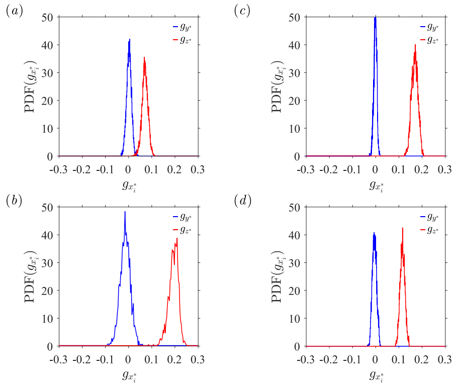
Figure 7.4 – Probability density functions of the Cartesian components of the base pressure gradient in the baseline configuration with open air-intake (blue horizontal gradient g_{y^*} and red vertical gradient g_{z^*} ): (a) Peugeot 5008, (b) Renault Kangoo, (c) Peugeot Partner and (d) Citroën Berlingo.
