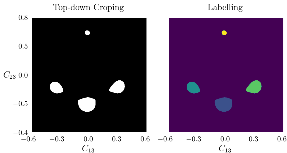
Figure B.2: Maxima locations identification. (left) Identification of multiple peaks of the landscape as white shapes. (right) Ranking of different peaks in order to analyze them separately.
